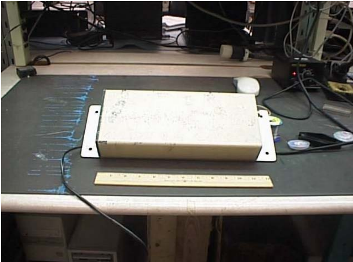
Photograph 4 – Antenna Overview
