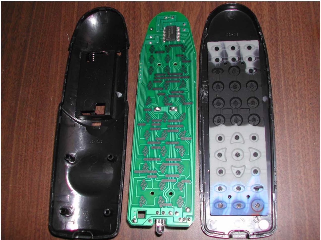
FIGURE 7: PLI Photograph Number 5392C2633SJ-15 illustrates the disassembled remote control and the circuit side of the remote control printed circuit assembly (assembly number S-251G203).
