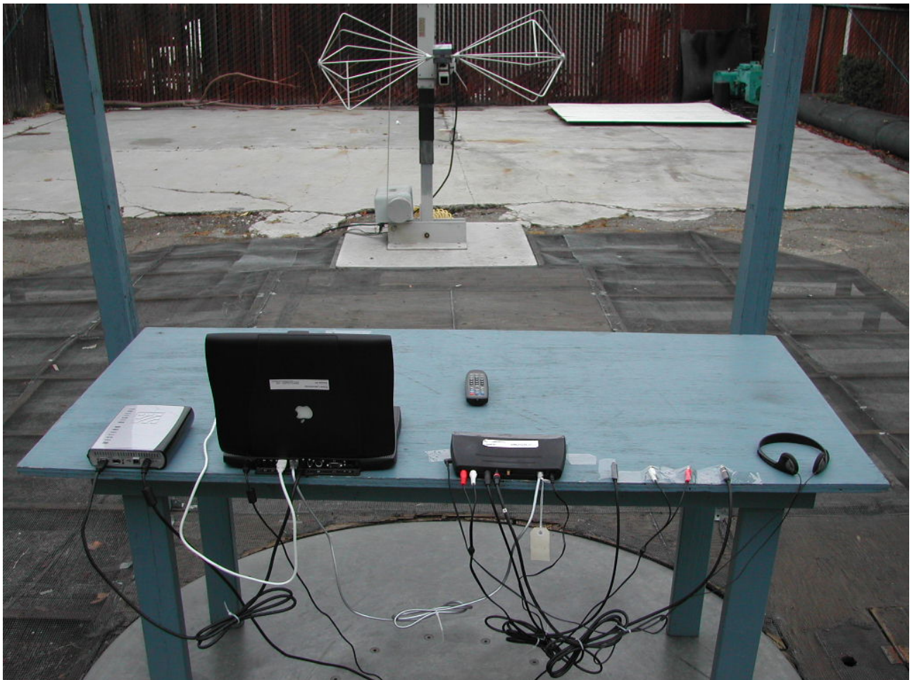
FIGURE 1: PLI Photograph Number 5392C3333SJ-02 illustrates the rear view of the Equipment Under Test in Radiated Electromagnetic Interference Test Configuration #1.
