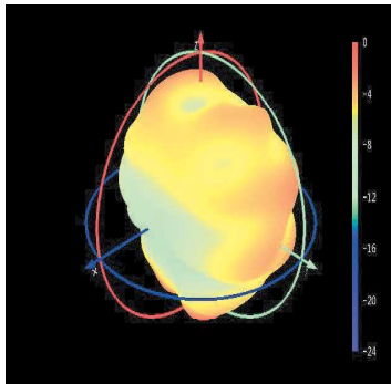
Theta=90 freq=2440MHz
