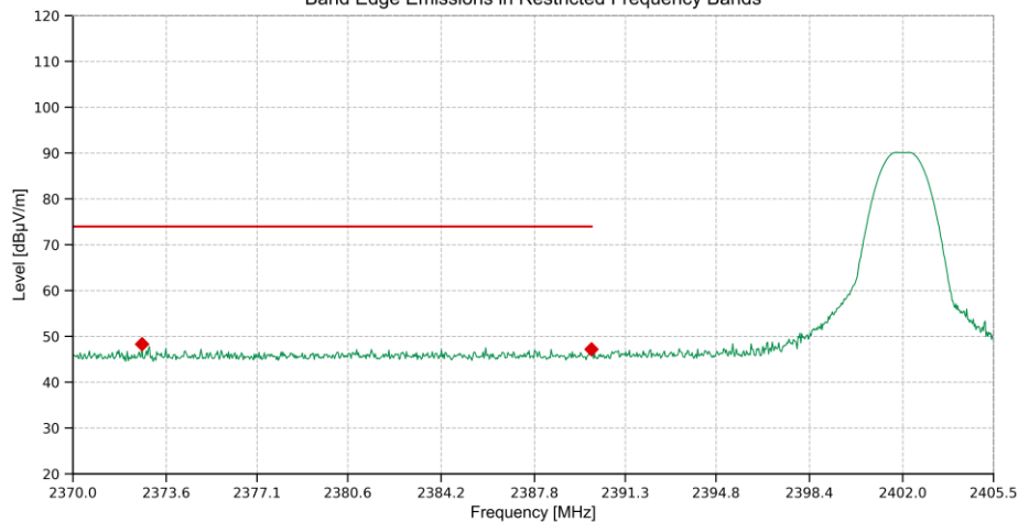
Band Edge Emissions in Restricted Frequency Bands
