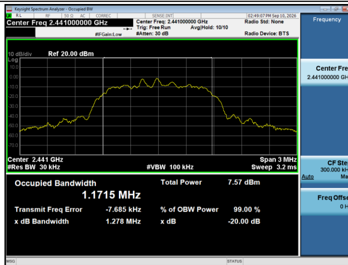
2DHS_Ant1_2441
