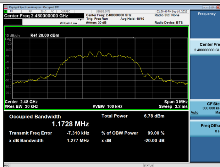
2DHS_Ant1_2480
