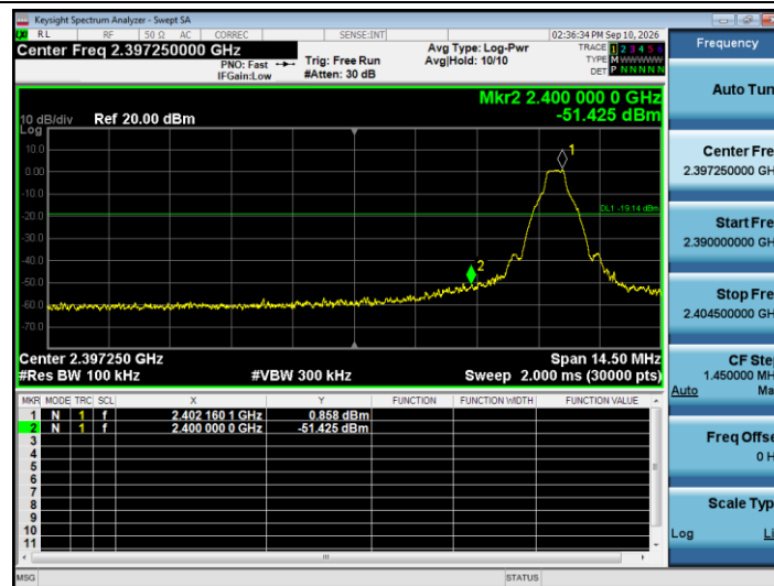
DH5_Ant1_2402_Low
