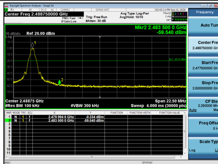
DH5_Ant1_2480_High
