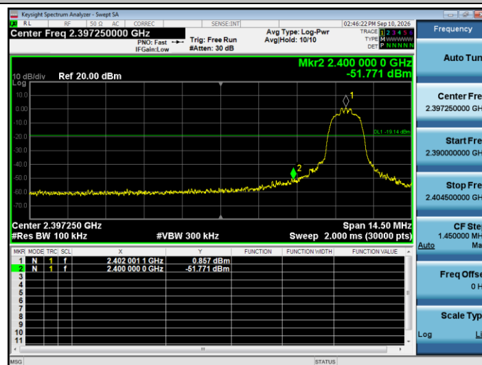
2DH5_Ant1_2402_Low
