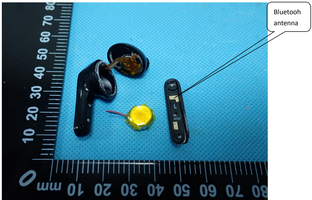
Internal Photo 2
