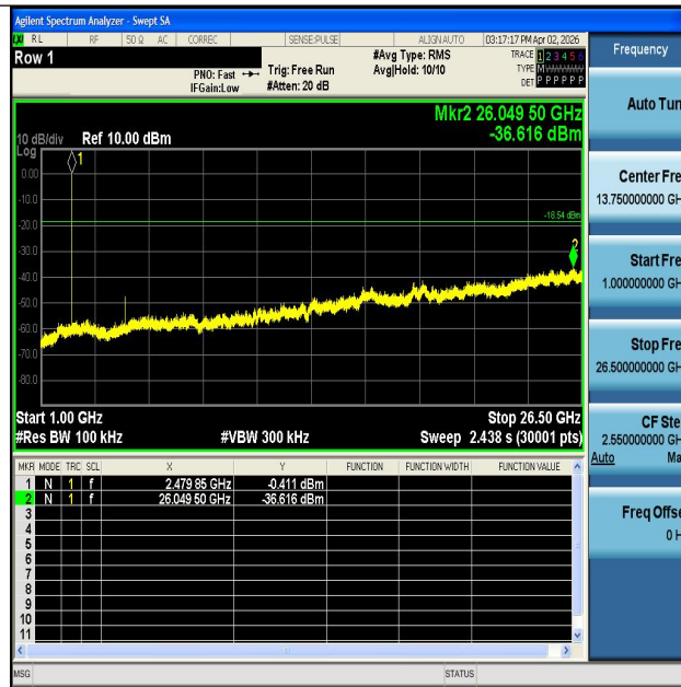
BLE_1M-Ant1-2480-1000~26500-PASS
