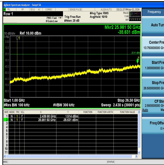
BLE_2M-Ant1-2440-1000~26500-PASS
