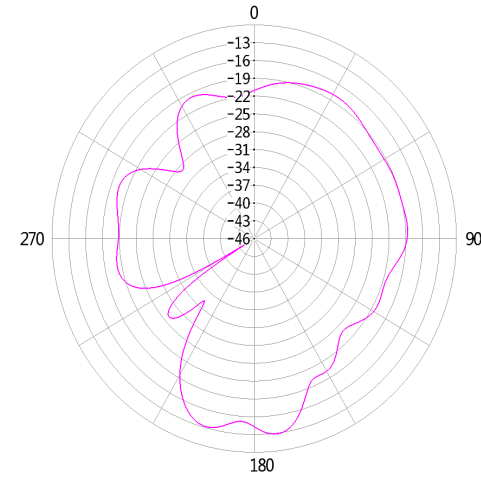
Phi= 90(Y0Z)
