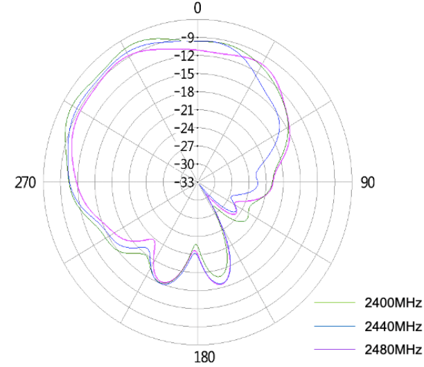
\Phi = 90 (Y0Z)
