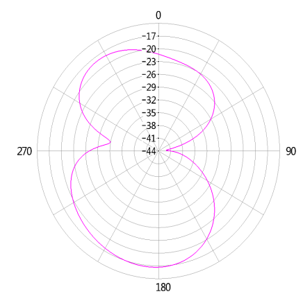
Theta= 90(X0Y)
