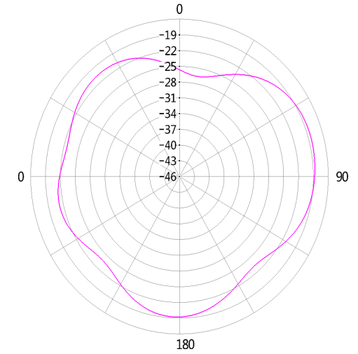
Theta= 90(X0Y)
