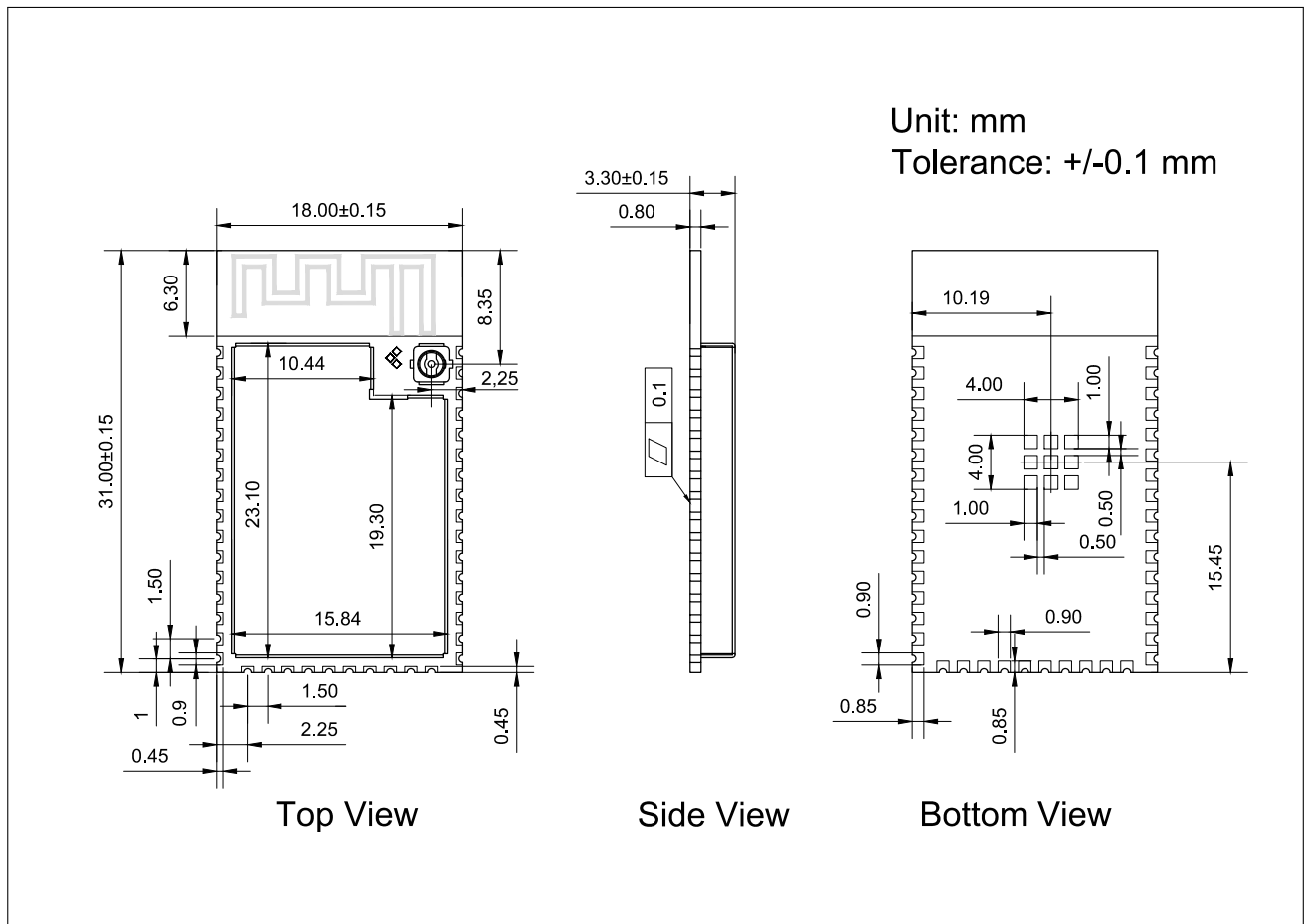
Figure 6: Physical Dimensions
