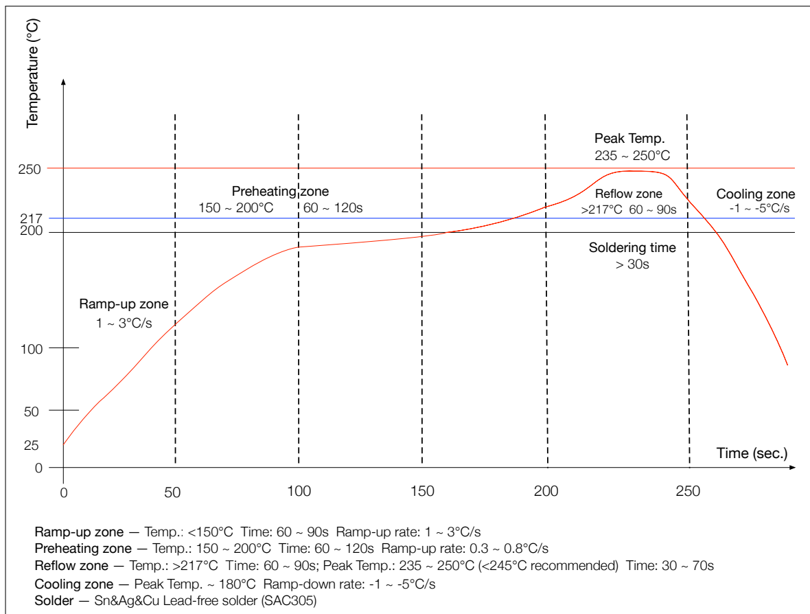
Figure 9: Reflow Profile
