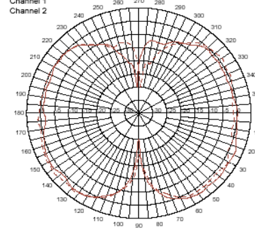
Elevation Cut
