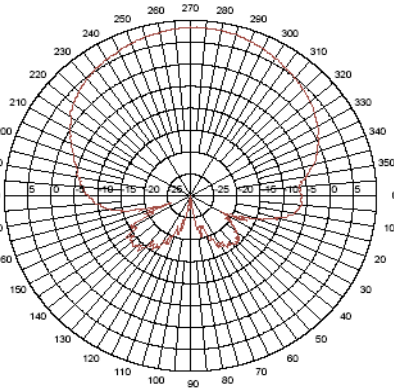
2.3-2.5 Azimuth Cut
