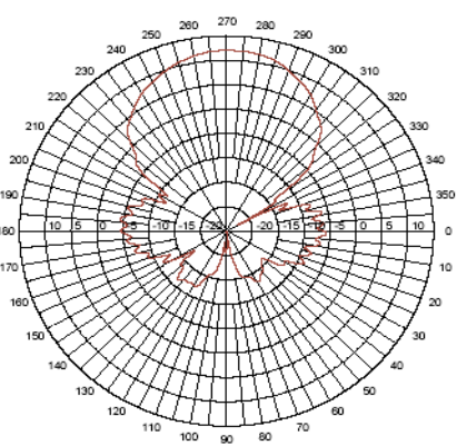
Elevation Cut
