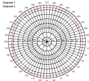
Azimuth Cut
