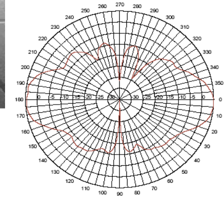
Elevation Cut
