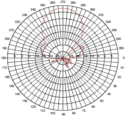
Elevation Cut
