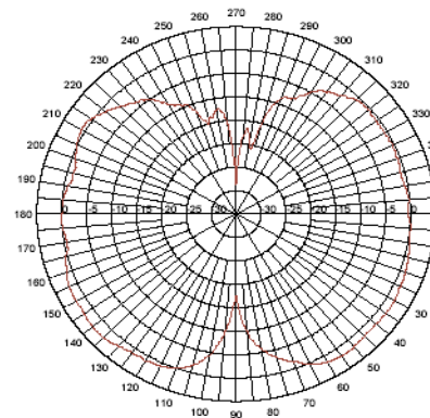
Elevation Cut
