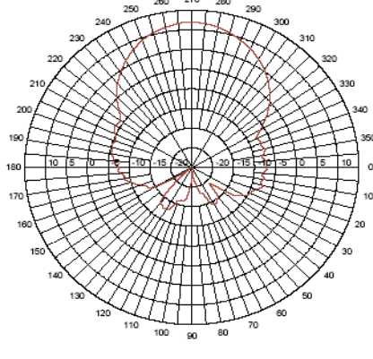
Azimuth Cut
