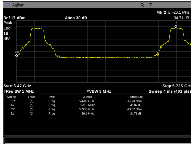
Plot 298. Frequency Stability, 5470 – 5725 MHz, 50°C, 120 V
