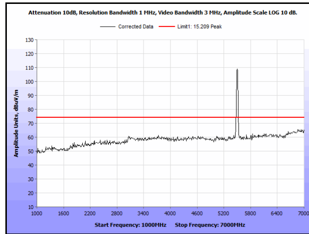
Plot 268. Radiated Spurs, Co-Location, 802.11n 20 MHz, 5580 MHz & 5580 MHz, 1 GHz – 7 GHz, Peak
