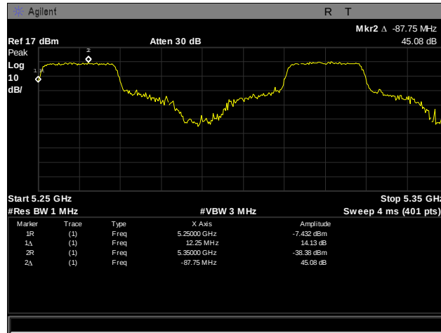
Plot 284. Frequency Stability, 5250 – 5350 MHz, 20°C, 120 V
