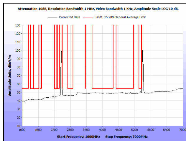
Plot 231. Radiated Spurs, Co-Location, 802.11n 20 MHz, 2462 MHz & 5580 MHz, 1 GHz – 7 GHz, Avg.
