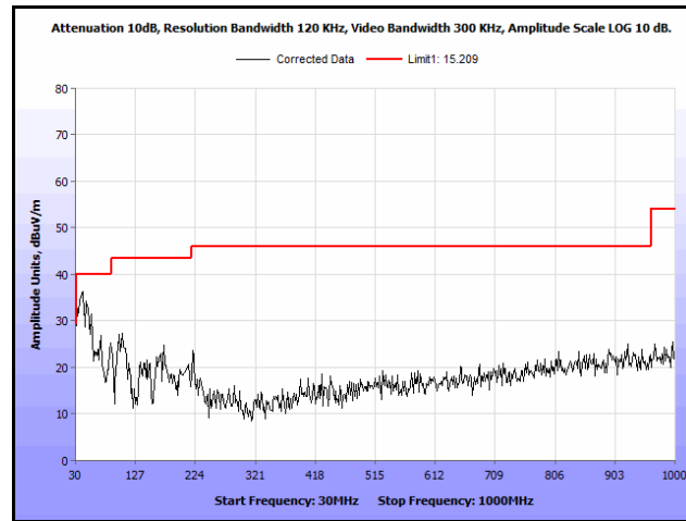
Plot 226. Radiated Spurs, Co-Location, 802.11n 20 MHz, 2462 MHz & 5300 MHz, 30 MHz – 1 GHz, Peak
