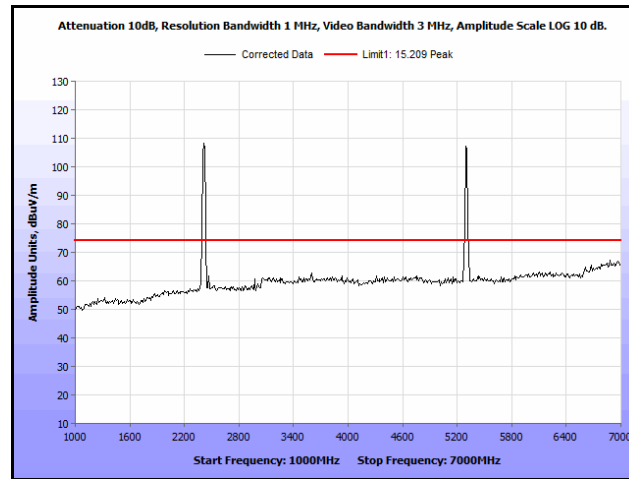
Plot 196. Radiated Spurs, Co-Location, 802.11n 20 MHz, 2412 MHz & 5300 MHz, 1 GHz – 7 GHz, Peak
