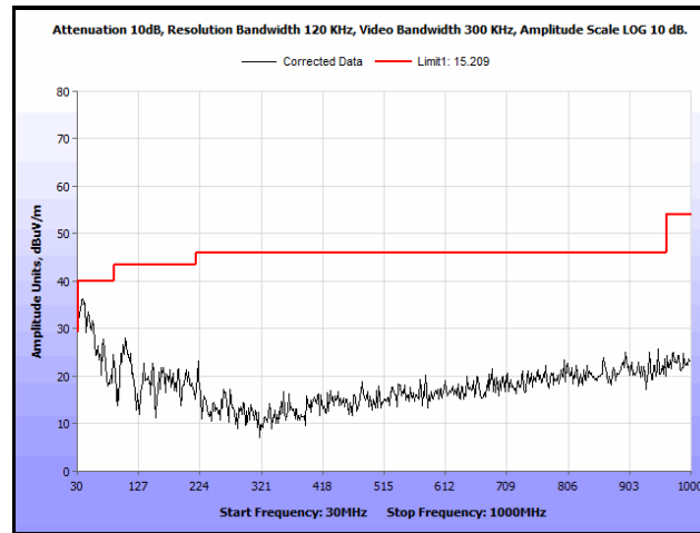
Plot 238. Radiated Spurs, Co-Location, 802.11n 20 MHz, 5200 MHz & 5200 MHz, 30 MHz – 1 GHz, Peak
