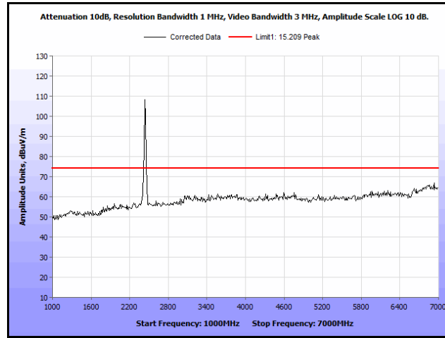
Plot 184. Radiated Spurs, Co-Location, 802.11n 20 MHz, 2437 MHz & 2462 MHz, 1 GHz – 7 GHz, Peak
