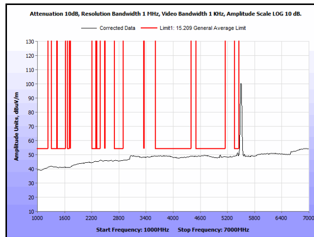
Plot 267. Radiated Spurs, Co-Location, 802.11n 20 MHz, 5580 MHz & 5580 MHz, 1 GHz – 7 GHz, Avg.
