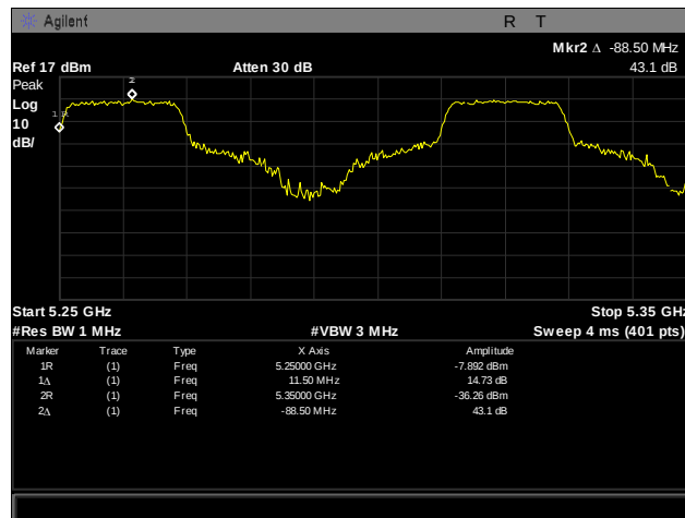
Plot 286. Frequency Stability, 5250 – 5350 MHz, 40°C, 120 V
