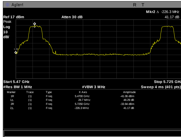
Plot 292. Frequency Stability, 5470 – 5725 MHz, -10°C, 120 V
