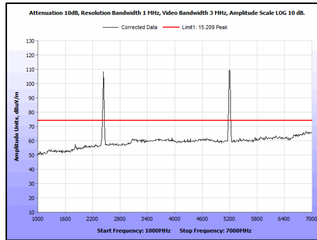
Plot 208. Radiated Spurs, Co-Location, 802.11n 20 MHz, 2437 MHz & 5200 MHz, 1 GHz – 7 GHz, Peak
