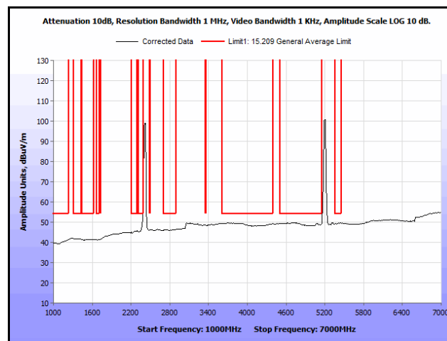
Plot 191. Radiated Spurs, Co-Location, 802.11n 20 MHz, 2412 MHz & 5200 MHz, 1 GHz – 7 GHz, Avg.
