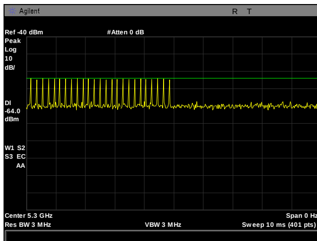
Plot 309. Radar Type 2 Calibration, 5300 MHz
