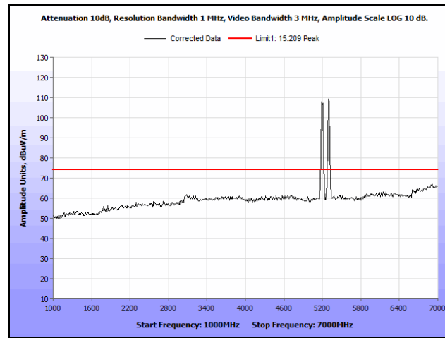
Plot 244. Radiated Spurs, Co-Location, 802.11n 20 MHz, 5200 MHz & 5300 MHz, 1 GHz – 7 GHz, Peak
