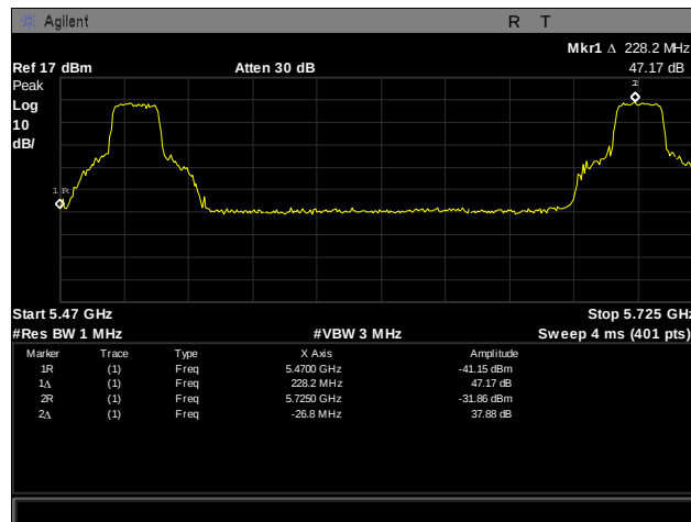
Plot 294. Frequency Stability, 5470 – 5725 MHz, 10°C, 120 V
