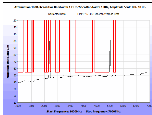
Plot 207. Radiated Spurs, Co-Location, 802.11n 20 MHz, 2437 MHz & 5200 MHz, 1 GHz – 7 GHz, Avg.
