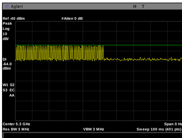
Plot 308. Radar Type 1 Calibration, 5300 MHz
