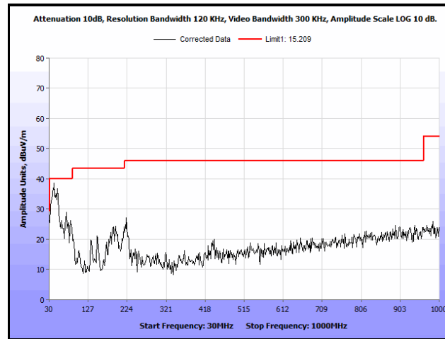
Plot 190. Radiated Spurs, Co-Location, 802.11n 20 MHz, 2412 MHz & 5200 MHz, 30 MHz – 1 GHz, Peak
