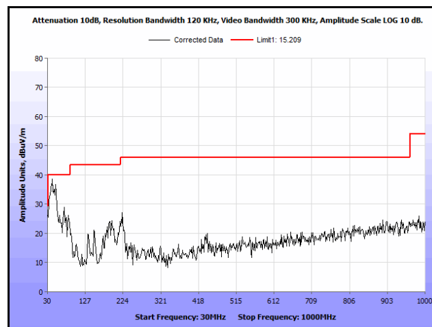
Plot 246. Radiated Spurs, Co-Location, 802.11n 20 MHz, 5200 MHz & 5580 MHz, 30 MHz – 1 GHz, Peak
