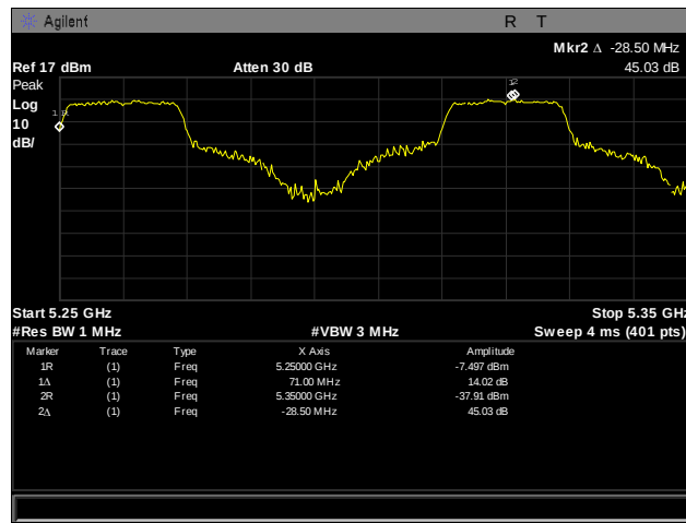
Plot 285. Frequency Stability, 5250 – 5350 MHz, 30°C, 120 V
