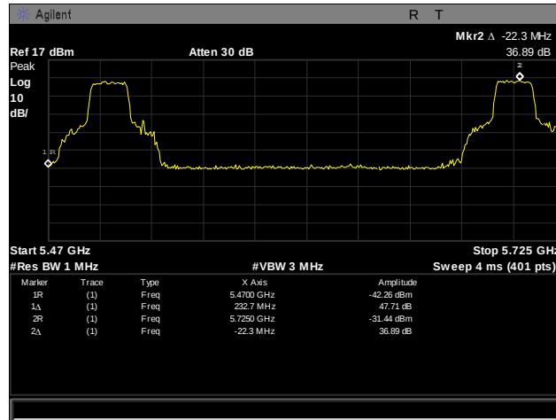
Plot 295. Frequency Stability, 5470 – 5725 MHz, 20°C, 120 V
