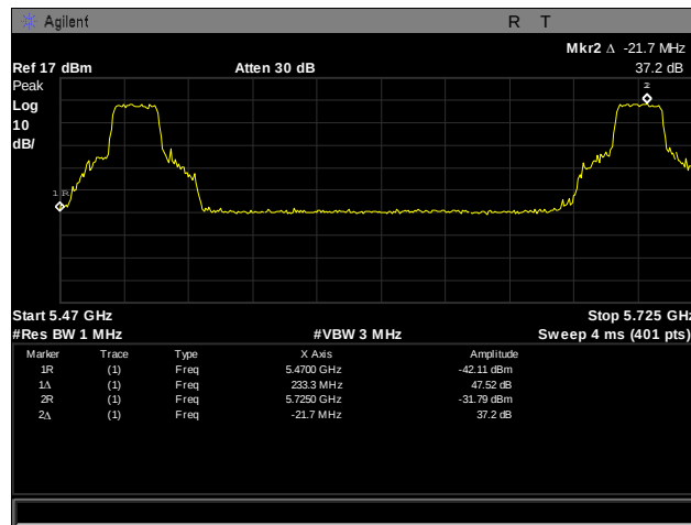
Plot 296. Frequency Stability, 5470 – 5725 MHz, 30°C, 120 V
