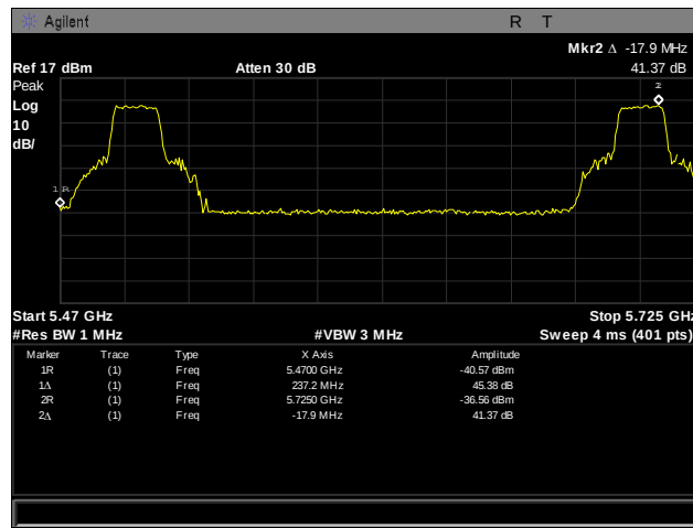
Plot 293. Frequency Stability, 5470 – 5725 MHz, 0°C, 120 V
