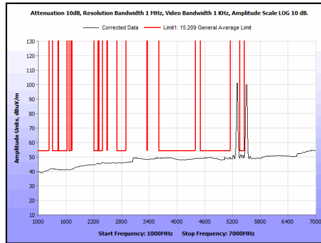
Plot 259. Radiated Spurs, Co-Location, 802.11n 20 MHz, 5300 MHz & 5580 MHz, 1 GHz – 7 GHz, Avg.
