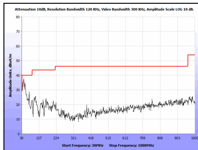
Plot 210. Radiated Spurs, Co-Location, 802.11n 20 MHz, 2437 MHz & 5300 MHz, 30 MHz – 1 GHz, Peak
