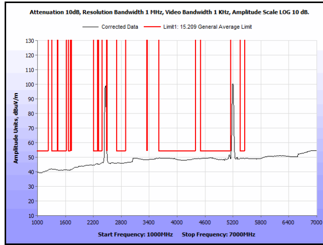
Plot 223. Radiated Spurs, Co-Location, 802.11n 20 MHz, 2462 MHz & 5200 MHz, 1 GHz – 7 GHz, Avg.
