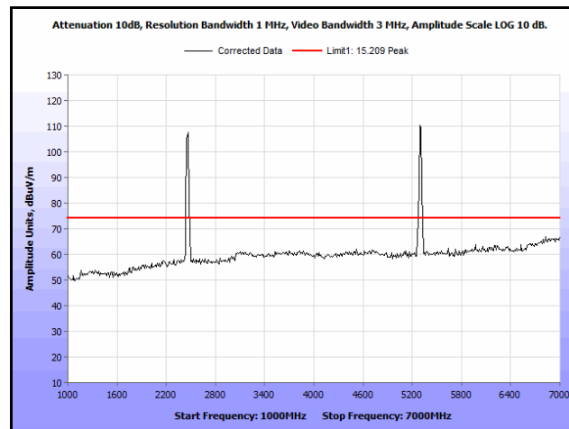
Plot 228. Radiated Spurs, Co-Location, 802.11n 20 MHz, 2462 MHz & 5300 MHz, 1 GHz – 7 GHz, Peak
