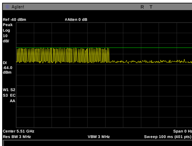
Plot 315. Radar Type 1 Calibration, 5510 MHz
