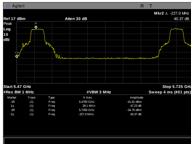
Plot 297. Frequency Stability, 5470 – 5725 MHz, 40°C, 120 V
