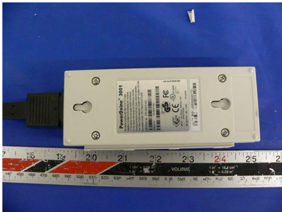
Power Injector – Rear View
