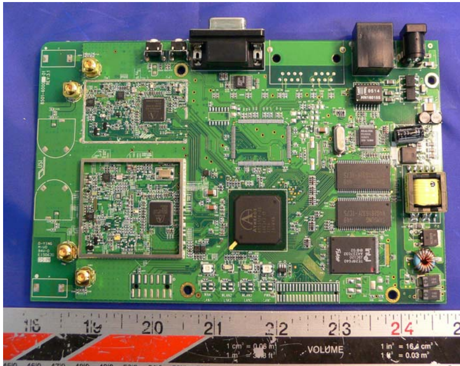
EUT Component Side With RF Shield Off - Top View
