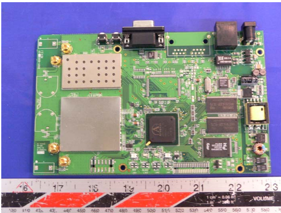
EUT Component Side - Top View
