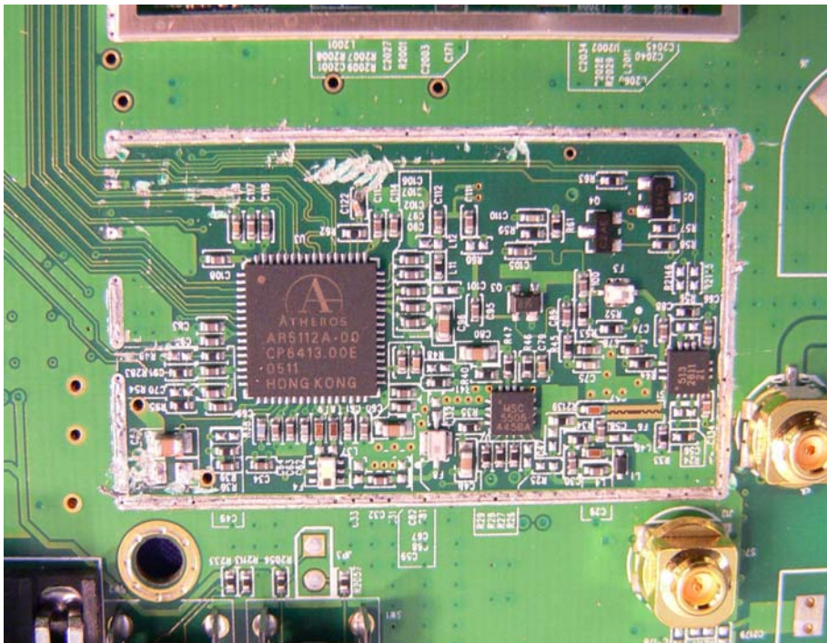
RF 2 With Shield Off - Top View
