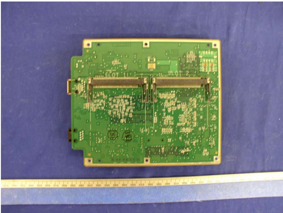
Main Board Bottom View without Radio Board
