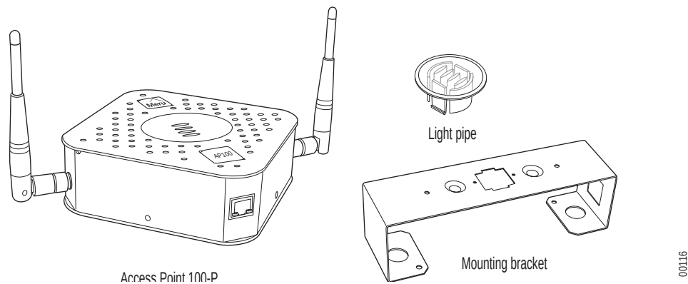
Figure 7: AP100-P Plenum Installation Items
