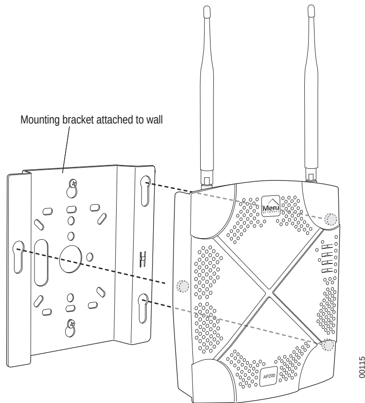
Figure 16: Aligning the AP200 with the Bracket
