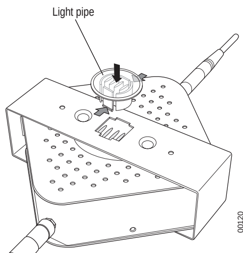
Figure 8: Light-Pipe Extender Attached to Bracket
