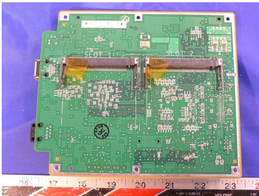
Solder Side - Back View
