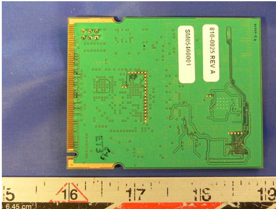
Solder Side With Two Radio Plug in - Back View
