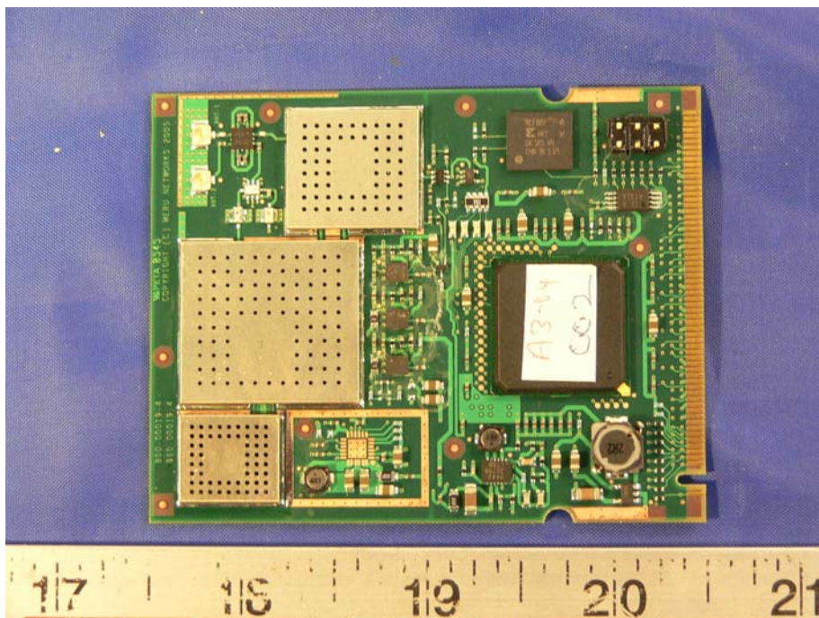
Radio 1 Board - Top View
