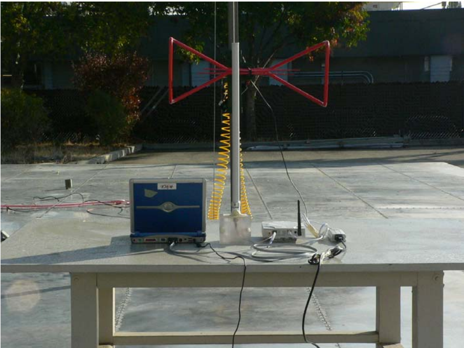
Radiated Emission – Rear View (MaxRad Dualband ( 6 dBi ))
