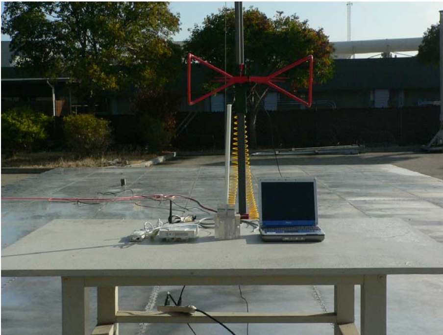
Radiated Emission – Rear View (SmartAnt 2.4 to 2.5 Ghz ( 8 dBi ))
