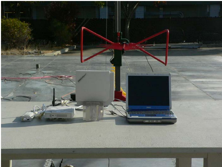
Radiated Emission – Rear View (MaxRad Antenna 2.4 to 2.5 Ghz ( 13 dBi ))
