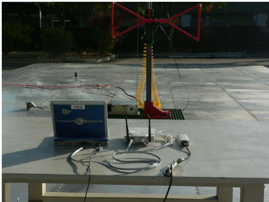
Radiated Emission – Rear View (Regular Antenna)
