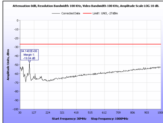
Plot 188. Radiated Spurious Emissions, 802.11a, 5300 MHz, 30 MHz – 1 GHz, 2 dBi Dipole Antenna
