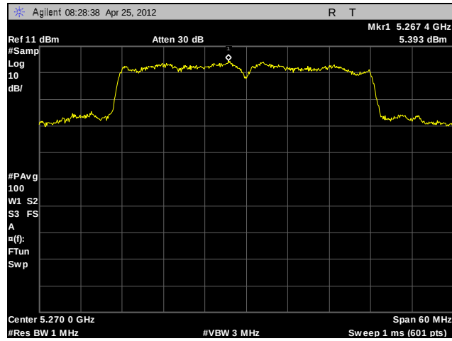
Plot 137. Power Spectral Density, 802.11n 40 MHz, A4, 5270 MHz
