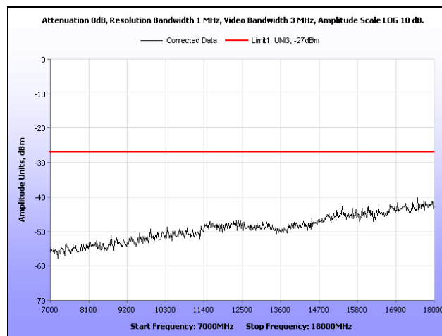
Plot 367. Radiated Spurious Emissions, 802.11n 40 MHz, 5270 MHz, 7 GHz – 18 GHz, Ceiling Mount
