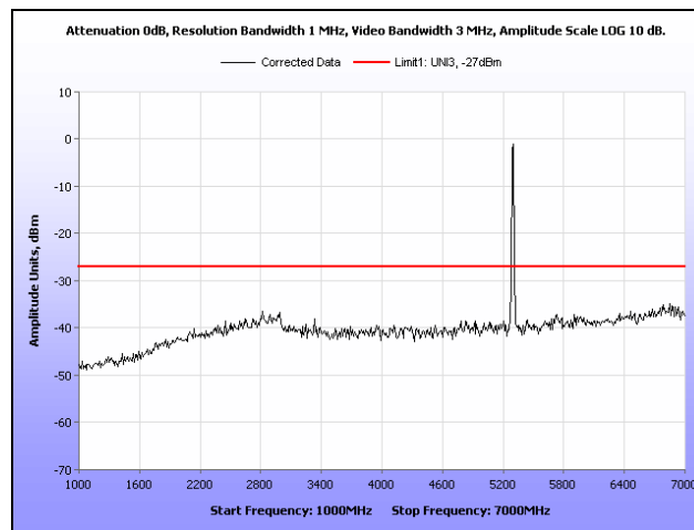
Plot 333. Radiated Spurious Emissions, 802.11a, 5300 MHz, 1 GHz – 7 GHz, Ceiling Mount
