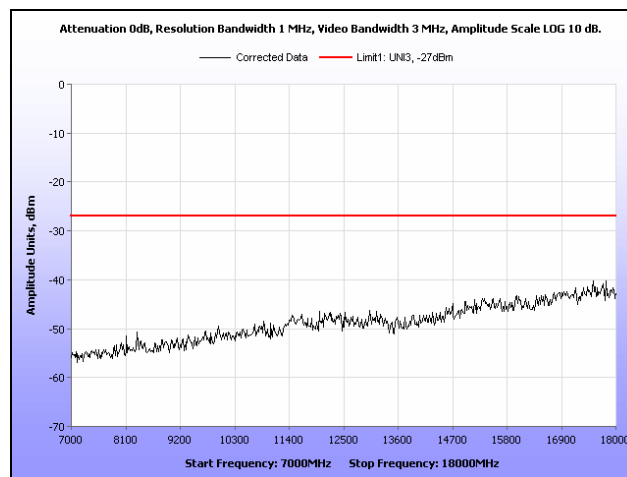
Plot 337. Radiated Spurious Emissions, 802.11a, 5320 MHz, 7 GHz – 18 GHz, Ceiling Mount
