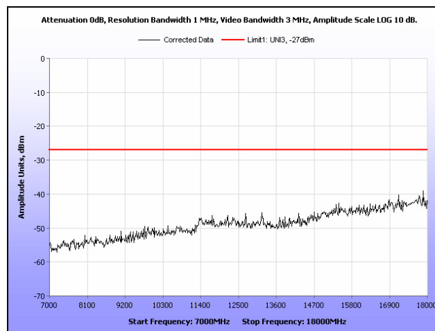
Plot 334. Radiated Spurious Emissions, 802.11a, 5300 MHz, 7 GHz – 18 GHz, Ceiling Mount
