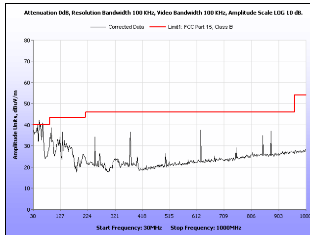
Plot 287. Radiated Spurious Emissions, 802.11a, 5320 MHz, 30 MHz – 1 GHz, 6 dBi Dipole Antenna
