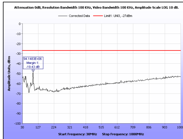
Plot 194. Radiated Spurious Emissions, 802.11a, 5500 MHz, 30 MHz – 1 GHz, 2 dBi Dipole Antenna
