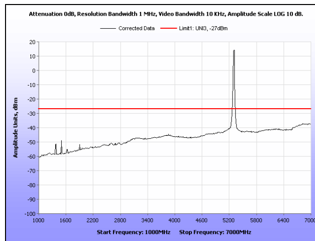
Plot 207. Radiated Spurious Emissions, 802.11n 20 MHz, 5300 MHz, 1 GHz – 7 GHz, 2 dBi Dipole Antenna
