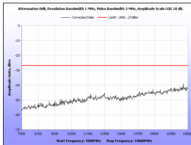
Plot 376. Radiated Spurious Emissions, 802.11n 40 MHz, 5670 MHz, 7 GHz – 18 GHz, Ceiling Mount
