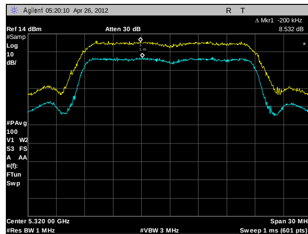
Plot 162. Peak Excursion Ratio, 802.11n 20 MHz, A5, 5320 MHz
