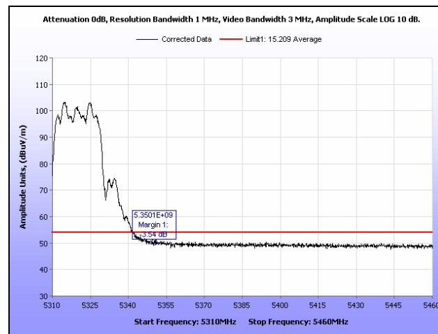
Plot 441. Restricted Band, 802.11n 20 MHz, 5320 MHz, Average, Patch
