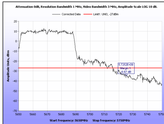
Plot 400. Radiated Band Edge, 802.11n 40 MHz, 5670 MHz, Patch
