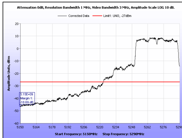
Plot 421. Radiated Band Edge, 802.11n 40 MHz, 5270 MHz, Ceiling Mount
