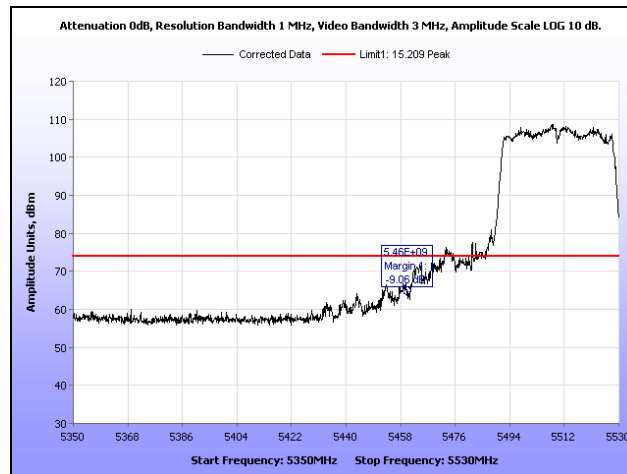
Plot 436. Restricted Band, 802.11n 40 MHz, 5510 MHz, Peak
