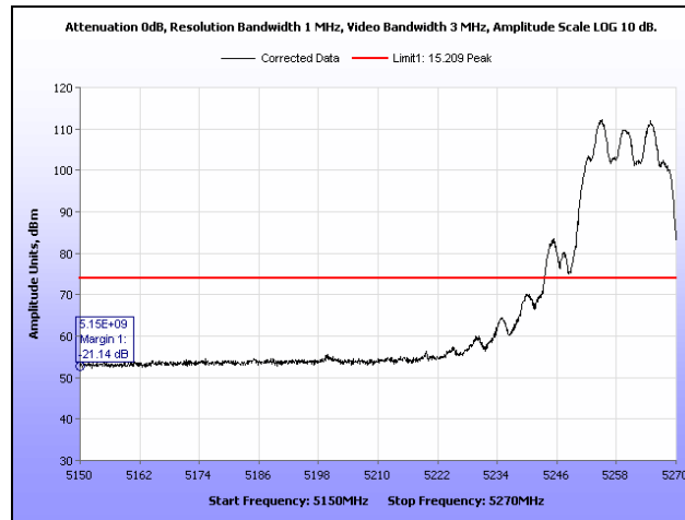
Plot 393. Radiated Band Edge, 802.11n 20 MHz, 5260 MHz, Patch
