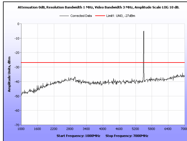
Plot 339. Radiated Spurious Emissions, 802.11a, 5500 MHz, 1 GHz – 7 GHz, Ceiling Mount
