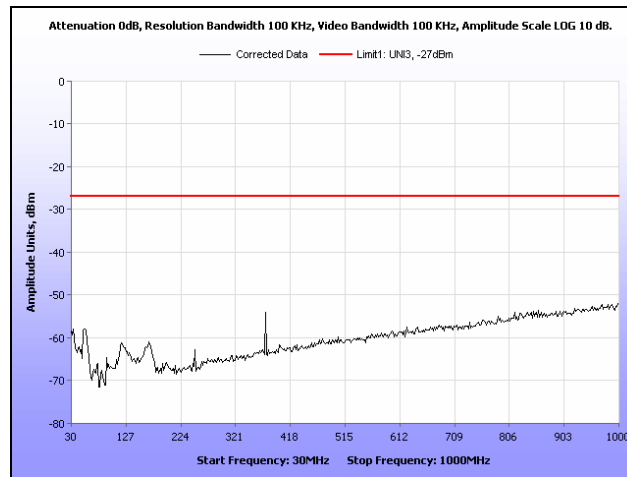
Plot 359. Radiated Spurious Emissions, 802.11n 20 MHz, 5580 MHz, 30 MHz – 1 GHz, Ceiling Mount
