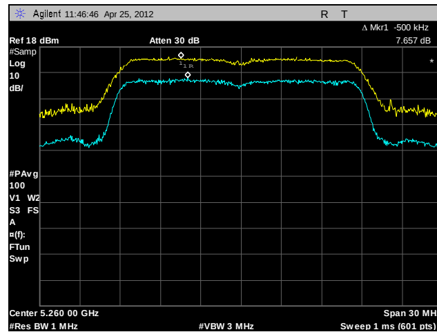
Plot 155. Peak Excursion Ratio, 802.11n 20 MHz, A4, 5260 MHz
