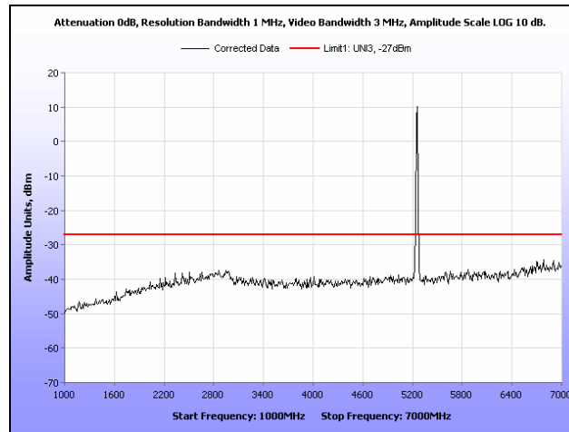
Plot 348. Radiated Spurious Emissions, 802.11n 20 MHz, 5260 MHz, 1 GHz – 7 GHz, Ceiling Mount
