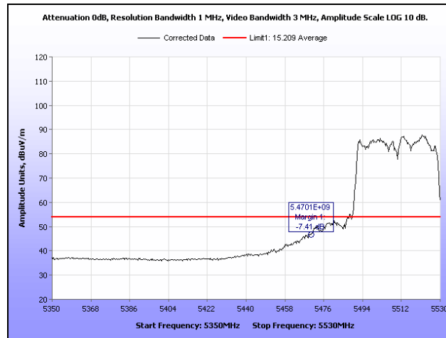
Plot 447. Restricted Band, 802.11n 40 MHz, 5510 MHz, Average, Patch
