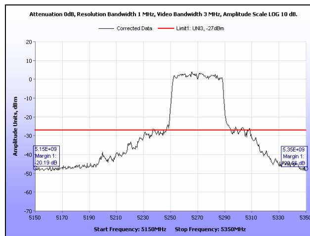
Plot 409. Radiated Band Edge, 802.11n 40 MHz, 5270 MHz, 6 dBi Dipole Antenna
