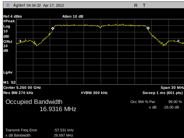
Plot 5. 26 dB Occupied Bandwidth, 802.11a, A4, 5260 MHz
