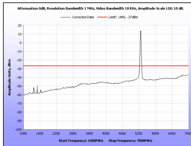
Plot 204. Radiated Spurious Emissions, 802.11n 20 MHz, 5260 MHz, 1 GHz – 7 GHz, 2 dBi Dipole Antenna
