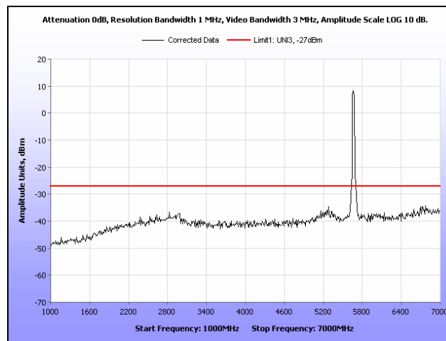
Plot 375. Radiated Spurious Emissions, 802.11n 40 MHz, 5670 MHz, 1 GHz – 7 GHz, Ceiling Mount
