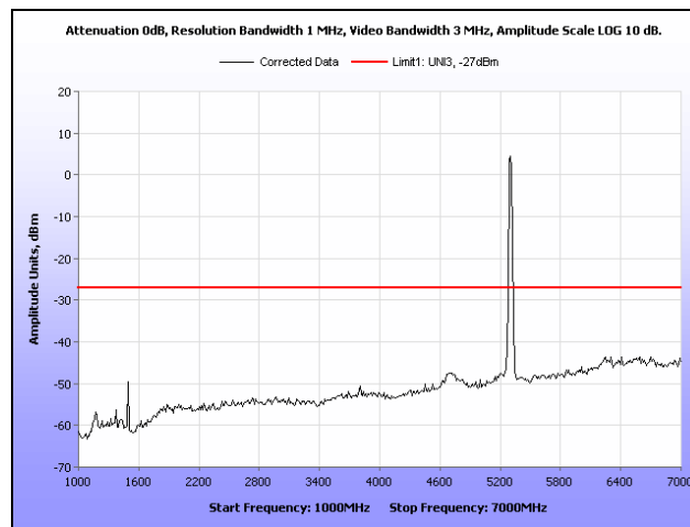
Plot 237. Radiated Spurious Emissions, 802.11a, 5300 MHz, 1 GHz – 7 GHz, Patch
