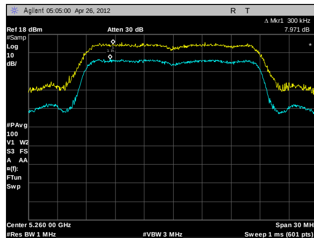
Plot 156. Peak Excursion Ratio, 802.11n 20 MHz, A5, 5260 MHz
