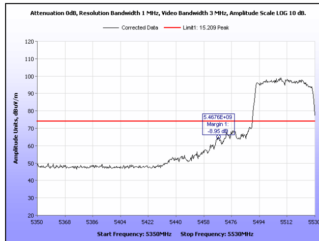
Plot 448. Restricted Band, 802.11n 40 MHz, 5510 MHz, Peak, Patch
