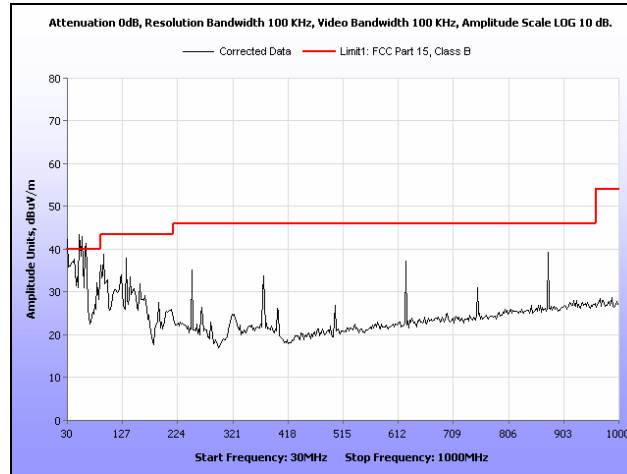
Plot 296. Radiated Spurious Emissions, 802.11a, 5700 MHz, 30 MHz – 1 GHz, 6 dBi Dipole Antenna
