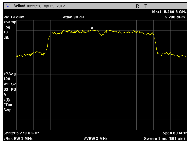
Plot 139. Power Spectral Density, 802.11n 40 MHz, A6, 5270 MHz
