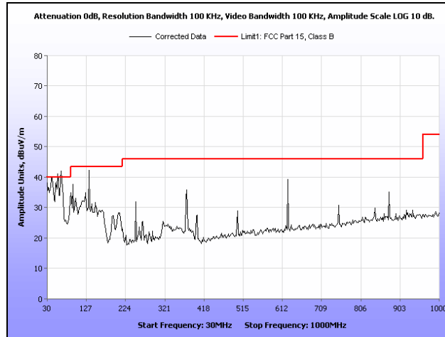
Plot 320. Radiated Spurious Emissions, 802.11n 40 MHz, 5310 MHz, 30 MHz – 1 GHz, 6 dBi Dipole Antenna
