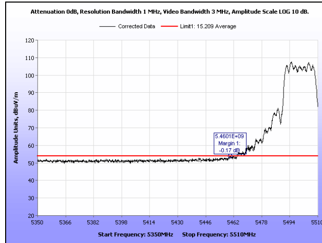
Plot 443. Restricted Band, 802.11n 20 MHz, 5500 MHz, Average, Patch
