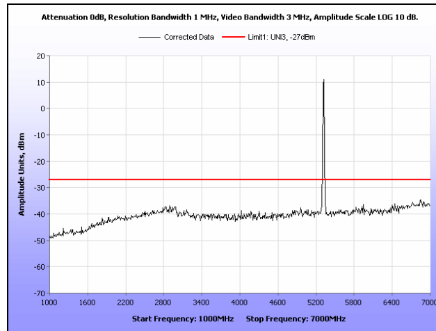
Plot 306. Radiated Spurious Emissions, 802.11n 20 MHz, 5320 MHz, 1 GHz – 7 GHz, 6 dBi Dipole Antenna
