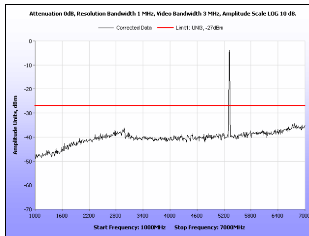
Plot 336. Radiated Spurious Emissions, 802.11a, 5320 MHz, 1 GHz – 7 GHz, Ceiling Mount
