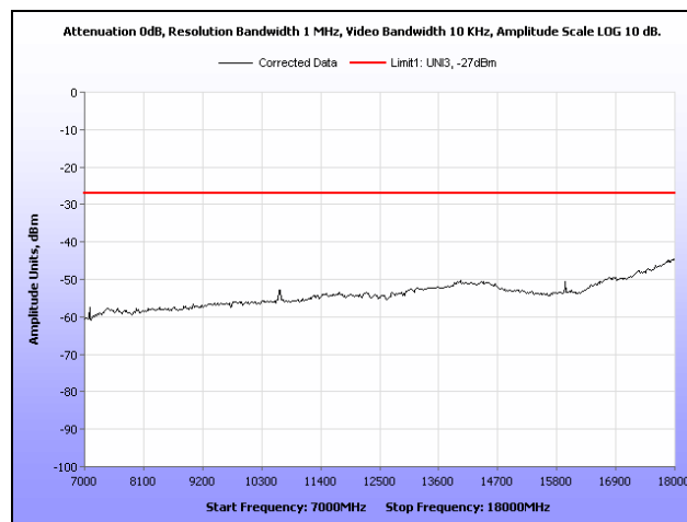
Plot 211. Radiated Spurious Emissions, 802.11n 20 MHz, 5320 MHz, 7 GHz – 18 GHz, 2 dBi Dipole Antenna
