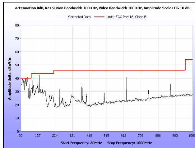
Plot 317. Radiated Spurious Emissions, 802.11n 40 MHz, 5270 MHz, 30 MHz – 1 GHz, 6 dBi Dipole Antenna
