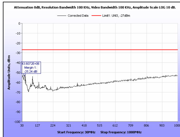
Plot 251. Radiated Spurious Emissions, 802.11n 20 MHz, 5260 MHz, 30 MHz – 1 GHz, Patch
