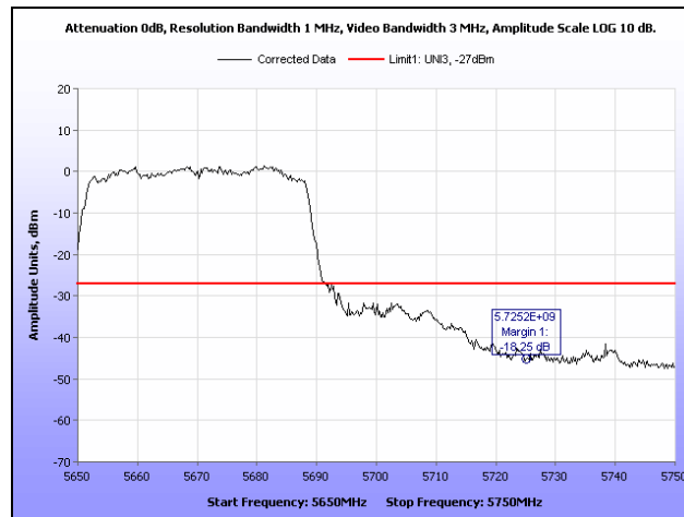
Plot 412. Radiated Band Edge, 802.11n 40 MHz, 5670 MHz, 6 dBi Dipole Antenna
