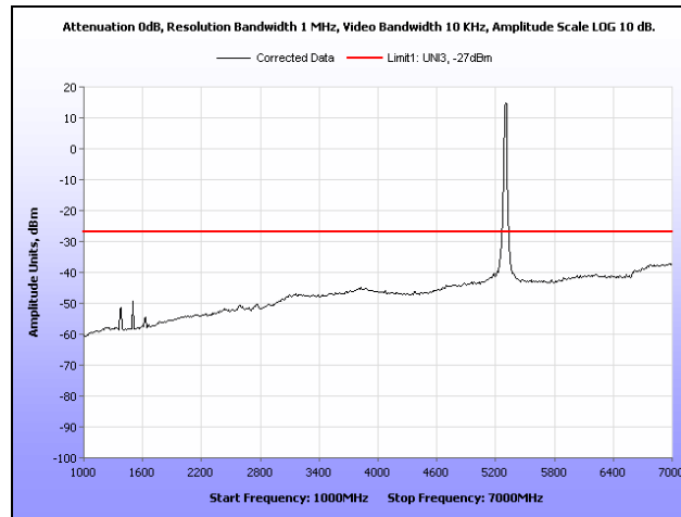
Plot 189. Radiated Spurious Emissions, 802.11a, 5300 MHz, 1 GHz – 7 GHz, 2 dBi Dipole Antenna
