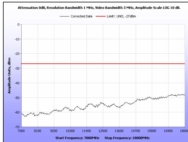
Plot 295. Radiated Spurious Emissions, 802.11a, 5580 MHz, 7 GHz – 18 GHz, 6 dBi Dipole Antenna
