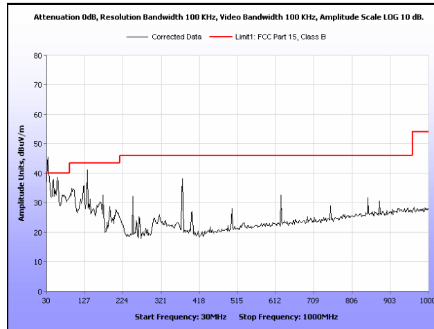
Plot 329. Radiated Spurious Emissions, 802.11a, 5260 MHz, 30 MHz – 1 GHz, Ceiling Mount
