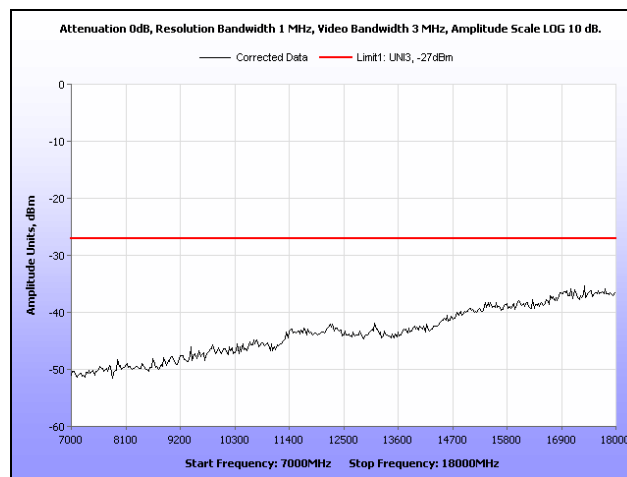
Plot 238. Radiated Spurious Emissions, 802.11a, 5300 MHz, 7 GHz – 18 GHz, Patch
