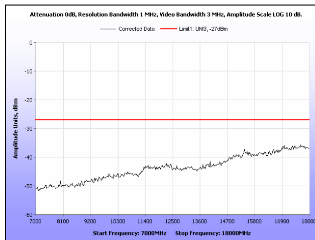
Plot 274. Radiated Spurious Emissions, 802.11n 40 MHz, 5310 MHz, 7 GHz – 18 GHz, Patch
