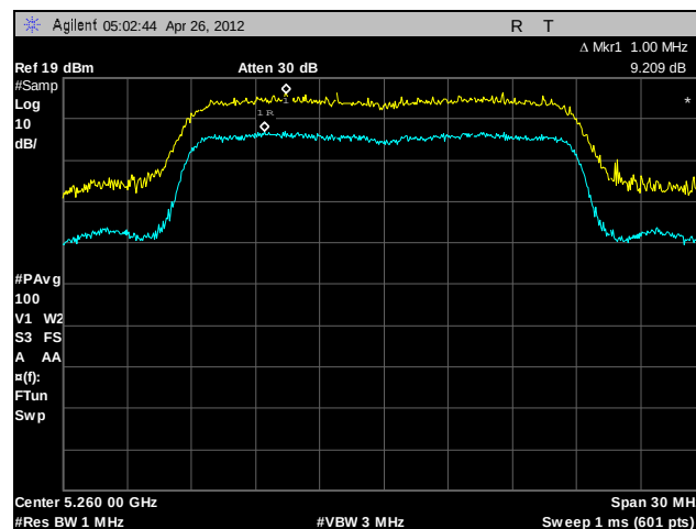
Plot 157. Peak Excursion Ratio, 802.11n 20 MHz, A6, 5260 MHz
