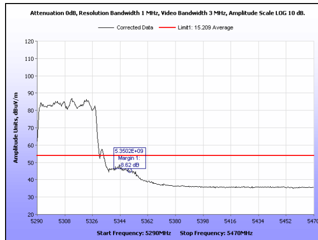
Plot 457. Restricted Band, 802.11n 40 MHz, 5310 MHz, Average, 6 dBi Dipole Antenna
