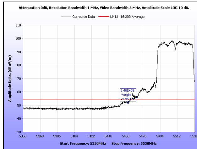
Plot 471. Restricted Band, 802.11n 40 MHz, 5510 MHz, Average, Ceiling Mount
