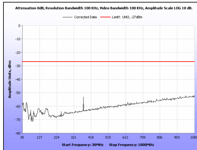
Plot 356. Radiated Spurious Emissions, 802.11n 20 MHz, 5500 MHz, 30 MHz – 1 GHz, Ceiling Mount
