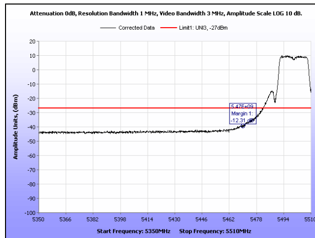
Plot 391. Radiated Band Edge, 802.11a, 5500 MHz, Patch
