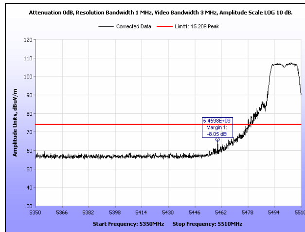
Plot 464. Restricted Band, 802.11a, 5500 MHz, Peak, Ceiling Mount
