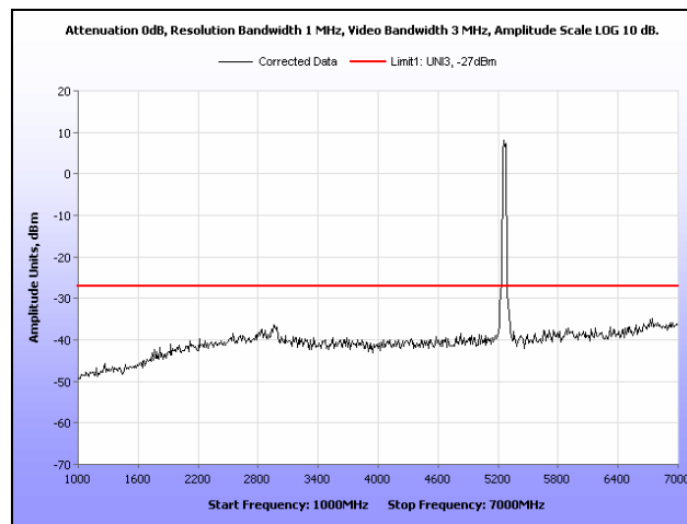
Plot 366. Radiated Spurious Emissions, 802.11n 40 MHz, 5270 MHz, 1 GHz – 7 GHz, Ceiling Mount
