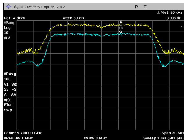
Plot 172. Peak Excursion Ratio, 802.11n 20 MHz, A6, 5700 MHz
