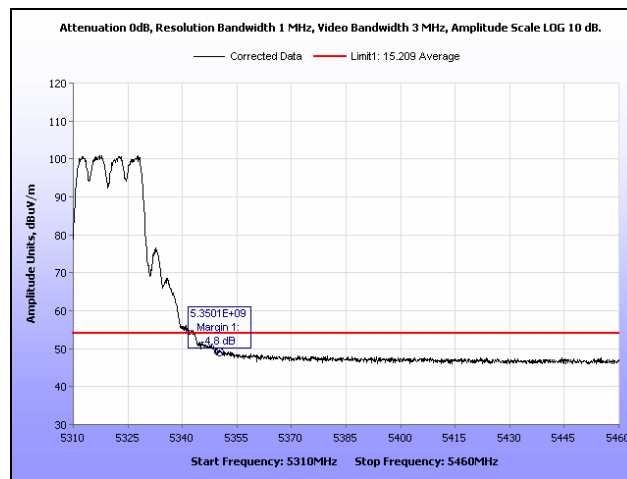
Plot 465. Restricted Band, 802.11n 20 MHz, 5320 MHz, Average, Ceiling Mount
