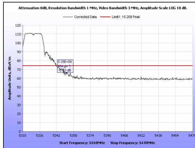
Plot 426. Restricted Band, 802.11a, 5320 MHz, Peak
