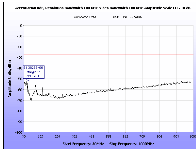
Plot 263. Radiated Spurious Emissions, 802.11n 20 MHz, 5580 MHz, 30 MHz – 1 GHz, Patch
