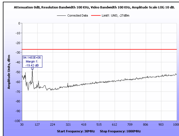
Plot 203. Radiated Spurious Emissions, 802.11n 20 MHz, 5260 MHz, 30 MHz – 1 GHz, 2 dBi Dipole Antenna
