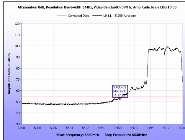
Plot 435. Restricted Band, 802.11n 40 MHz, 5510 MHz, Average
