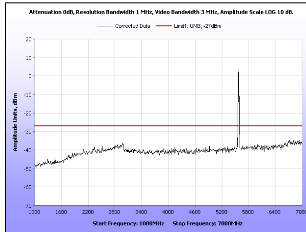
Plot 294. Radiated Spurious Emissions, 802.11a, 5580 MHz, 1 GHz – 7 GHz, 6 dBi Dipole Antenna
