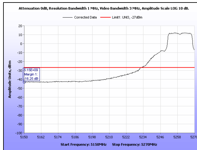
Plot 377. Radiated Band Edge, 802.11a, 5260 MHz
