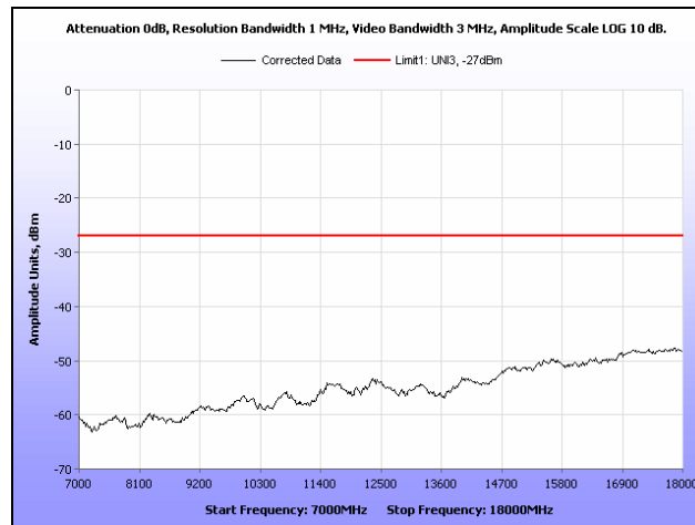
Plot 307. Radiated Spurious Emissions, 802.11n 20 MHz, 5320 MHz, 7 GHz – 18 GHz, 6 dBi Dipole Antenna
