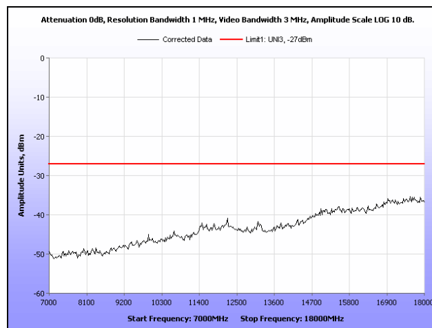
Plot 259. Radiated Spurious Emissions, 802.11n 20 MHz, 5320 MHz, 7 GHz – 18 GHz, Patch
