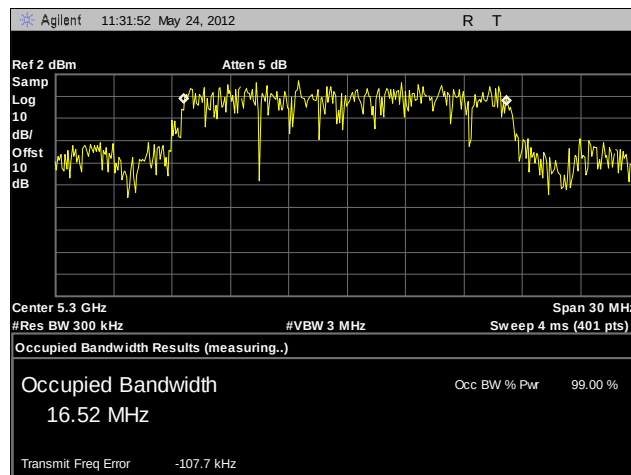
Plot 42. 99% Occupied Bandwidth, 802.11a, A4, 5300 MHz
