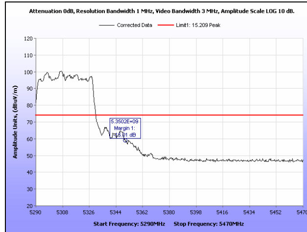
Plot 446. Restricted Band, 802.11n 40 MHz, 5310 MHz, Peak, Patch
