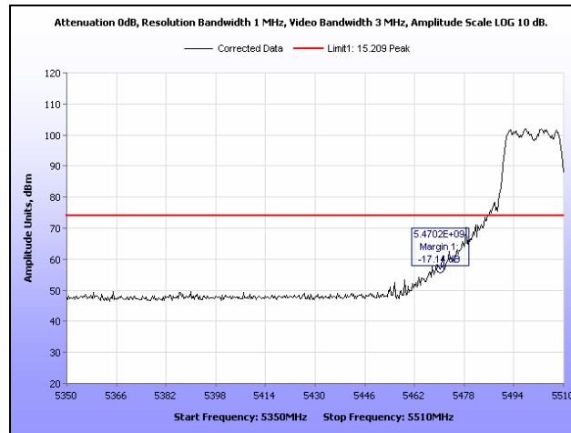
Plot 456. Restricted Band, 802.11n 20 MHz, 5500 MHz, Peak, 6 dBi Dipole Antenna
