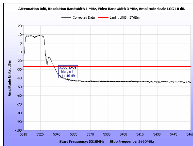
Plot 390. Radiated Band Edge, 802.11a, 5320 MHz, Patch
