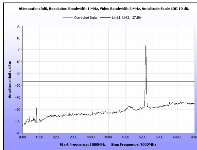
Plot 255. Radiated Spurious Emissions, 802.11n 20 MHz, 5300 MHz, 1 GHz – 7 GHz, Patch
