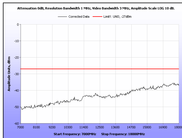
Plot 280. Radiated Spurious Emissions, 802.11n 40 MHz, 5670 MHz, 7 GHz – 18 GHz, Patch
