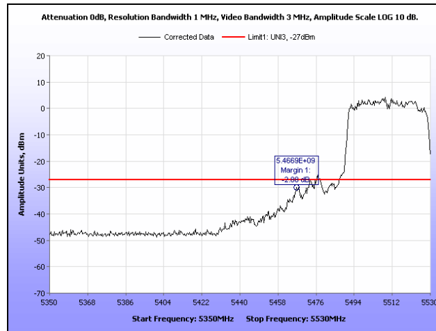
Plot 411. Radiated Band Edge, 802.11n 40 MHz, 5510 MHz, 6 dBi Dipole Antenna
