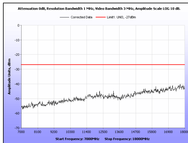
Plot 361. Radiated Spurious Emissions, 802.11n 20 MHz, 5580 MHz, 7 GHz – 18 GHz, Ceiling Mount
