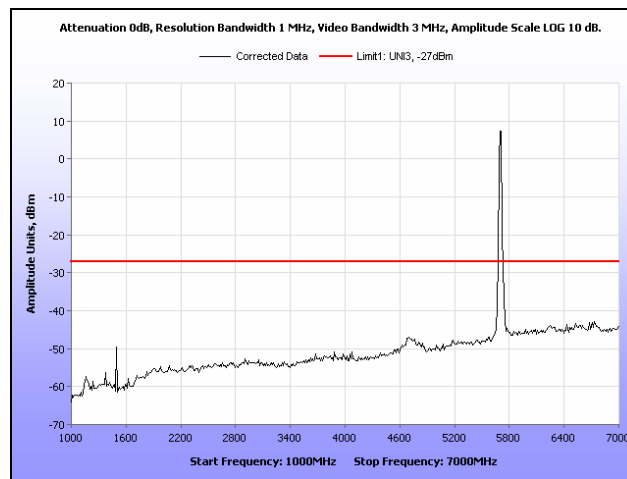
Plot 267. Radiated Spurious Emissions, 802.11n 20 MHz, 5700 MHz, 1 GHz – 7 GHz, Patch
