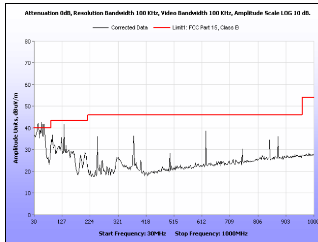
Plot 311. Radiated Spurious Emissions, 802.11n 20 MHz, 5580 MHz, 30 MHz – 1 GHz, 6 dBi Dipole Antenna
