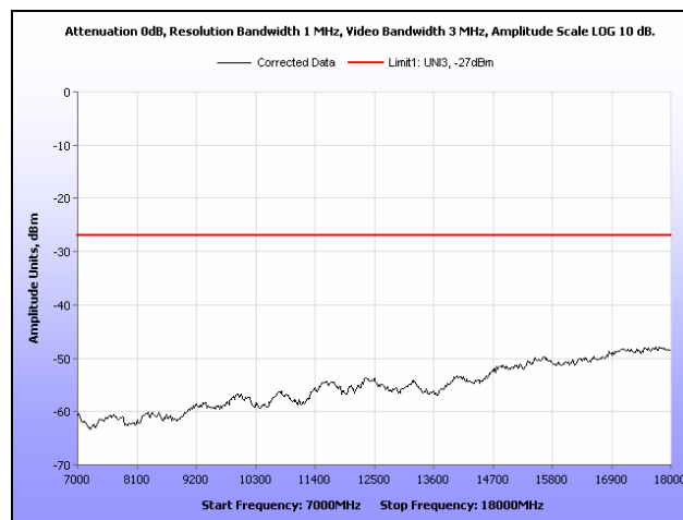
Plot 319. Radiated Spurious Emissions, 802.11n 40 MHz, 5270 MHz, 7 GHz – 18 GHz, 6 dBi Dipole Antenna
