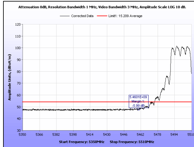
Plot 467. Restricted Band, 802.11n 20 MHz, 5500 MHz, Average, Ceiling Mount
