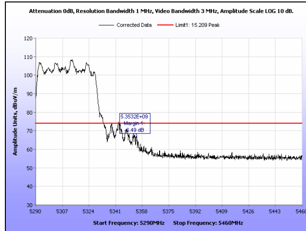
Plot 434. Restricted Band, 802.11n 40 MHz, 5310 MHz, Peak
