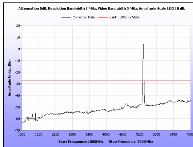
Plot 258. Radiated Spurious Emissions, 802.11n 20 MHz, 5320 MHz, 1 GHz – 7 GHz, Patch
