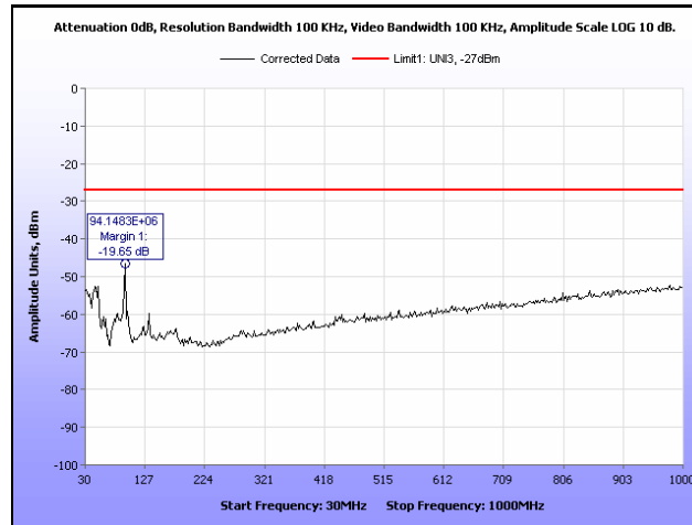
Plot 185. Radiated Spurious Emissions, 802.11a, 5260 MHz, 30 MHz – 1 GHz, 2 dBi Dipole Antenna
