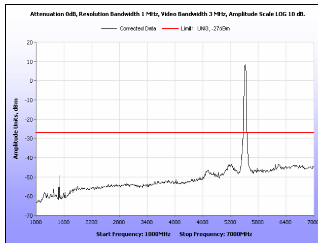
Plot 276. Radiated Spurious Emissions, 802.11n 40 MHz, 5510 MHz, 1 GHz – 7 GHz, Patch
