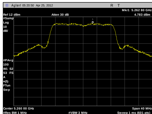
Plot 120. Power Spectral Density, 802.11n 20 MHz, A5, 5260 MHz
