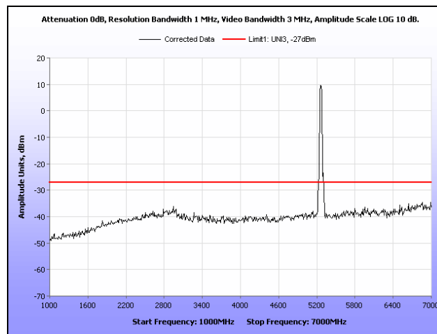
Plot 318. Radiated Spurious Emissions, 802.11n 40 MHz, 5270 MHz, 1 GHz – 7 GHz, 6 dBi Dipole Antenna
