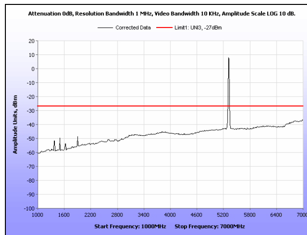
Plot 210. Radiated Spurious Emissions, 802.11n 20 MHz, 5320 MHz, 1 GHz – 7 GHz, 2 dBi Dipole Antenna
