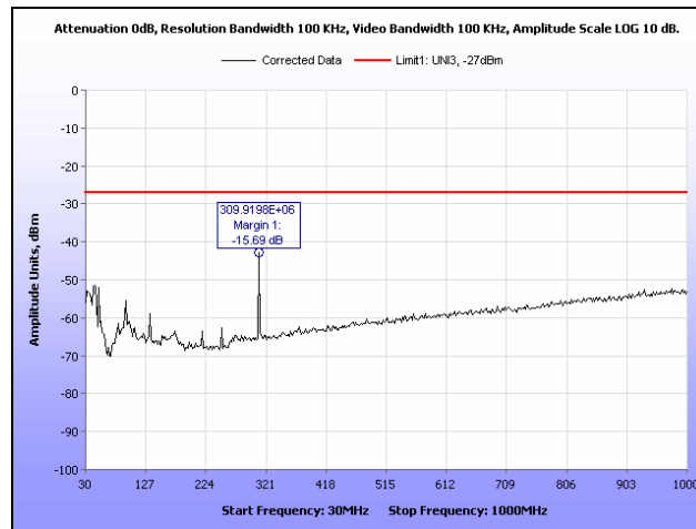
Plot 266. Radiated Spurious Emissions, 802.11n 20 MHz, 5700 MHz, 30 MHz – 1 GHz, Patch
