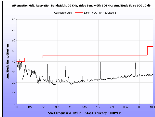
Plot 293. Radiated Spurious Emissions, 802.11a, 5580 MHz, 30 MHz – 1 GHz, 6 dBi Dipole Antenna
