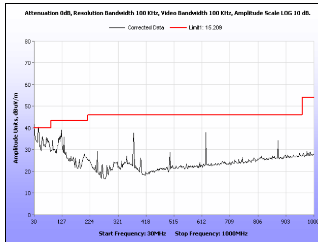
Plot 278. Radiated Spurious Emissions, 802.11n 40 MHz, 5670 MHz, 30 MHz – 1 GHz, Patch
