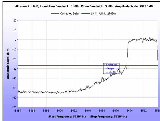
Plot 399. Radiated Band Edge, 802.11n 40 MHz, 5510 MHz, Patch
