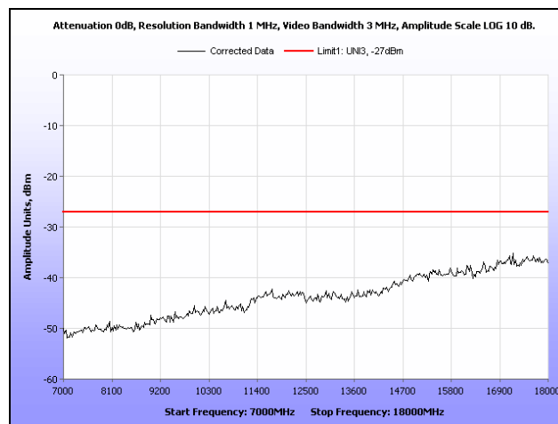
Plot 268. Radiated Spurious Emissions, 802.11n 20 MHz, 5700 MHz, 7 GHz – 18 GHz, Patch
