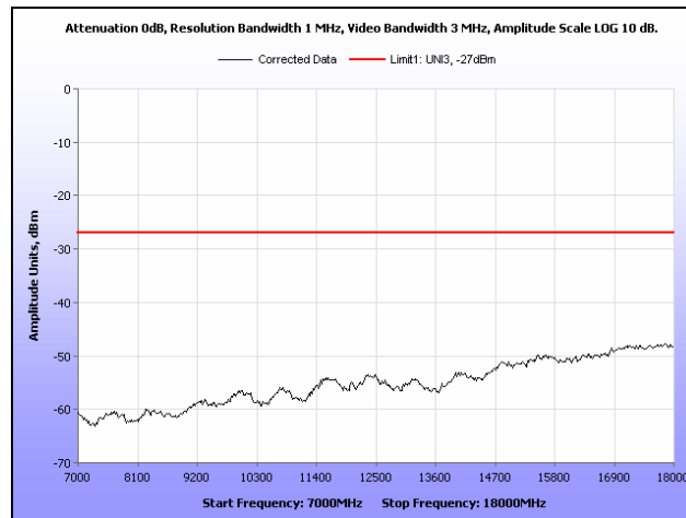
Plot 298. Radiated Spurious Emissions, 802.11a, 5700 MHz, 7 GHz – 18 GHz, 6 dBi Dipole Antenna
