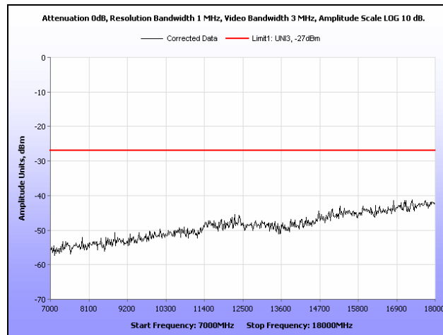
Plot 346. Radiated Spurious Emissions, 802.11a, 5700 MHz, 7 GHz – 18 GHz, Ceiling Mount
