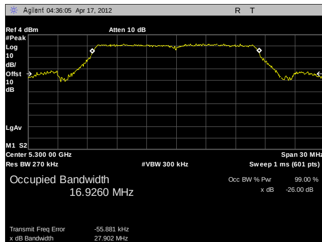
Plot 6. 26 dB Occupied Bandwidth, 802.11a, A4, 5300 MHz
