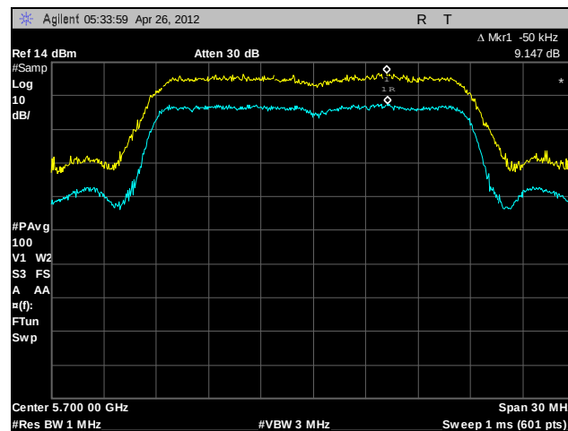
Plot 171. Peak Excursion Ratio, 802.11n 20 MHz, A5, 5700 MHz
