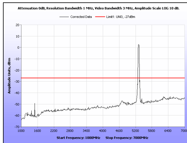
Plot 273. Radiated Spurious Emissions, 802.11n 40 MHz, 5310 MHz, 1 GHz – 7 GHz, Patch
