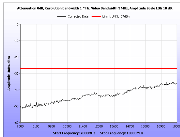
Plot 277. Radiated Spurious Emissions, 802.11n 40 MHz, 5510 MHz, 7 GHz – 18 GHz, Patch
