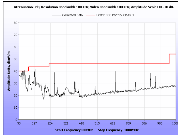
Plot 281. Radiated Spurious Emissions, 802.11a, 5260 MHz, 30 MHz – 1 GHz, 6 dBi Dipole Antenna
