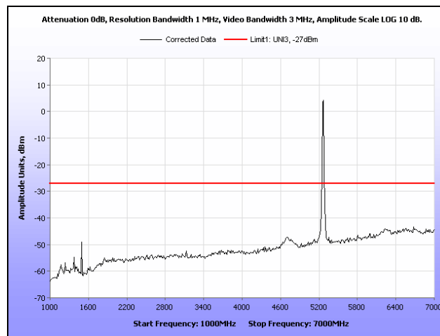
Plot 252. Radiated Spurious Emissions, 802.11n 20 MHz, 5260 MHz, 1 GHz – 7 GHz, Patch
