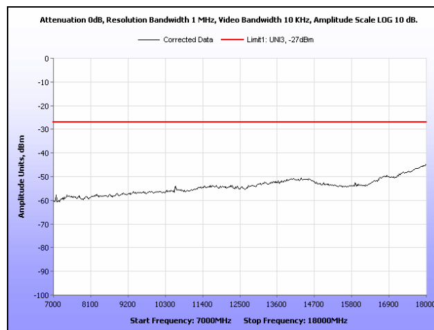
Plot 208. Radiated Spurious Emissions, 802.11n 20 MHz, 5300 MHz, 7 GHz – 18 GHz, 2 dBi Dipole Antenna
