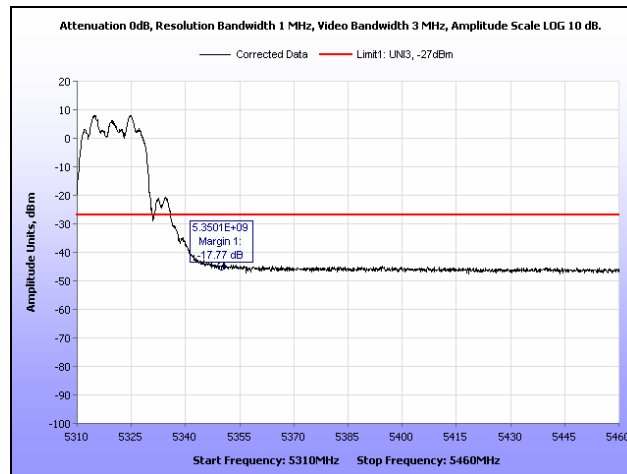
Plot 394. Radiated Band Edge, 802.11n 20 MHz, 5320 MHz, Patch
