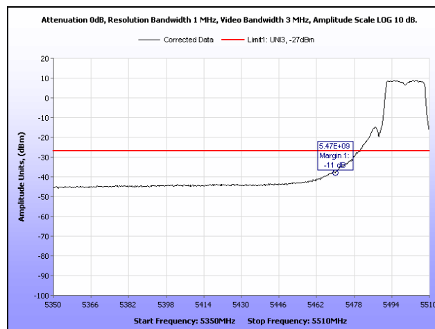
Plot 379. Radiated Band Edge, 802.11a, 5500 MHz
