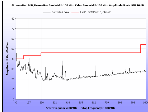
Plot 338. Radiated Spurious Emissions, 802.11a, 5500 MHz, 30 MHz – 1 GHz, Ceiling Mount
