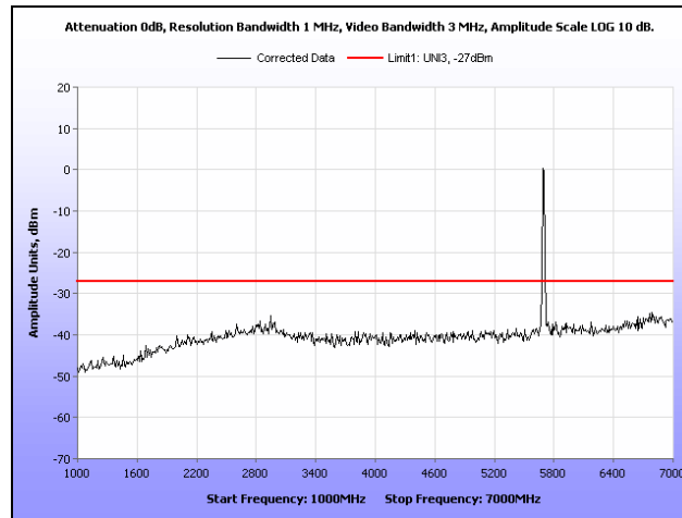
Plot 297. Radiated Spurious Emissions, 802.11a, 5700 MHz, 1 GHz – 7 GHz, 6 dBi Dipole Antenna
