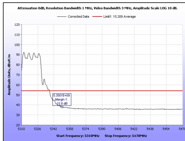
Plot 453. Restricted Band, 802.11n 20 MHz, 5320 MHz, Average, 6 dBi Dipole Antenna
