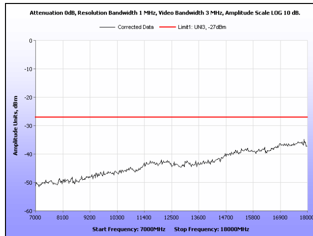
Plot 244. Radiated Spurious Emissions, 802.11a, 5500 MHz, 7 GHz – 18 GHz, Patch
