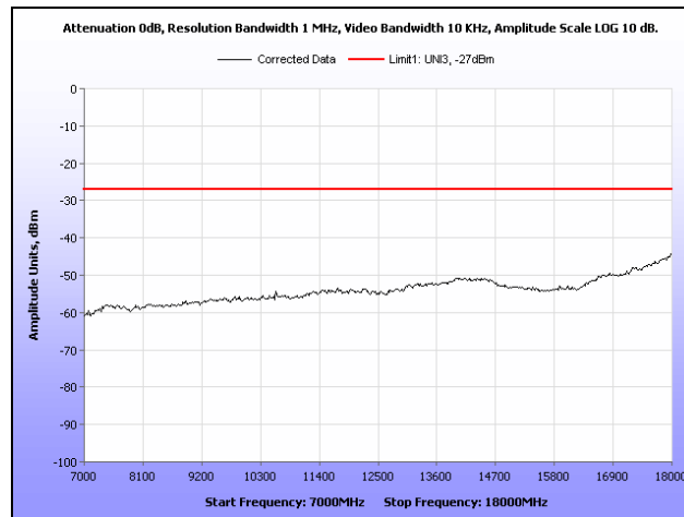
Plot 190. Radiated Spurious Emissions, 802.11a, 5300 MHz, 7 GHz – 18 GHz, 2 dBi Dipole Antenna
