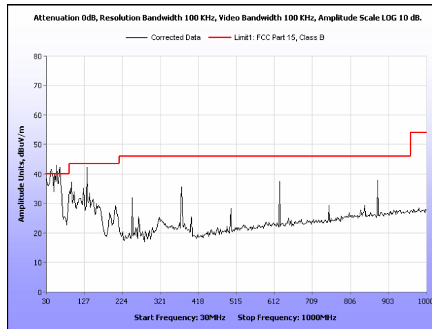
Plot 308. Radiated Spurious Emissions, 802.11n 20 MHz, 5500 MHz, 30 MHz – 1 GHz, 6 dBi Dipole Antenna
