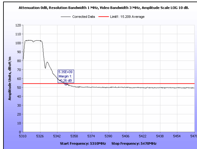
Plot 425. Restricted Band, 802.11a, 5320 MHz, Average
