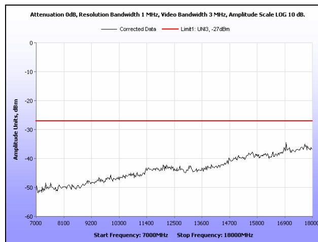
Plot 253. Radiated Spurious Emissions, 802.11n 20 MHz, 5260 MHz, 7 GHz – 18 GHz, Patch
