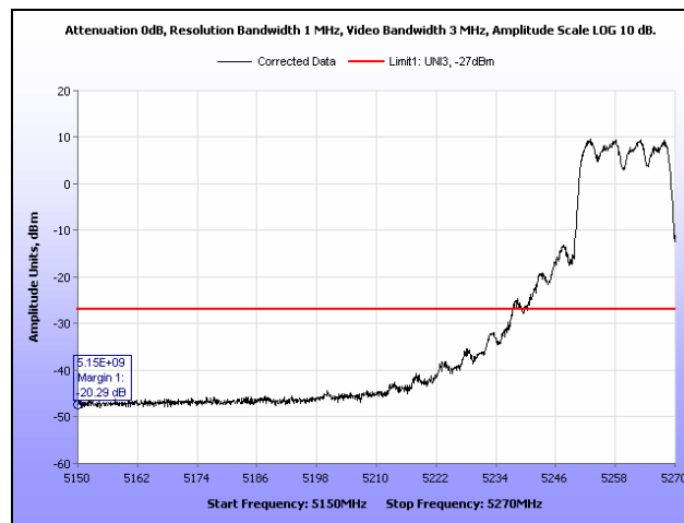
Plot 417. Radiated Band Edge, 802.11n 20 MHz, 5260 MHz, Ceiling Mount
