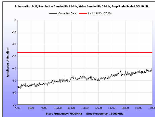
Plot 349. Radiated Spurious Emissions, 802.11n 20 MHz, 5260 MHz, 7 GHz – 18 GHz, Ceiling Mount
