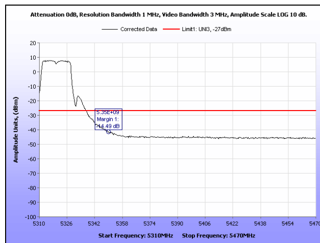
Plot 378. Radiated Band Edge, 802.11a, 5320 MHz
