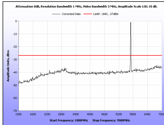
Plot 345. Radiated Spurious Emissions, 802.11a, 5700 MHz, 1 GHz – 7 GHz, Ceiling Mount
