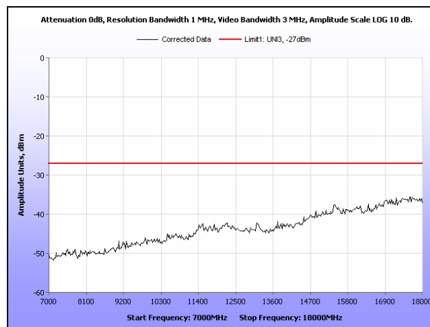
Plot 256. Radiated Spurious Emissions, 802.11n 20 MHz, 5300 MHz, 7 GHz – 18 GHz, Patch
