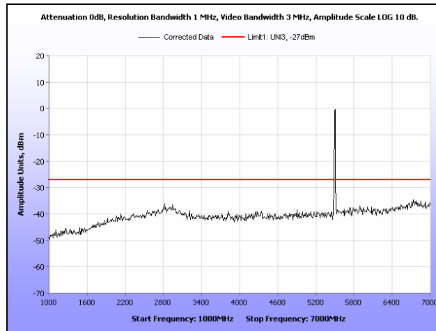
Plot 291. Radiated Spurious Emissions, 802.11a, 5500 MHz, 1 GHz – 7 GHz, 6 dBi Dipole Antenna
