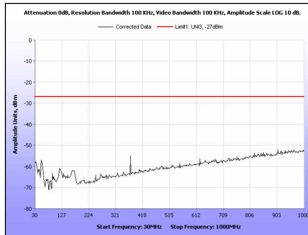
Plot 365. Radiated Spurious Emissions, 802.11n 40 MHz, 5270 MHz, 30 MHz – 1 GHz, Ceiling Mount
