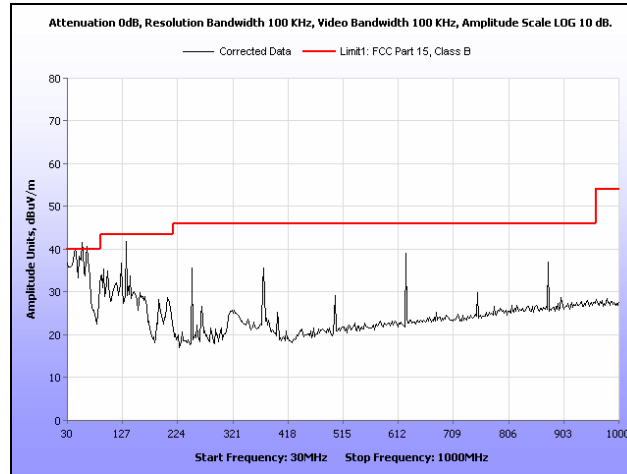
Plot 305. Radiated Spurious Emissions, 802.11n 20 MHz, 5320 MHz, 30 MHz – 1 GHz, 6 dBi Dipole Antenna
