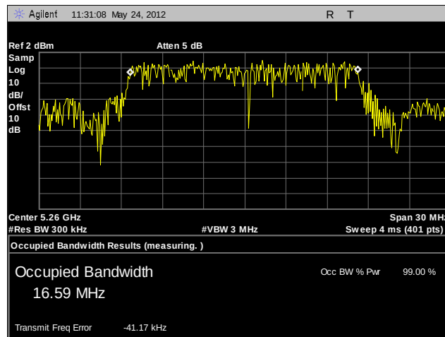
Plot 41. 99% Occupied Bandwidth, 802.11a, A4, 5260 MHz
