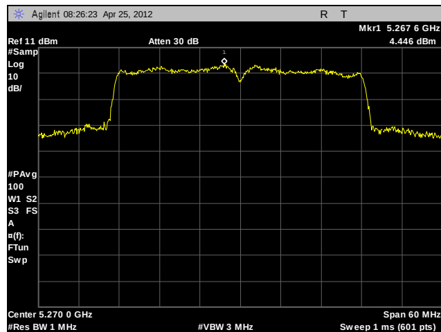
Plot 138. Power Spectral Density, 802.11n 40 MHz, A5, 5270 MHz
