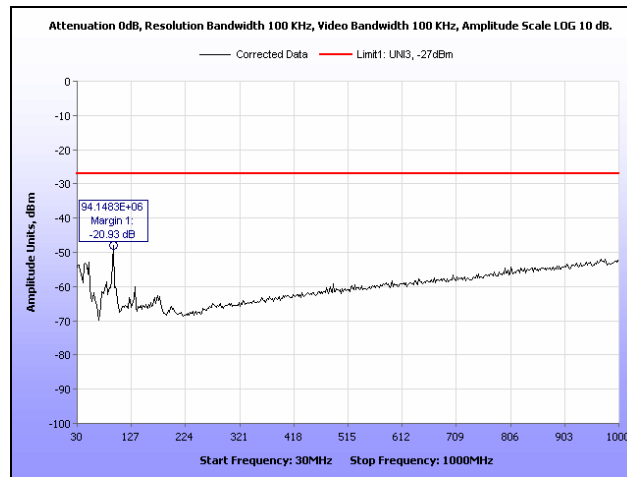
Plot 209. Radiated Spurious Emissions, 802.11n 20 MHz, 5320 MHz, 30 MHz – 1 GHz, 2 dBi Dipole Antenna
