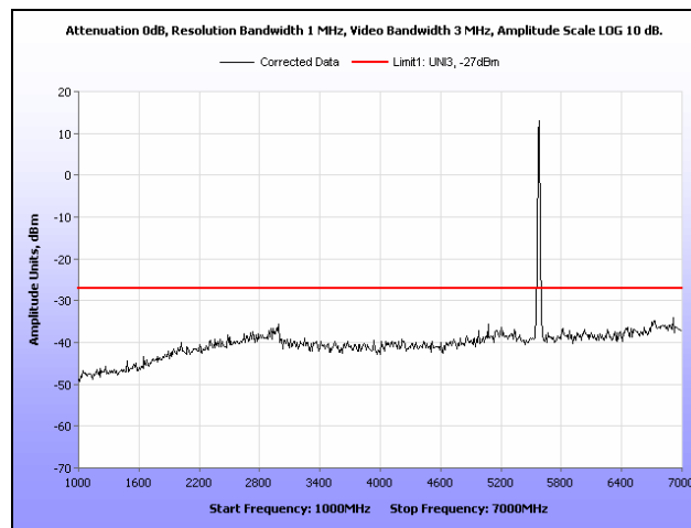
Plot 360. Radiated Spurious Emissions, 802.11n 20 MHz, 5580 MHz, 1 GHz – 7 GHz, Ceiling Mount
