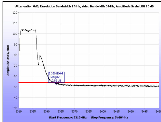
Plot 437. Restricted Band, 802.11a, 5320 MHz, Average, Patch
