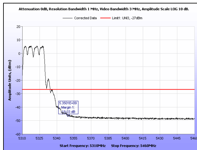
Plot 418. Radiated Band Edge, 802.11n 20 MHz, 5320 MHz, Ceiling Mount
