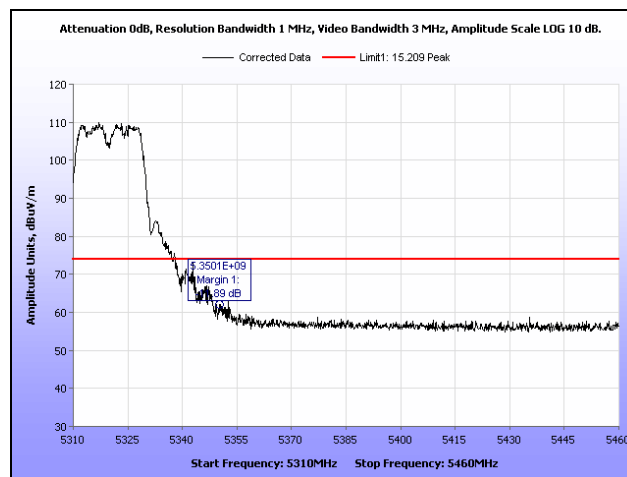
Plot 466. Restricted Band, 802.11n 20 MHz, 5320 MHz, Peak, Ceiling Mount
