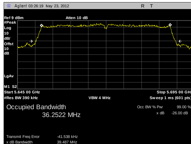
Plot 39. 26 dB Occupied Bandwidth, 802.11n 40 MHz, A5, 5670 MHz
