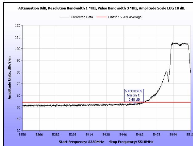
Plot 439. Restricted Band, 802.11a, 5500 MHz, Average, Patch
