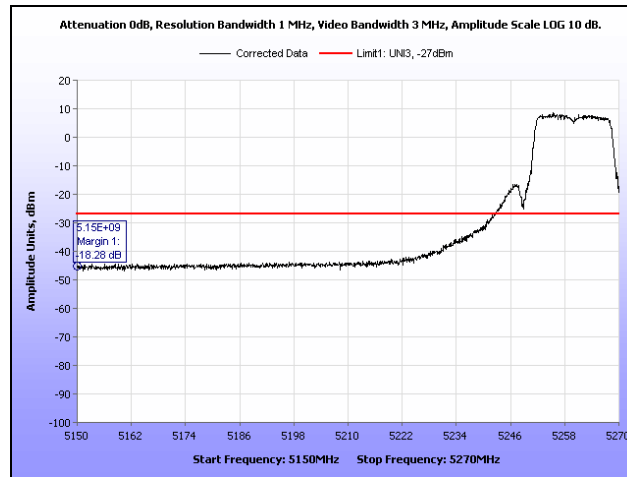
Plot 389. Radiated Band Edge, 802.11a, 5260 MHz, Patch
