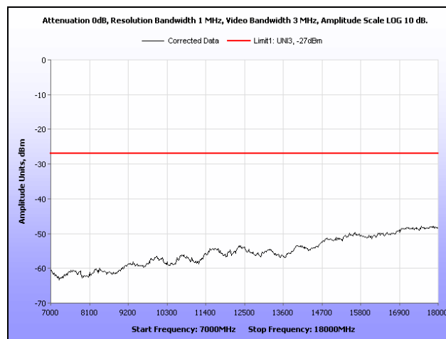
Plot 310. Radiated Spurious Emissions, 802.11n 20 MHz, 5500 MHz, 7 GHz – 18 GHz, 6 dBi Dipole Antenna
