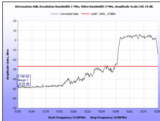
Plot 397. Radiated Band Edge, 802.11n 40 MHz, 5270 MHz, Patch
