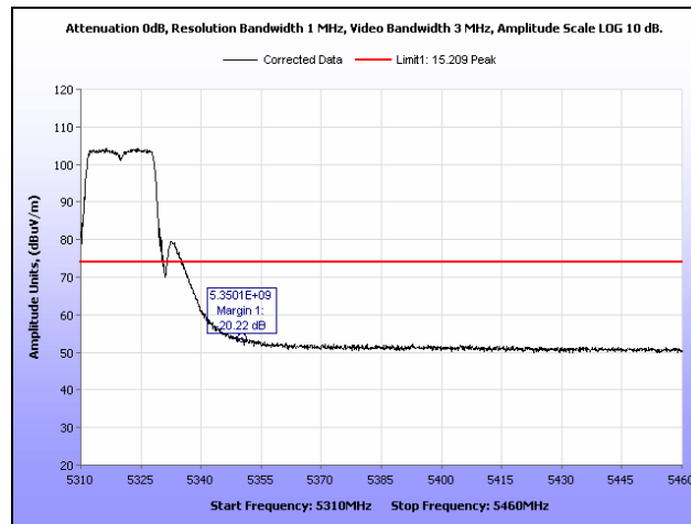
Plot 438. Restricted Band, 802.11a, 5320 MHz, Peak, Patch
