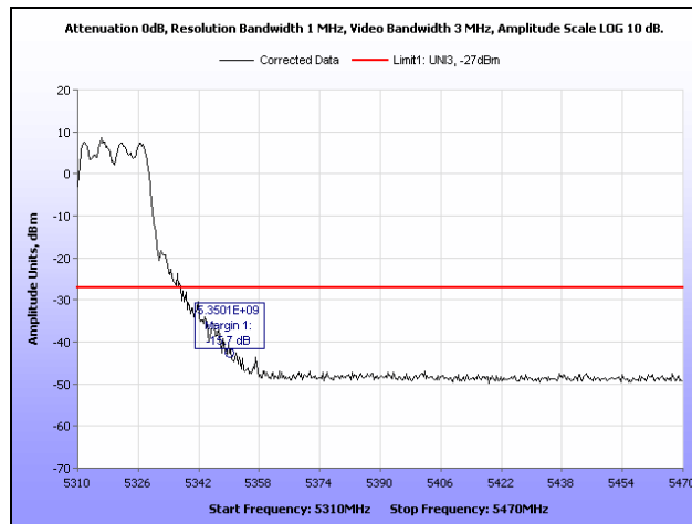
Plot 406. Radiated Band Edge, 802.11n 20 MHz, 5320 MHz, 6 dBi Dipole Antenna
