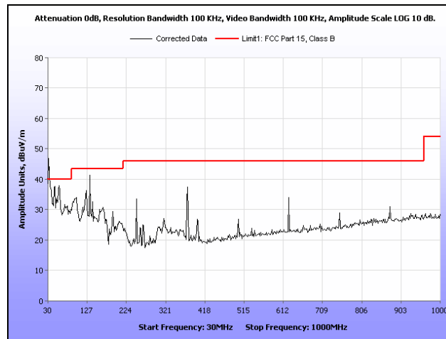
Plot 335. Radiated Spurious Emissions, 802.11a, 5320 MHz, 30 MHz – 1 GHz, Ceiling Mount
