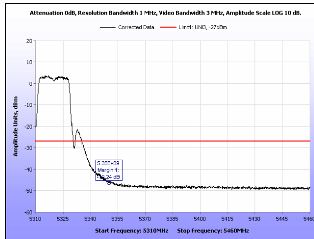
Plot 414. Radiated Band Edge, 802.11a, 5320 MHz, Ceiling Mount
