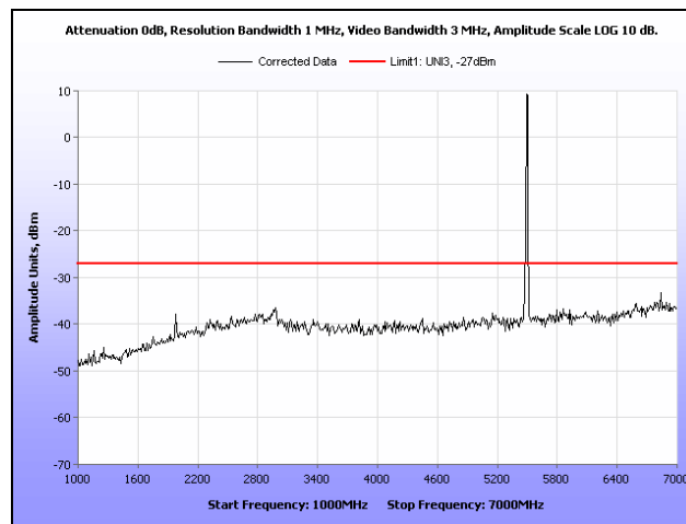
Plot 357. Radiated Spurious Emissions, 802.11n 20 MHz, 5500 MHz, 1 GHz – 7 GHz, Ceiling Mount
