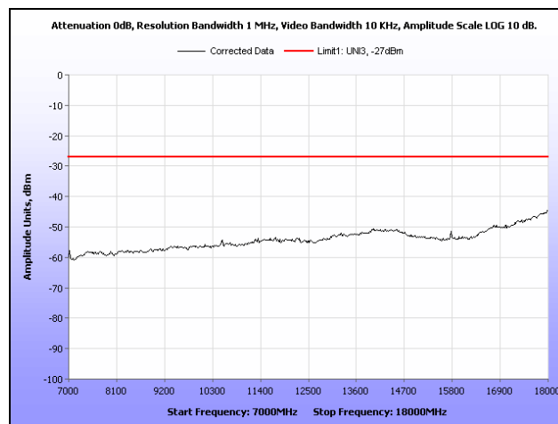
Plot 205. Radiated Spurious Emissions, 802.11n 20 MHz, 5260 MHz, 7 GHz – 18 GHz, 2 dBi Dipole Antenna
