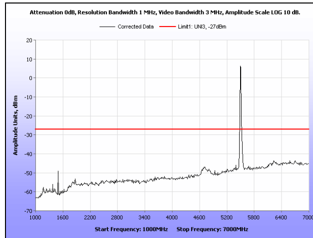
Plot 243. Radiated Spurious Emissions, 802.11a, 5500 MHz, 1 GHz – 7 GHz, Patch
