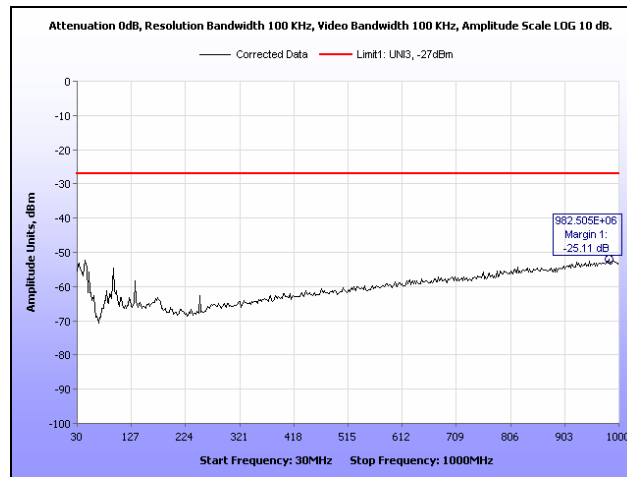
Plot 236. Radiated Spurious Emissions, 802.11a, 5300 MHz, 30 MHz – 1 GHz, Patch
