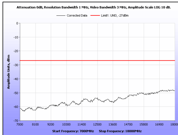
Plot 322. Radiated Spurious Emissions, 802.11n 40 MHz, 5310 MHz, 7 GHz – 18 GHz, 6 dBi Dipole Antenna
