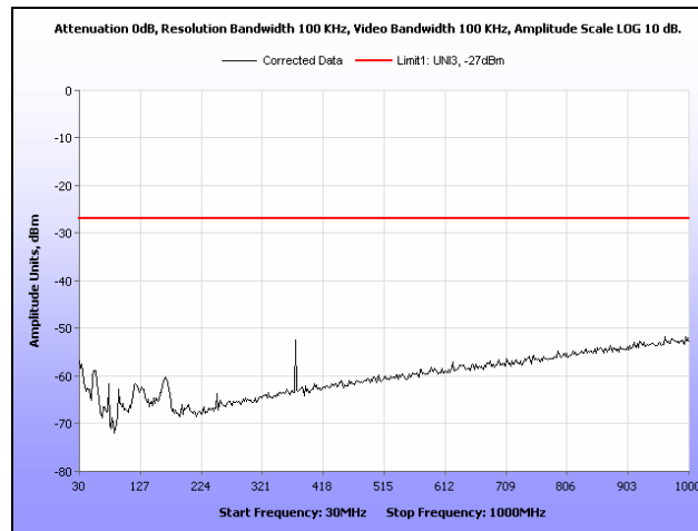
Plot 350. Radiated Spurious Emissions, 802.11n 20 MHz, 5300 MHz, 30 MHz – 1 GHz, Ceiling Mount
