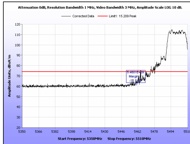
Plot 444. Restricted Band, 802.11n 20 MHz, 5500 MHz, Peak, Patch
