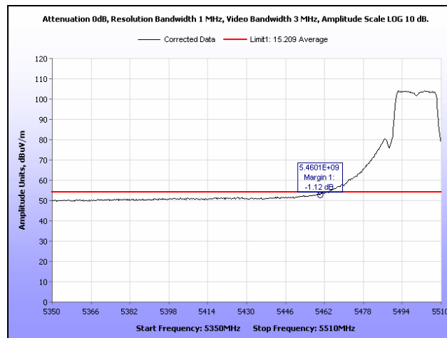
Plot 427. Restricted Band, 802.11a, 5500 MHz, Average
