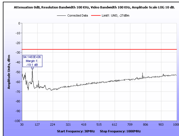
Plot 206. Radiated Spurious Emissions, 802.11n 20 MHz, 5300 MHz, 30 MHz – 1 GHz, 2 dBi Dipole Antenna
