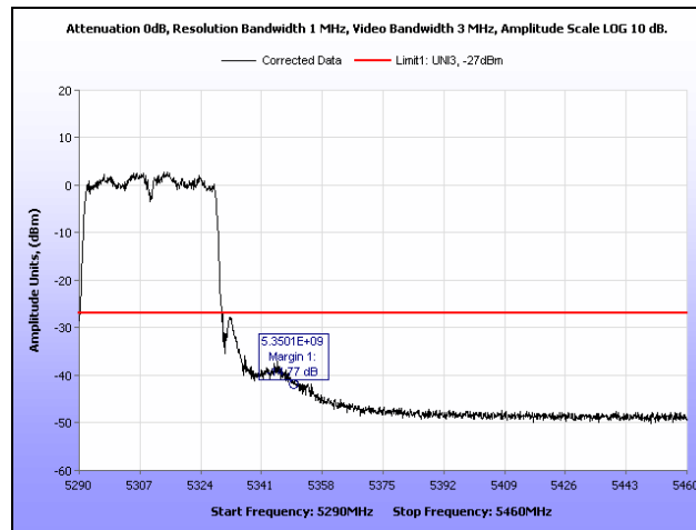
Plot 422. Radiated Band Edge, 802.11n 40 MHz, 5310 MHz, Ceiling Mount
