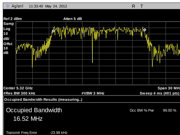
Plot 43. 99% Occupied Bandwidth, 802.11a, A4, 5320 MHz
