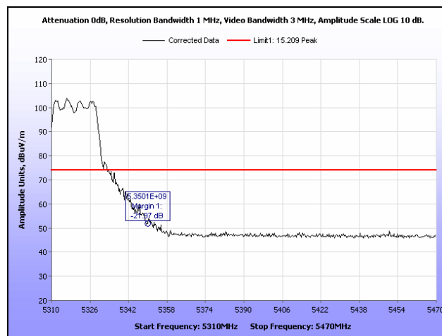
Plot 454. Restricted Band, 802.11n 20 MHz, 5320 MHz, Peak, 6 dBi Dipole Antenna
