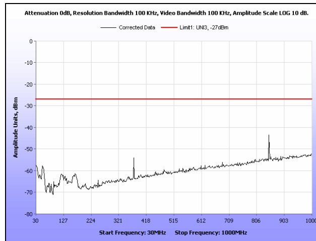
Plot 371. Radiated Spurious Emissions, 802.11n 40 MHz, 5510 MHz, 30 MHz – 1 GHz, Ceiling Mount
