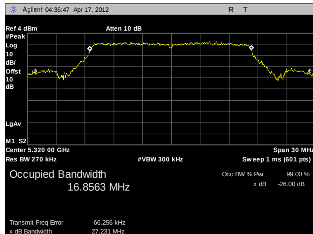
Plot 7. 26 dB Occupied Bandwidth, 802.11a, A4, 5320 MHz
