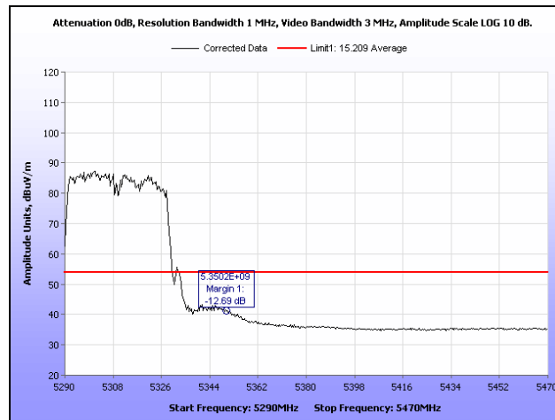
Plot 445. Restricted Band, 802.11n 40 MHz, 5320 MHz, Average, Patch
