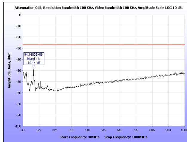
Plot 191. Radiated Spurious Emissions, 802.11a, 5320 MHz, 30 MHz – 1 GHz, 2 dBi Dipole Antenna
