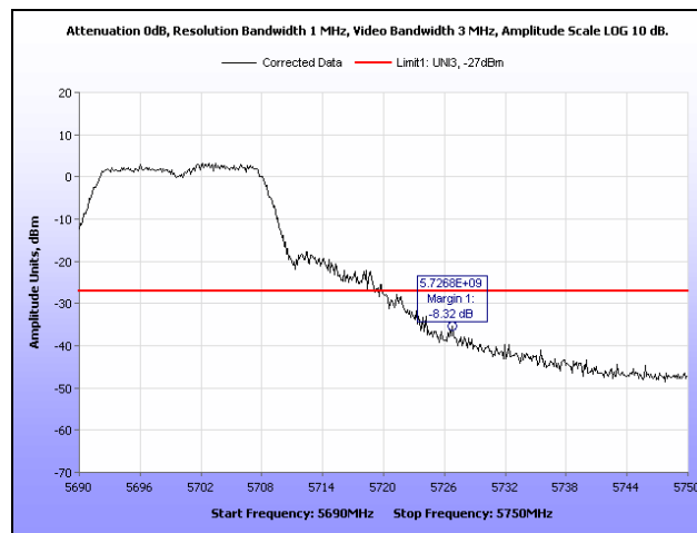
Plot 408. Radiated Band Edge, 802.11n 20 MHz, 5700 MHz, 6 dBi Dipole Antenna
