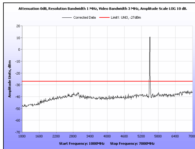
Plot 309. Radiated Spurious Emissions, 802.11n 20 MHz, 5500 MHz, 1 GHz – 7 GHz, 6 dBi Dipole Antenna
