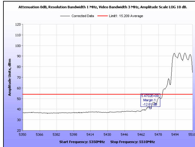
Plot 455. Restricted Band, 802.11n 20 MHz, 5500 MHz, Average, 6 dBi Dipole Antenna
