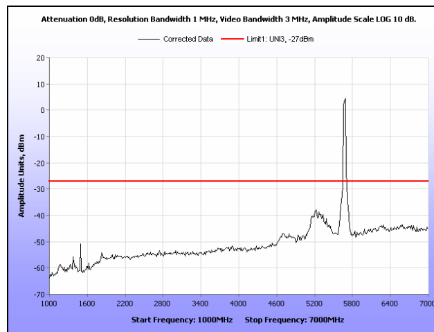
Plot 279. Radiated Spurious Emissions, 802.11n 40 MHz, 5670 MHz, 1 GHz – 7 GHz, Patch
