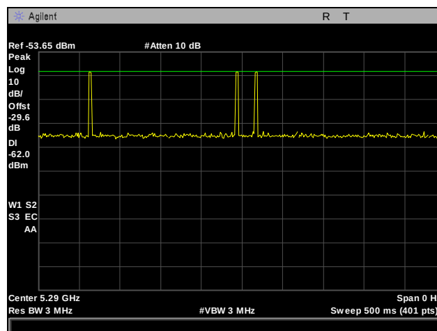
Plot 502. Radar Type 6 Calibration, 5290 MHz
