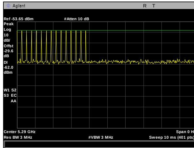
Plot 500. Radar Type 4 Calibration, 5290 MHz
