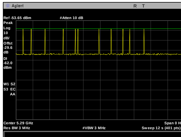
Plot 501. Radar Type 5 Calibration, 5290 MHz
