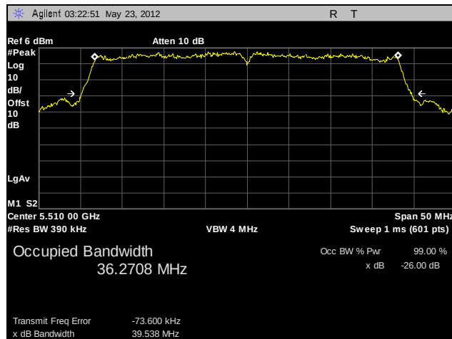
Plot 34. 26 dB Occupied Bandwidth, 802.11n 40 MHz, 5510 MHz, A5
