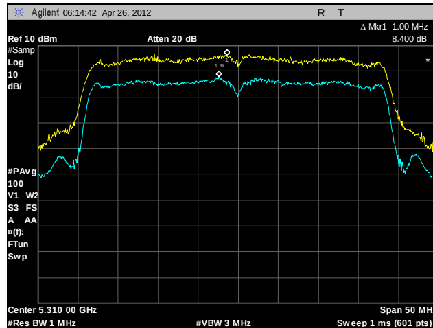
Plot 175. Peak Excursion Ratio, 802.11n 40 MHz, A5, 5310 MHz
