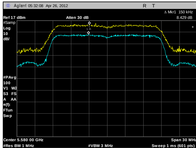
Plot 166. Peak Excursion Ratio, 802.11n 20 MHz, A5, 5580 MHz
