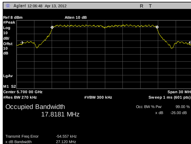
Plot 25. 26 dB Occupied Bandwidth, 802.11n 20 MHz, 5700 MHz, A5
