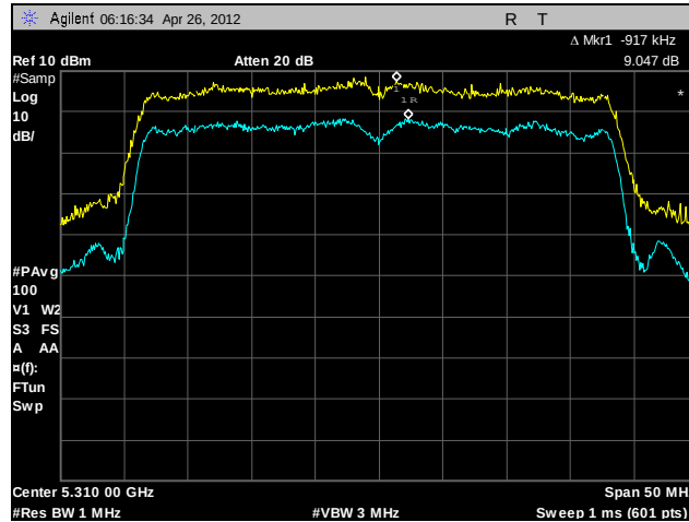
Plot 174. Peak Excursion Ratio, 802.11n 40 MHz, A4, 5310 MHz
