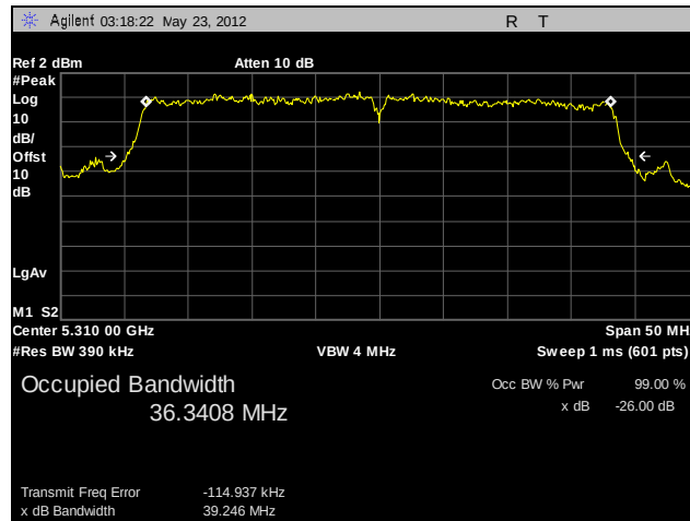
Plot 30. 26 dB Occupied Bandwidth, 802.11n 40 MHz, 5310 MHz, A4
