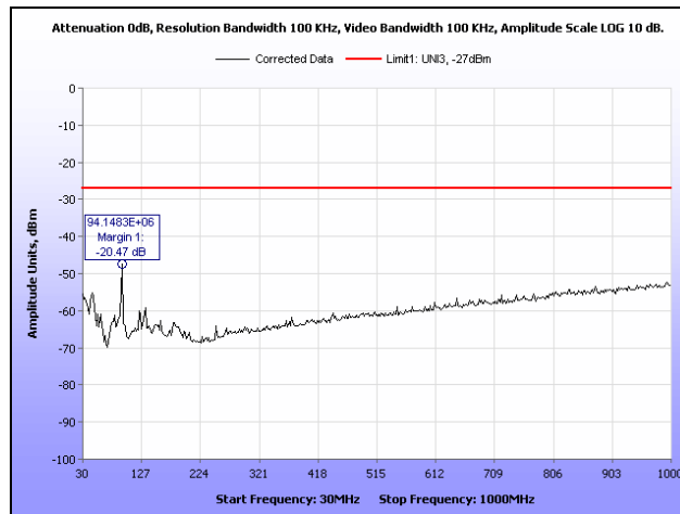
Plot 215. Radiated Spurious Emissions, 802.11n 20 MHz, 5320 MHz, 30 MHz – 1 GHz
