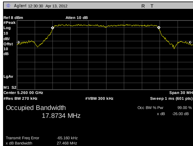
Plot 9. 26 dB Occupied Bandwidth, 802.11n 20 MHz, 5260 MHz, A4
