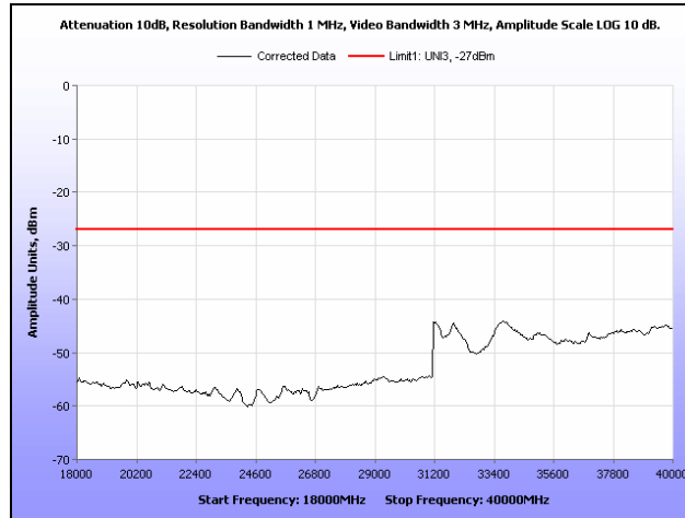
Plot 234. Radiated Spurious Emissions, 802.11n 40 MHz, 5270 MHz, 18 GHz – 40 GHz
