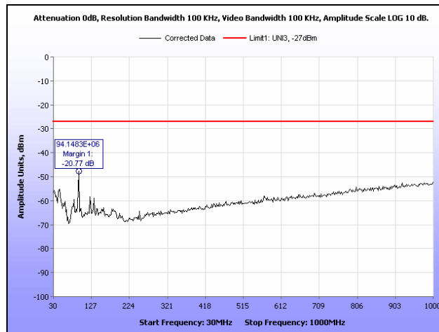
Plot 191. Radiated Spurious Emissions, 802.11a, 5320 MHz, 30 MHz – 1 GHz
