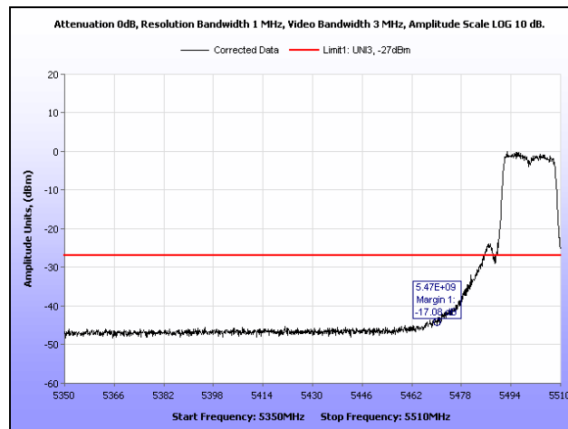
Plot 249. Radiated Band Edge, 802.11a, 5500 MHz
