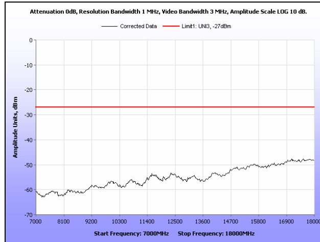
Plot 189. Radiated Spurious Emissions, 802.11a, 5300 MHz, 7 GHz – 18 GHz
