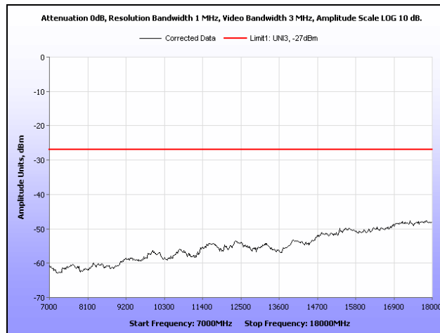
Plot 221. Radiated Spurious Emissions, 802.11n 20 MHz, 5500 MHz, 7 GHz – 18 GHz
