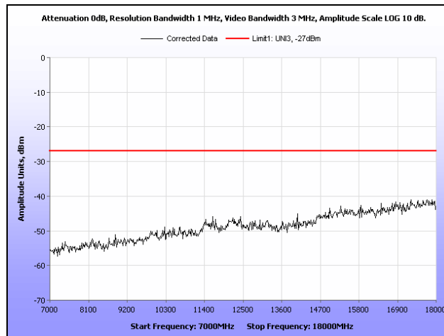
Plot 245. Radiated Spurious Emissions, 802.11n 40 MHz, 5670 MHz, 7 GHz – 18 GHz
