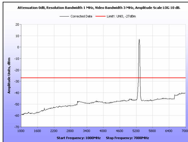
Plot 236. Radiated Spurious Emissions, 802.11n 40 MHz, 5310 MHz, 1 GHz – 7 GHz
