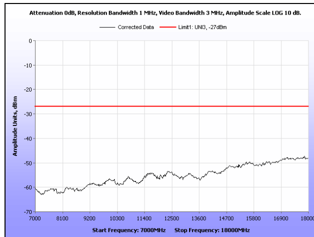
Plot 197. Radiated Spurious Emissions, 802.11a, 5500 MHz, 7 GHz – 18 GHz
