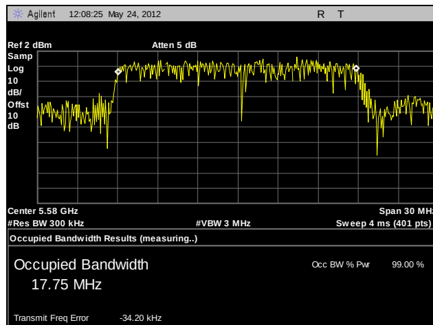
Plot 59. 99% Occupied Bandwidth, 802.11n 20 MHz, 5580 MHz, A6
