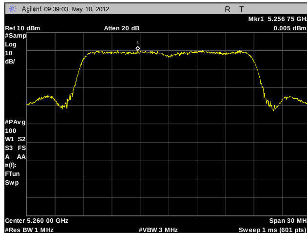
Plot 118. Peak Spectral Density, 802.11n 20 MHz, 5260 MHz, A5
