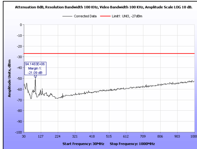
Plot 207. Radiated Spurious Emissions, 802.11n 20 MHz, 5260 MHz, 30 MHz – 1 GHz
