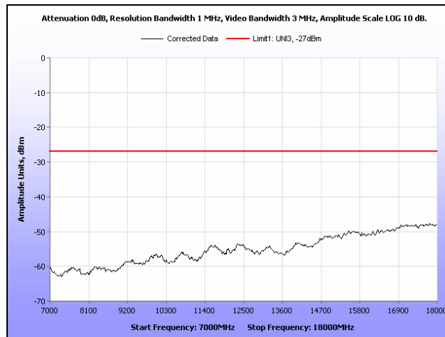
Plot 209. Radiated Spurious Emissions, 802.11n 20 MHz, 5260 MHz, 7 GHz – 18 GHz
