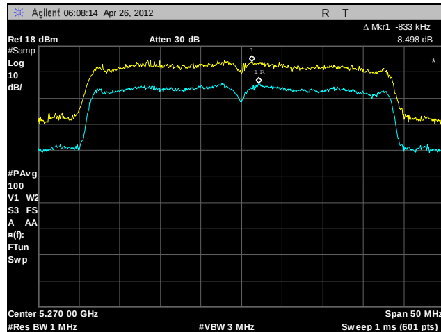
Plot 172. Peak Excursion Ratio, 802.11n 40 MHz, A5, 5270 MHz
