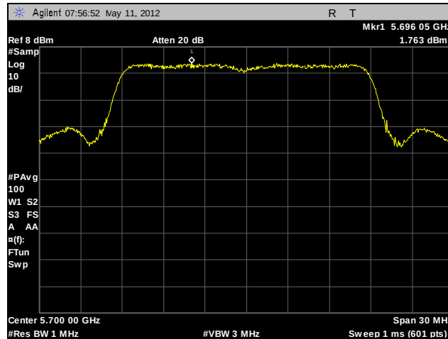
Plot 132. Peak Spectral Density, 802.11n 20 MHz, 5700 MHz, A4
