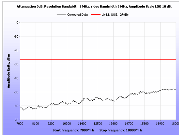
Plot 237. Radiated Spurious Emissions, 802.11n 40 MHz, 5310 MHz, 7 GHz – 18 GHz
