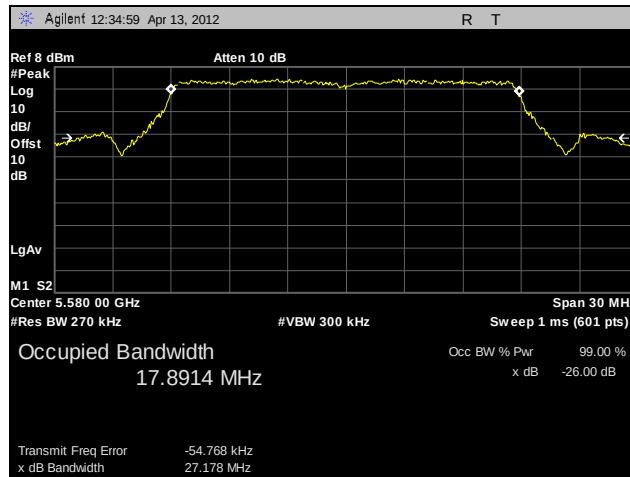
Plot 21. 26 dB Occupied Bandwidth, 802.11n 20 MHz, 5580 MHz, A4
