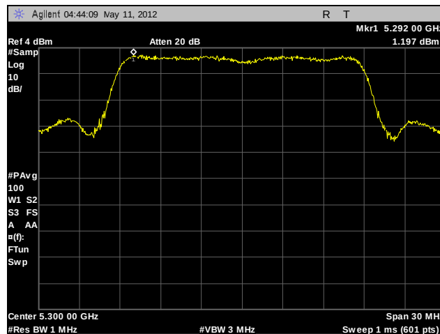
Plot 121. Peak Spectral Density, 802.11n 20 MHz, 5300 MHz, A5
