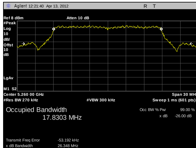
Plot 10. 26 dB Occupied Bandwidth, 802.11n 20 MHz, 5260 MHz, A5
