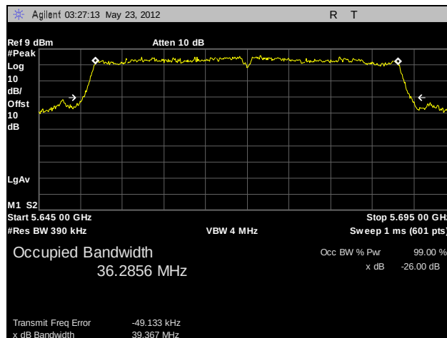
Plot 38. 26 dB Occupied Bandwidth, 802.11n 40 MHz, 5670 MHz, A6
