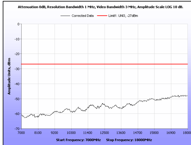
Plot 225. Radiated Spurious Emissions, 802.11n 20 MHz, 5580 MHz, 7 GHz – 18 GHz
