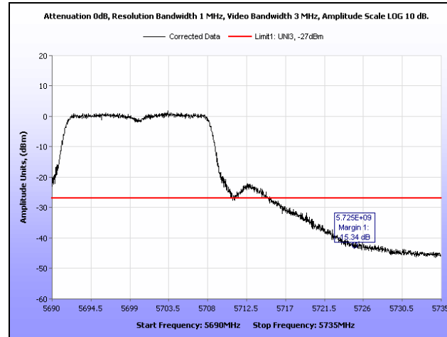
Plot 250. Radiated Band Edge, 802.11a, 5700 MHz
