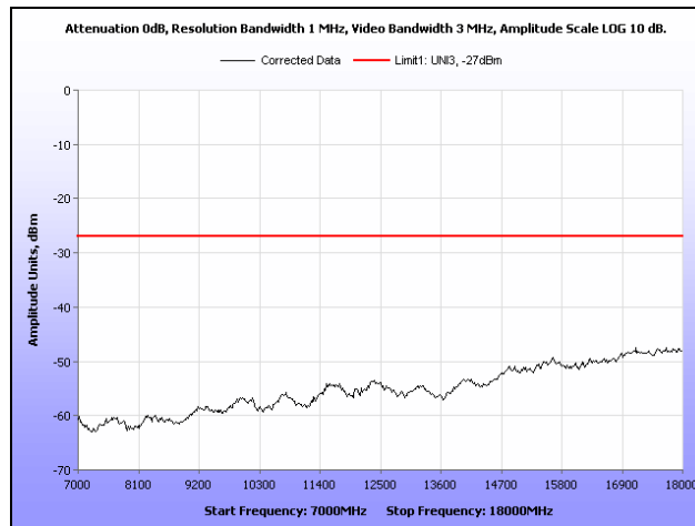
Plot 233. Radiated Spurious Emissions, 802.11n 40 MHz, 5270 MHz, 7 GHz – 18 GHz
