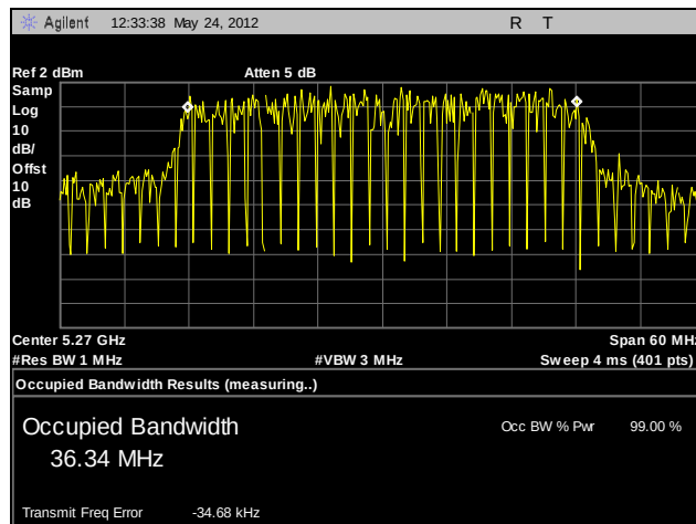
Plot 65. 99% Occupied Bandwidth, 802.11n 40 MHz, 5270 MHz, A6
