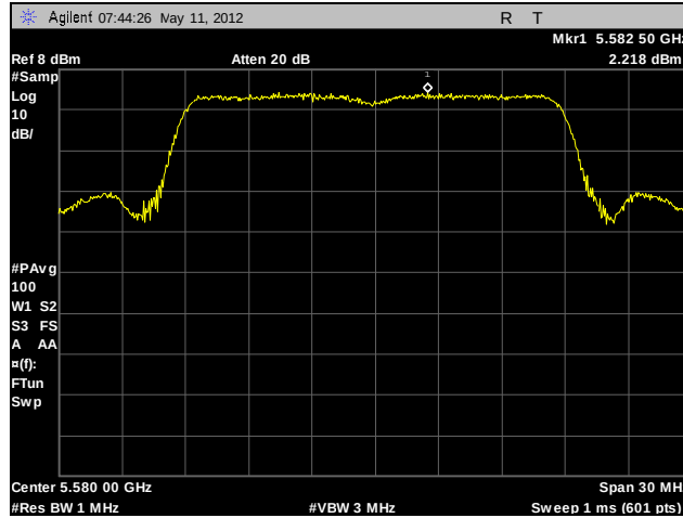
Plot 129. Peak Spectral Density, 802.11n 20 MHz, 5580 MHz, A4
