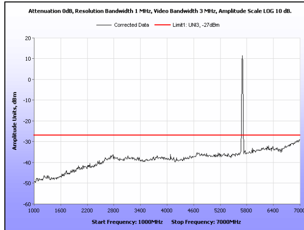
Plot 204. Radiated Spurious Emissions, 802.11a, 5700 MHz, 1 GHz – 7 GHz
