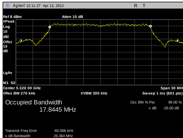
Plot 16. 26 dB Occupied Bandwidth, 802.11n 20 MHz, 5320 MHz, A5
