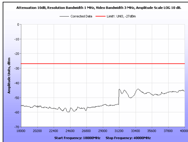
Plot 206. Radiated Spurious Emissions, 802.11a, 5700 MHz, 18 GHz – 40 GHz
