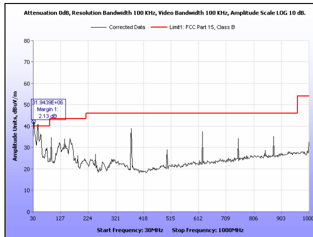
Plot 239. Radiated Spurious Emissions, 802.11n 40 MHz, 5510 MHz, 30 MHz – 1 GHz
