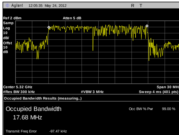
Plot 52. 99% Occupied Bandwidth, 802.11n 20 MHz, 5320 MHz, A5
