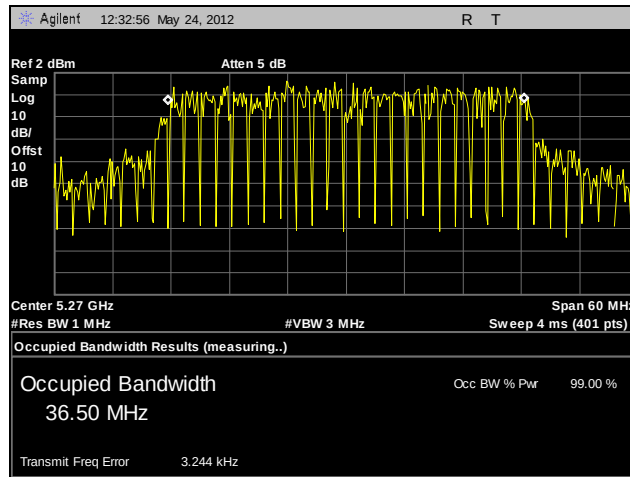
Plot 63. 99% Occupied Bandwidth, 802.11n 40 MHz, 5270 MHz, A4
