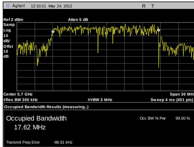
Plot 60. 99% Occupied Bandwidth, 802.11n 20 MHz, 5700 MHz, A4
