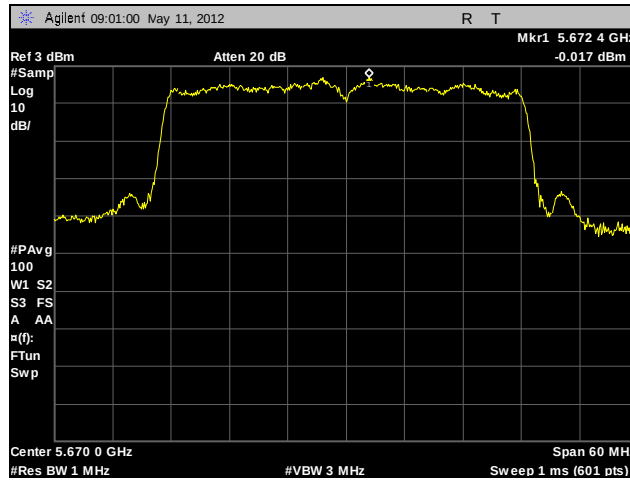
Plot 144. Peak Spectral Density, 802.11n 40 MHz, 5670 MHz, A4
