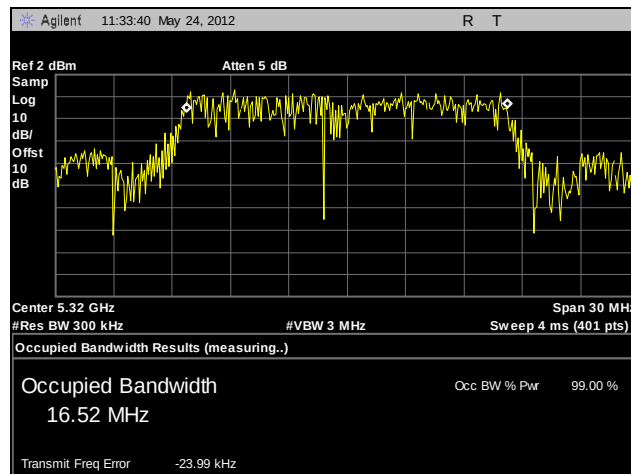
Plot 41. 99% Occupied Bandwidth, 802.11a, 5320 MHz, A4
