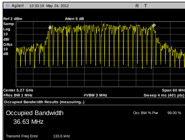
Plot 64. 99% Occupied Bandwidth, 802.11n 40 MHz, 5270 MHz, A5
