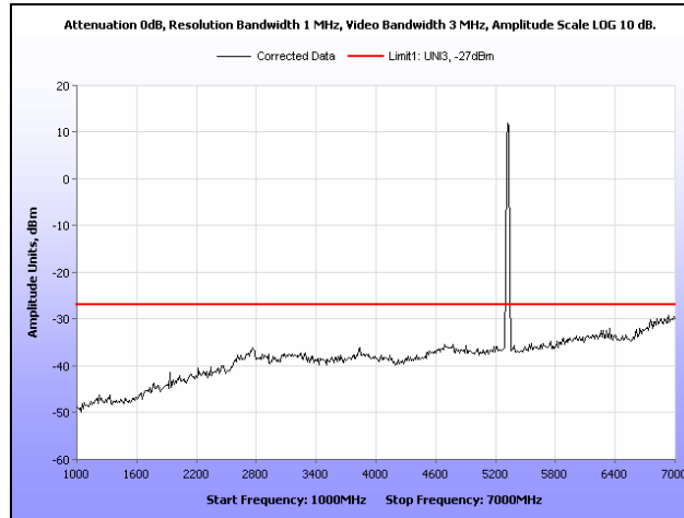
Plot 216. Radiated Spurious Emissions, 802.11n 20 MHz, 5320 MHz, 1 GHz – 7 GHz
