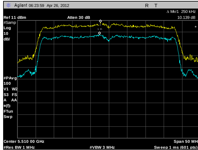
Plot 177. Peak Excursion Ratio, 802.11n 40 MHz, A4, 5510 MHz
