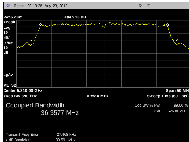
Plot 31. 26 dB Occupied Bandwidth, 802.11n 40 MHz, 5310 MHz, A5
