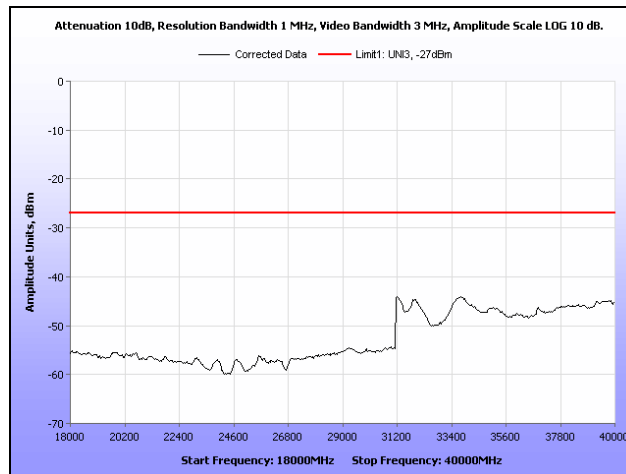
Plot 218. Radiated Spurious Emissions, 802.11n 20 MHz, 5320 MHz, 18 GHz – 40 GHz
