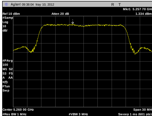
Plot 117. Peak Spectral Density, 802.11n 20 MHz, 5260 MHz, A4
