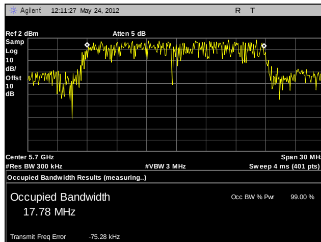
Plot 62. 99% Occupied Bandwidth, 802.11n 20 MHz, 5700 MHz, A6
