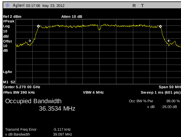
Plot 27. 26 dB Occupied Bandwidth, 802.11n 40 MHz, 5270 MHz, A4
