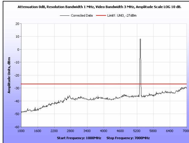
Plot 192. Radiated Spurious Emissions, 802.11a, 5320 MHz, 1 GHz – 7 GHz
