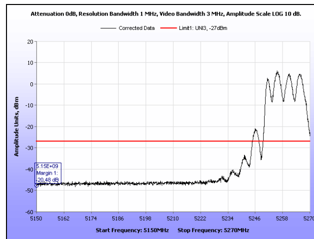
Plot 251. Radiated Band Edge, 802.11n 20 MHz, 5260 MHz
