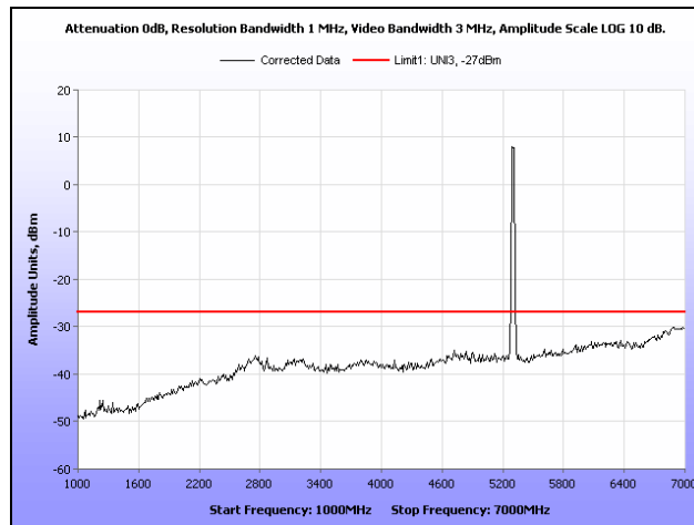
Plot 188. Radiated Spurious Emissions, 802.11a, 5300 MHz, 1 GHz – 7 GHz
