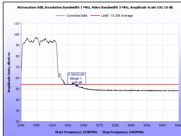
Plot 267. Restricted Band, 802.11n 40 MHz, 5310 MHz, Average
