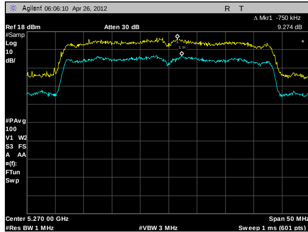
Plot 171. Peak Excursion Ratio, 802.11n 40 MHz, A4, 5270 MHz
