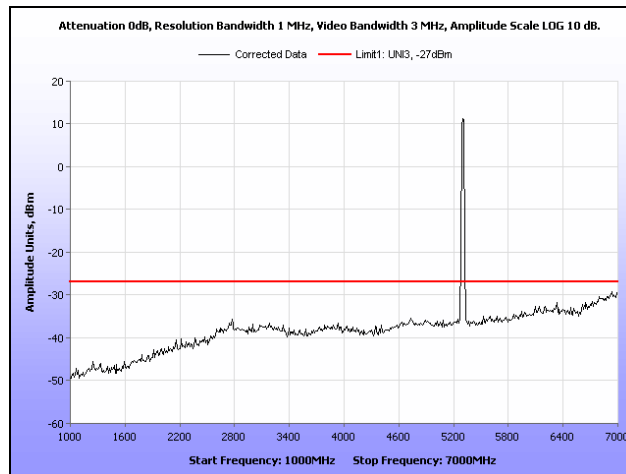
Plot 212. Radiated Spurious Emissions, 802.11n 20 MHz, 5300 MHz, 1 GHz – 7 GHz
