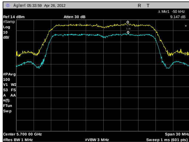
Plot 169. Peak Excursion Ratio, 802.11n 20 MHz, A5, 5700 MHz
