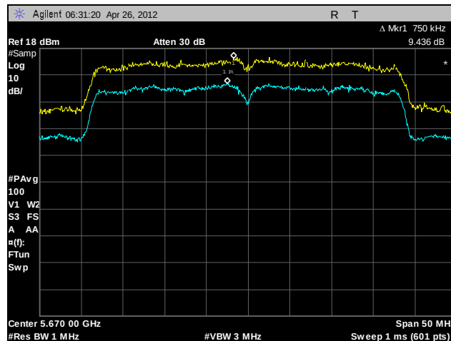
Plot 182. Peak Excursion Ratio, 802.11n 40 MHz, A6, 5670 MHz
