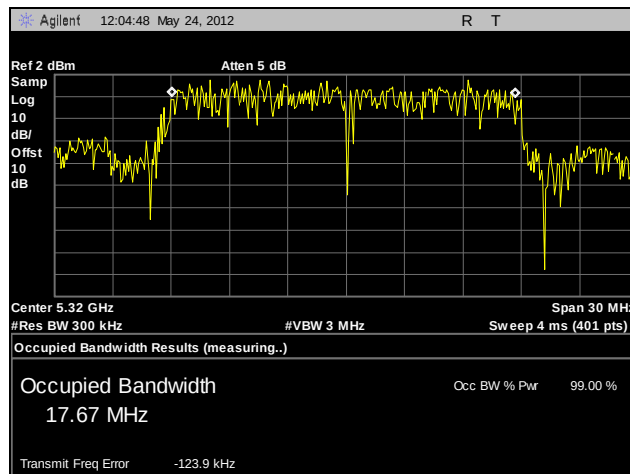
Plot 53. 99% Occupied Bandwidth, 802.11n 20 MHz, 5320 MHz, A6
