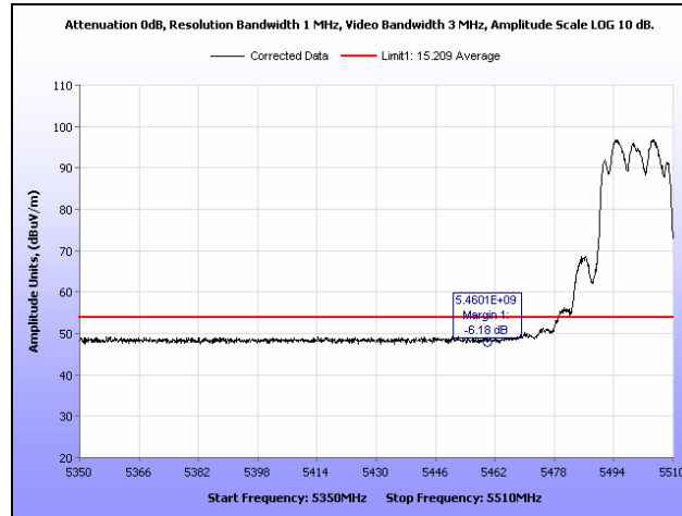
Plot 265. Restricted Band, 802.11n 20 MHz, 5500 MHz, Average
