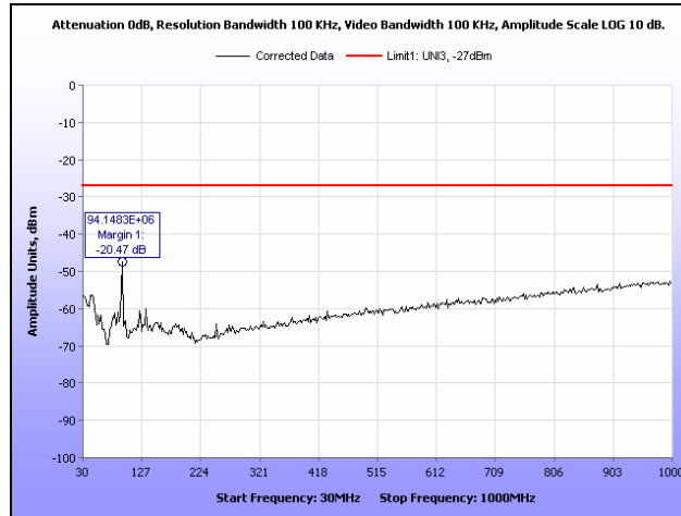
Plot 195. Radiated Spurious Emissions, 802.11a, 5500 MHz, 30 MHz – 1 GHz
