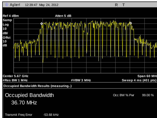
Plot 73. 99% Occupied Bandwidth, 802.11n 40 MHz, 5670 MHz, A5
