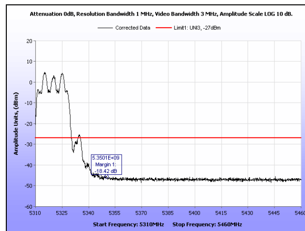
Plot 252. Radiated Band Edge, 802.11n 20 MHz, 5320 MHz
