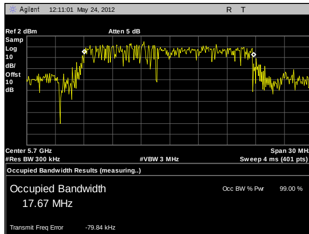
Plot 61. 99% Occupied Bandwidth, 802.11n 20 MHz, 5700 MHz, A5
