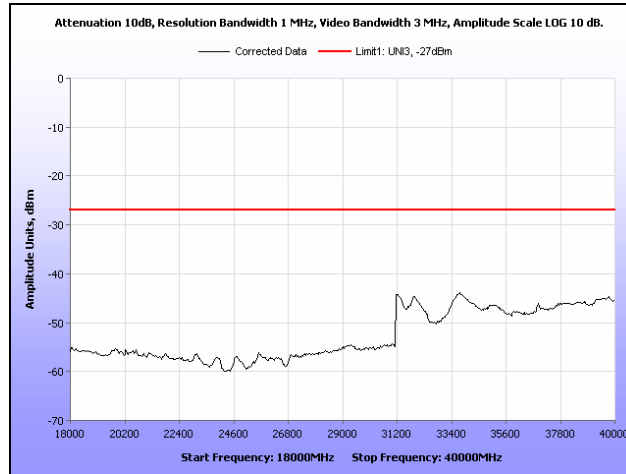
Plot 198. Radiated Spurious Emissions, 802.11a, 5500 MHz, 18 GHz – 40 GHz
