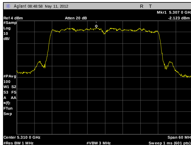
Plot 139. Peak Spectral Density, 802.11n 40 MHz, 5310 MHz, A5
