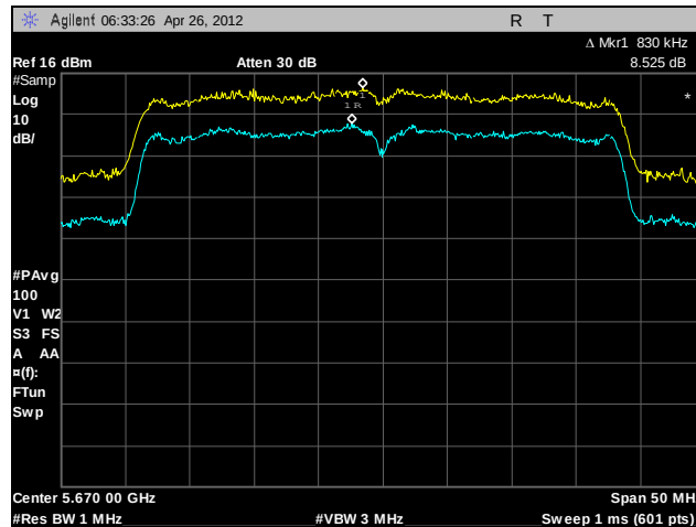
Plot 181. Peak Excursion Ratio, 802.11n 40 MHz, A5, 5670 MHz
