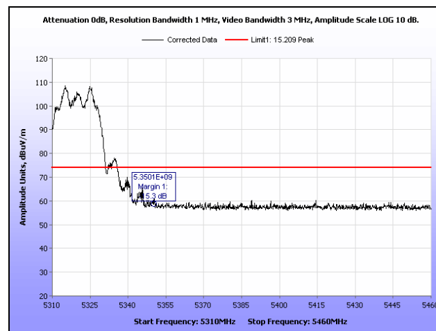
Plot 264. Restricted Band, 802.11n 20 MHz, 5320 MHz, Peak
