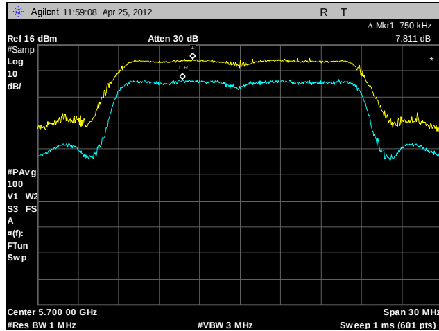
Plot 168. Peak Excursion Ratio, 802.11n 20 MHz, A4, 5700 MHz
