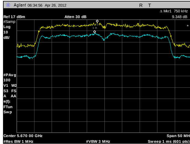
Plot 180. Peak Excursion Ratio, 802.11n 40 MHz, A4, 5670 MHz
