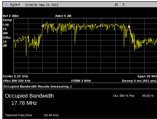
Plot 51. 99% Occupied Bandwidth, 802.11n 20 MHz, 5320 MHz, A4
