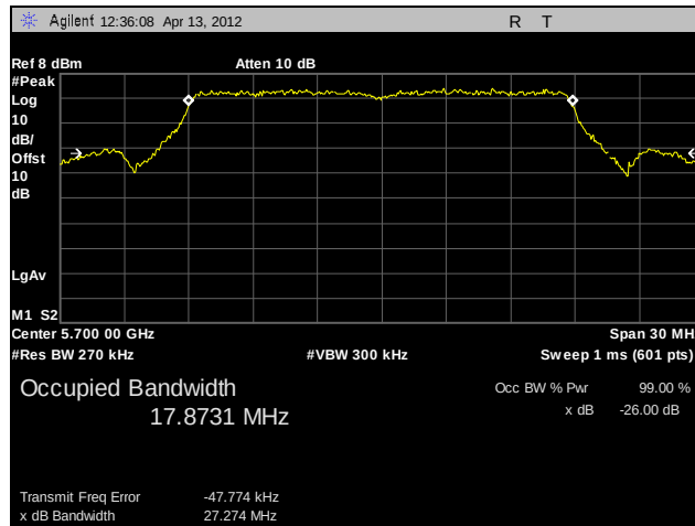
Plot 24. 26 dB Occupied Bandwidth, 802.11n 20 MHz, 5700 MHz, A4
