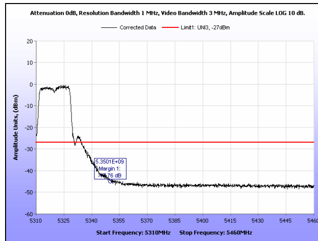
Plot 248. Radiated Band Edge, 802.11a, 5320 MHz
