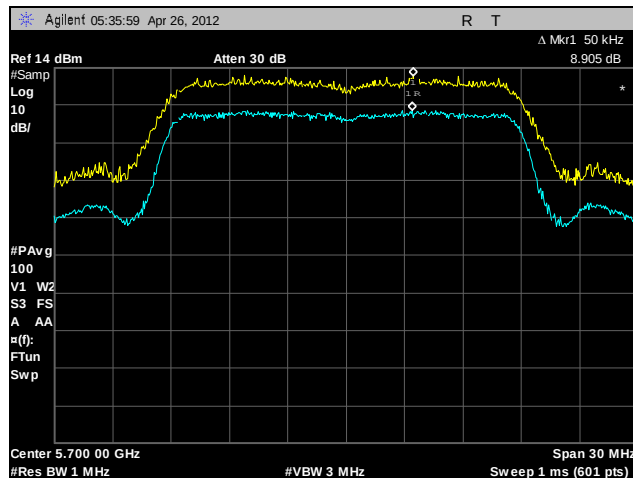
Plot 170. Peak Excursion Ratio, 802.11n 20 MHz, A6, 5700 MHz
