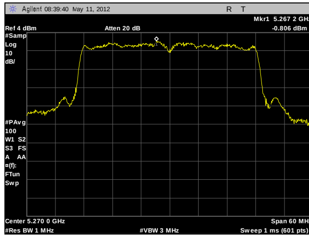
Plot 136. Peak Spectral Density, 802.11n 40 MHz, 5270 MHz, A5
