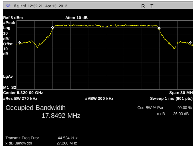
Plot 15. 26 dB Occupied Bandwidth, 802.11n 20 MHz, 5320 MHz, A4
