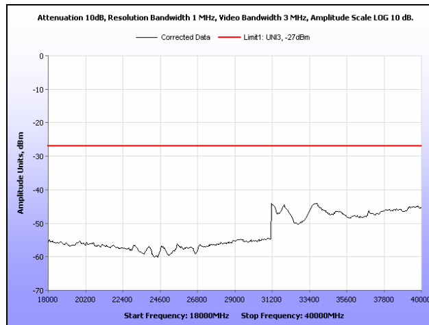
Plot 194. Radiated Spurious Emissions, 802.11a, 5320 MHz, 18 GHz – 40 GHz
