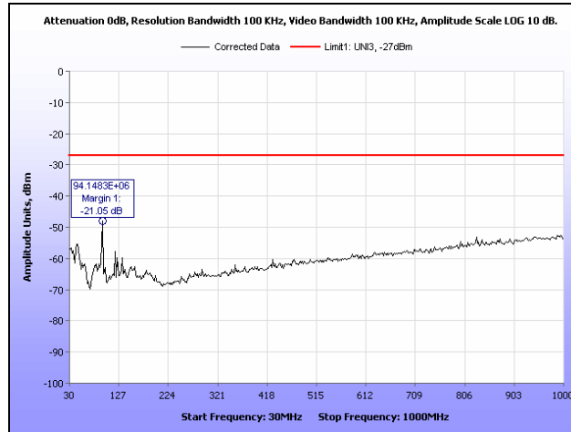
Plot 219. Radiated Spurious Emissions, 802.11n 20 MHz, 5500 MHz, 30 MHz – 1 GHz
