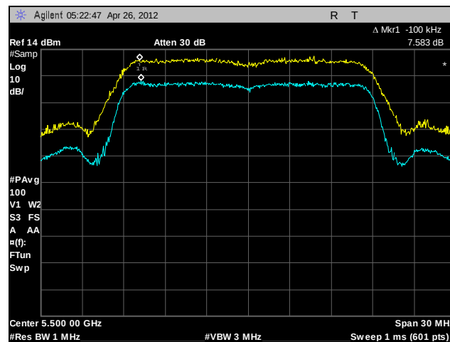
Plot 163. Peak Excursion Ratio, 802.11n 20 MHz, A5, 5500 MHz
