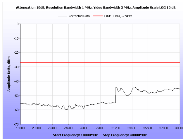
Plot 242. Radiated Spurious Emissions, 802.11n 40 MHz, 5510 MHz, 18 GHz – 40 GHz
