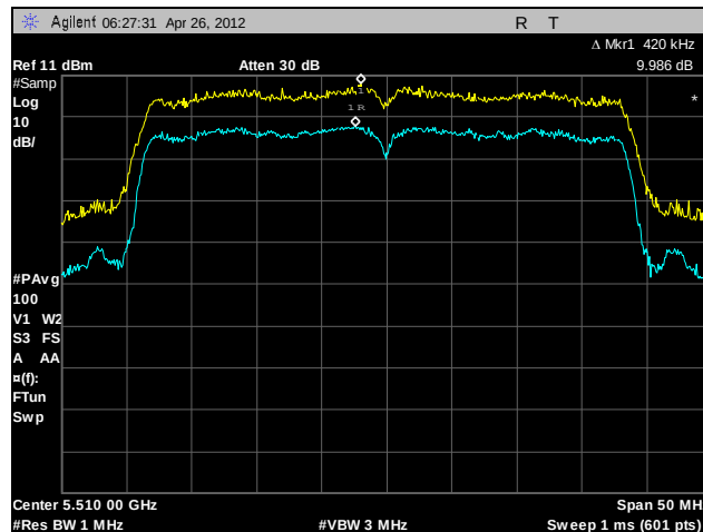
Plot 179. Peak Excursion Ratio, 802.11n 40 MHz, A6, 5510 MHz
