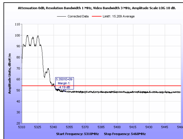
Plot 263. Restricted Band, 802.11n 20 MHz, 5320 MHz, Average
