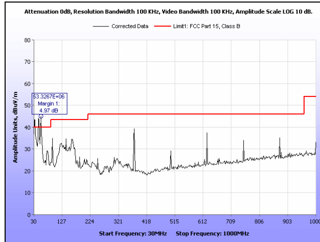
Plot 231. Radiated Spurious Emissions, 802.11n 40 MHz, 5270 MHz, 30 MHz – 1 GHz
