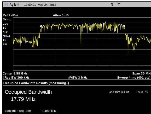
Plot 58. 99% Occupied Bandwidth, 802.11n 20 MHz, 5580 MHz, A5
