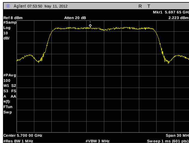
Plot 133. Peak Spectral Density, 802.11n 20 MHz, 5700 MHz, A5
