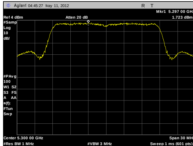
Plot 120. Peak Spectral Density, 802.11n 20 MHz, 5300 MHz, A4
