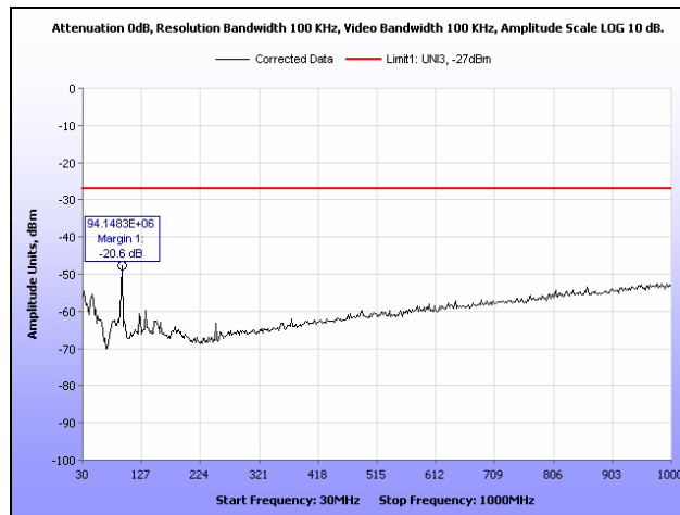
Plot 227. Radiated Spurious Emissions, 802.11n 20 MHz, 5700 MHz, 30 MHz – 1 GHz
