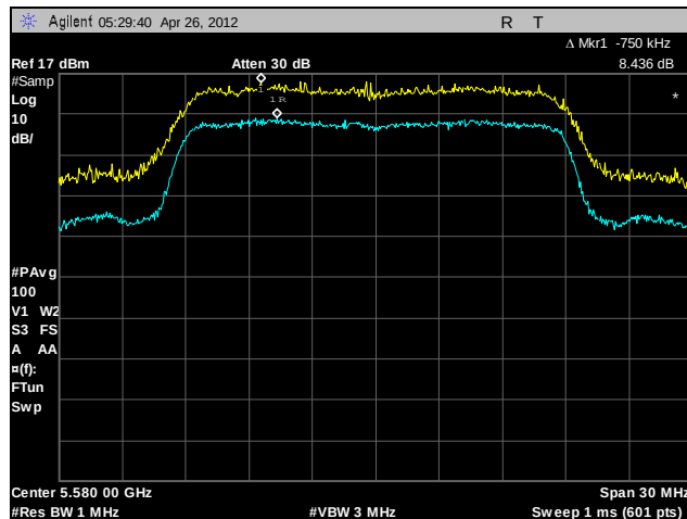
Plot 167. Peak Excursion Ratio, 802.11n 20 MHz, A6, 5580 MHz
