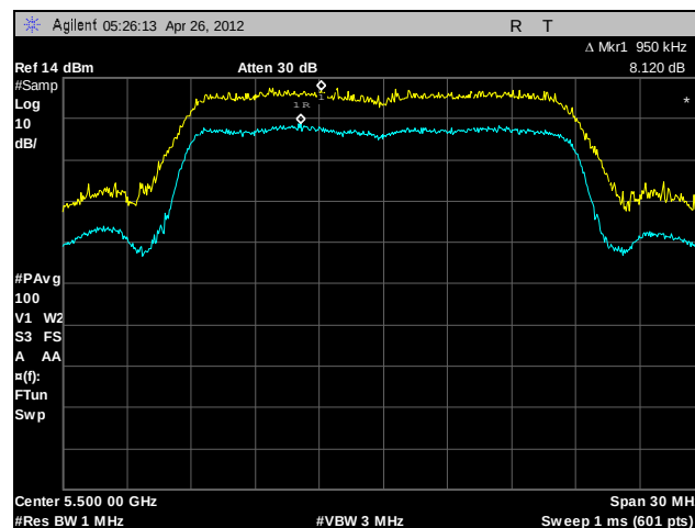
Plot 164. Peak Excursion Ratio, 802.11n 20 MHz, A6, 5500 MHz
