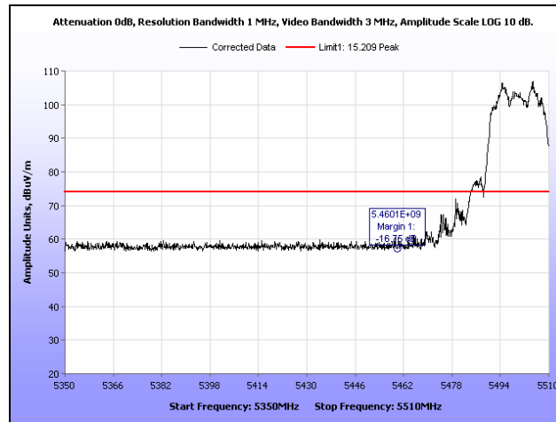
Plot 266. Restricted Band, 802.11n 20 MHz, 5500 MHz, Peak
