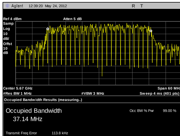
Plot 74. 99% Occupied Bandwidth, 802.11n 40 MHz, 5670 MHz, A6
