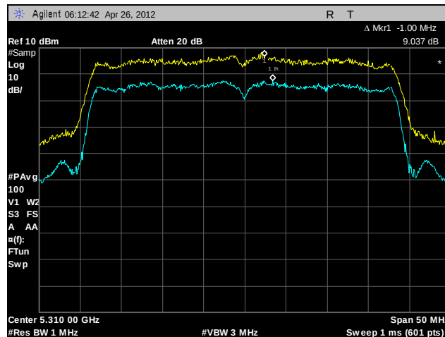
Plot 176. Peak Excursion Ratio, 802.11n 40 MHz, A6, 5310 MHz
