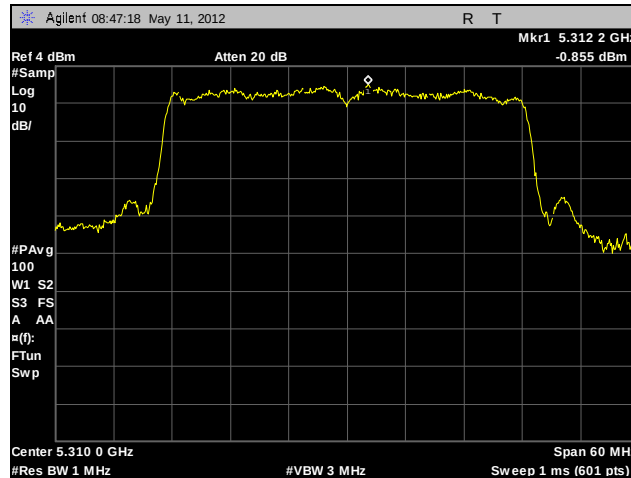
Plot 138. Peak Spectral Density, 802.11n 40 MHz, 5310 MHz, A4
