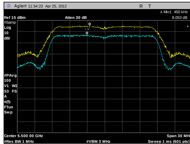
Plot 162. Peak Excursion Ratio, 802.11n 20 MHz, A4, 5500 MHz
