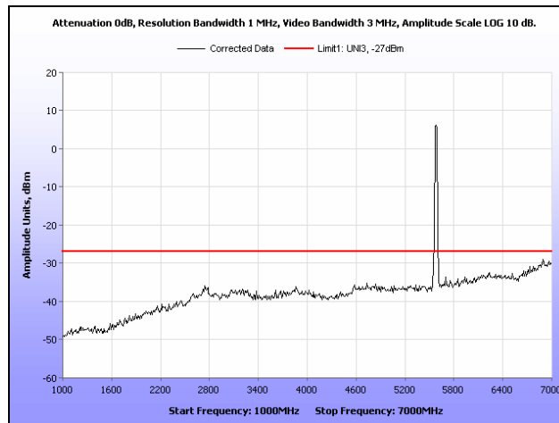
Plot 200. Radiated Spurious Emissions, 802.11a, 5580 MHz, 1 GHz – 7 GHz
