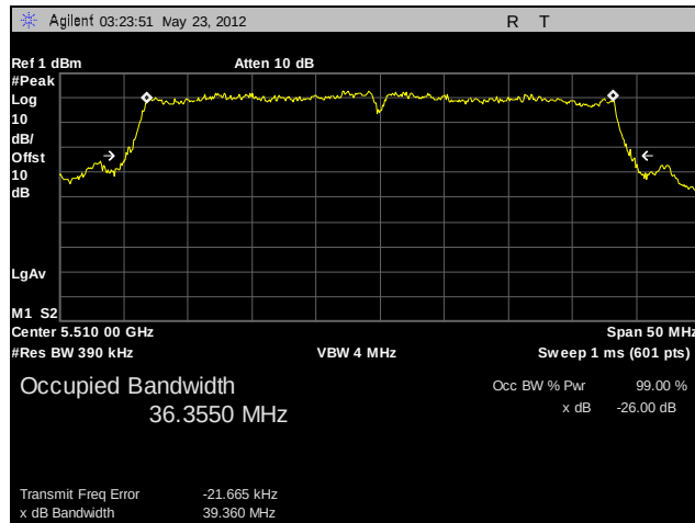
Plot 33. 26 dB Occupied Bandwidth, 802.11n 40 MHz, 5510 MHz, A4
