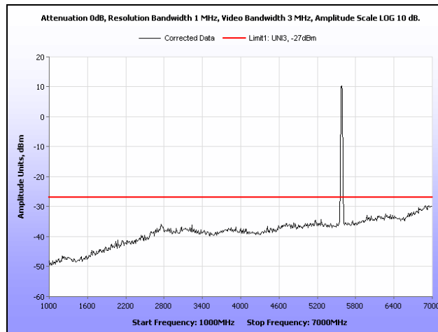
Plot 224. Radiated Spurious Emissions, 802.11n 20 MHz, 5580 MHz, 1 GHz – 7 GHz
