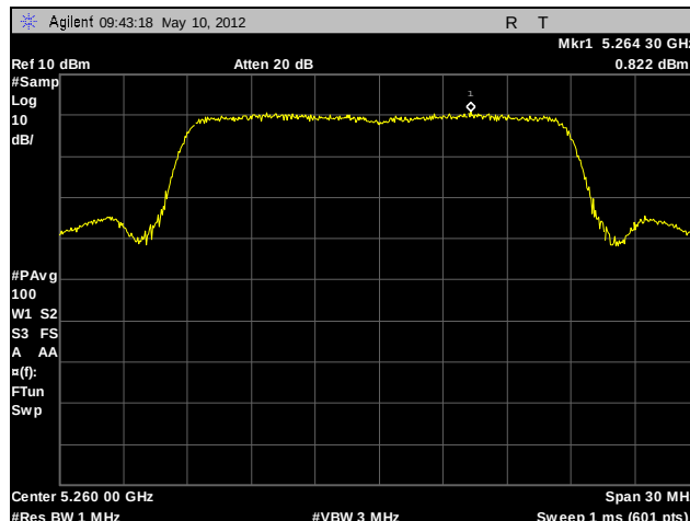
Plot 119. Peak Spectral Density, 802.11n 20 MHz, 5260 MHz, A6
