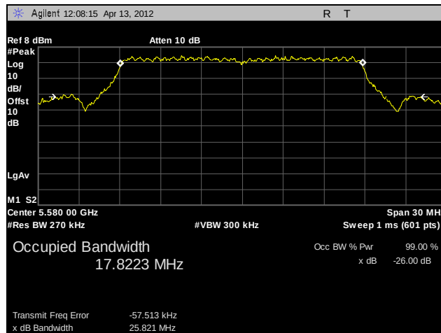
Plot 22. 26 dB Occupied Bandwidth, 802.11n 20 MHz, 5580 MHz, A5
