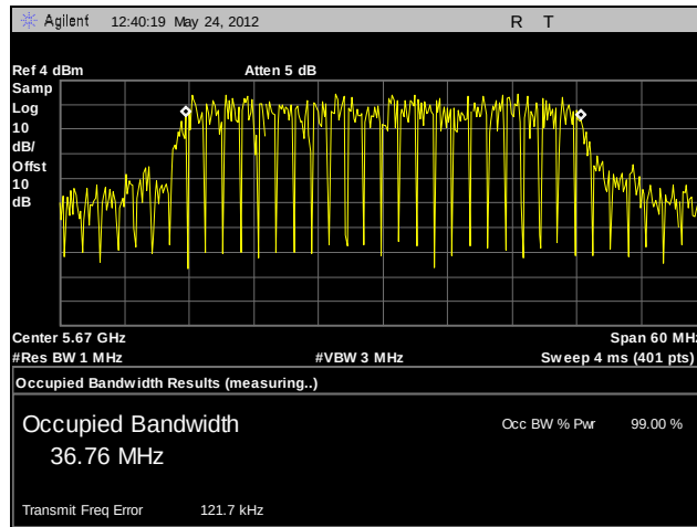
Plot 72. 99% Occupied Bandwidth, 802.11n 40 MHz, 5670 MHz, A4
