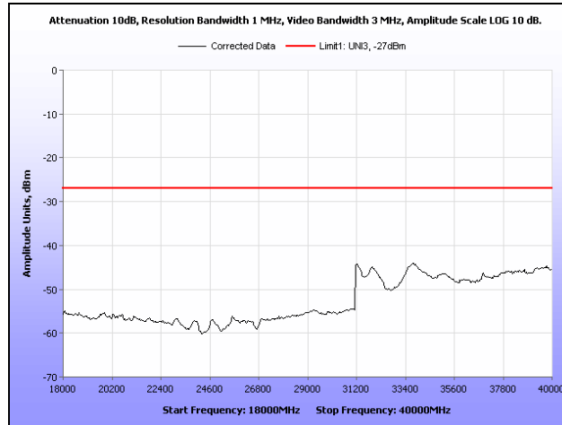
Plot 186. Radiated Spurious Emissions, 802.11a, 5260 MHz, 18 GHz – 40 GHz
