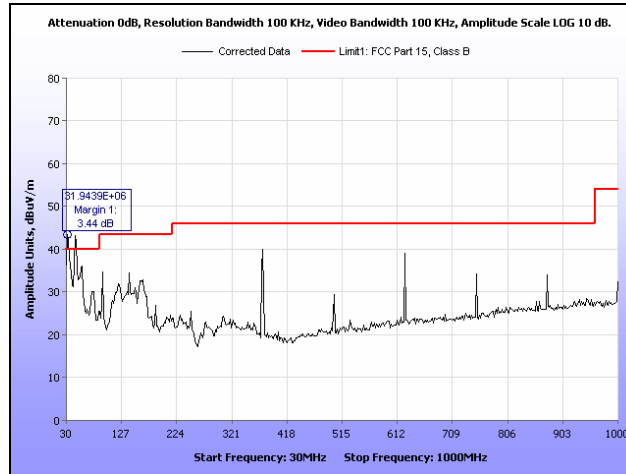
Plot 243. Radiated Spurious Emissions, 802.11n 40 MHz, 5670 MHz, 30 MHz – 1 GHz
