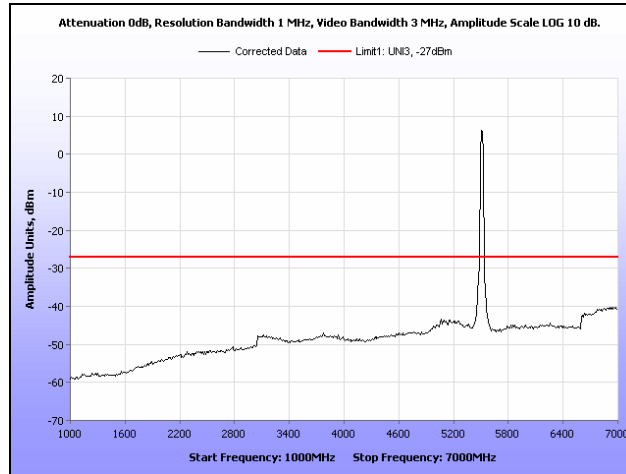
Plot 240. Radiated Spurious Emissions, 802.11n 40 MHz, 5510 MHz, 1 GHz – 7 GHz
