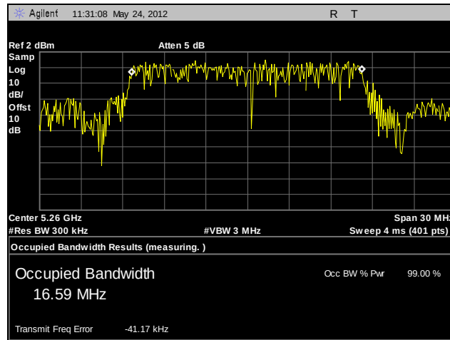
Plot 39. 99% Occupied Bandwidth, 802.11a, 5260 MHz, A4
