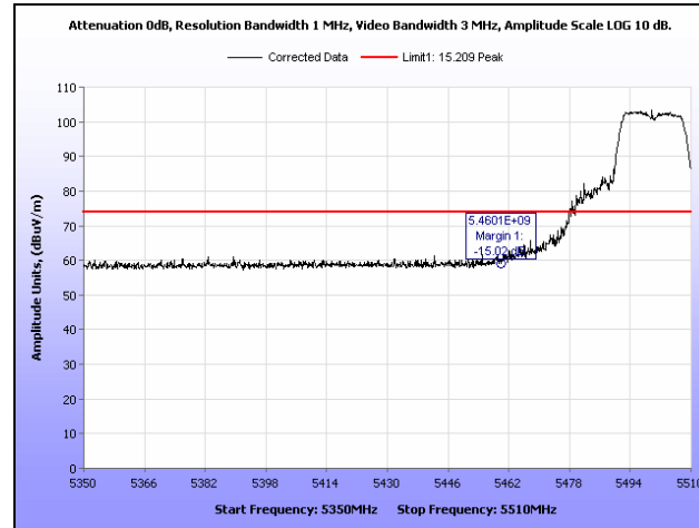
Plot 262. Restricted Band, 802.11a, 5500 MHz, Peak
