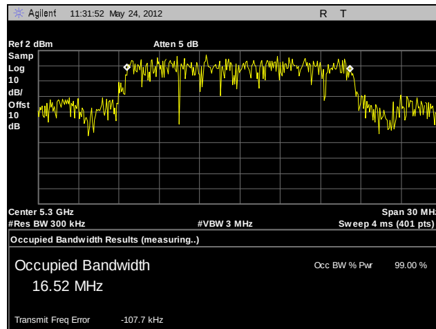
Plot 40. 99% Occupied Bandwidth, 802.11a, 5300 MHz, A4
