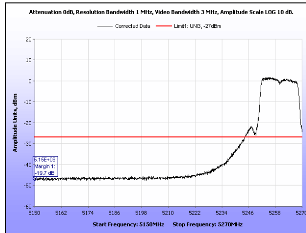
Plot 247. Radiated Band Edge, 802.11a, 5260 MHz
