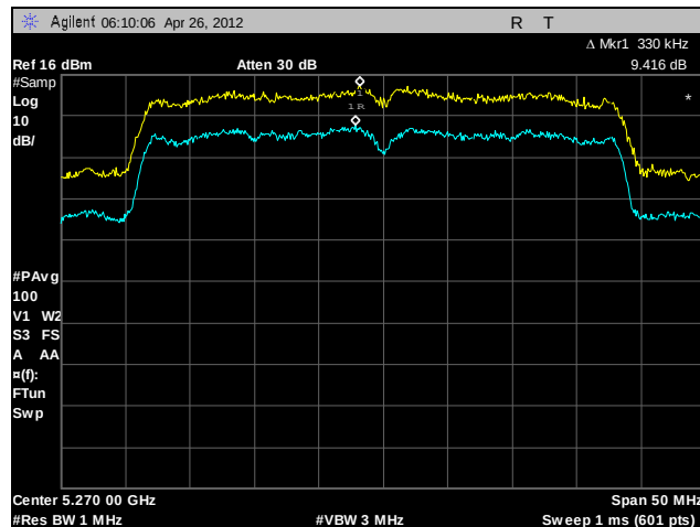
Plot 173. Peak Excursion Ratio, 802.11n 40 MHz, A6, 5270 MHz
