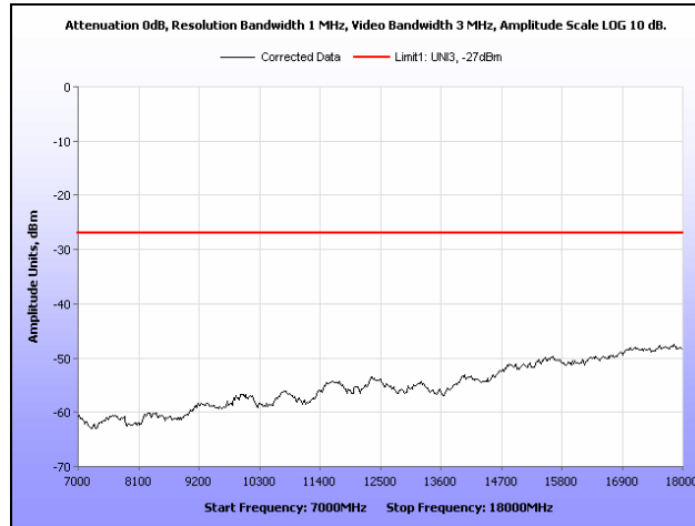
Plot 213. Radiated Spurious Emissions, 802.11n 20 MHz, 5300 MHz, 7 GHz – 18 GHz
