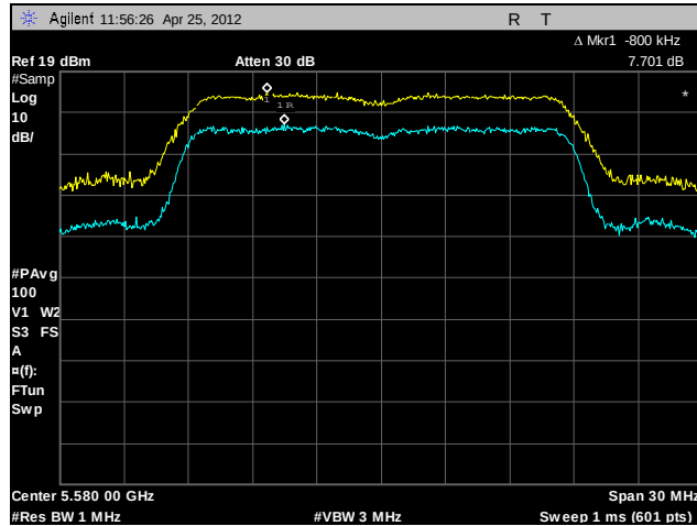
Plot 165. Peak Excursion Ratio, 802.11n 20 MHz, A4, 5580 MHz
