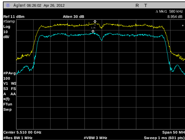
Plot 178. Peak Excursion Ratio, 802.11n 40 MHz, A5, 5510 MHz
