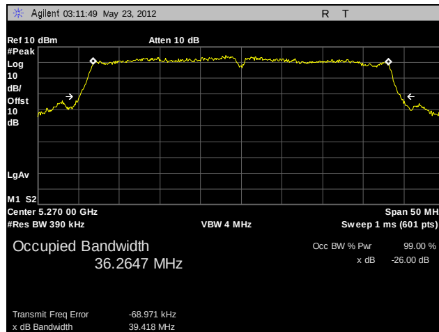
Plot 28. 26 dB Occupied Bandwidth, 802.11n 40 MHz, 5270 MHz, A5
