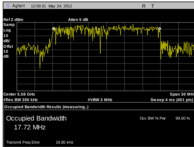
Plot 57. 99% Occupied Bandwidth, 802.11n 20 MHz, 5580 MHz, A4
