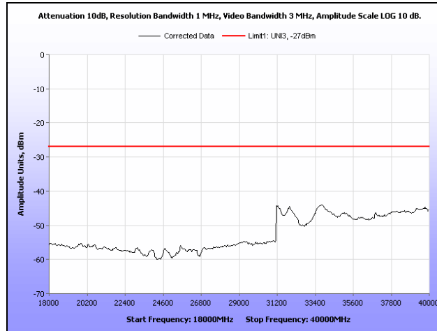
Plot 210. Radiated Spurious Emissions, 802.11n 20 MHz, 5260 MHz, 18 GHz – 40 GHz
