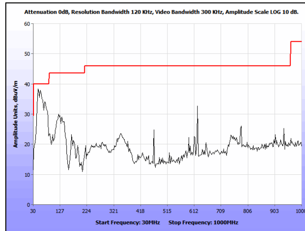
Plot 371. Radiated Spurious Emissions, 802.11n 20 MHz, Low Channel, 30 MHz – 1 GHz, Ceiling, 5500 MHz
