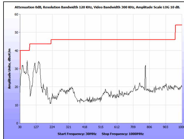
Plot 431. Radiated Spurious Emissions, 802.11n 40 MHz, Mid Channel, 30 MHz – 1 GHz, Omni, 5550 MHz
