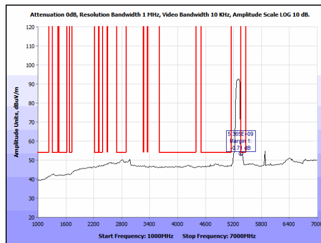
Plot 276. Radiated Spurious Emissions, 802.11n 80 MHz, 1 GHz – 7 GHz, Average, Ceiling, 5290 MHz
