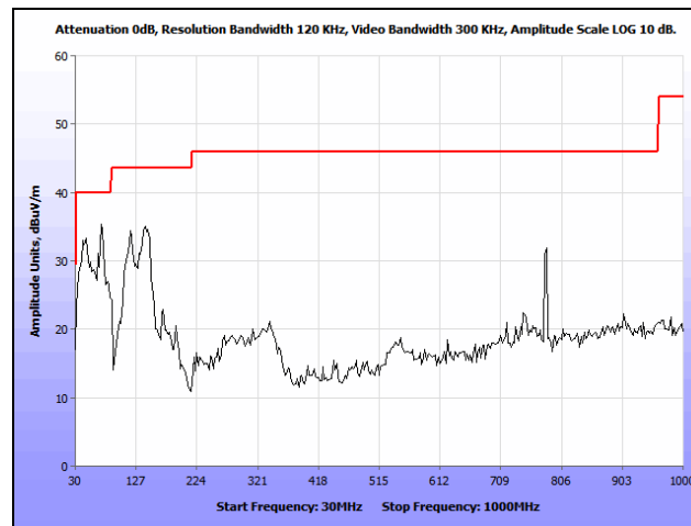
Plot 439. Radiated Spurious Emissions, 802.11n 80 MHz, 30 MHz – 1 GHz, Omni, 5530 MHz
