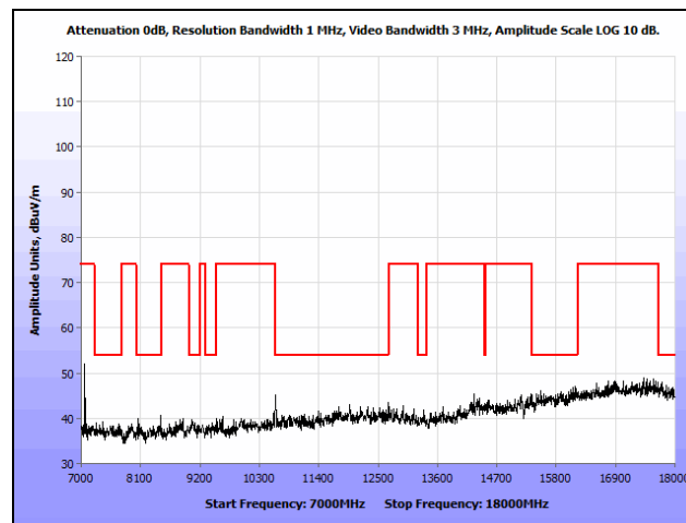
Plot 298. Radiated Spurious Emissions, 802.11n 20 MHz, Mid Channel, 7 GHz – 18 GHz, Omni, 5300 MHz
