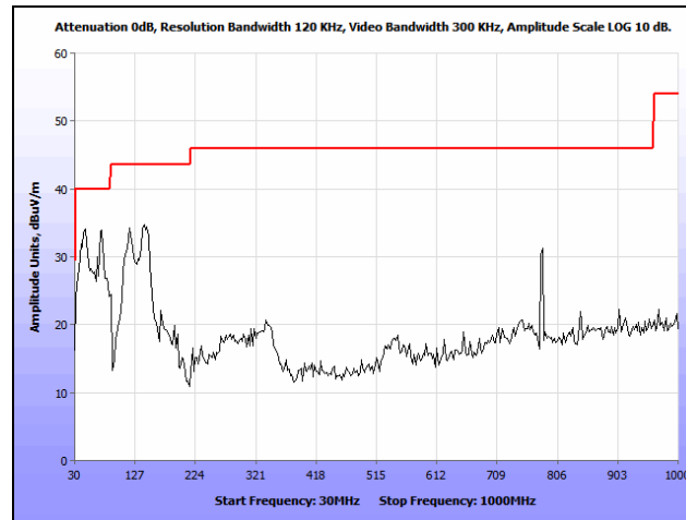
Plot 311. Radiated Spurious Emissions, 802.11n 80 MHz, 30 MHz – 1 GHz, Omni, 5290 MHz
