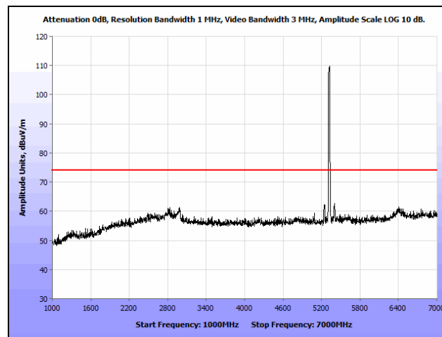
Plot 301. Radiated Spurious Emissions, 802.11n 20 MHz, High Channel, 1 GHz – 7 GHz, Peak, Omni, 5320 MHz
