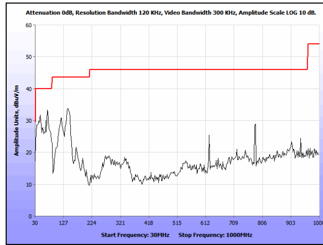
Plot 239. Radiated Spurious Emissions, 802.11n 80 MHz, 30 MHz – 1 GHz, Patch, 5290 MHz
