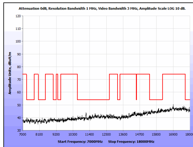
Plot 410. Radiated Spurious Emissions, 802.11a, Mid Channel, 7 GHz – 18 GHz, Omni, 5580 MHz
