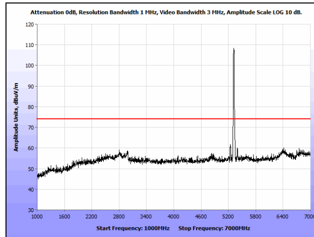
Plot 289. Radiated Spurious Emissions, 802.11a, High Channel, 1 GHz – 7 GHz, Peak, Omni, 5320 MHz
