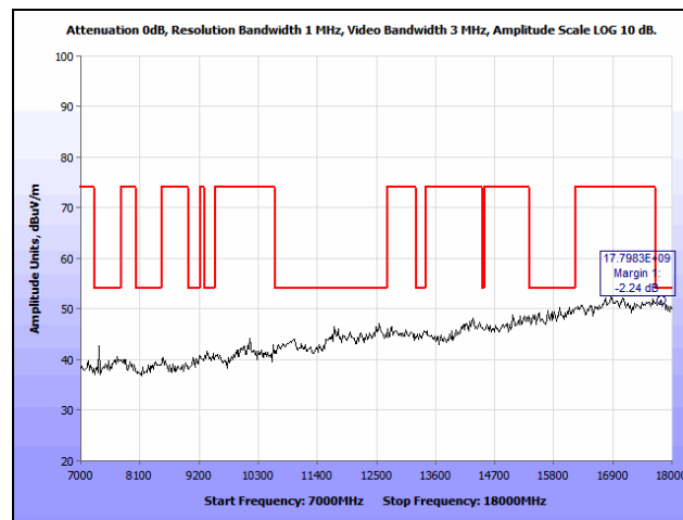
Plot 334. Radiated Spurious Emissions, 802.11n 20 MHz, Mid Channel, 7 GHz – 18 GHz, Patch, 5580 MHz
