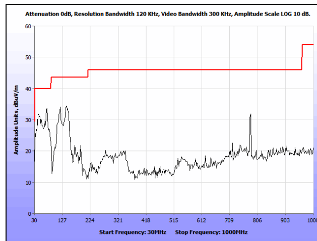
Plot 307. Radiated Spurious Emissions, 802.11n 40 MHz, High Channel, 30 MHz – 1 GHz, Omni, 5310 MHz
