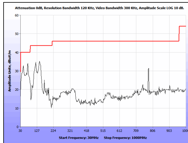
Plot 303. Radiated Spurious Emissions, 802.11n 40 MHz, Low Channel, 30 MHz – 1 GHz, Omni, 5270 MHz
