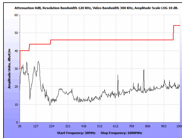
Plot 319. Radiated Spurious Emissions, 802.11a, Mid Channel, 30 MHz – 1 GHz, Patch, 5580 MHz
