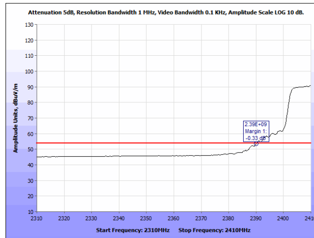
Plot 205. Radiated Restricted Band Edge, 802.11n 20 MHz, 2412 MHz @ 2390 MHz, Average
