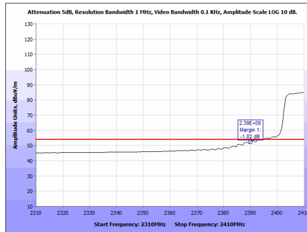
Plot 209. Radiated Restricted Band Edge, 802.11n 40 MHz, 2412 MHz @ 2390 MHz, Average
