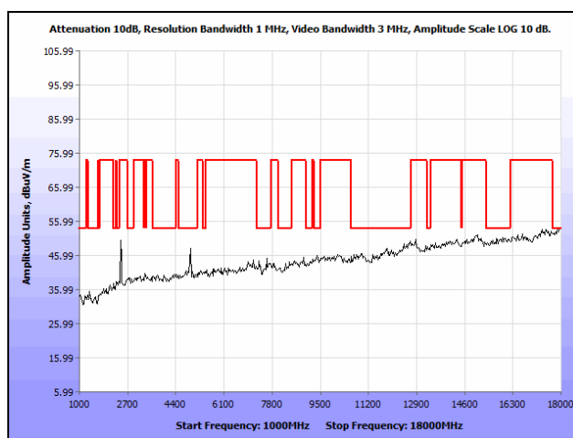
Plot 156. Radiated Spurious Emissions, High Channel, 802.11n 40 MHz, 1 GHz – 18 GHz, Omni-Directional Antenna, Average
