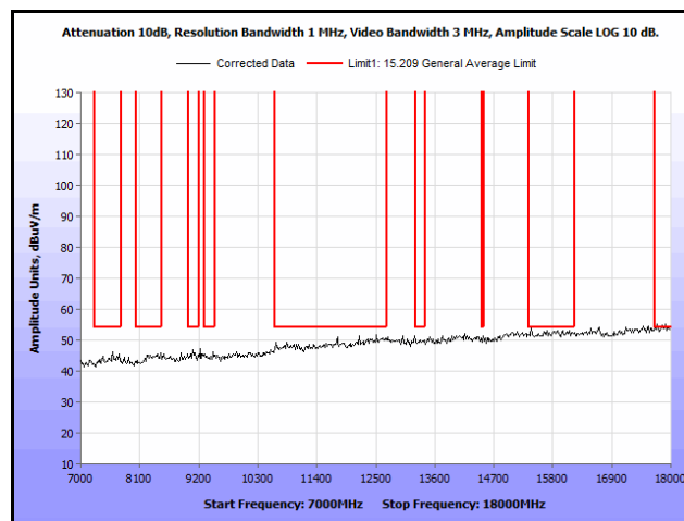
Plot 326. Radiated Spurs, Co-Location, 802.11n 20 MHz, 2412 MHz & 5300 MHz, 7 GHz – 18 GHz, Peak, Omni
