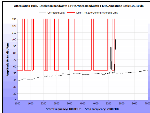
Plot 388. Radiated Spurs, Co-Location, 802.11n 20 MHz, 5300 MHz & 5580 MHz, 1 GHz – 7 GHz, Avg., Omni
