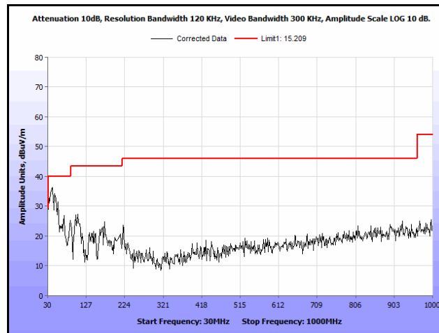
Plot 355. Radiated Spurs, Co-Location, 802.11n 20 MHz, 2462 MHz & 5300 MHz, 30 MHz – 1 GHz, Peak, Omni
