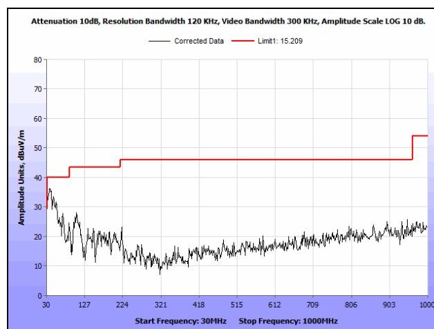
Plot 129. Radiated Spurious Emissions, Mid Channel, 802.11n 40 MHz, 30 MHz – 1 GHz, Omni Antenna, Average
