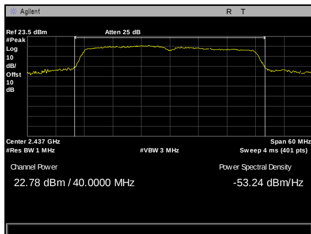
Plot 83. Peak Power Output, Mid Channel, 2437 MHz, 802.11n 40 MHz, Port 2
