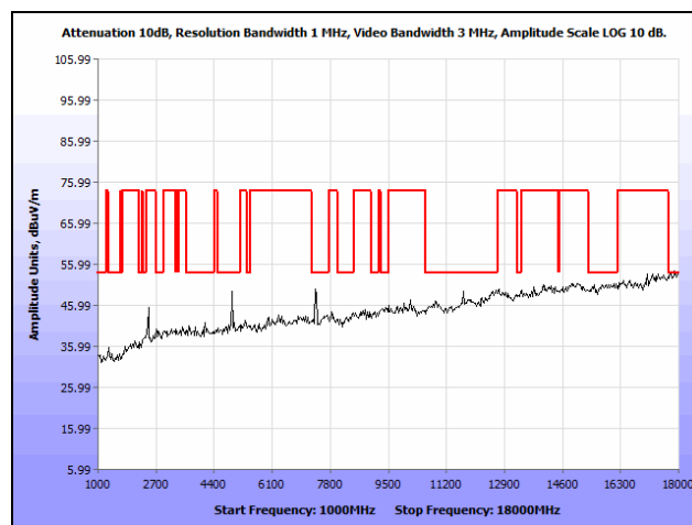
Plot 102. Radiated Spurious Emissions, High Channel, 802.11n 20 MHz, 1 GHz – 18 GHz, Ceiling Antenna, Average
