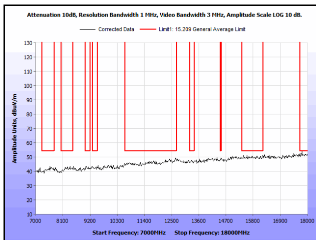
Plot 406. Radiated Spurs, Co-Location, 802.11n 20 MHz, 5785 MHz & 5785 MHz, 7 GHz – 18 GHz, Peak, Omni
