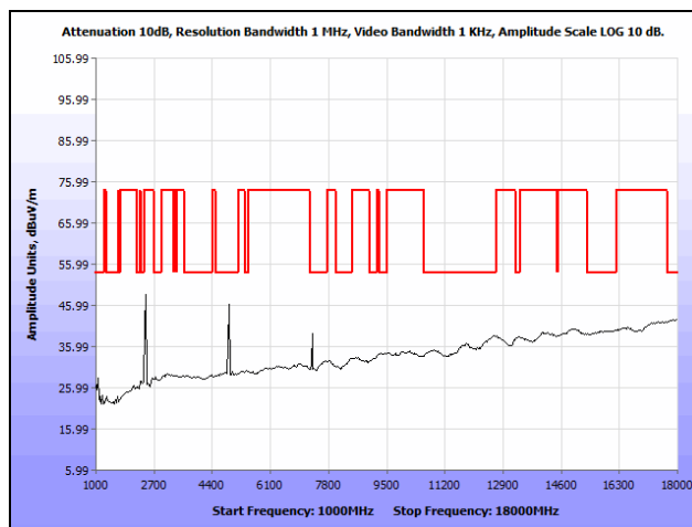
Plot 136. Radiated Spurious Emissions, Mid Channel, 802.11b, 1 GHz – 18 GHz, Omni-Directional Antenna, Average
