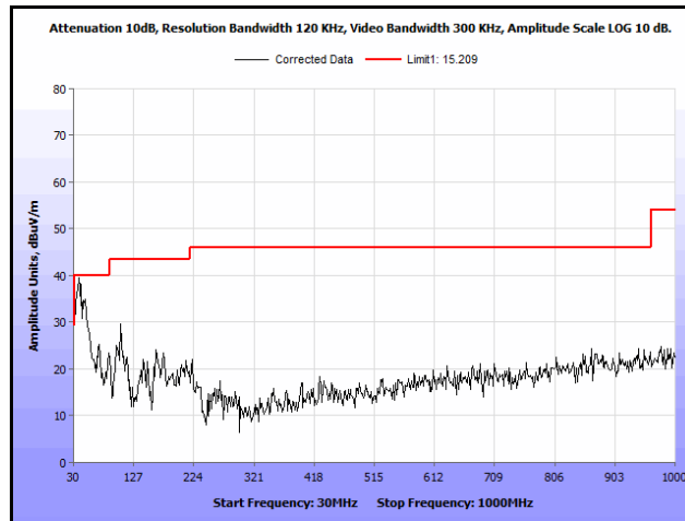
Plot 391. Radiated Spurs, Co-Location, 802.11n 20 MHz, 5300 MHz & 5785 MHz, 30 MHz – 1 GHz, Peak, Omni
