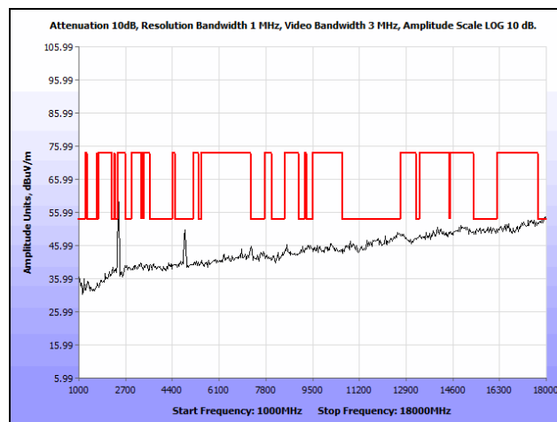
Plot 176. Radiated Spurious Emissions, Low Channel, 802.11n 40 MHz, 1 GHz – 18 GHz, Patch Antenna, Average
