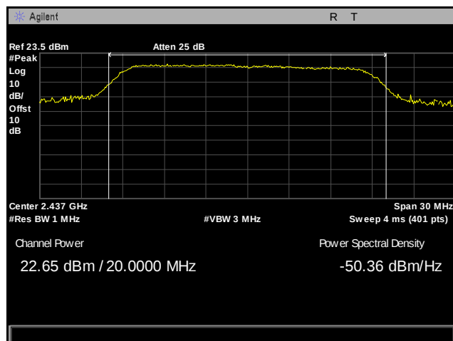
Plot 77. Peak Power Output, Mid Channel, 2437 MHz, 802.11n 20 MHz, Port 2
