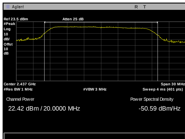
Plot 74. Peak Power Output, Mid Channel, 2437 MHz, 802.11n 20 MHz, Port 1
