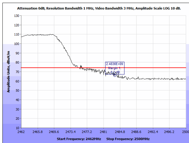
Plot 204. Radiated Restricted Band Edge, 802.11g, 2462 MHz @ 2483.5 MHz, Peak
