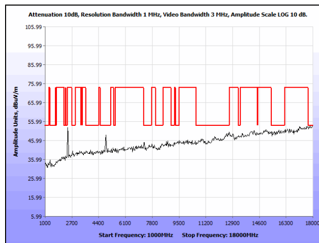
Plot 152. Radiated Spurious Emissions, Low Channel, 802.11n 40 MHz, 1 GHz – 18 GHz, Omni-Directional Antenna, Average
