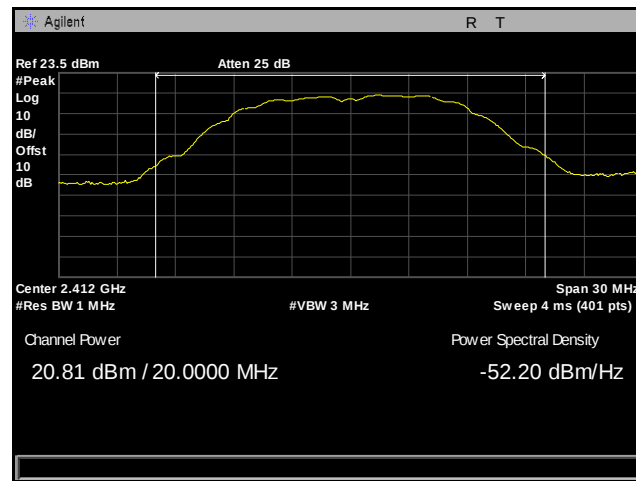
Plot 67. Peak Power Output, Low Channel, 2412 MHz, 802.11b
