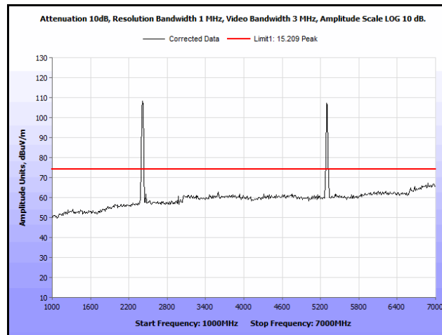
Plot 325. Radiated Spurs, Co-Location, 802.11n 20 MHz, 2412 MHz & 5300 MHz, 1 GHz – 7 GHz, Peak, Omni
