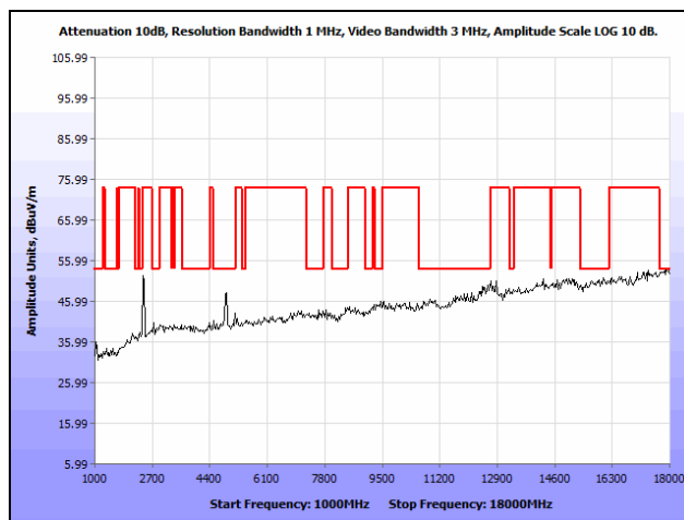
Plot 154. Radiated Spurious Emissions, Mid Channel, 802.11n 40 MHz, 1 GHz – 18 GHz, Omni-Directional Antenna, Average
