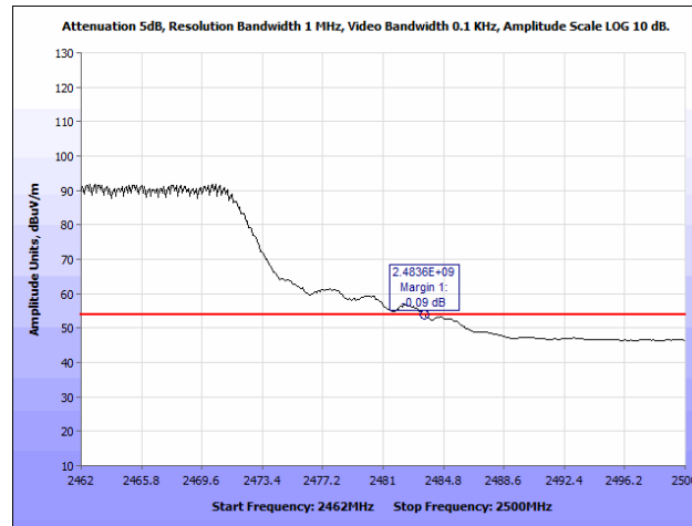
Plot 223. Radiated Restricted Band Edge, 802.11n 20 MHz, 2462 MHz @ 2483.5 MHz, Average
