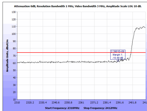
Plot 206. Radiated Restricted Band Edge, 802.11n 20 MHz, 2412 MHz @ 2390 MHz, Peak
