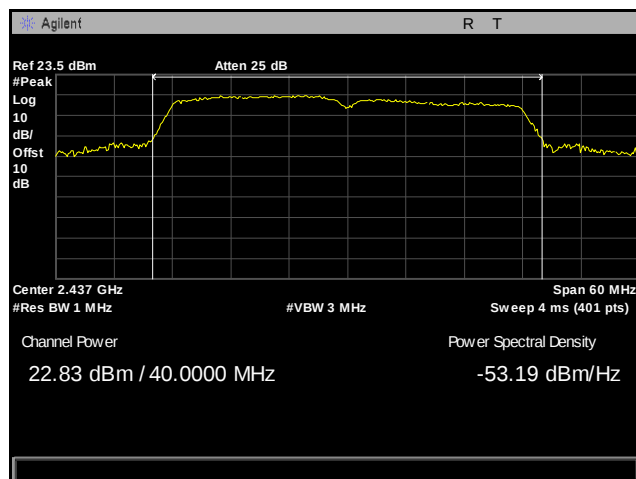
Plot 80. Peak Power Output, Mid Channel, 2437 MHz, 802.11n 40 MHz, Port 1
