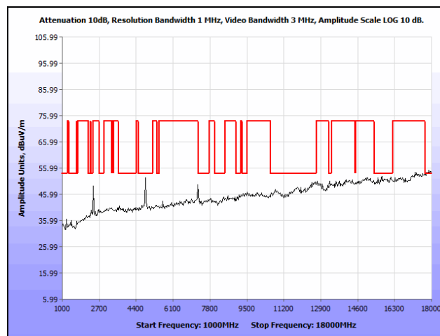
Plot 98. Radiated Spurious Emissions, Low Channel, 802.11n 20 MHz, 1 GHz – 18 GHz, Ceiling Antenna, Average
