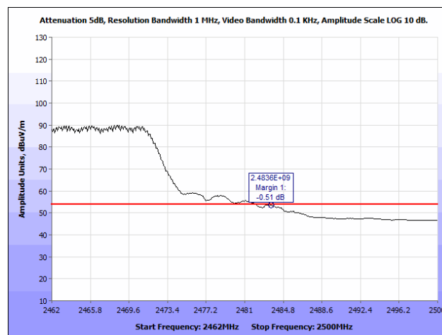
Plot 207. Radiated Restricted Band Edge, 802.11n 20 MHz, 2462 MHz @ 2483.5 MHz, Average
