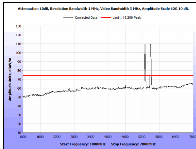
Plot 389. Radiated Spurs, Co-Location, 802.11n 20 MHz, 5300 MHz & 5580 MHz, 1 GHz – 7 GHz, Peak, Omni
