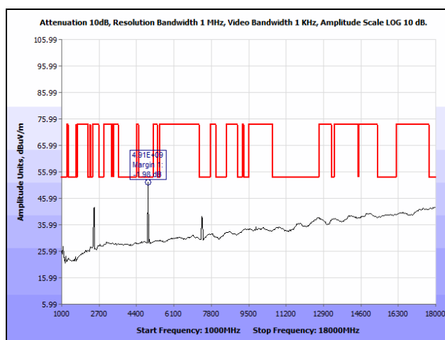
Plot 138. Radiated Spurious Emissions, High Channel, 802.11b, 1 GHz – 18 GHz, Omni-Directional Antenna, Average
