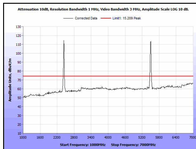
Plot 433. Radiated Spurs, Co-Location, 802.11n 20 MHz, 2437 MHz & 5580 MHz, 1 GHz – 7 GHz, Peak, Patch
