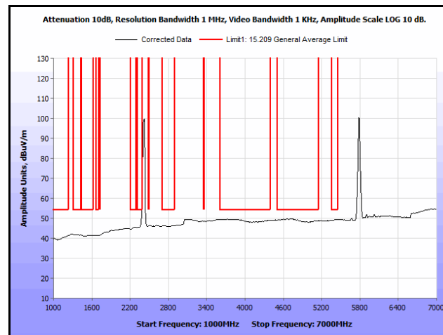
Plot 332. Radiated Spurs, Co-Location, 802.11n 20 MHz, 2412 MHz & 5785 MHz, 1 GHz – 7 GHz, Avg., Omni
