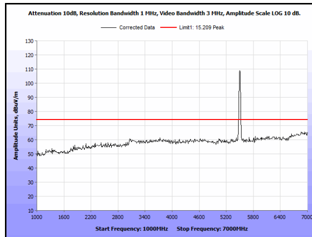
Plot 397. Radiated Spurs, Co-Location, 802.11n 20 MHz, 5580 MHz & 5580 MHz, 1 GHz – 7 GHz, Peak, Omni
