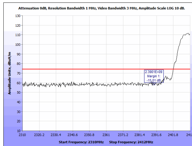
Plot 198. Radiated Restricted Band Edge, 802.11b, 2412 MHz @ 2390 MHz, Peak
