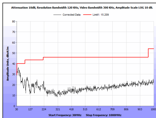
Plot 123. Radiated Spurious Emissions, Mid Channel, 802.11n 20 MHz, 30 MHz – 1 GHz, Omni Antenna, Average
