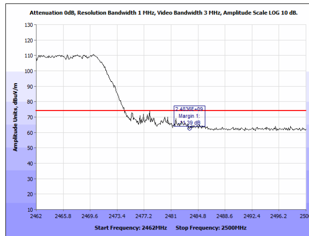
Plot 208. Radiated Restricted Band Edge, 802.11n 20 MHz, 2462 MHz @ 2483.5 MHz, Peak
