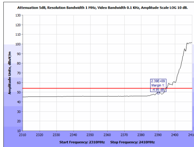
Plot 197. Radiated Restricted Band Edge, 802.11b, 2412 MHz @ 2390 MHz, Average
