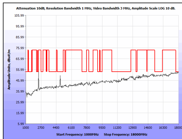
Plot 146. Radiated Spurious Emissions, Low Channel, 802.11n 20 MHz, 1 GHz – 18 GHz, Omni-Directional Antenna, Average
