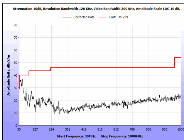
Plot 155. Radiated Spurious Emissions, High Channel, 802.11n 40 MHz, 30 MHz – 1 GHz, Omni-Directional Antenna, Average
