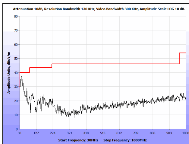
Plot 167. Radiated Spurious Emissions, High Channel, 802.11g, 30 MHz – 1 GHz, Patch Antenna, Average
