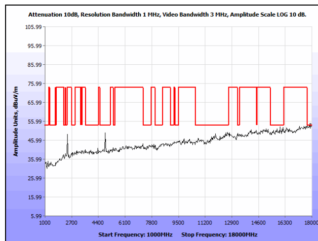
Plot 122. Radiated Spurious Emissions, Low Channel, 802.11n 20 MHz, 1 GHz – 18 GHz, Omni Antenna, Average
