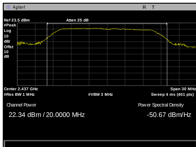
Plot 71. Peak Power Output, Mid Channel, 2437 MHz, 802.11g
