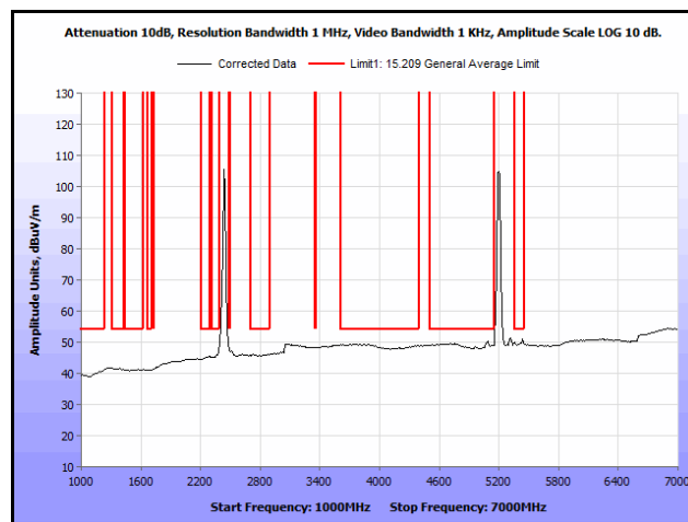
Plot 424. Radiated Spurs, Co-Location, 802.11n 20 MHz, 2437 MHz & 5200 MHz, 1 GHz – 7 GHz, Avg., Patch
