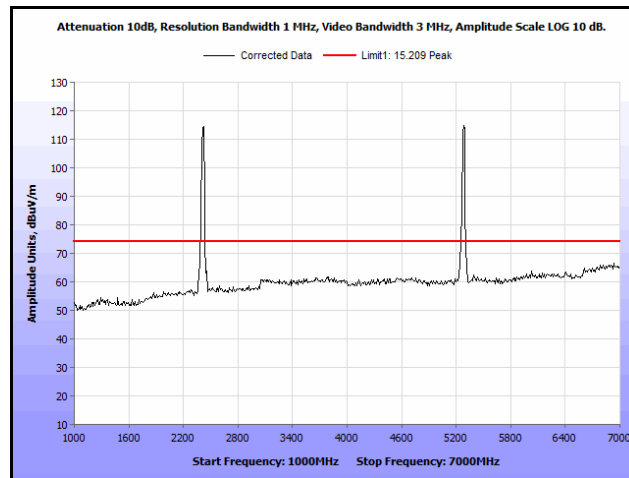
Plot 413. Radiated Spurs, Co-Location, 802.11n 20 MHz, 2412 MHz & 5300 MHz, 1 GHz – 7 GHz, Peak, Patch
