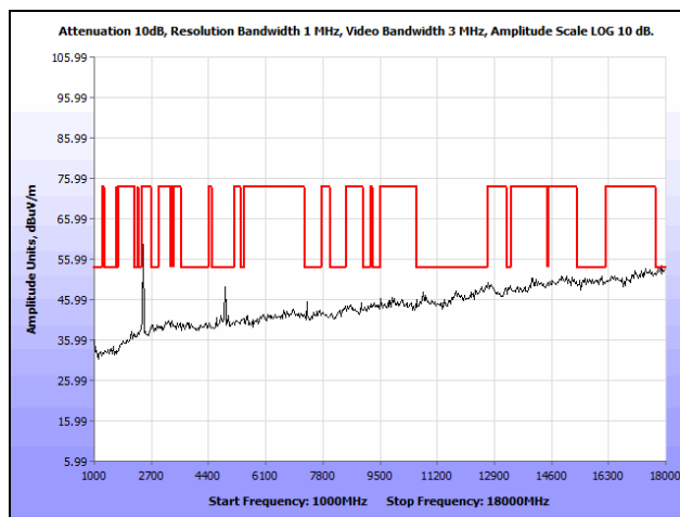
Plot 166. Radiated Spurious Emissions, Mid Channel, 802.11g, 1 GHz – 18 GHz, Patch Antenna, Average
