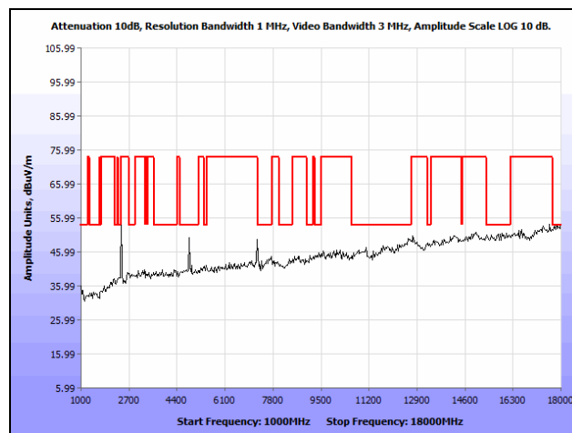
Plot 164. Radiated Spurious Emissions, Low Channel, 802.11g, 1 GHz – 18 GHz, Patch Antenna, Average
