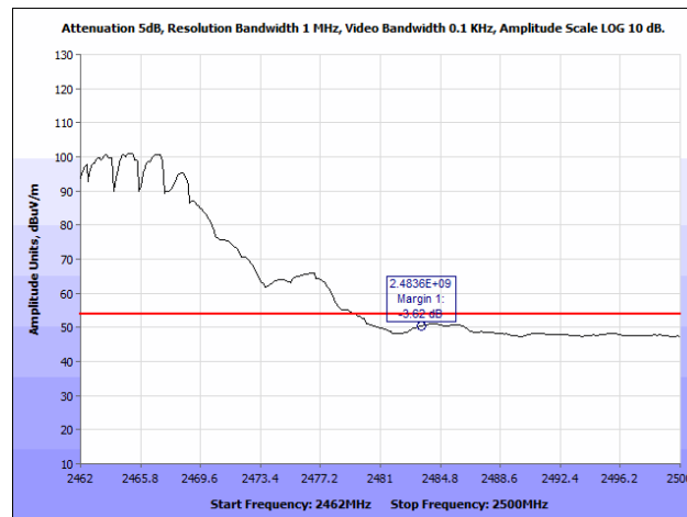
Plot 199. Radiated Restricted Band Edge, 802.11b, 2462 MHz @ 2483.5 MHz, Average
