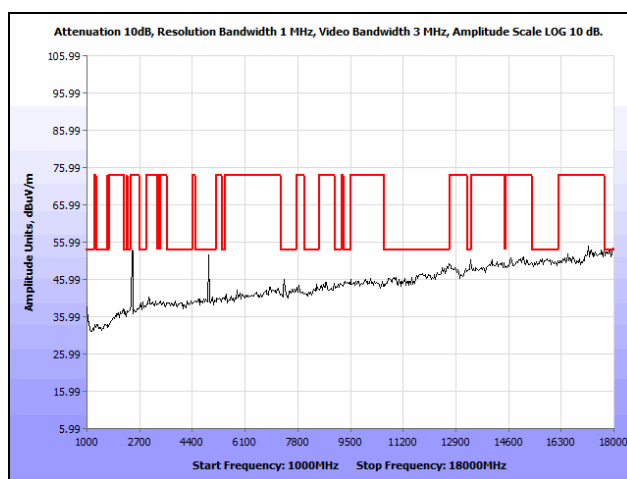
Plot 168. Radiated Spurious Emissions, High Channel, 802.11g, 1 GHz – 18 GHz, Patch Antenna, Average
