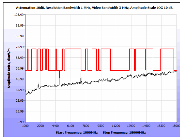
Plot 86. Radiated Spurious Emissions, Low Channel, 802.11b, 1 GHz – 18 GHz, Ceiling Antenna, Average
