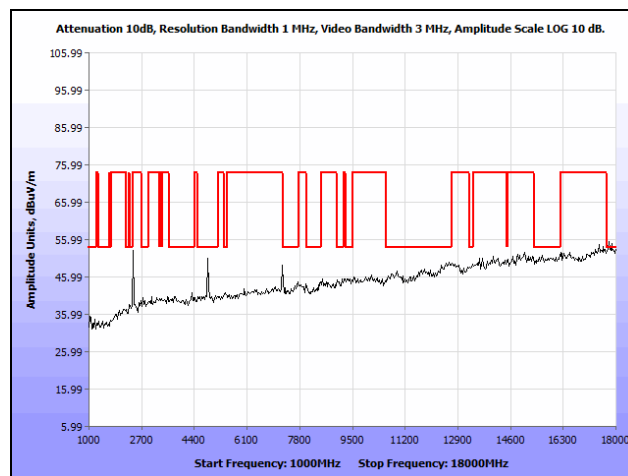
Plot 140. Radiated Spurious Emissions, Low Channel, 802.11g, 1 GHz – 18 GHz, Omni-Directional Antenna, Average
