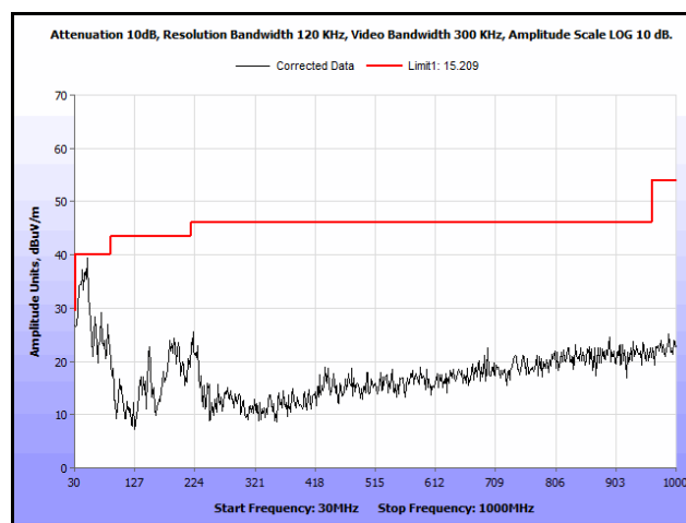
Plot 327. Radiated Spurs, Co-Location, 802.11n 20 MHz, 2412 MHz & 5580 MHz, 30 MHz – 1 GHz, Peak, Omni
