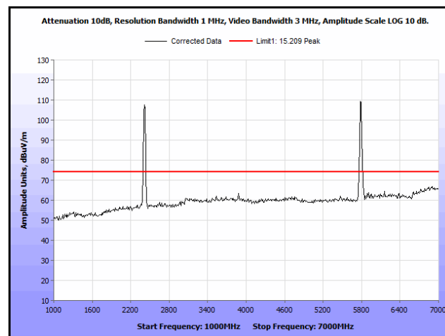
Plot 333. Radiated Spurs, Co-Location, 802.11n 20 MHz, 2412 MHz & 5785 MHz, 1 GHz – 7 GHz, Peak, Omni
