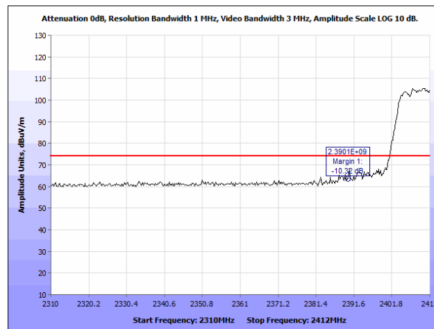
Plot 226. Radiated Restricted Band Edge, 802.11n 40 MHz, 2412 MHz @ 2390 MHz, Peak
