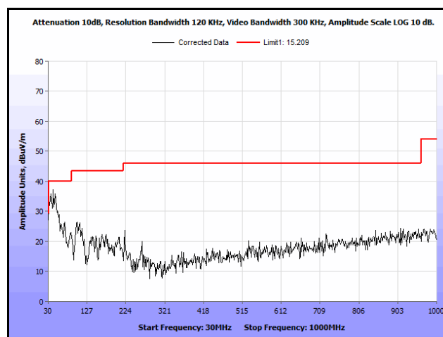
Plot 399. Radiated Spurs, Co-Location, 802.11n 20 MHz, 5580 MHz & 5785 MHz, 30 MHz – 1 GHz, Peak, Omni
