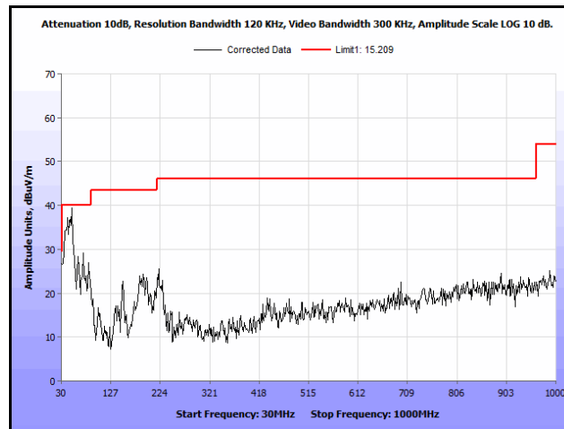
Plot 379. Radiated Spurs, Co-Location, 802.11n 20 MHz, 5200 MHz & 5785 MHz, 30 MHz – 1 GHz, Peak, Omni
