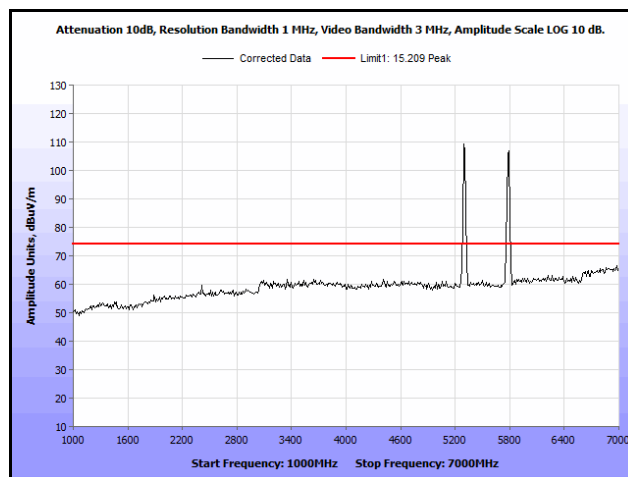
Plot 393. Radiated Spurs, Co-Location, 802.11n 20 MHz, 5300 MHz & 5785 MHz, 1 GHz – 7 GHz, Peak, Omni
