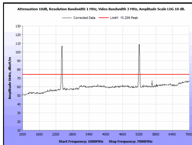
Plot 321. Radiated Spurs, Co-Location, 802.11n 20 MHz, 2412 MHz & 5200 MHz, 1 GHz – 7 GHz, Peak, Omni
