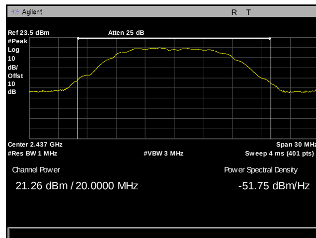
Plot 68. Peak Power Output, Mid Channel, 2437 MHz, 802.11b
