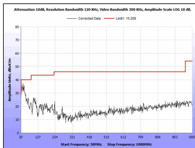
Plot 165. Radiated Spurious Emissions, Mid Channel, 802.11g, 30 MHz – 1 GHz, Patch Antenna, Average
