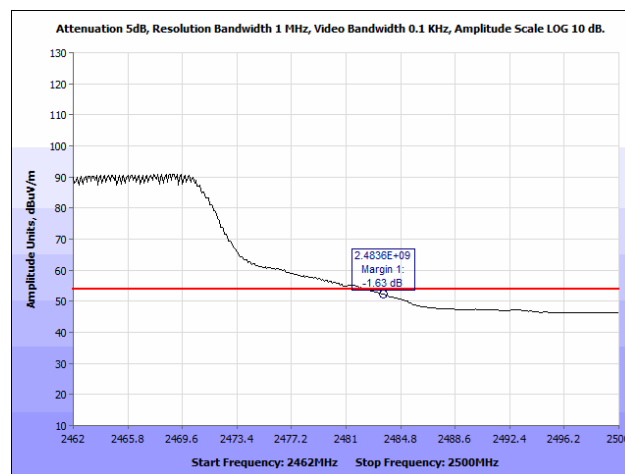
Plot 219. Radiated Restricted Band Edge, 802.11g, 2462 MHz @ 2483.5 MHz, Average
