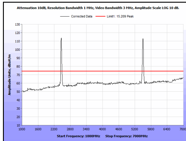
Plot 449. Radiated Spurs, Co-Location, 802.11n 20 MHz, 2462 MHz & 5580 MHz, 1 GHz – 7 GHz, Peak, Patch
