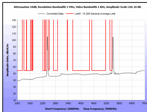
Plot 448. Radiated Spurs, Co-Location, 802.11n 20 MHz, 2462 MHz & 5580 MHz, 1 GHz – 7 GHz, Avg., Patch
