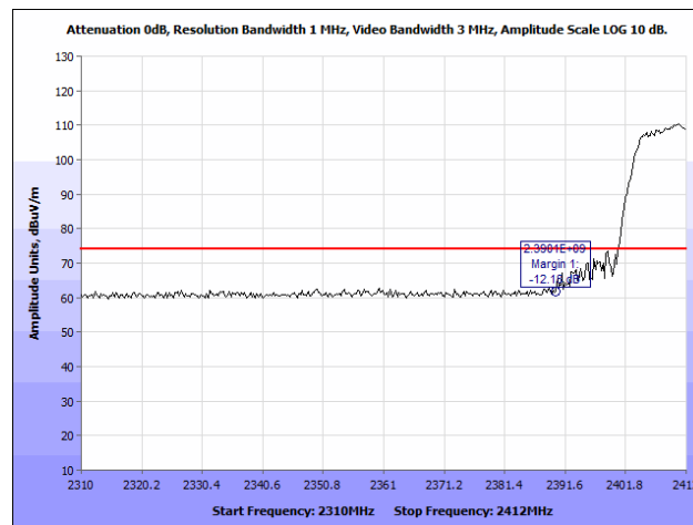
Plot 218. Radiated Restricted Band Edge, 802.11g, 2412 MHz @ 2390 MHz, Peak
