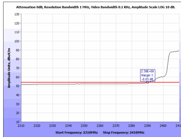
Plot 185. Radiated Restricted Band Edge, 802.11g, 2412 MHz @ 2390 MHz, Average
