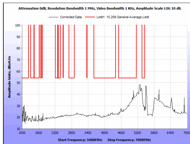
Plot 229. Radiated Spurious Emissions, 802.11n 40 MHz, High Channel, 1 GHz – 7 GHz, Average, Ceiling Antenna
