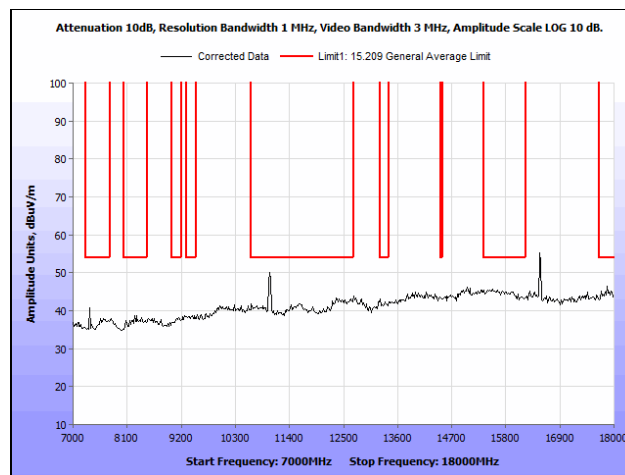
Plot 303. Radiated Spurious Emissions, 802.11n 20 MHz, Mid Channel, 7 GHz – 18 GHz, Patch Antenna
