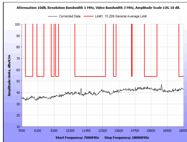
Plot 271. Radiated Spurious Emissions, 802.11n 40 MHz, High Channel, 7 GHz – 18 GHz, Peak, Omni Antenna
