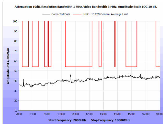
Plot 200. Radiated Spurious Emissions, 802.11a 40 MHz, Low Channel, 7 GHz – 18 GHz, Ceiling Antenna
