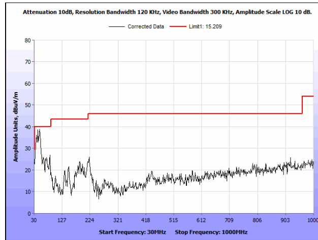
Plot 76. Radiated Spurious Emissions, 802.11a 20 MHz, High Channel, 30 MHz – 1 GHz, Ceiling Antenna
