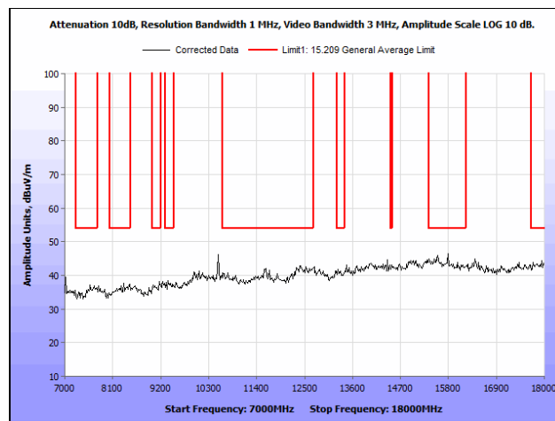
Plot 118. Radiated Spurious Emissions, 802.11a 20 MHz, Mid Channel, 7 GHz – 18 GHz, Omni Antenna
