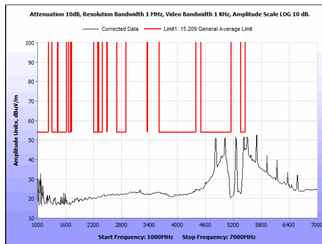
Plot 162. Radiated Spurious Emissions, 802.11a 20 MHz, High Channel, 1 GHz – 7 GHz, Average, Patch Antenna
