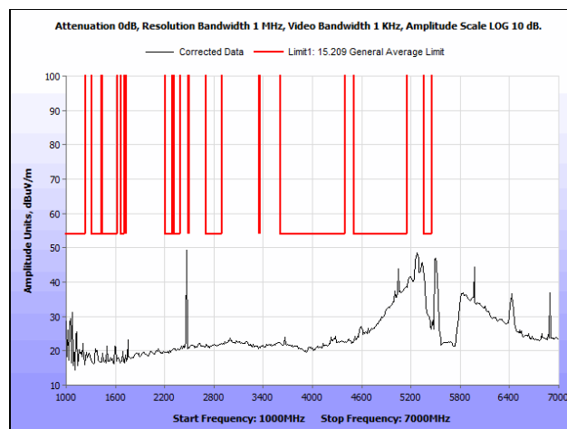
Plot 217. Radiated Spurious Emissions, 802.11n 40 MHz, Low Channel, 1 GHz – 7 GHz, Average, Ceiling Antenna
