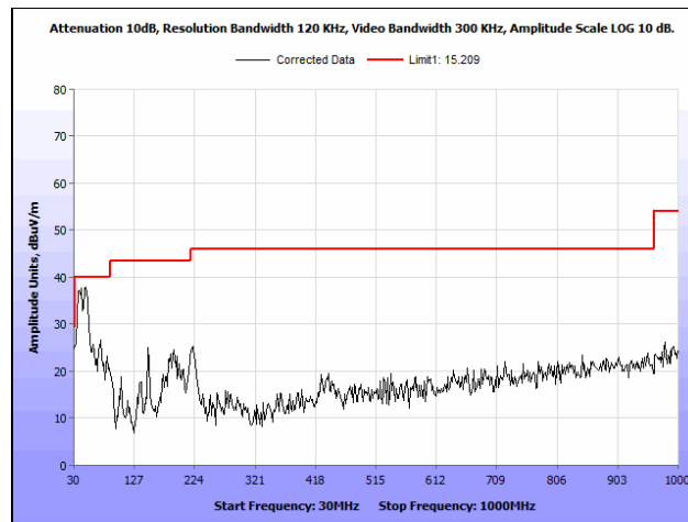
Plot 158. Radiated Spurious Emissions, 802.11a 20 MHz, Mid Channel, 30 MHz – 1 GHz, Patch Antenna
