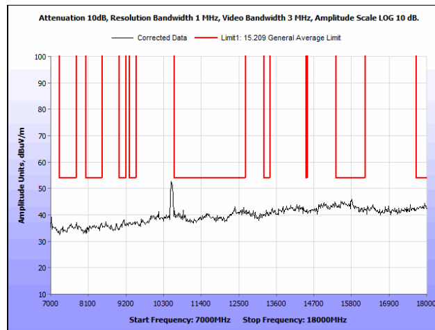
Plot 114. Radiated Spurious Emissions, 802.11a 40 MHz, Low Channel, 7 GHz – 18 GHz, Omni Antenna
