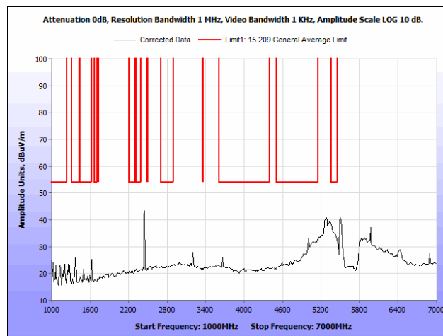
Plot 249. Radiated Spurious Emissions, 802.11a 40 MHz, High Channel, 1 GHz – 7 GHz, Average, Omni Antenna
