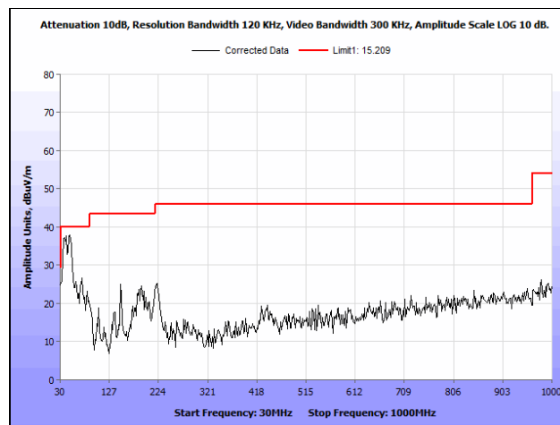
Plot 240. Radiated Spurious Emissions, 802.11a 20 MHz, Mid Channel, 30 MHz – 1 GHz, Omni Antenna
