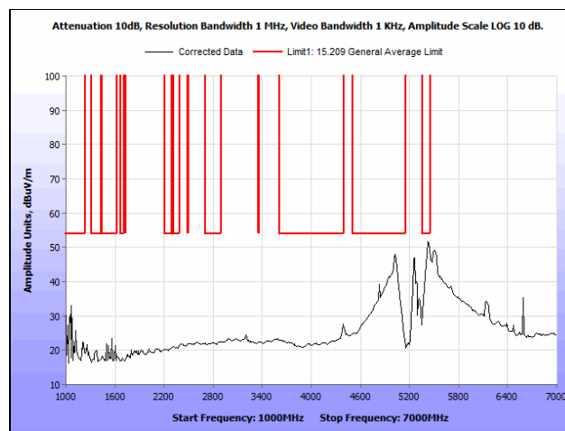
Plot 88. Radiated Spurious Emissions, 802.11n 40 MHz, Low Channel, 1 GHz – 7 GHz, Average, Ceiling Antenna
