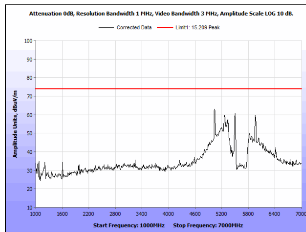
Plot 286. Radiated Spurious Emissions, 802.11a 20 MHz, High Channel, 1 GHz – 7 GHz, Peak, Patch Antenna
