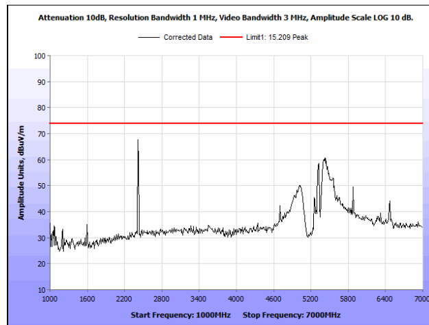
Plot 191. Radiated Spurious Emissions, 802.11ac 80 MHz, 1 GHz – 7 GHz, Peak, Patch Antenna
