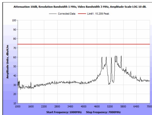
Plot 171. Radiated Spurious Emissions, 802.11n 20 MHz, Low Channel, 1 GHz – 7 GHz, Peak, Patch Antenna
