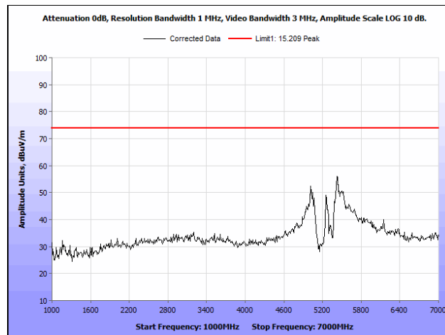
Plot 149. Radiated Spurious Emissions, 802.11ac 80 MHz, 1 GHz – 7 GHz, Peak, Omni Antenna
