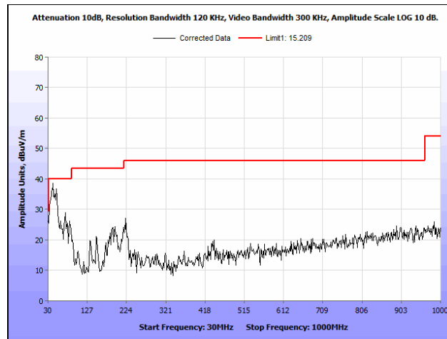
Plot 212. Radiated Spurious Emissions, 802.11n 20 MHz, Low Channel, 30 MHz – 1 GHz, Ceiling Antenna
