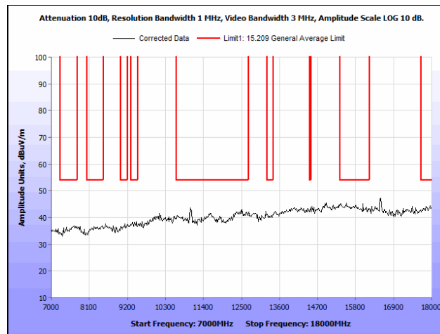
Plot 259. Radiated Spurious Emissions, 802.11n 40 MHz, Low Channel, 7 GHz – 18 GHz, Omni Antenna
