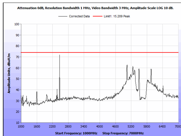
Plot 214. Radiated Spurious Emissions, 802.11n 20 MHz, Low Channel, 1 GHz – 7 GHz, Peak, Ceiling Antenna
