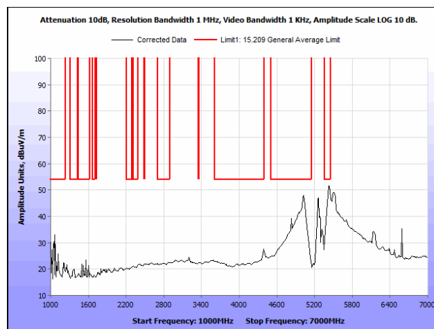
Plot 174. Radiated Spurious Emissions, 802.11n 40 MHz, Low Channel, 1 GHz – 7 GHz, Average, Patch Antenna
