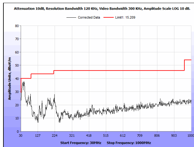
Plot 165. Radiated Spurious Emissions, 802.11a 40 MHz, High Channel, 30 MHz – 1 GHz, Patch Antenna
