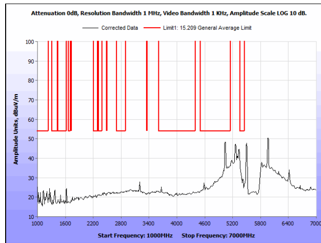
Plot 265. Radiated Spurious Emissions, 802.11n 20 MHz, High Channel, 1 GHz – 7 GHz, Average, Omni Antenna
