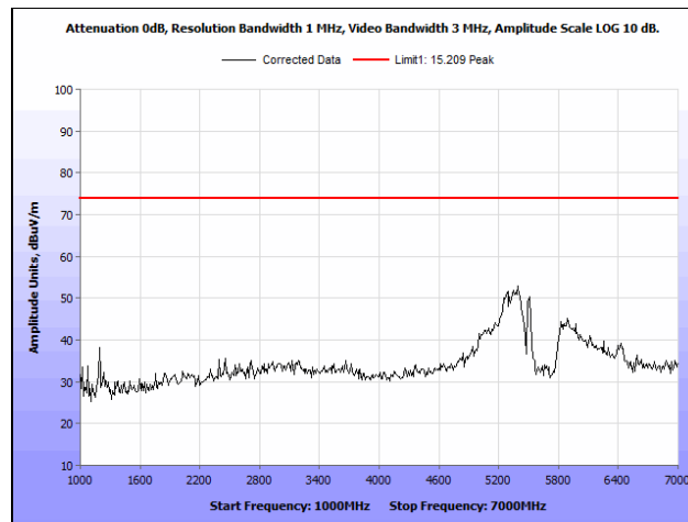
Plot 242. Radiated Spurious Emissions, 802.11a 20 MHz, Mid Channel, 1 GHz – 7 GHz, Peak, Omni Antenna
