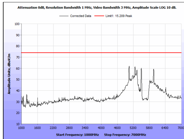
Plot 282. Radiated Spurious Emissions, 802.11a 20 MHz, Mid Channel, 1 GHz – 7 GHz, Peak, Patch Antenna
