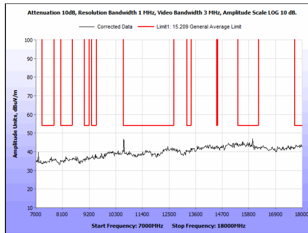
Plot 164. Radiated Spurious Emissions, 802.11a 20 MHz, High Channel, 7 GHz – 18 GHz, Patch Antenna
