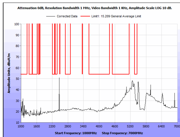
Plot 209. Radiated Spurious Emissions, 802.11a 40 MHz, High Channel, 1 GHz – 7 GHz, Average, Ceiling Antenna
