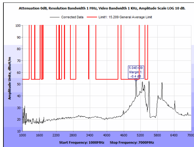
Plot 293. Radiated Spurious Emissions, 802.11n 20 MHz, Low Channel, 1 GHz – 7 GHz, Average, Patch Antenna
