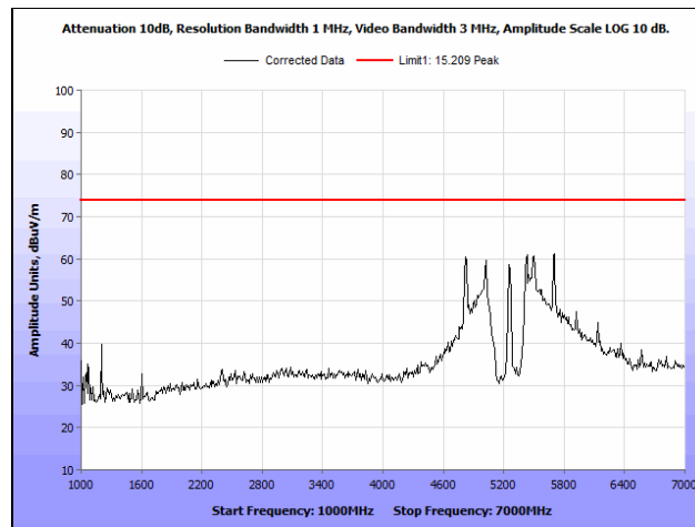
Plot 179. Radiated Spurious Emissions, 802.11n 20 MHz, Mid Channel, 1 GHz – 7 GHz, Peak, Patch Antenna
