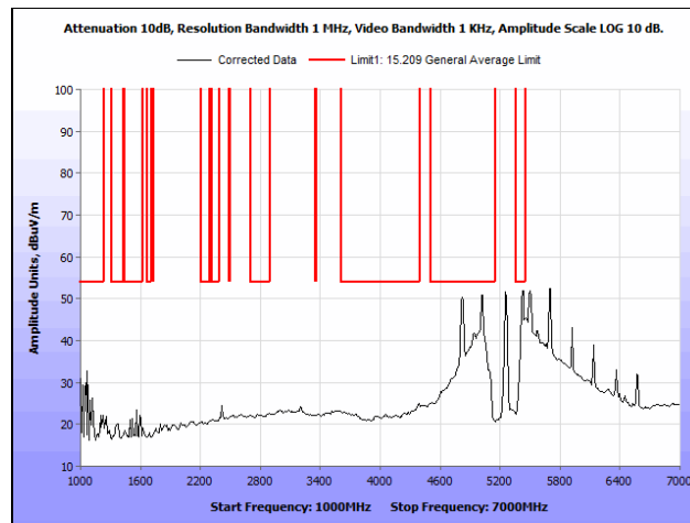
Plot 96. Radiated Spurious Emissions, 802.11n 20 MHz, High Channel, 1 GHz – 7 GHz, Average, Ceiling Antenna
