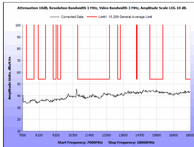
Plot 90. Radiated Spurious Emissions, 802.11n 40 MHz, Low Channel, 7 GHz – 18 GHz, Ceiling Antenna
