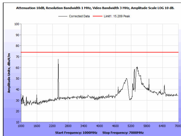
Plot 105. Radiated Spurious Emissions, 802.11ac 80 MHz, 1 GHz – 7 GHz, Peak, Ceiling Antenna
