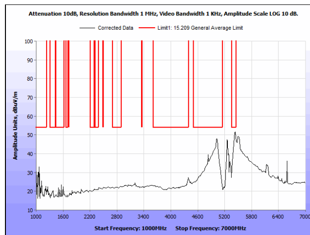
Plot 80. Radiated Spurious Emissions, 802.11a 40 MHz, High Channel, 1 GHz – 7 GHz, Average, Ceiling Antenna
