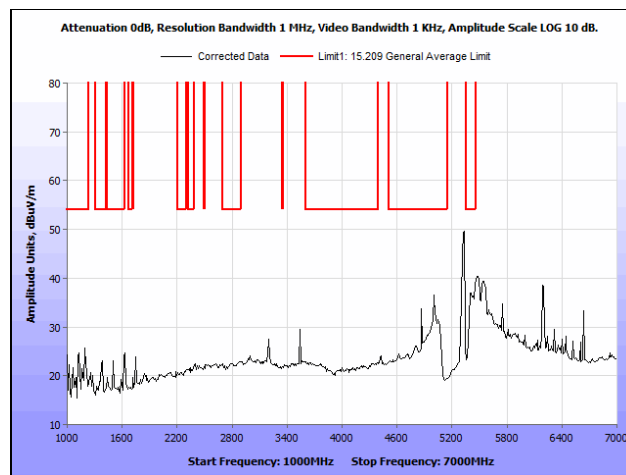
Plot 144. Radiated Spurious Emissions, 802.11n 40 MHz, High Channel, 1 GHz – 7 GHz, Average, Omni Antenna
