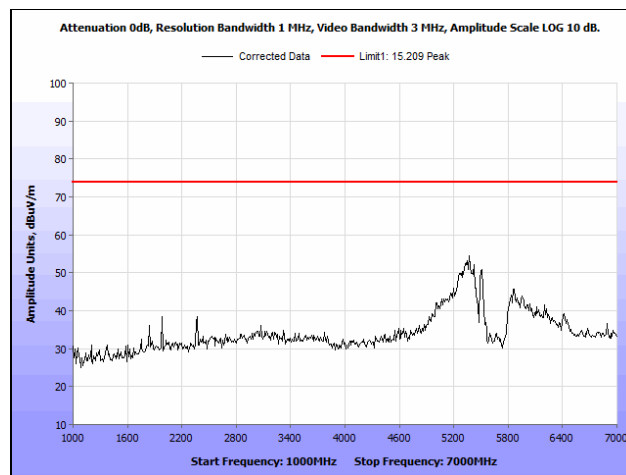
Plot 246. Radiated Spurious Emissions, 802.11a 20 MHz, High Channel, 1 GHz – 7 GHz, Peak, Omni Antenna
