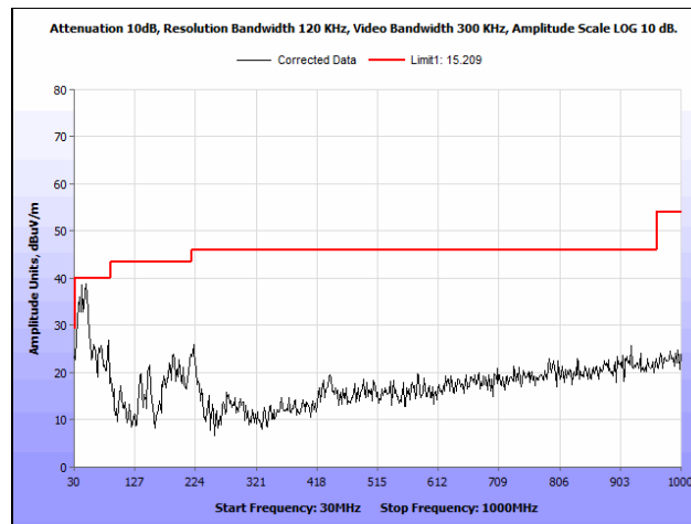
Plot 161. Radiated Spurious Emissions, 802.11a 20 MHz, High Channel, 30 MHz – 1 GHz, Patch Antenna
