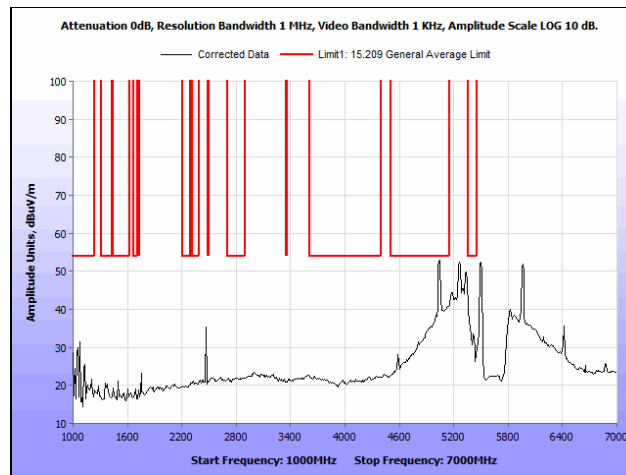
Plot 305. Radiated Spurious Emissions, 802.11n 20 MHz, High Channel, 1 GHz – 7 GHz, Average, Patch Antenna
