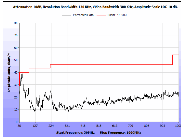
Plot 205. Radiated Spurious Emissions, 802.11a 20 MHz, High Channel, 30 MHz – 1 GHz, Ceiling Antenna
