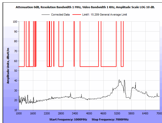
Plot 237. Radiated Spurious Emissions, 802.11a 40 MHz, Low Channel, 1 GHz – 7 GHz, Average, Omni Antenna
