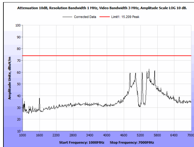
Plot 74. Radiated Spurious Emissions, 802.11a 20 MHz, Mid Channel, 1 GHz – 7 GHz, Peak, Ceiling Antenna
