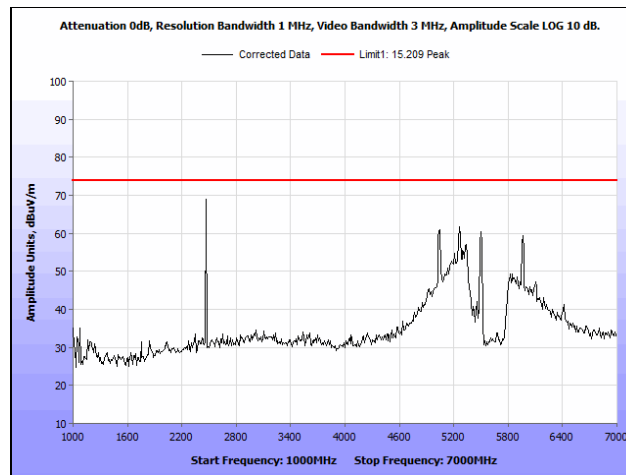
Plot 222. Radiated Spurious Emissions, 802.11n 20 MHz, Mid Channel, 1 GHz – 7 GHz, Peak, Ceiling Antenna
