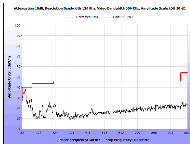
Plot 177. Radiated Spurious Emissions, 802.11n 20 MHz, Mid Channel, 30 MHz – 1 GHz, Patch Antenna
