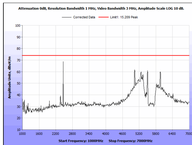
Plot 226. Radiated Spurious Emissions, 802.11n 20 MHz, High Channel, 1 GHz – 7 GHz, Peak, Ceiling Antenna
