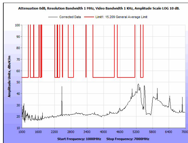
Plot 277. Radiated Spurious Emissions, 802.11a 40 MHz, Low Channel, 1 GHz – 7 GHz, Average, Patch Antenna
