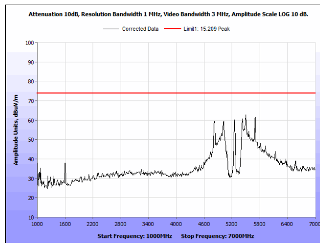
Plot 159. Radiated Spurious Emissions, 802.11a 20 MHz, Mid Channel, 1 GHz – 7 GHz, Peak, Patch Antenna
