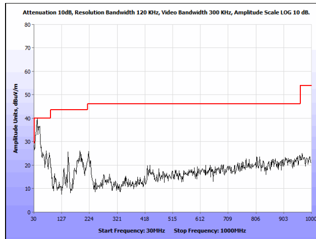
Plot 103. Radiated Spurious Emissions, 802.11ac 80 MHz, 30 MHz – 1 GHz, Ceiling Antenna
