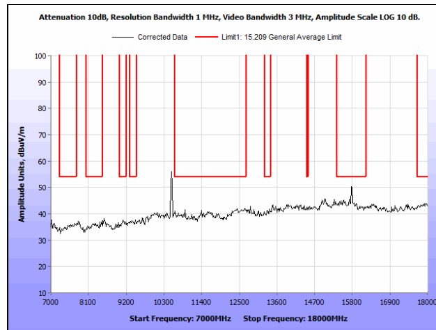
Plot 172. Radiated Spurious Emissions, 802.11n 20 MHz, Low Channel, 7 GHz – 18 GHz, Patch Antenna
