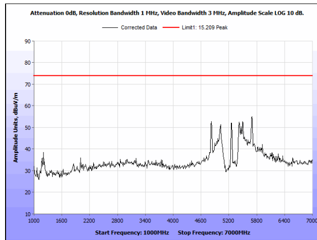
Plot 117. Radiated Spurious Emissions, 802.11a 20 MHz, Mid Channel, 1 GHz – 7 GHz, Peak, Omni Antenna
