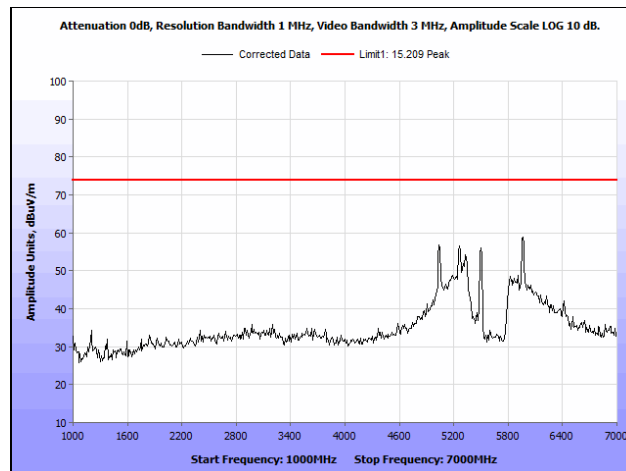
Plot 254. Radiated Spurious Emissions, 802.11n 20 MHz, Low Channel, 1 GHz – 7 GHz, Peak, Omni Antenna
