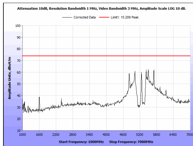
Plot 97. Radiated Spurious Emissions, 802.11n 20 MHz, High Channel, 1 GHz – 7 GHz, Peak, Ceiling Antenna
