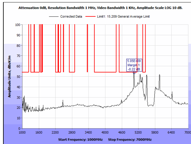
Plot 285. Radiated Spurious Emissions, 802.11a 20 MHz, High Channel, 1 GHz – 7 GHz, Average, Patch Antenna
