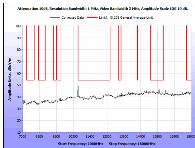
Plot 138. Radiated Spurious Emissions, 802.11n 20 MHz, Mid Channel, 7 GHz – 18 GHz, Omni Antenna
