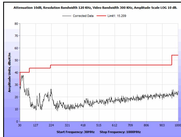
Plot 335. Radiated Spurs, Co-Location, 802.11n 20 MHz, 2412 MHz & 5785 MHz, 30 MHz – 1 GHz, Peak, Patch
