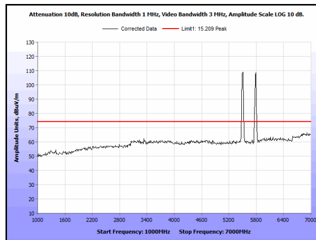
Plot 317. Radiated Spurs, Co-Location, 802.11n 20 MHz, 5580 MHz & 5785 MHz, 1 GHz – 7 GHz, Peak, Omni
