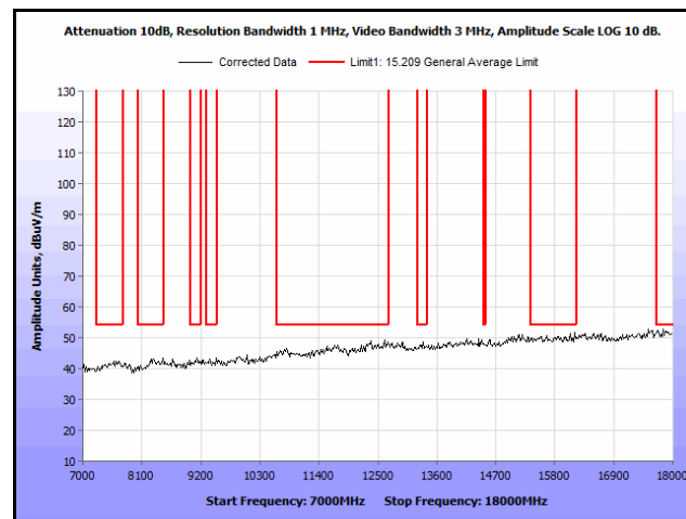
Plot 218. Radiated Spurs, Co-Location, 802.11n 20 MHz, 2412 MHz & 2437 MHz, 7 GHz – 18 GHz, Peak, Omni
