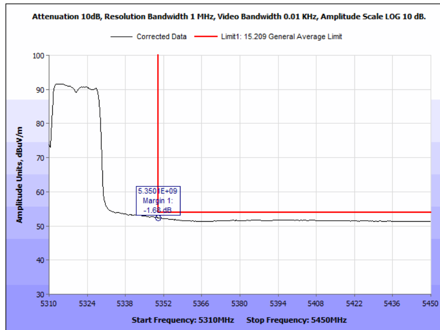
Plot 198. Radiated Band Edge, 802.11a, 40 MHz, High Channel, 7 dBi Antenna, Average
