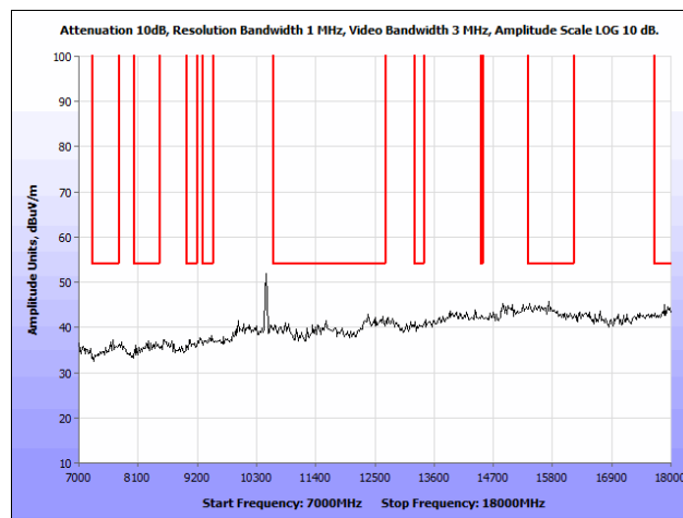
Plot 100. Radiated Spurious Emissions, 802.11n, 20 MHz, High Channel, 7 GHz – 18 GHz, Omni Antenna
