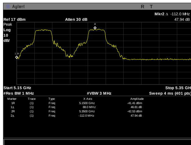
Plot 379. Frequency Stability, 5150 – 5350 MHz, 40°C, 120 V
