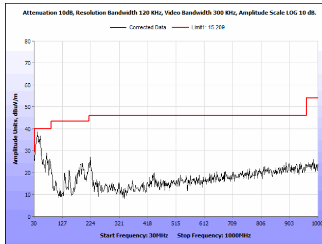
Plot 50. Radiated Spurious Emissions, 802.11n, 20 MHz, Low Channel, 30 MHz – 1 GHz, Ceiling Antenna
