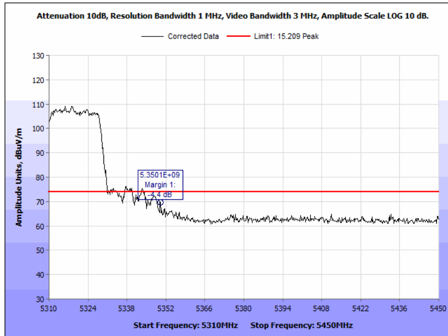
Plot 205. Radiated Band Edge, 802.11n, 40 MHz, High Channel, 7 dBi Antenna, Peak
