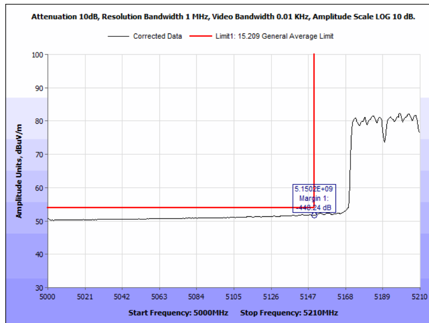
Plot 188. Radiated Band Edge, 802.11ac, 80 MHz, Low Channel, 4 dBi Antenna, Average
