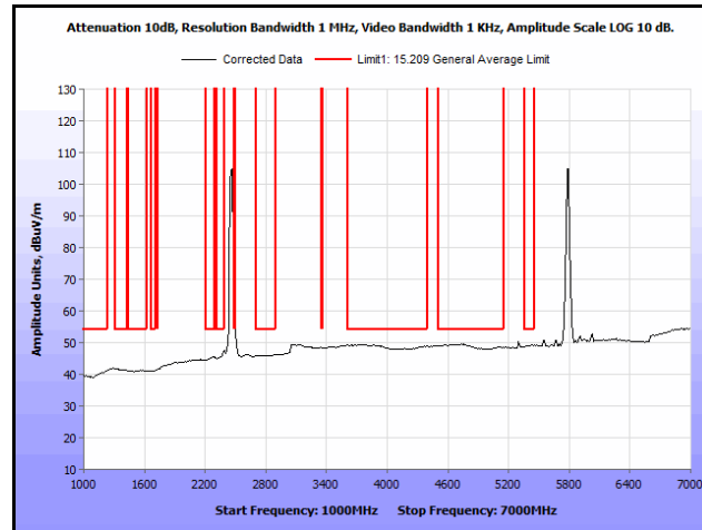
Plot 368. Radiated Spurs, Co-Location, 802.11n 20 MHz, 2462 MHz & 5785 MHz, 1 GHz – 7 GHz, Avg., Patch
