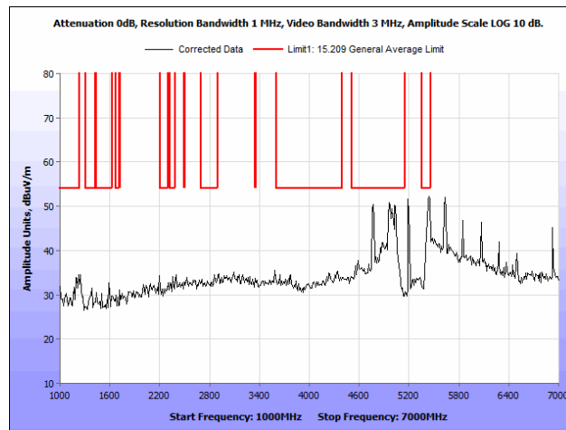
Plot 81. Radiated Spurious Emissions, 802.11a, 20 MHz, Mid Channel, 1 GHz – 7 GHz, Average, Omni Antenna
