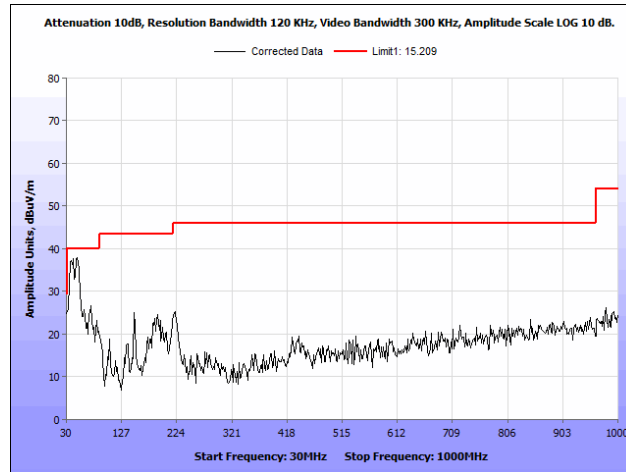
Plot 80. Radiated Spurious Emissions, 802.11a, 20 MHz, Mid Channel, 30 MHz – 1 GHz, Omni Antenna
