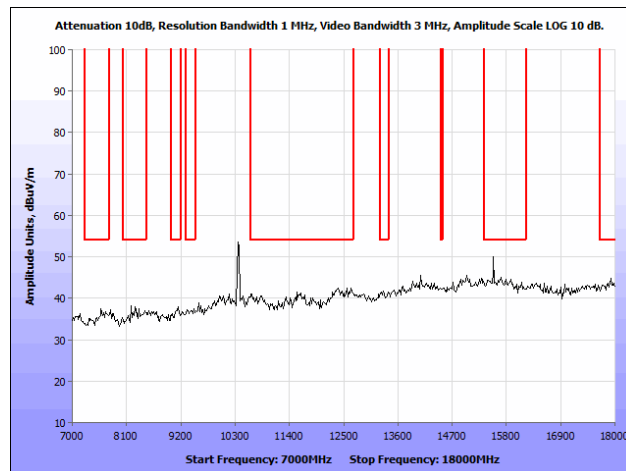
Plot 91. Radiated Spurious Emissions, 802.11n, 20 MHz, Low Channel, 7 GHz – 18 GHz, Omni Antenna
