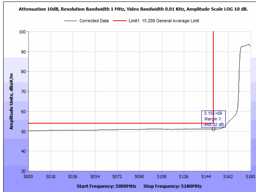
Plot 172. Radiated Band Edge, 802.11a, 20 MHz, Low Channel, 4 dBi Antenna, Average
