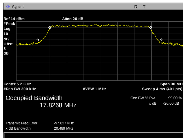
Plot 20. 26 dB Occupied Bandwidth, 802.11n, Port 1, 5200 MHz
