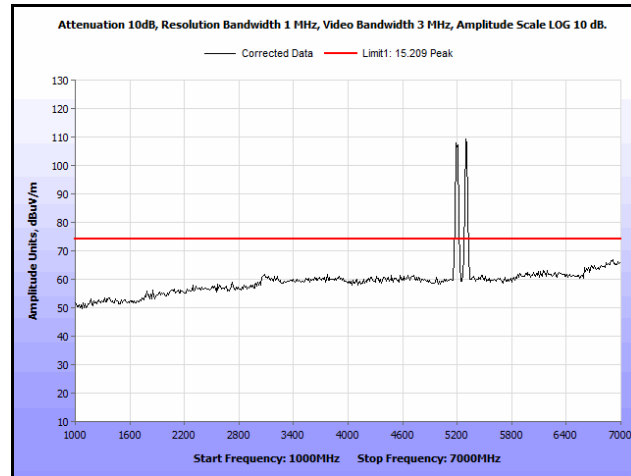
Plot 289. Radiated Spurs, Co-Location, 802.11n 20 MHz, 5200 MHz & 5300 MHz, 1 GHz – 7 GHz, Peak, Omni
