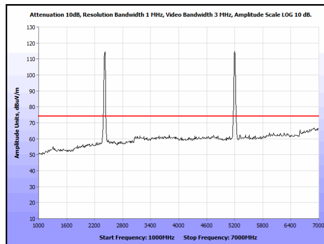
Plot 325. Radiated Spurs, Co-Location, 802.11n 20 MHz, 2412 MHz & 5200 MHz, 1 GHz – 7 GHz, Peak, Patch
