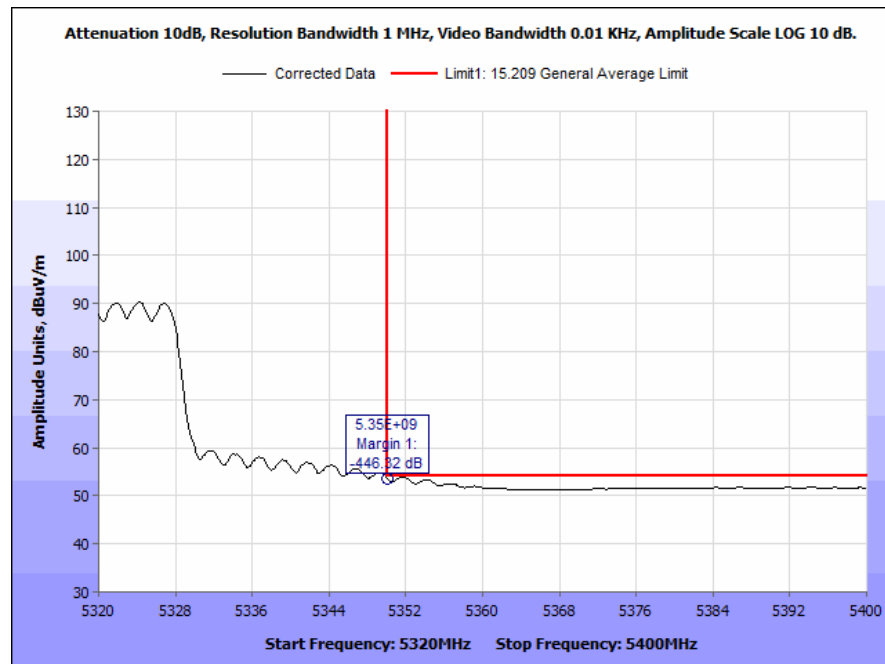
Plot 166. Radiated Band Edge, 802.11n, 40 MHz, High Channel, 6 dBi Omni Outdoor Antenna, Average
