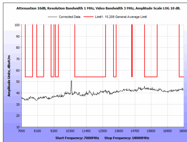
Plot 94. Radiated Spurious Emissions, 802.11n, 40 MHz, Low Channel, 7 GHz – 18 GHz, Omni Antenna
