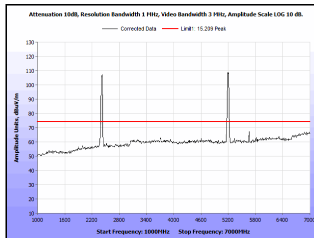
Plot 237. Radiated Spurs, Co-Location, 802.11n 20 MHz, 2412 MHz & 5200 MHz, 1 GHz – 7 GHz, Peak, Omni
