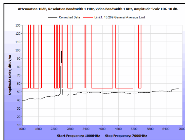
Plot 224. Radiated Spurs, Co-Location, 802.11n 20 MHz, 2437 MHz & 2437 MHz, 1 GHz – 7 GHz, Avg., Omni
