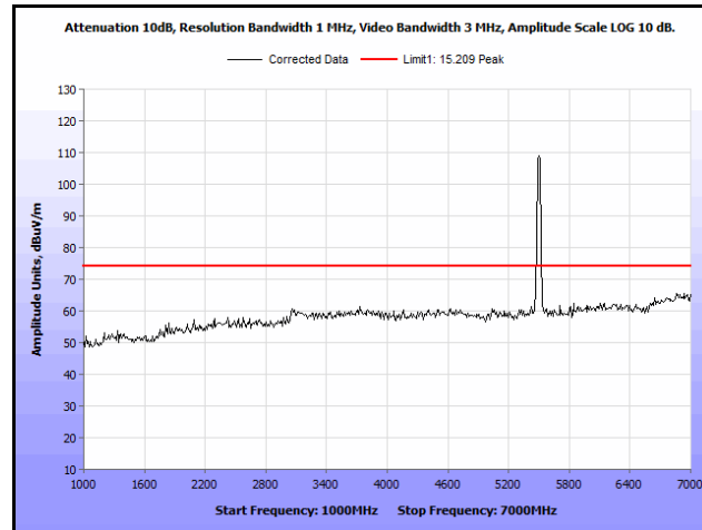
Plot 313. Radiated Spurs, Co-Location, 802.11n 20 MHz, 5580 MHz & 5580 MHz, 1 GHz – 7 GHz, Peak, Omni
