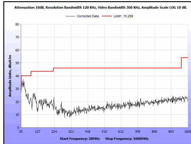
Plot 347. Radiated Spurs, Co-Location, 802.11n 20 MHz, 2437 MHz & 5580 MHz, 30 MHz – 1 GHz, Peak, Patch
