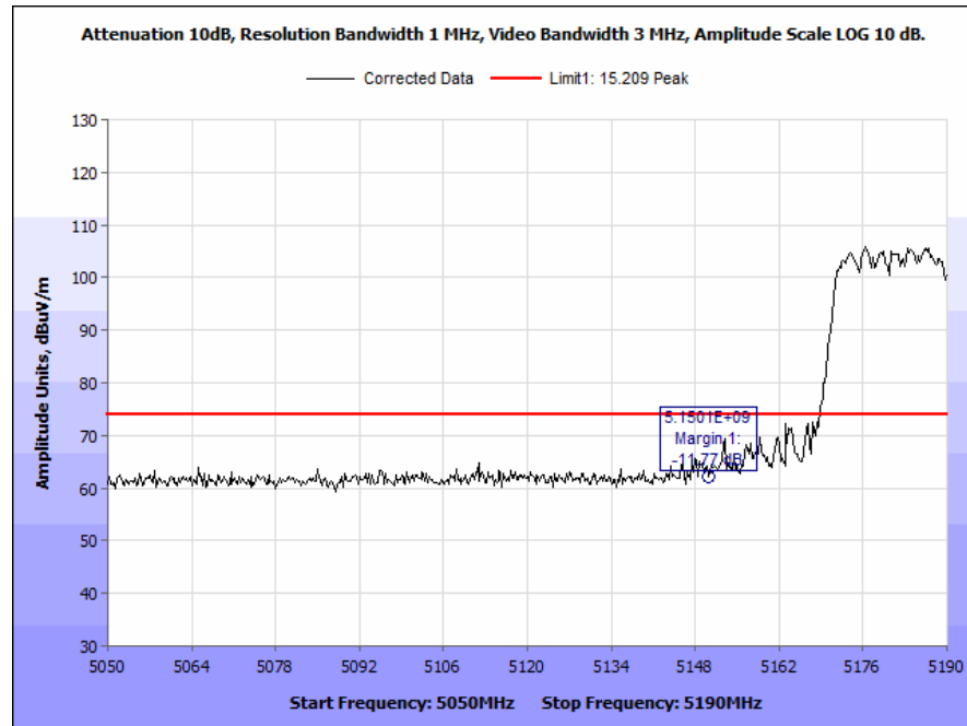
Plot 161. Radiated Band Edge, 802.11n, 40 MHz, Low Channel, 6 dBi Omni Outdoor Antenna, Peak
