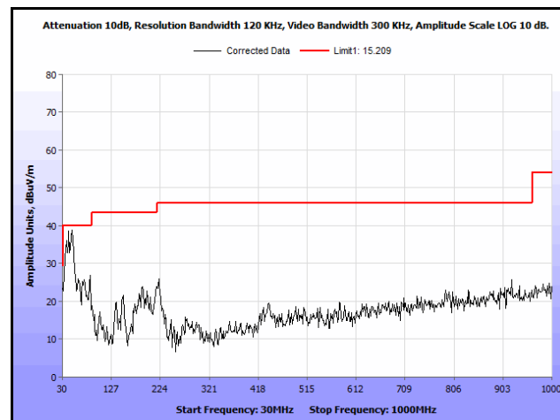
Plot 219. Radiated Spurs, Co-Location, 802.11n 20 MHz, 2412 MHz & 2462 MHz, 30 MHz – 1 GHz, Peak, Omni
