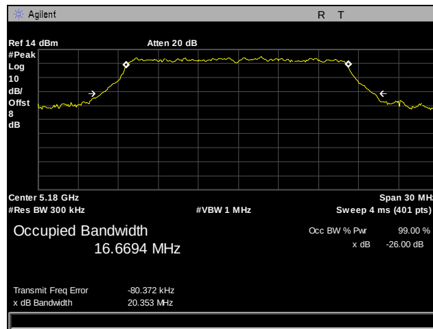
Plot 13. 26 dB Occupied Bandwidth, 802.11a, 5180 MHz
