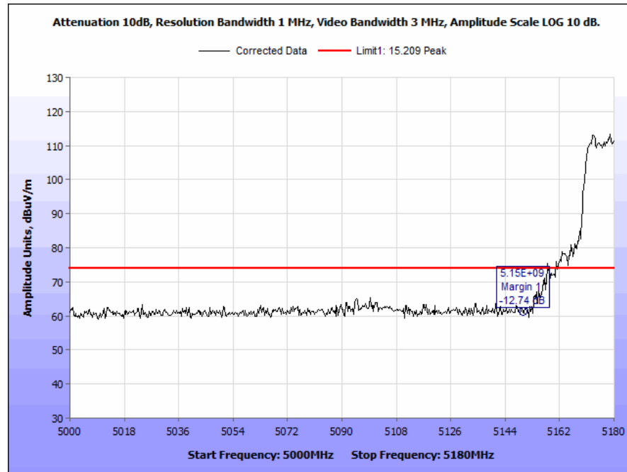
Plot 199. Radiated Band Edge, 802.11n, 20 MHz, Low Channel, 7 dBi Antenna, Peak
