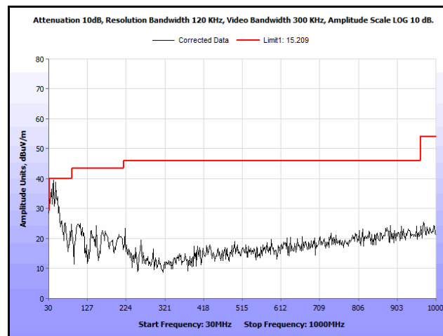
Plot 275. Radiated Spurs, Co-Location, 802.11n 20 MHz, 2462 MHz & 5580 MHz, 30 MHz – 1 GHz, Peak, Omni
