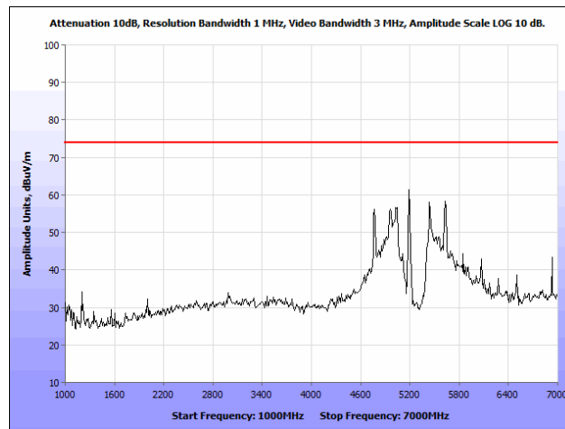
Plot 137. Radiated Spurious Emissions, 802.11n, 20 MHz, Mid Channel, 1 GHz – 7 GHz, Patch Antenna
