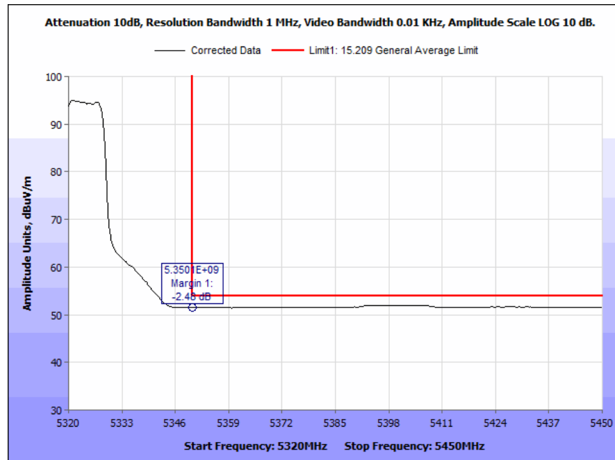
Plot 176. Radiated Band Edge, 802.11a, 20 MHz, High Channel, 4 dBi Antenna, Average
