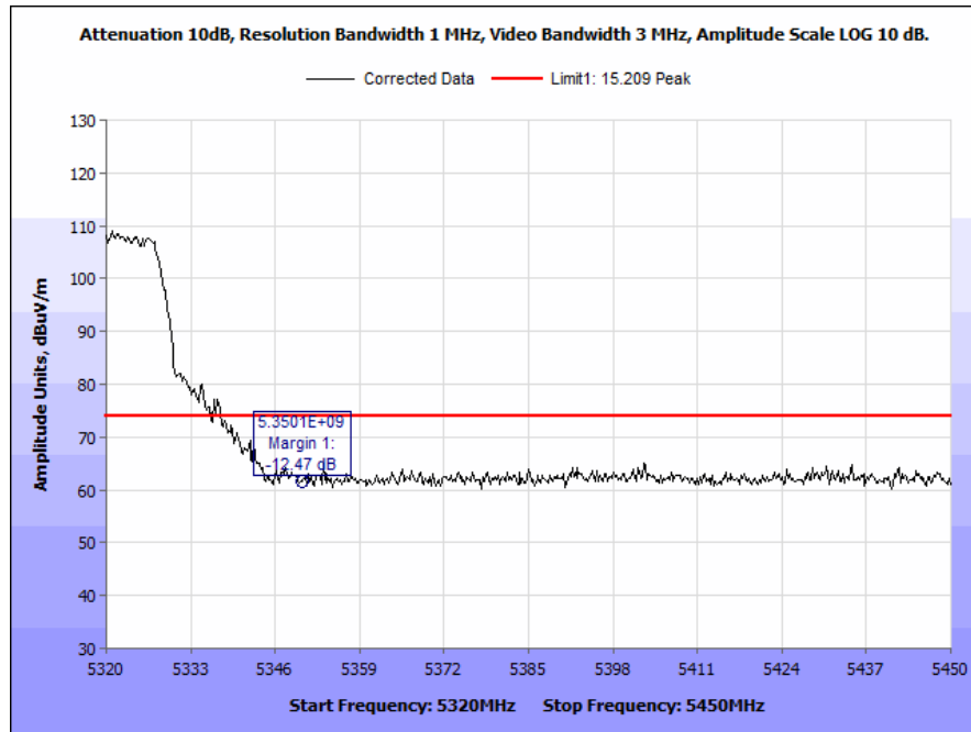
Plot 195. Radiated Band Edge, 802.11a, 20 MHz, High Channel, 7 dBi Antenna, Peak
