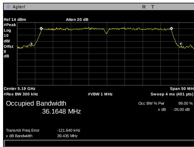
Plot 19. 26 dB Occupied Bandwidth, 802.11n, Port 1, 5190 MHz
