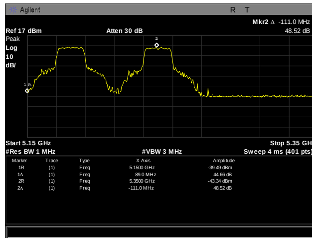
Plot 381. Frequency Stability, 5150 – 5350 MHz, 55°C, 120 V
