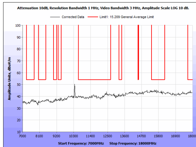
Plot 76. Radiated Spurious Emissions, 802.11a, 20 MHz, Low Channel, 7 GHz – 18 GHz, Omni Antenna
