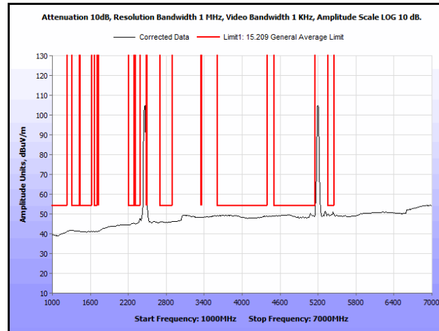
Plot 356. Radiated Spurs, Co-Location, 802.11n 20 MHz, 2462 MHz & 5200 MHz, 1 GHz – 7 GHz, Avg., Patch
