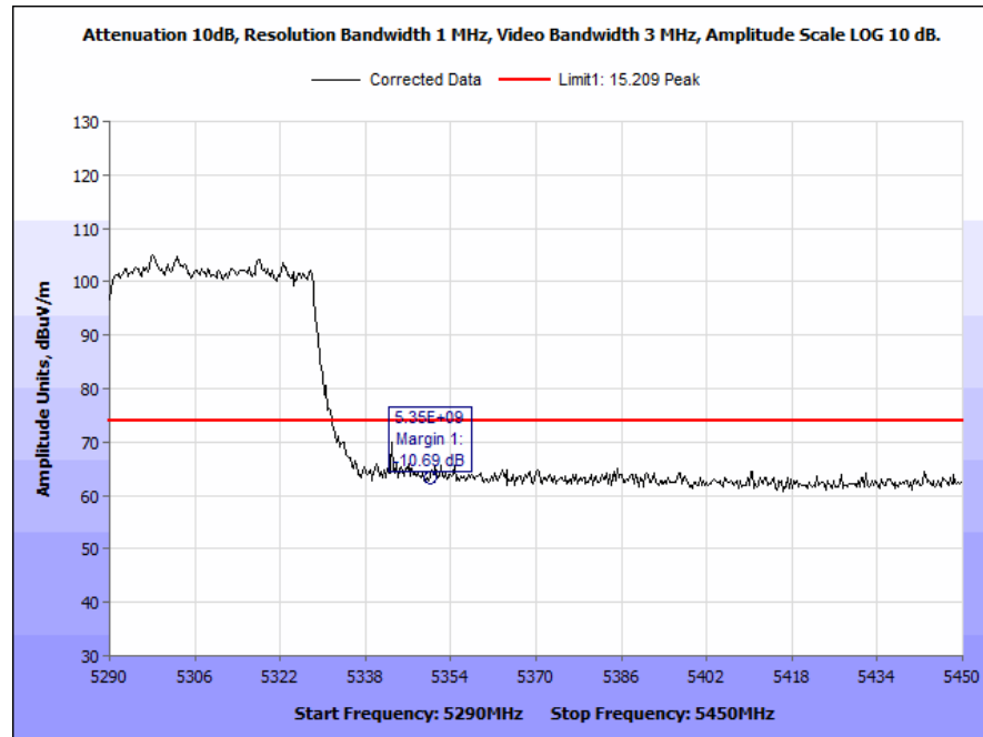
Plot 209. Radiated Band Edge, 802.11ac, 80 MHz, High Channel, 7 dBi Antenna, Peak
