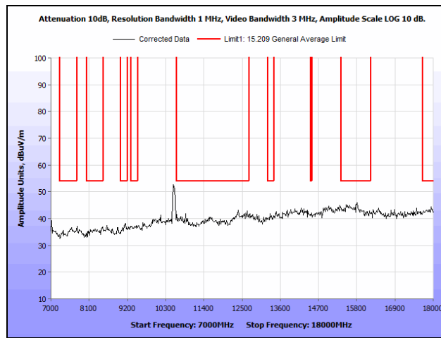
Plot 37. Radiated Spurious Emissions, 802.11a, 40 MHz, Low Channel, 7 GHz – 18 GHz, Peak, Ceiling Antenna
