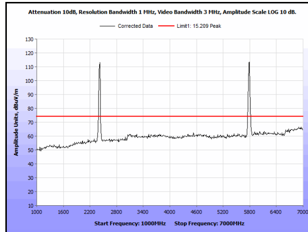
Plot 353. Radiated Spurs, Co-Location, 802.11n 20 MHz, 2437 MHz & 5785 MHz, 1 GHz – 7 GHz, Peak, Patch
