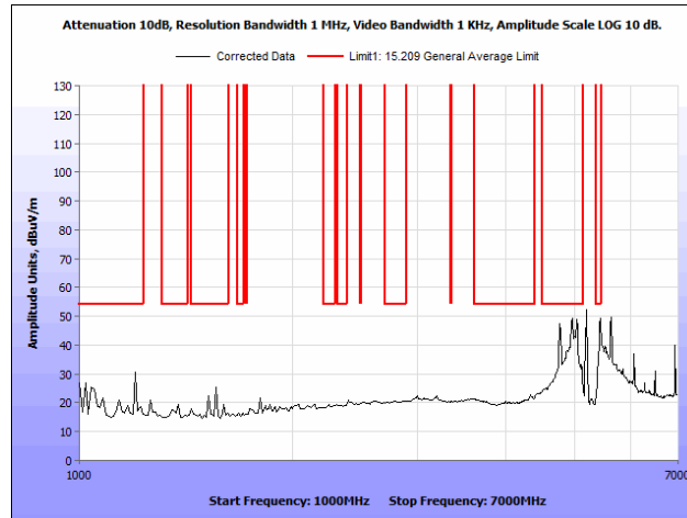
Plot 136. Radiated Spurious Emissions, 802.11n, 20 MHz, Mid Channel, 1 GHz – 7 GHz, Average, Patch Antenna
