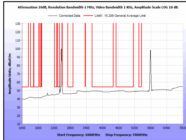
Plot 280. Radiated Spurs, Co-Location, 802.11n 20 MHz, 2462 MHz & 5785 MHz, 1 GHz – 7 GHz, Avg., Omni
