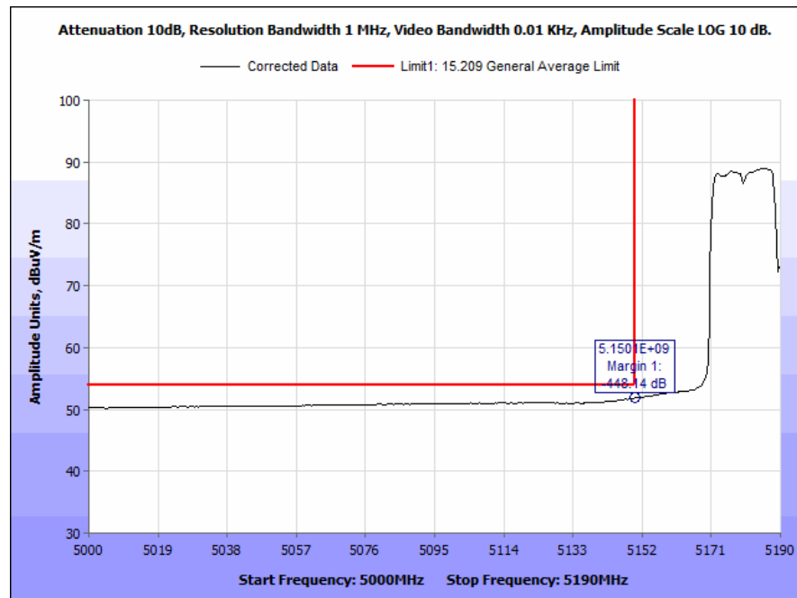
Plot 174. Radiated Band Edge, 802.11a, 40 MHz, Low Channel, 4 dBi Antenna, Average
