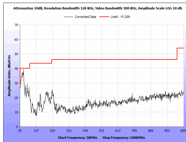
Plot 131. Radiated Spurious Emissions, 802.11n, 40 MHz, Low Channel, 30 MHz – 1 GHz, Patch Antenna
