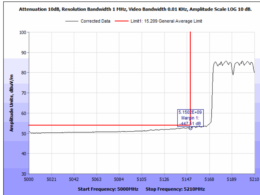
Plot 208. Radiated Band Edge, 802.11ac, 80 MHz, Low Channel, 7 dBi Antenna, Average
