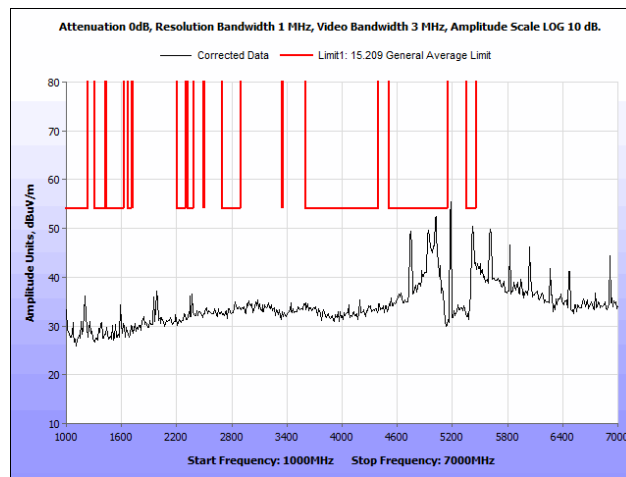
Plot 90. Radiated Spurious Emissions, 802.11n, 20 MHz, Low Channel, 1 GHz – 7 GHz, Average, Omni Antenna
