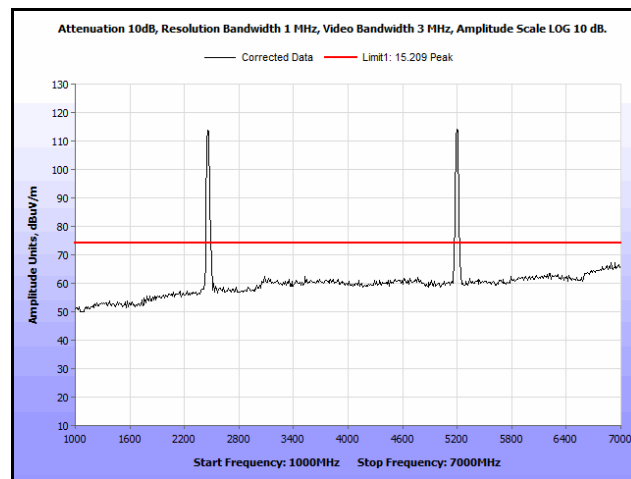
Plot 357. Radiated Spurs, Co-Location, 802.11n 20 MHz, 2462 MHz & 5200 MHz, 1 GHz – 7 GHz, Peak, Patch
