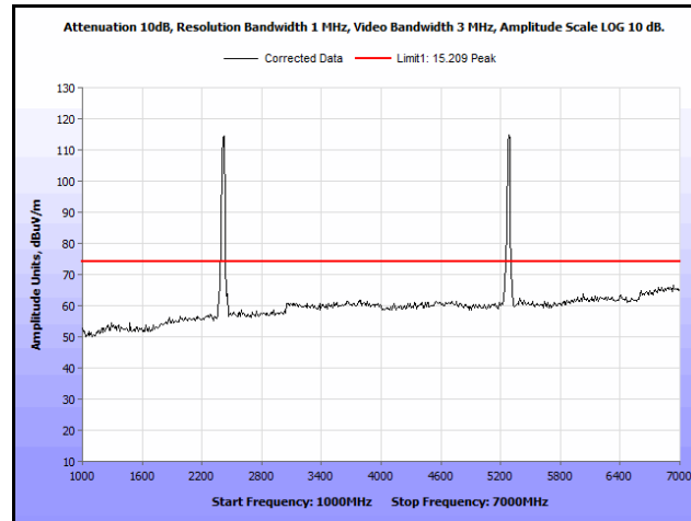
Plot 329. Radiated Spurs, Co-Location, 802.11n 20 MHz, 2412 MHz & 5300 MHz, 1 GHz – 7 GHz, Peak, Patch
