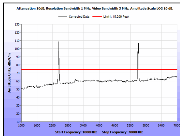
Plot 261. Radiated Spurs, Co-Location, 802.11n 20 MHz, 2437 MHz & 5580 MHz, 1 GHz – 7 GHz, Peak, Omni
