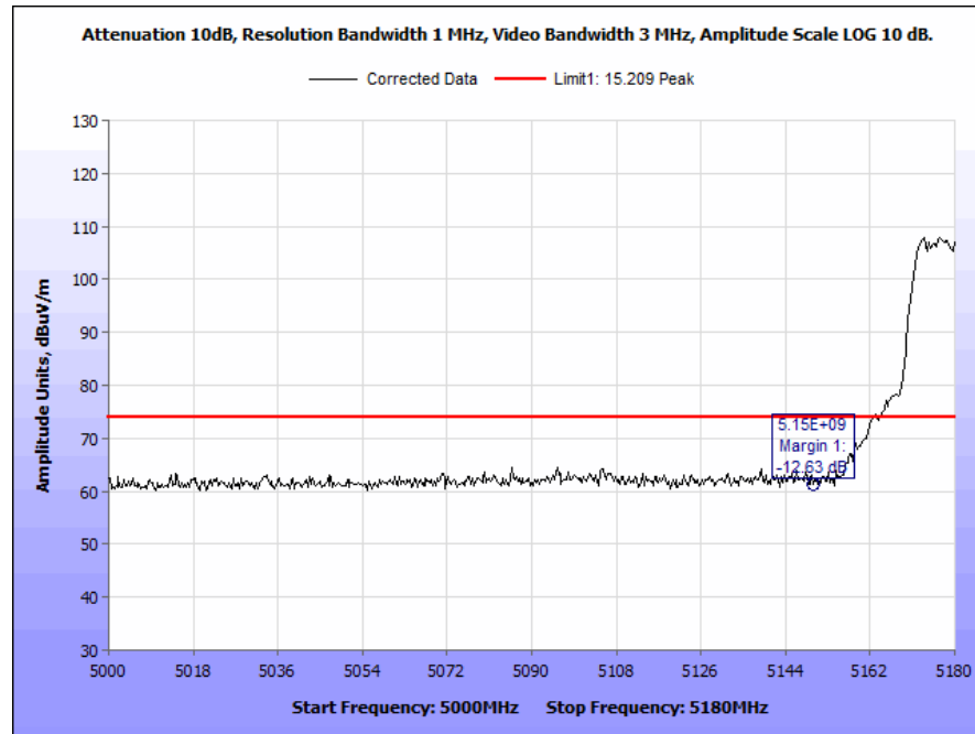
Plot 191. Radiated Band Edge, 802.11a, 20 MHz, Low Channel, 7 dBi Antenna, Peak
