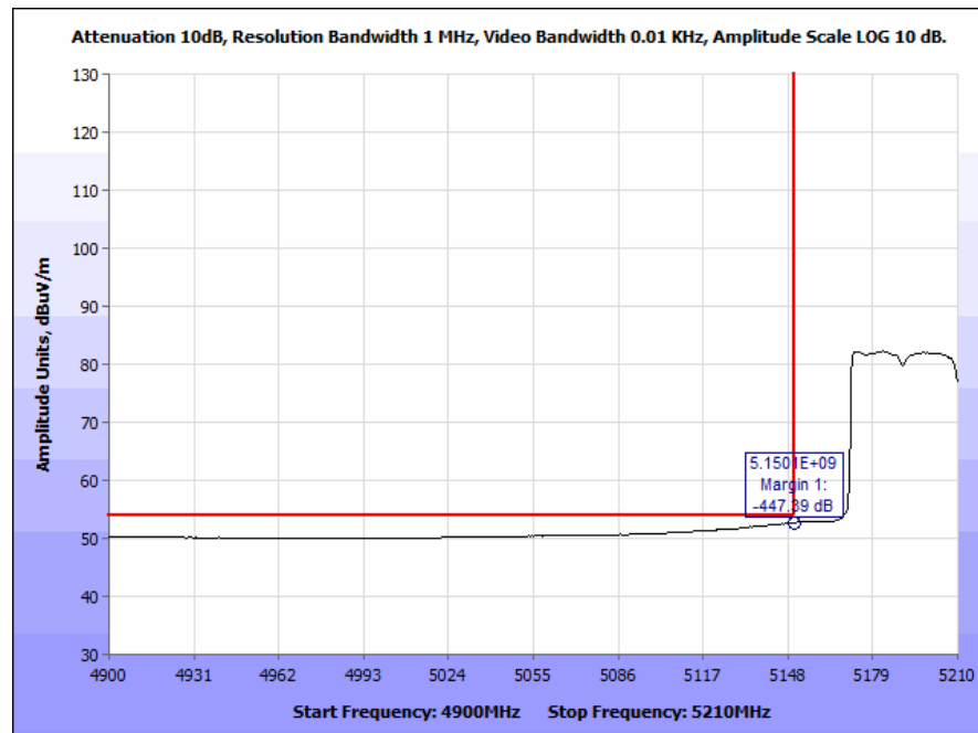
Plot 168. Radiated Band Edge, 802.11ac, 80 MHz, Low Channel, 6 dBi Omni Outdoor Antenna, Average
