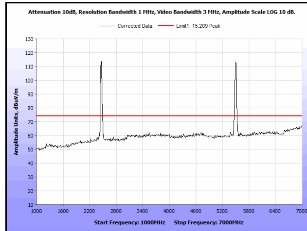
Plot 365. Radiated Spurs, Co-Location, 802.11n 20 MHz, 2462 MHz & 5580 MHz, 1 GHz – 7 GHz, Peak, Patch
