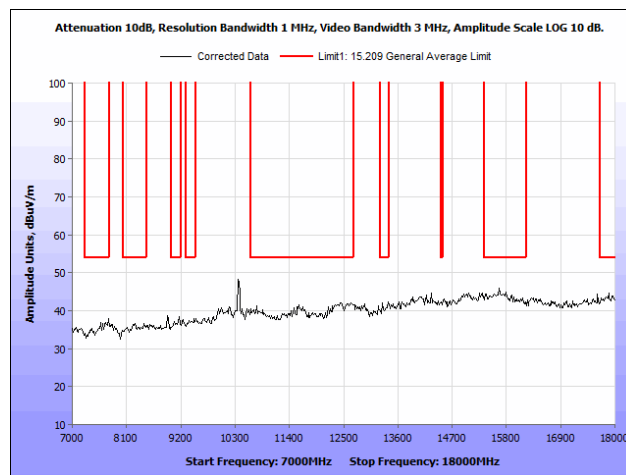
Plot 79. Radiated Spurious Emissions, 802.11a, 40 MHz, Low Channel, 7 GHz – 18 GHz, Omni Antenna
