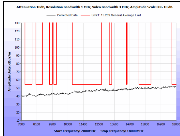
Plot 298. Radiated Spurs, Co-Location, 802.11n 20 MHz, 5200 MHz & 5785 MHz, 7 GHz – 18 GHz, Peak, Omni
