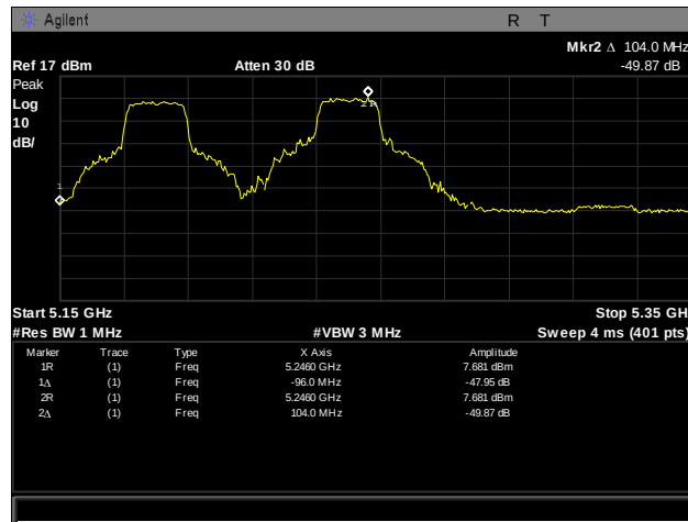
Plot 371. Frequency Stability, 5150 – 5350 MHz, -40°C, 120 V
