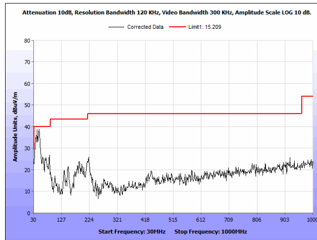
Plot 30. Radiated Spurious Emissions, 802.11a, 20 MHz, Low Channel, 30 MHz – 1 GHz, Ceiling Antenna
