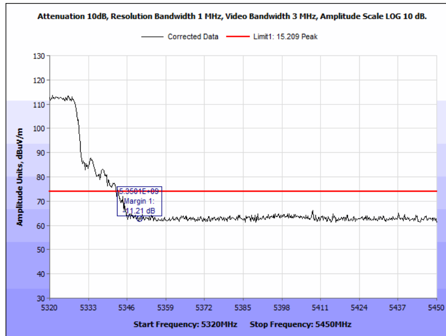
Plot 203. Radiated Band Edge, 802.11n, 20 MHz, High Channel, 7 dBi Antenna, Peak
