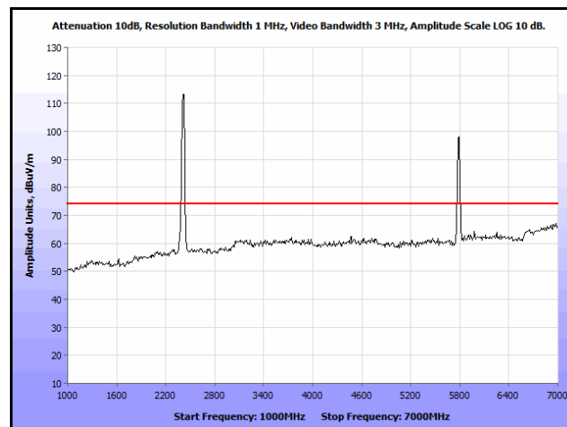
Plot 337. Radiated Spurs, Co-Location, 802.11n 20 MHz, 2412 MHz & 5785 MHz, 1 GHz – 7 GHz, Peak, Patch
