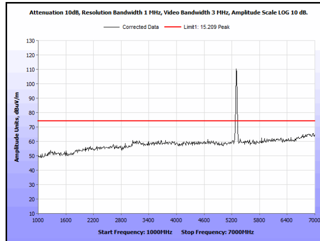
Plot 301. Radiated Spurs, Co-Location, 802.11n 20 MHz, 5300 MHz & 5300 MHz, 1 GHz – 7 GHz, Peak, Omni
