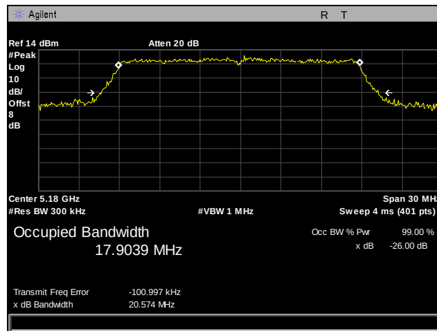
Plot 18. 26 dB Occupied Bandwidth, 802.11n, Port 1, 5180 MHz
