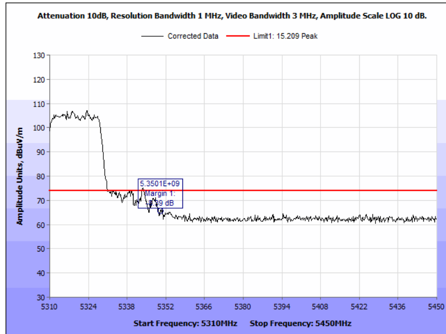
Plot 185. Radiated Band Edge, 802.11n, 40 MHz, High Channel, 4 dBi Antenna, Peak
