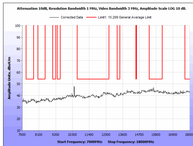
Plot 82. Radiated Spurious Emissions, 802.11a, 20 MHz, Mid Channel, 7 GHz – 18 GHz, Omni Antenna
