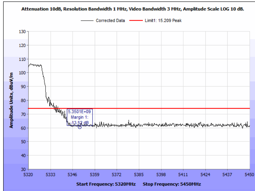
Plot 175. Radiated Band Edge, 802.11a, 20 MHz, High Channel, 4 dBi Antenna, Peak
