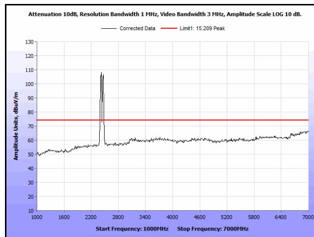
Plot 221. Radiated Spurs, Co-Location, 802.11n 20 MHz, 2412 MHz & 2462 MHz, 1 GHz – 7 GHz, Peak, Omni
