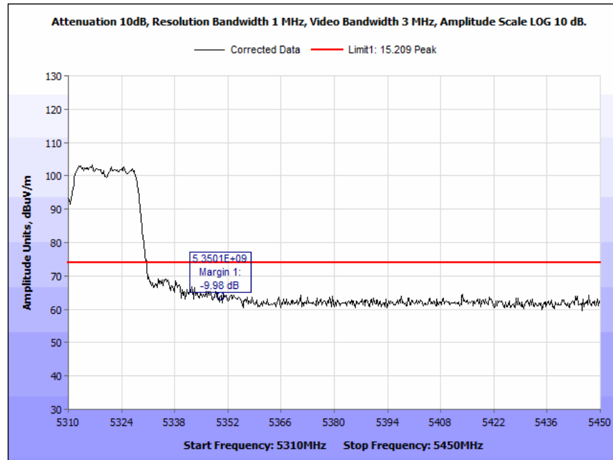
Plot 197. Radiated Band Edge, 802.11a, 40 MHz, High Channel, 7 dBi Antenna, Peak
