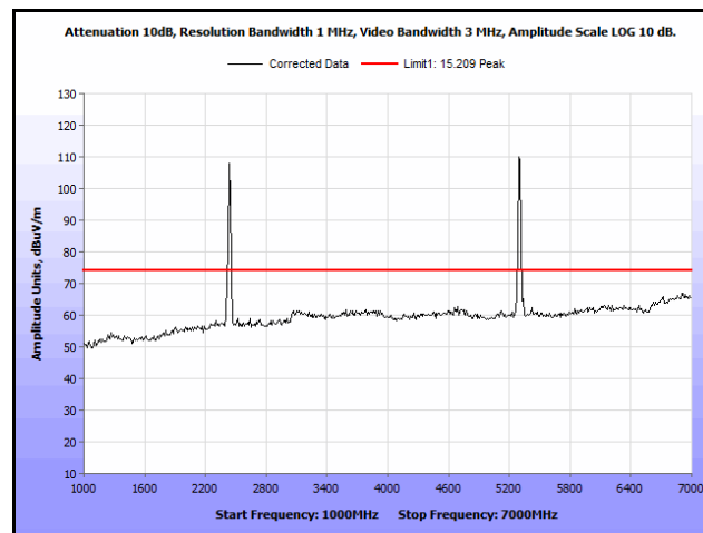
Plot 257. Radiated Spurs, Co-Location, 802.11n 20 MHz, 2437 MHz & 5300 MHz, 1 GHz – 7 GHz, Peak, Omni
