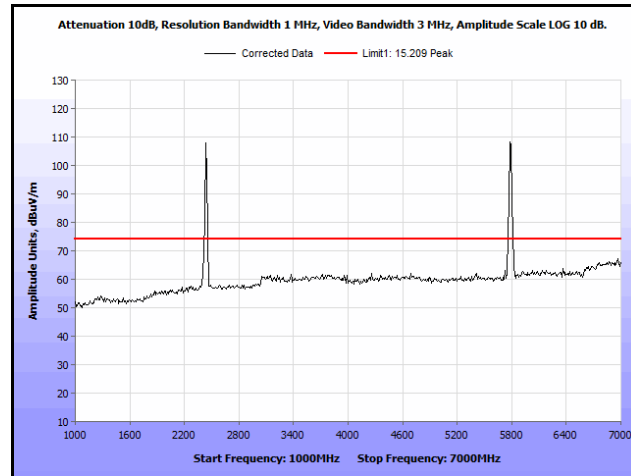
Plot 265. Radiated Spurs, Co-Location, 802.11n 20 MHz, 2437 MHz & 5785 MHz, 1 GHz – 7 GHz, Peak, Omni
