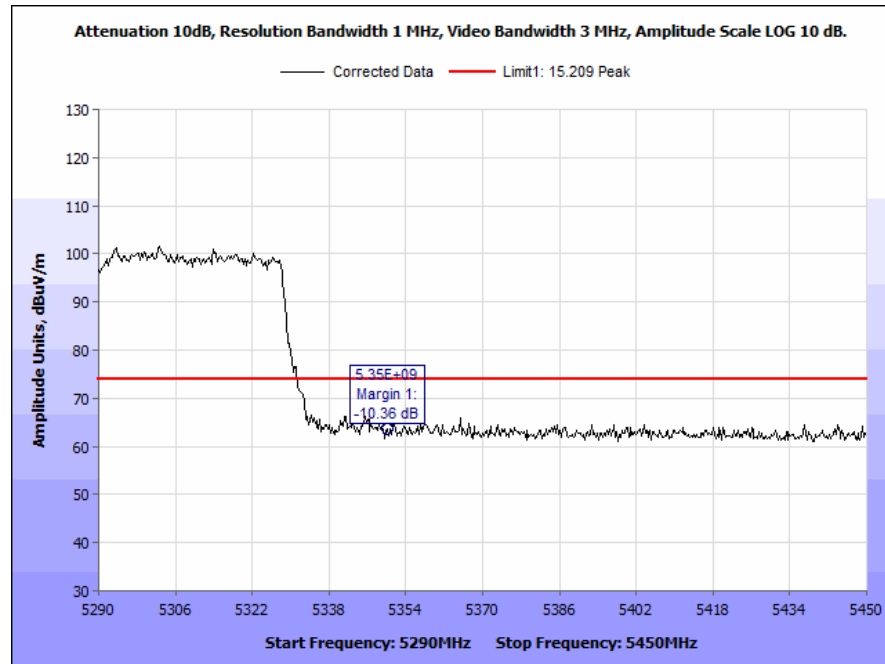
Plot 189. Radiated Band Edge, 802.11ac, 80 MHz, High Channel, 4 dBi Antenna, Peak
