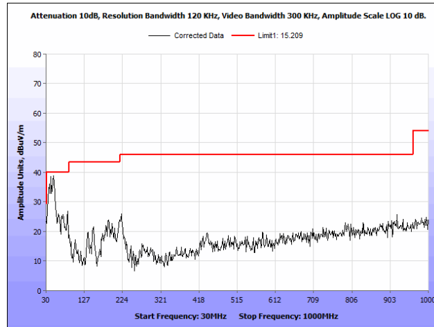
Plot 42. Radiated Spurious Emissions, 802.11a, 20 MHz, High Channel, 30 MHz – 1 GHz, Ceiling Antenna
