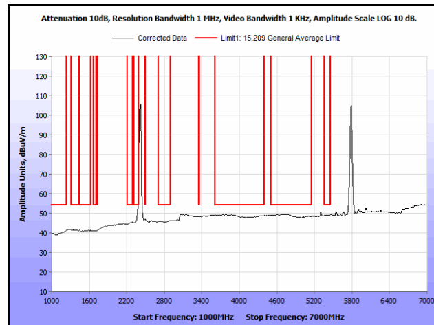
Plot 352. Radiated Spurs, Co-Location, 802.11n 20 MHz, 2437 MHz & 5785 MHz, 1 GHz – 7 GHz, Avg., Patch
