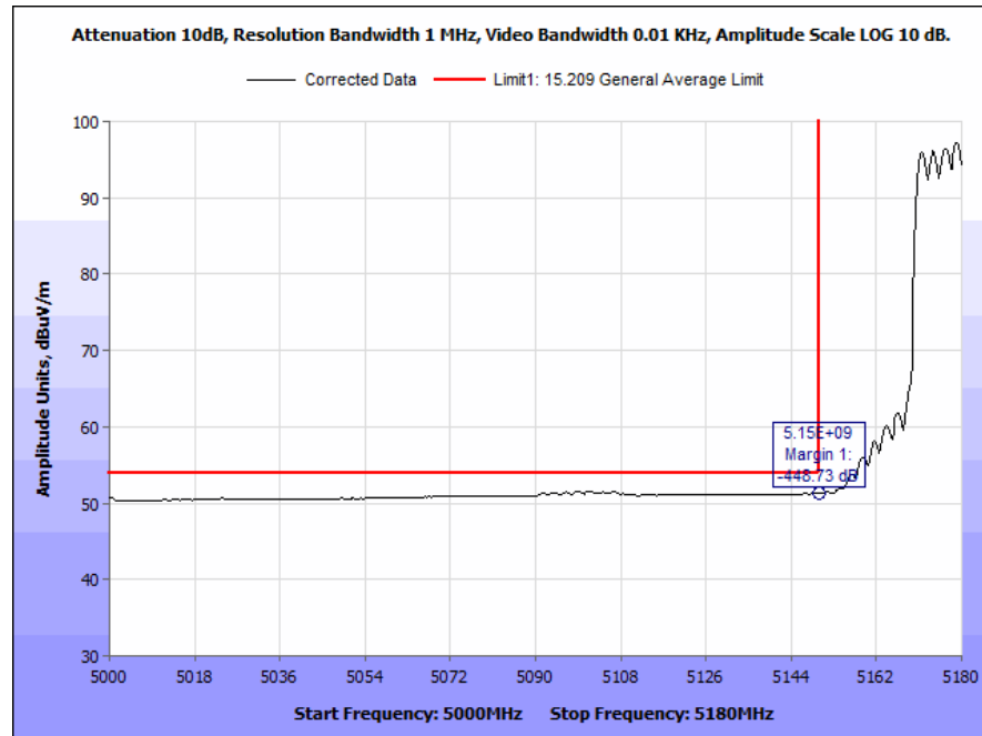
Plot 180. Radiated Band Edge, 802.11n, 20 MHz, Low Channel, 4 dBi Antenna, Average
