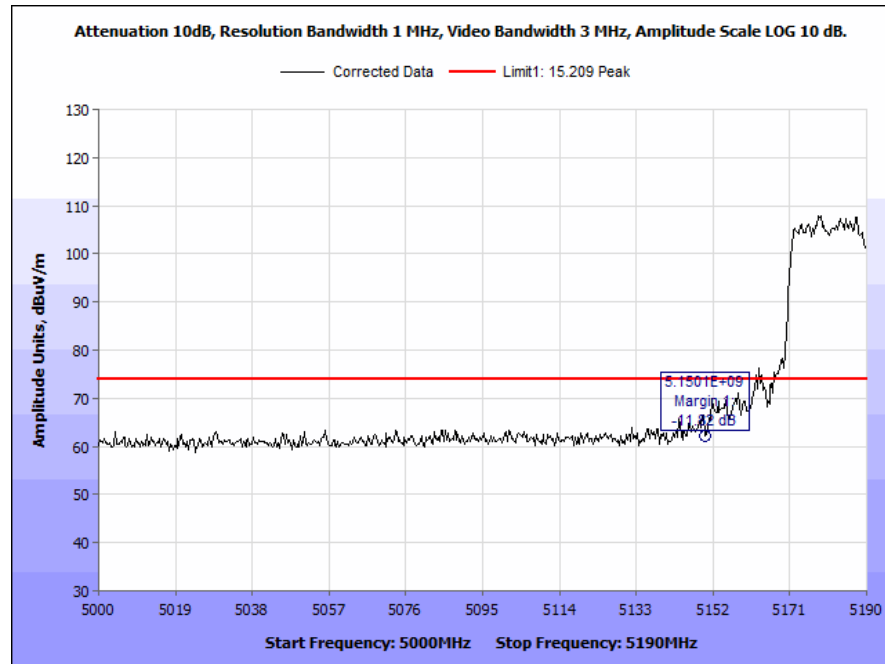
Plot 201. Radiated Band Edge, 802.11n, 40 MHz, Low Channel, 7 dBi Antenna, Peak
