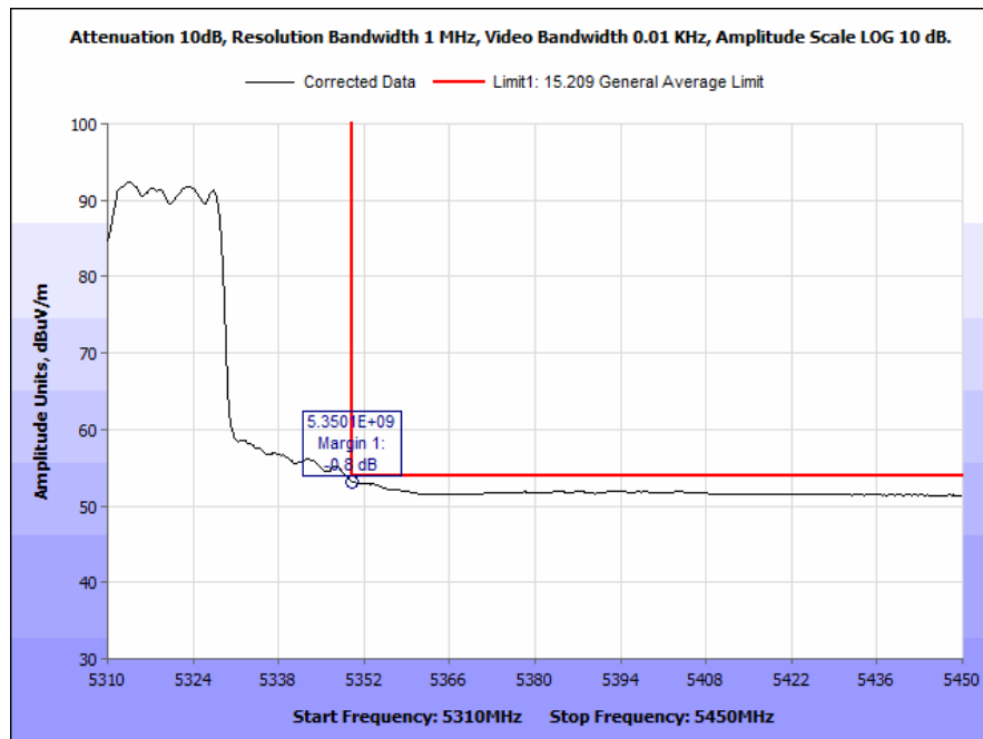
Plot 206. Radiated Band Edge, 802.11n, 40 MHz, High Channel, 7 dBi Antenna, Average
