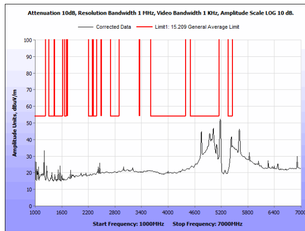
Plot 108. Radiated Spurious Emissions, 802.11a, 20 MHz, Low Channel, 1 GHz – 7 GHz, Average, Patch Antenna
