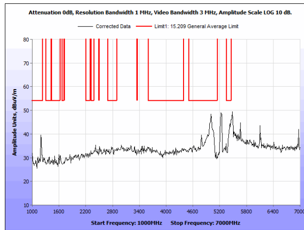
Plot 87. Radiated Spurious Emissions, 802.11a, 40 MHz, High Channel, 1 GHz – 7 GHz, Average, Omni Antenna
