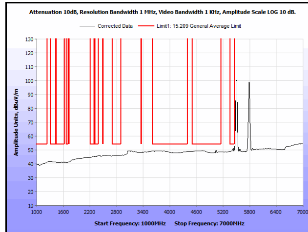
Plot 316. Radiated Spurs, Co-Location, 802.11n 20 MHz, 5580 MHz & 5785 MHz, 1 GHz – 7 GHz, Avg., Omni
