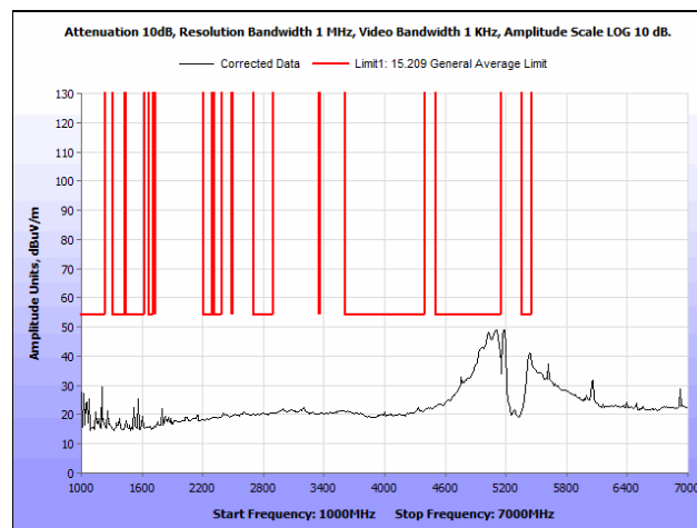
Plot 112. Radiated Spurious Emissions, 802.11a, 40 MHz, Low Channel, 1 GHz – 7 GHz, Average, Patch Antenna
