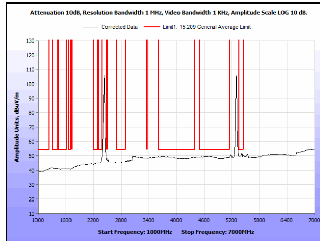
Plot 344. Radiated Spurs, Co-Location, 802.11n 20 MHz, 2437 MHz & 5300 MHz, 1 GHz – 7 GHz, Avg., Patch
