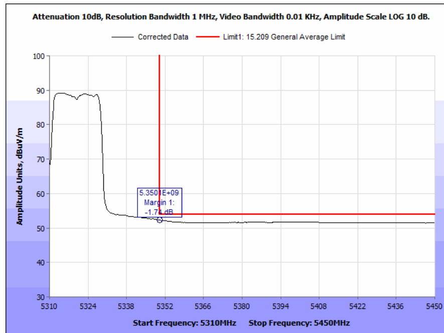
Plot 178. Radiated Band Edge, 802.11a, 40 MHz, High Channel, 4 dBi Antenna, Average
