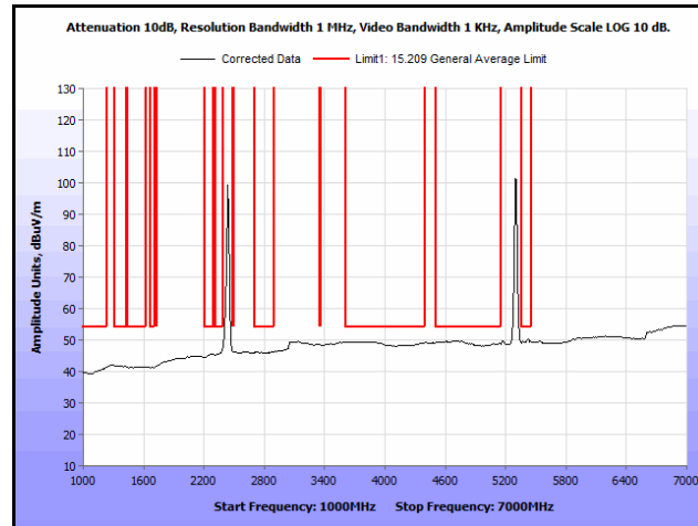
Plot 256. Radiated Spurs, Co-Location, 802.11n 20 MHz, 2437 MHz & 5300 MHz, 1 GHz – 7 GHz, Avg., Omni
