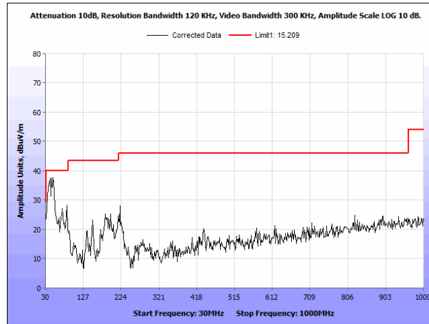
Plot 86. Radiated Spurious Emissions, 802.11a, 40 MHz, High Channel, 30 MHz – 1 GHz, Omni Antenna
