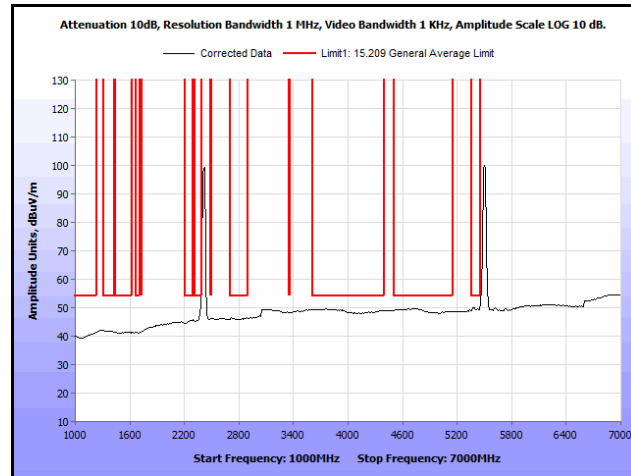
Plot 244. Radiated Spurs, Co-Location, 802.11n 20 MHz, 2412 MHz & 5580 MHz, 1 GHz – 7 GHz, Avg., Omni
