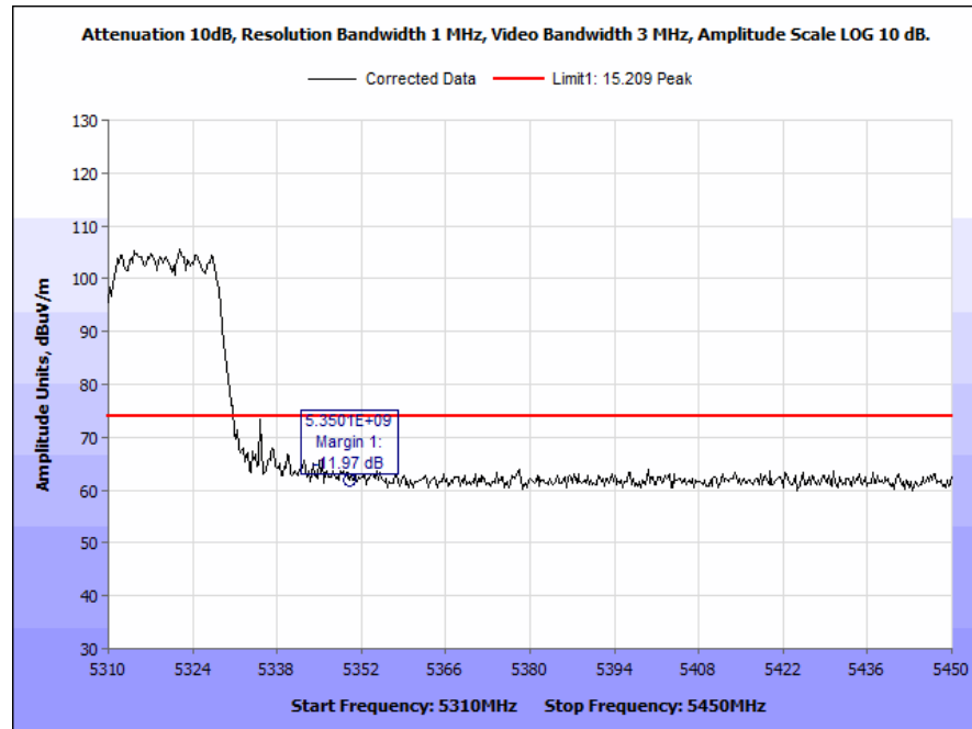
Plot 165. Radiated Band Edge, 802.11n, 40 MHz, High Channel, 6 dBi Omni Outdoor Antenna, Peak
