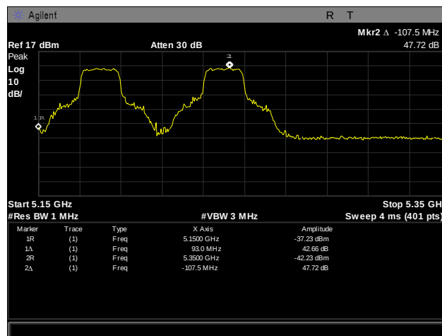
Plot 378. Frequency Stability, 5150 – 5350 MHz, 30°C, 120 V
