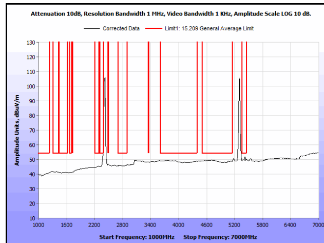
Plot 328. Radiated Spurs, Co-Location, 802.11n 20 MHz, 2412 MHz & 5300 MHz, 1 GHz – 7 GHz, Avg., Patch
