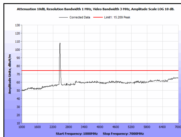
Plot 225. Radiated Spurs, Co-Location, 802.11n 20 MHz, 2437 MHz & 2437 MHz, 1 GHz – 7 GHz, Peak, Omni
