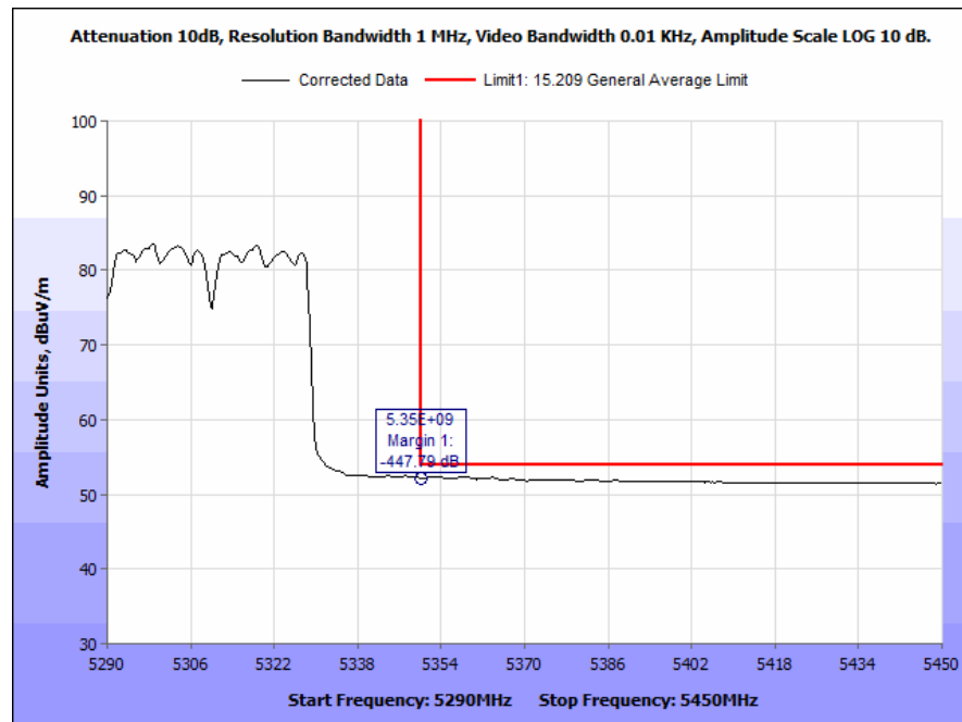
Plot 190. Radiated Band Edge, 802.11ac, 80 MHz, High Channel, 4 dBi Antenna, Average
