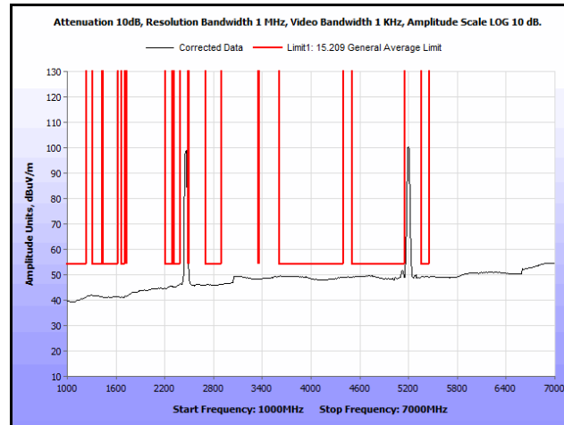
Plot 268. Radiated Spurs, Co-Location, 802.11n 20 MHz, 2462 MHz & 5200 MHz, 1 GHz – 7 GHz, Avg., Omni
