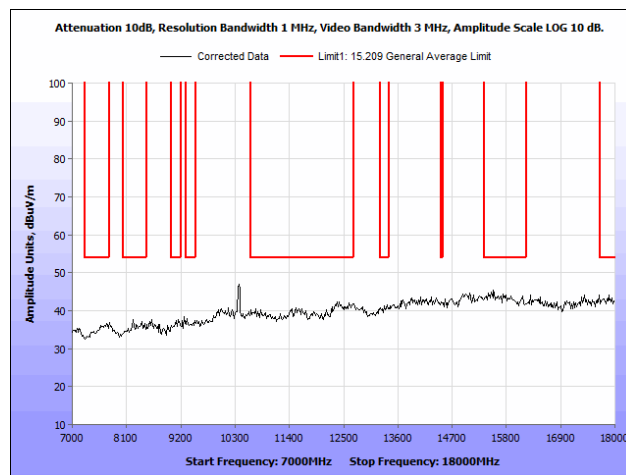
Plot 88. Radiated Spurious Emissions, 802.11a, 40 MHz, High Channel, 7 GHz – 18 GHz, Omni Antenna
