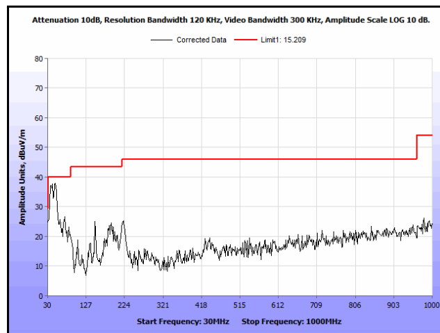
Plot 215. Radiated Spurs, Co-Location, 802.11n 20 MHz, 2412 MHz & 2437 MHz, 30 MHz – 1 GHz, Peak, Omni
