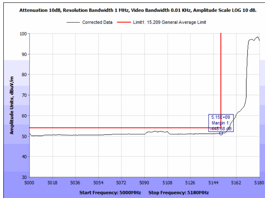
Plot 200. Radiated Band Edge, 802.11n, 20 MHz, Low Channel, 7 dBi Antenna, Average
