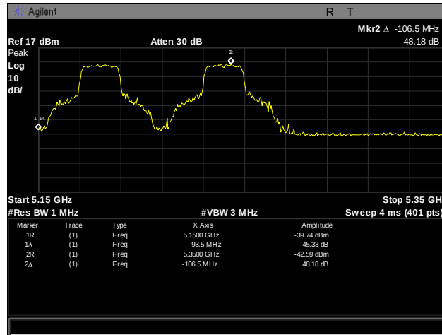
Plot 380. Frequency Stability, 5150 – 5350 MHz, 50°C, 120 V
