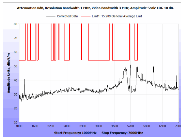
Plot 93. Radiated Spurious Emissions, 802.11n, 40 MHz, Low Channel, 1 GHz – 7 GHz, Average, Omni Antenna
