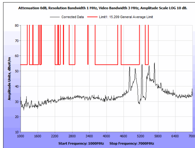
Plot 84. Radiated Spurious Emissions, 802.11a, 20 MHz, High Channel, 1 GHz – 7 GHz, Average, Omni Antenna
