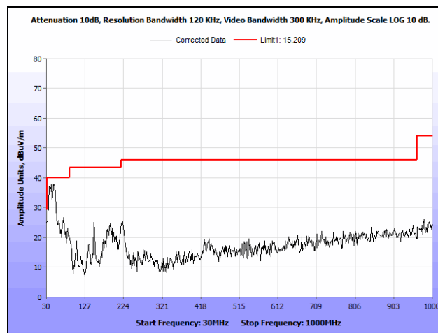
Plot 115. Radiated Spurious Emissions, 802.11a, 20 MHz, Mid Channel, 30 MHz – 1 GHz, Patch Antenna
