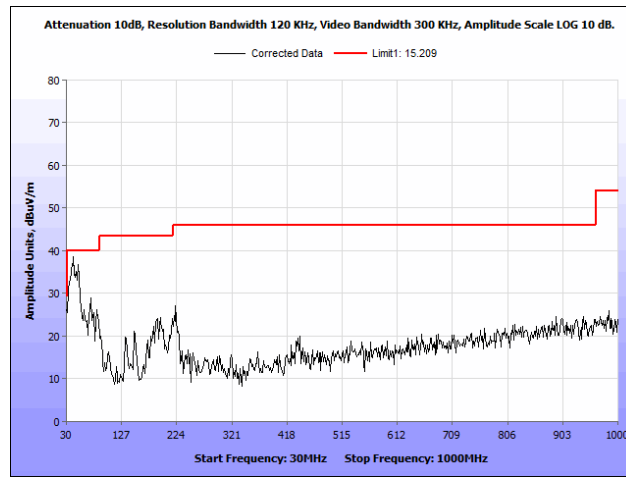
Plot 89. Radiated Spurious Emissions, 802.11n, 20 MHz, Low Channel, 30 MHz – 1 GHz, Omni Antenna
