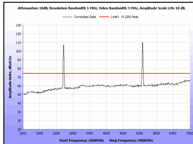
Plot 273. Radiated Spurs, Co-Location, 802.11n 20 MHz, 2462 MHz & 5300 MHz, 1 GHz – 7 GHz, Peak, Omni
