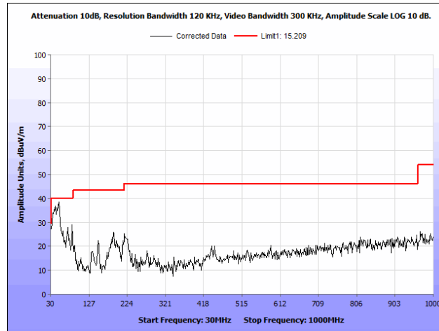
Plot 95. Radiated Spurious Emissions, 802.11n, 20 MHz, Mid Channel, 30 MHz – 1 GHz, Omni Antenna
