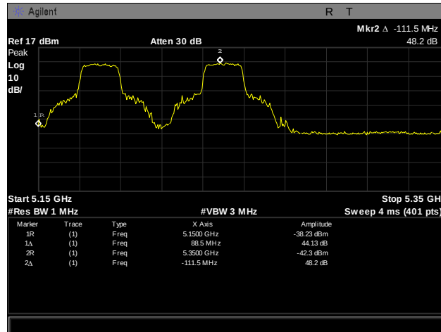
Plot 377. Frequency Stability, 5150 – 5350 MHz, 20°C, 120 V
