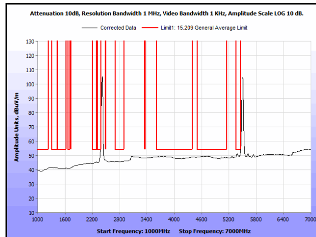
Plot 364. Radiated Spurs, Co-Location, 802.11n 20 MHz, 2462 MHz & 5580 MHz, 1 GHz – 7 GHz, Avg., Patch
