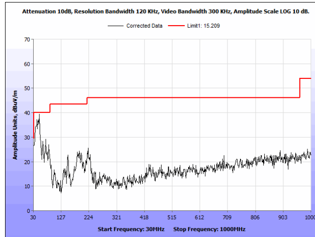
Plot 62. Radiated Spurious Emissions, 802.11n, 20 MHz, High Channel, 30 MHz – 1 GHz, Ceiling Antenna
