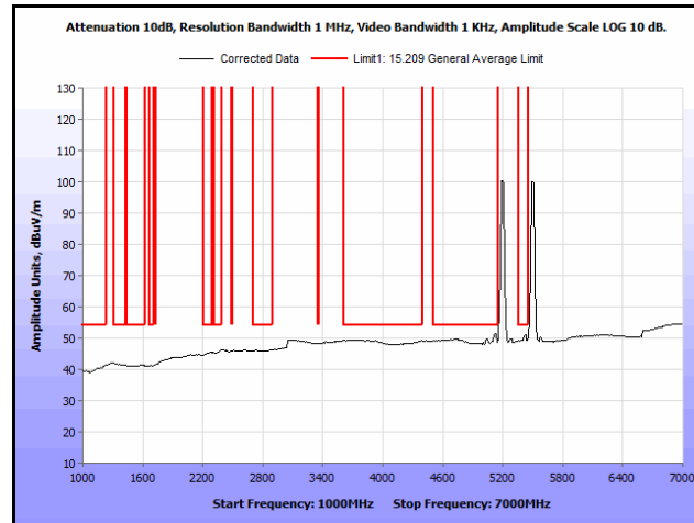
Plot 292. Radiated Spurs, Co-Location, 802.11n 20 MHz, 5200 MHz & 5580 MHz, 1 GHz – 7 GHz, Avg., Omni
