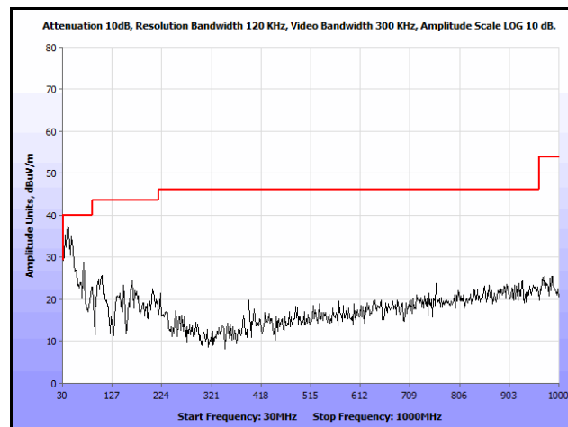
Plot 255. Radiated Spurs, Co-Location, 802.11n 20 MHz, 2437 MHz & 5300 MHz, 30 MHz – 1 GHz, Peak, Omni
