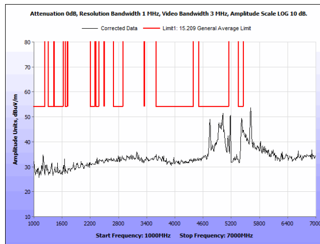
Plot 75. Radiated Spurious Emissions, 802.11a, 20 MHz, Low Channel, 1 GHz – 7 GHz, Average, Omni Antenna
