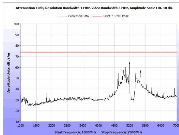
Plot 52. Radiated Spurious Emissions, 802.11n, Low Channel, 1 GHz – 7 GHz, Peak, Ceiling Antenna
