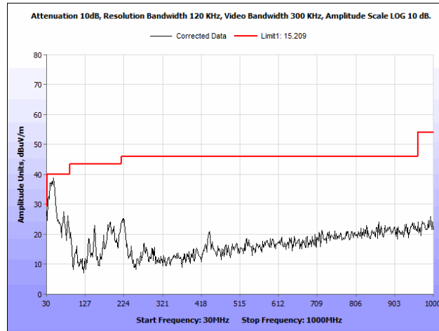
Plot 77. Radiated Spurious Emissions, 802.11a, 40 MHz, Low Channel, 30 MHz – 1 GHz, Omni Antenna
