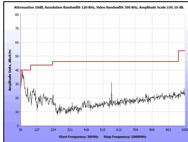
Plot 319. Radiated Spurs, Co-Location, 802.11n 20 MHz, 5785 MHz & 5785 MHz, 30 MHz – 1 GHz, Peak, Omni
