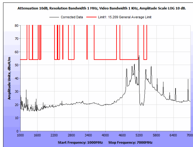
Plot 51. Radiated Spurious Emissions, 802.11n, Low Channel, 1 GHz – 7 GHz, Average, Ceiling Antenna
