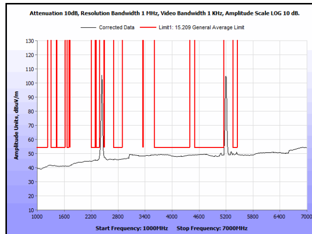
Plot 340. Radiated Spurs, Co-Location, 802.11n 20 MHz, 2437 MHz & 5200 MHz, 1 GHz – 7 GHz, Avg., Patch
