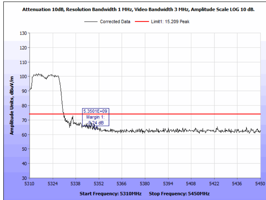
Plot 177. Radiated Band Edge, 802.11a, 40 MHz, High Channel, 4 dBi Antenna, Peak
