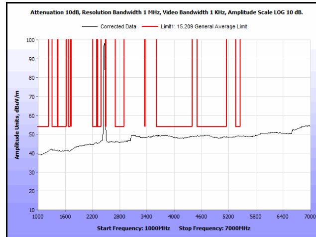
Plot 232. Radiated Spurs, Co-Location, 802.11n 20 MHz, 2462 MHz & 2462 MHz, 1 GHz – 7 GHz, Avg., Omni
