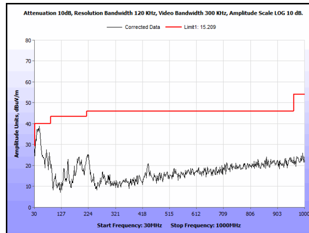
Plot 223. Radiated Spurs, Co-Location, 802.11n 20 MHz, 2437 MHz & 2437 MHz, 30 MHz – 1 GHz, Peak, Omni
