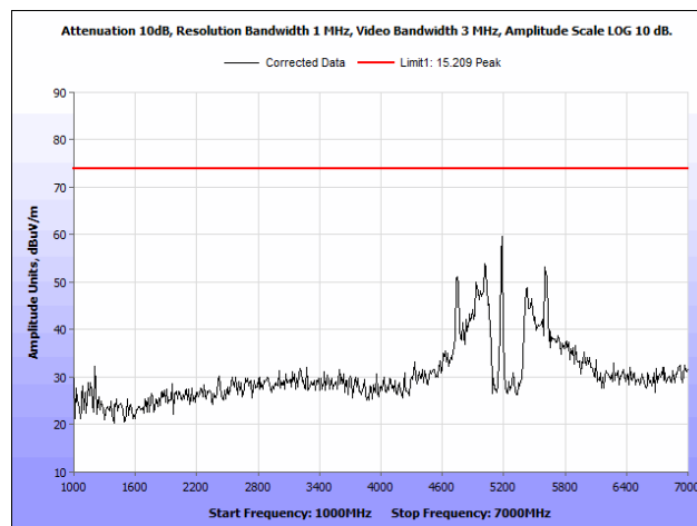
Plot 32. Radiated Spurious Emissions, 802.11a, Low Channel, 1 GHz – 7 GHz, Peak, Ceiling Antenna
