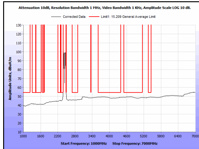
Plot 220. Radiated Spurs, Co-Location, 802.11n 20 MHz, 2412 MHz & 2462 MHz, 1 GHz – 7 GHz, Avg., Omni
