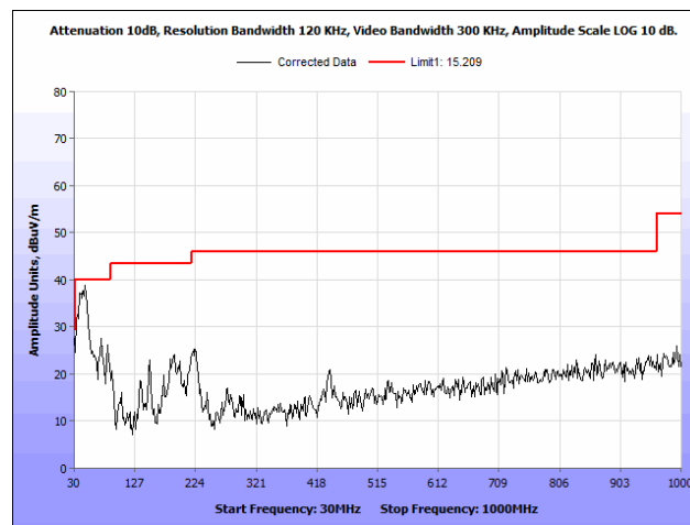
Plot 111. Radiated Spurious Emissions, 802.11a, 40 MHz, Low Channel, 30 MHz – 1 GHz, Patch Antenna
