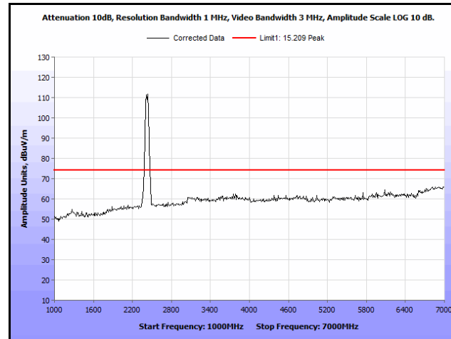
Plot 217. Radiated Spurs, Co-Location, 802.11n 20 MHz, 2412 MHz & 2437 MHz, 1 GHz – 7 GHz, Peak, Omni
