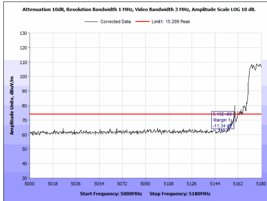
Plot 179. Radiated Band Edge, 802.11n, 20 MHz, Low Channel, 4 dBi Antenna, Peak
