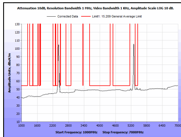
Plot 360. Radiated Spurs, Co-Location, 802.11n 20 MHz, 2462 MHz & 5300 MHz, 1 GHz – 7 GHz, Avg., Patch
