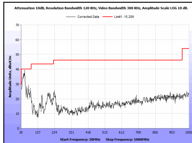
Plot 331. Radiated Spurs, Co-Location, 802.11n 20 MHz, 2412 MHz & 5580 MHz, 30 MHz – 1 GHz, Peak, Patch
