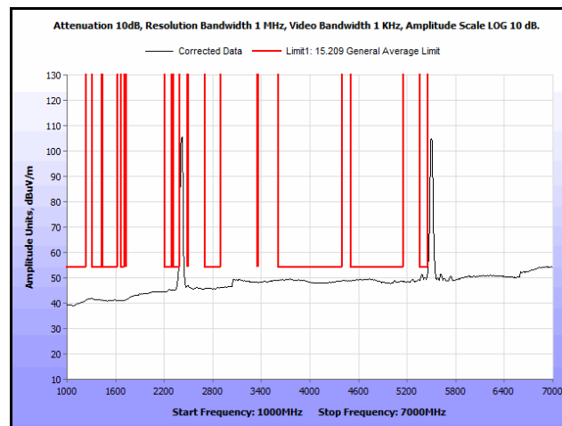
Plot 348. Radiated Spurs, Co-Location, 802.11n 20 MHz, 2437 MHz & 5580 MHz, 1 GHz – 7 GHz, Avg., Patch
