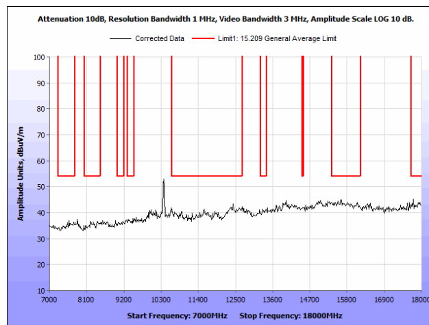
Plot 103. Radiated Spurious Emissions, 802.11n, 40 MHz, High Channel, 7 GHz – 18 GHz, Omni Antenna
