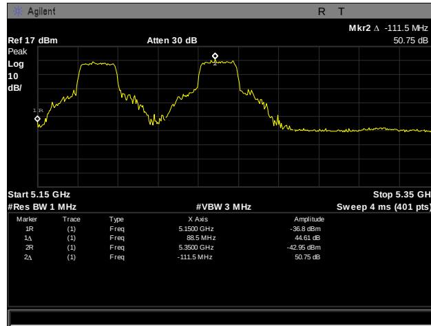
Plot 374. Frequency Stability, 5150 – 5350 MHz, -10°C, 120 V
