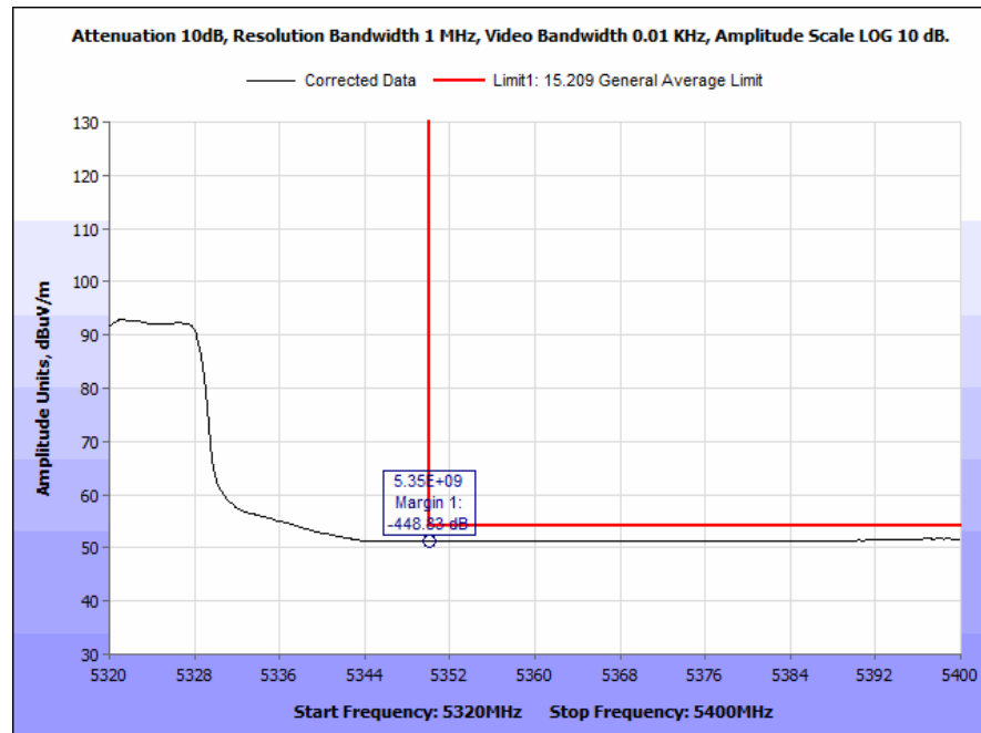
Plot 156. Radiated Band Edge, 802.11a, 20 MHz, High Channel, 6 dBi Omni Outdoor Antenna, Average
