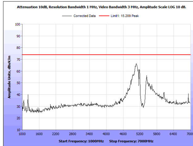
Plot 56. Radiated Spurious Emissions, 802.11n, 40 MHz, Low Channel, 1 GHz – 7 GHz, Peak, Ceiling Antenna
