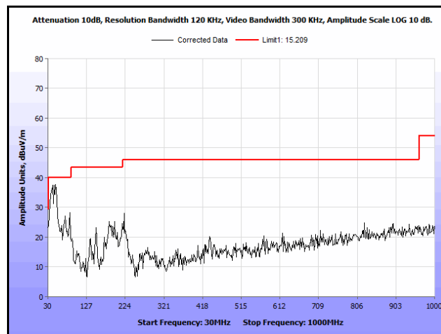
Plot 227. Radiated Spurs, Co-Location, 802.11n 20 MHz, 2437 MHz & 2462 MHz, 30 MHz – 1 GHz, Peak, Omni
