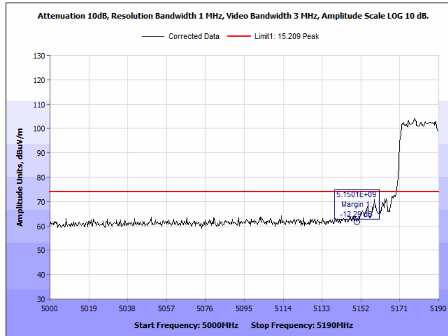
Plot 181. Radiated Band Edge, 802.11n, 40 MHz, Low Channel, 4 dBi Antenna, Peak
