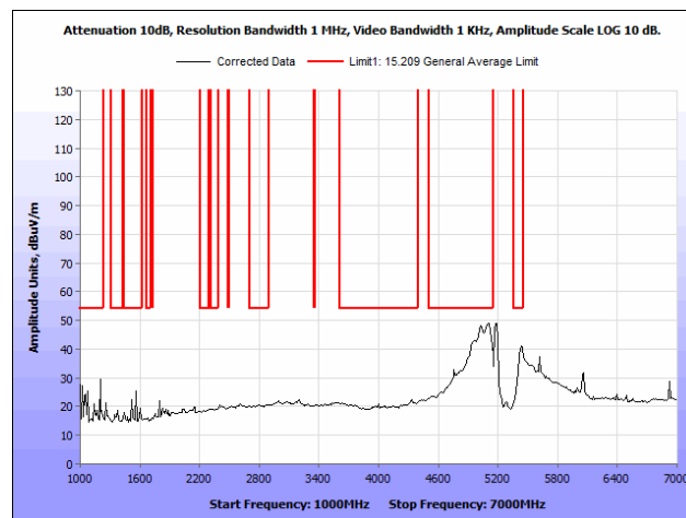
Plot 35. Radiated Spurious Emissions, 802.11a, 40 MHz, Low Channel, 1 GHz – 7 GHz, Average, Ceiling Antenna
