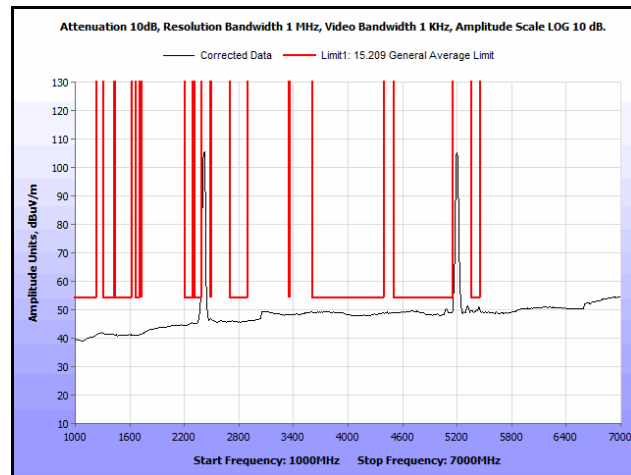
Plot 324. Radiated Spurs, Co-Location, 802.11n 20 MHz, 2412 MHz & 5200 MHz, 1 GHz – 7 GHz, Avg., Patch
