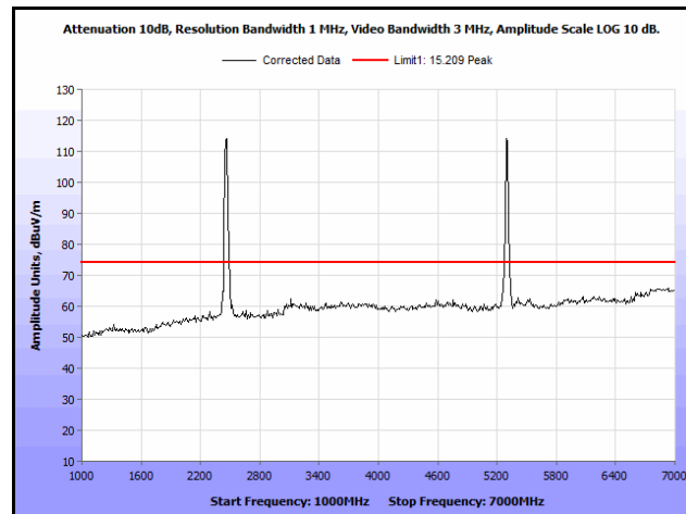
Plot 361. Radiated Spurs, Co-Location, 802.11n 20 MHz, 2462 MHz & 5300 MHz, 1 GHz – 7 GHz, Peak, Patch
