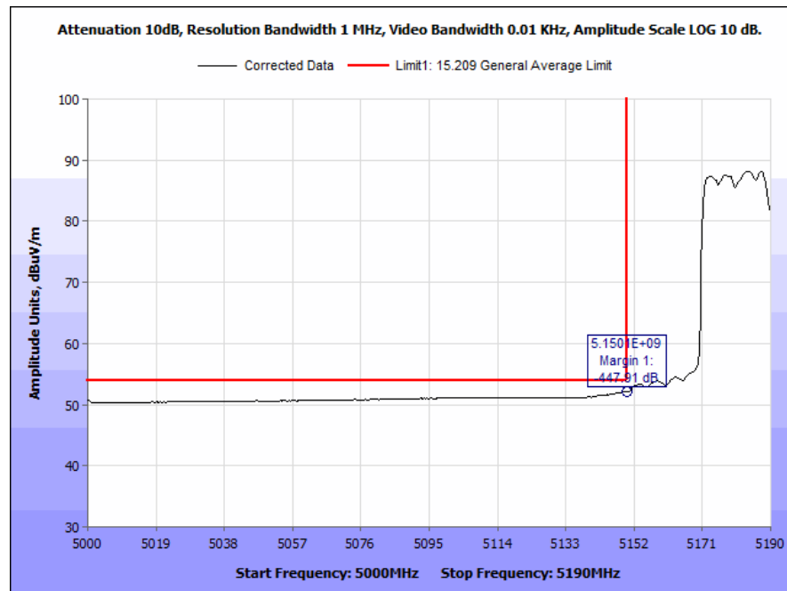
Plot 182. Radiated Band Edge, 802.11n, 40 MHz, Low Channel, 4 dBi Antenna, Average
