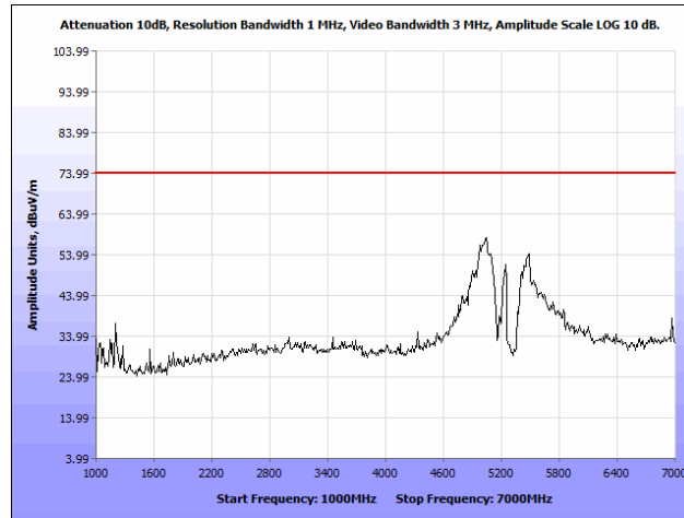
Plot 125. Radiated Spurious Emissions, 802.11a, 40 MHz, High Channel, 1 GHz – 7 GHz, Peak, Patch Antenna
