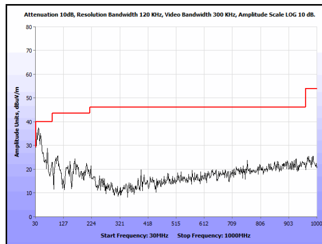
Plot 311. Radiated Spurs, Co-Location, 802.11n 20 MHz, 5580 MHz & 5580 MHz, 30 MHz – 1 GHz, Peak, Omni
