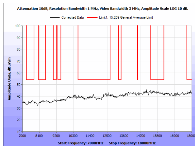
Plot 106. Radiated Spurious Emissions, 802.11ac, 7 GHz – 18 GHz, Omni Antenna
