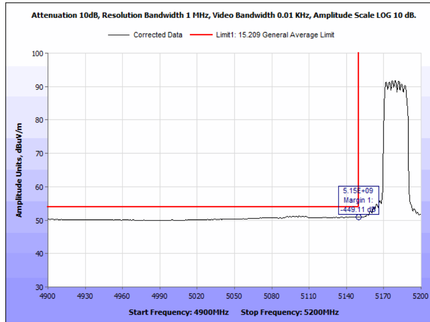
Plot 160. Radiated Band Edge, 802.11n, 20 MHz, Low Channel, 6 dBi Omni Outdoor Antenna, Average
