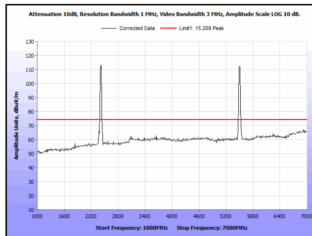
Plot 333. Radiated Spurs, Co-Location, 802.11n 20 MHz, 2412 MHz & 5580 MHz, 1 GHz – 7 GHz, Peak, Patch
