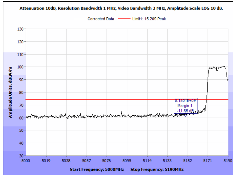
Plot 173. Radiated Band Edge, 802.11a, 40 MHz, Low Channel, 4 dBi Antenna, Peak
