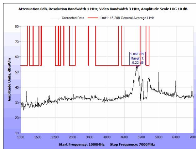
Plot 105. Radiated Spurious Emissions, 802.11ac, 1 GHz – 7 GHz, Average, Omni Antenna
