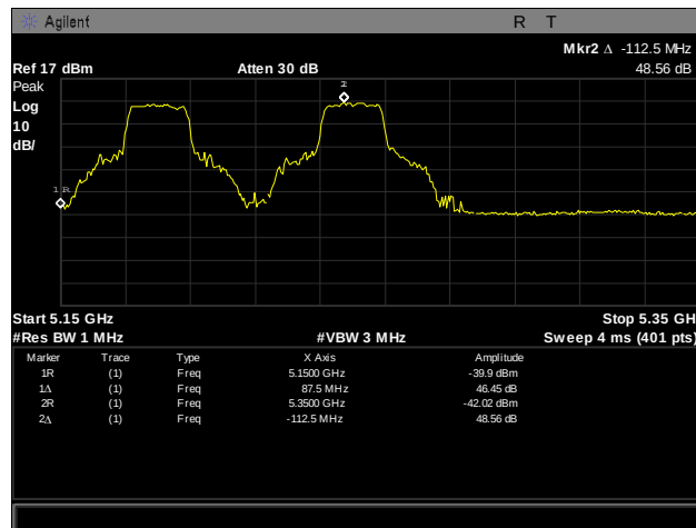
Plot 375. Frequency Stability, 5150 – 5350 MHz, 0°C, 120 V
