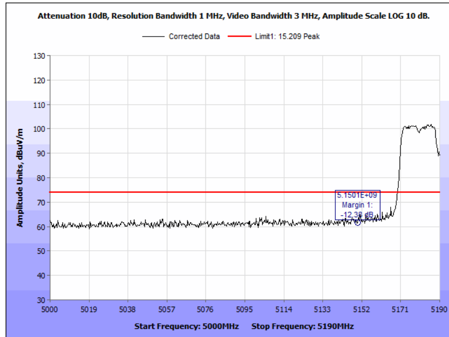
Plot 153. Radiated Band Edge, 802.11a, 40 MHz, Low Channel, 6 dBi Omni Outdoor Antenna, Peak
