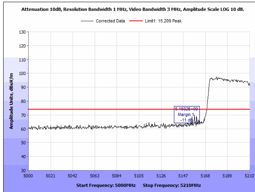
Plot 167. Radiated Band Edge, 802.11ac, 80 MHz, Low Channel, 6 dBi Omni Outdoor Antenna, Peak
