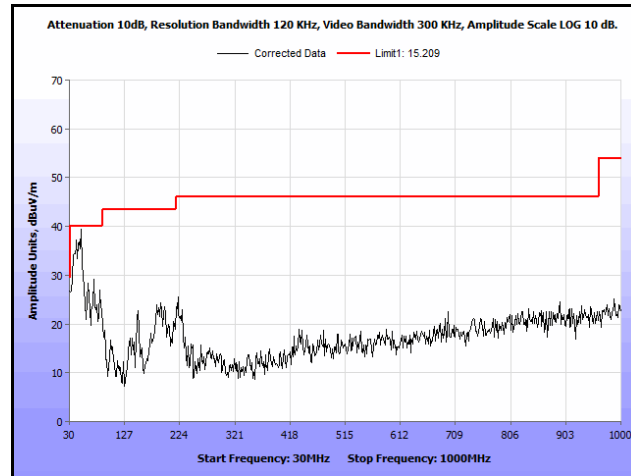
Plot 295. Radiated Spurs, Co-Location, 802.11n 20 MHz, 5200 MHz & 5785 MHz, 30 MHz – 1 GHz, Peak, Omni
