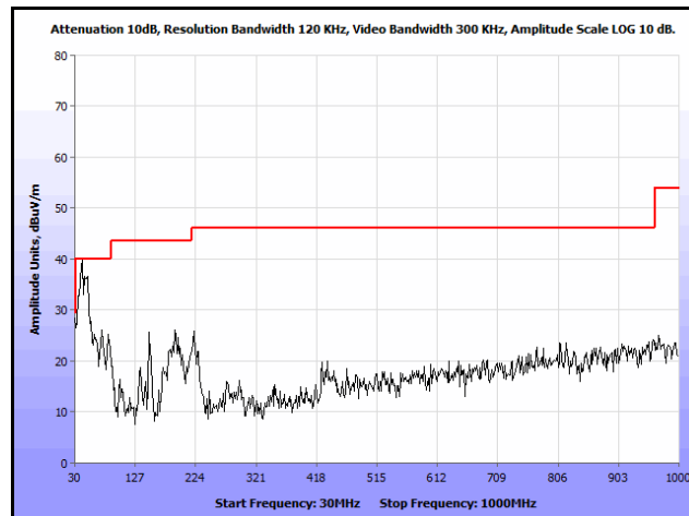
Plot 231. Radiated Spurs, Co-Location, 802.11n 20 MHz, 2462 MHz & 2462 MHz, 30 MHz – 1 GHz, Peak, Omni
