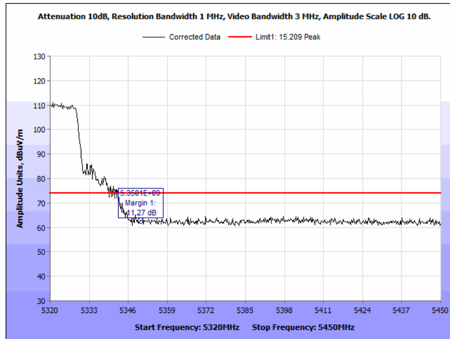
Plot 183. Radiated Band Edge, 802.11n, 20 MHz, High Channel, 4 dBi Antenna, Peak
