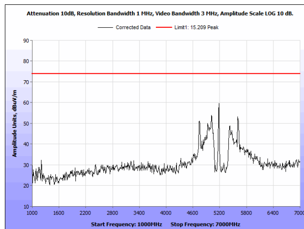
Plot 109. Radiated Spurious Emissions, 802.11a, 20 MHz, Low Channel, 1 GHz – 7 GHz, Peak, Patch Antenna
