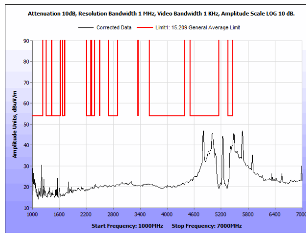
Plot 120. Radiated Spurious Emissions, 802.11a, 20 MHz, High Channel, 1 GHz – 7 GHz, Average, Patch Antenna
