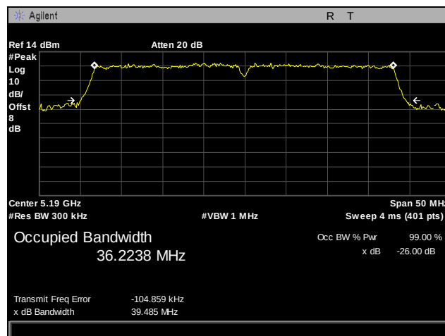
Plot 24. 26 dB Occupied Bandwidth, 802.11n, Port 2, 5190 MHz
