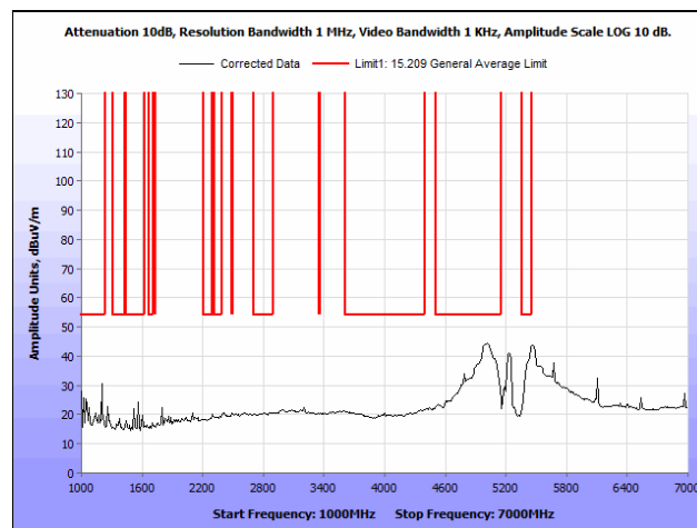
Plot 124. Radiated Spurious Emissions, 802.11a, 40 MHz, High Channel, 1 GHz – 7 GHz, Average, Patch Antenna
