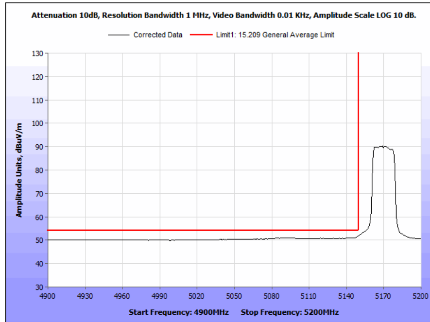
Plot 152. Radiated Band Edge, 802.11a, 20 MHz, Low Channel, 6 dBi Omni Outdoor Antenna, Average
