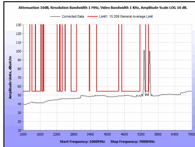
Plot 304. Radiated Spurs, Co-Location, 802.11n 20 MHz, 5300 MHz & 5580 MHz, 1 GHz – 7 GHz, Avg., Omni
