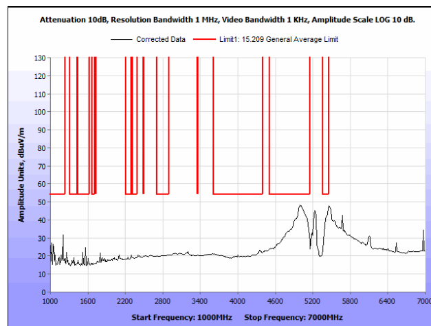
Plot 67. Radiated Spurious Emissions, 802.11n, 40 MHz, High Channel, 1 GHz – 7 GHz, Average, Ceiling Antenna
