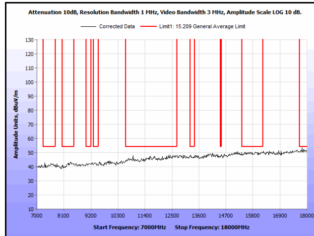
Plot 214. Radiated Spurs, Co-Location, 802.11n 20 MHz, 2412 MHz & 2412 MHz, 7 GHz – 18 GHz, Peak, Omni
