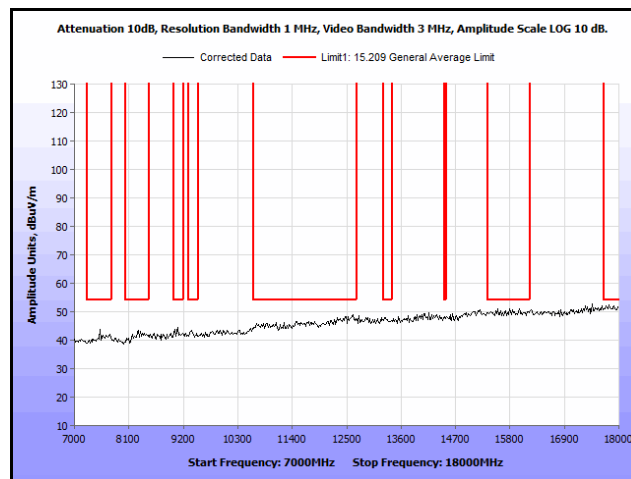
Plot 230. Radiated Spurs, Co-Location, 802.11n 20 MHz, 2437 MHz & 2462 MHz, 7 GHz – 18 GHz, Peak, Omni
