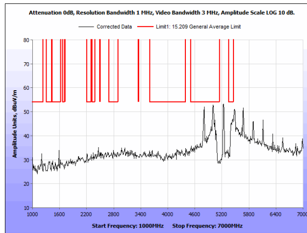
Plot 96. Radiated Spurious Emissions, 802.11n, 20 MHz, Mid Channel, 1 GHz – 7 GHz, Average, Omni Antenna
