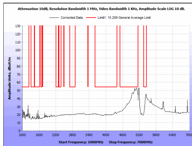
Plot 55. Radiated Spurious Emissions, 802.11n, 40 MHz, Low Channel, 1 GHz – 7 GHz, Average, Ceiling Antenna
