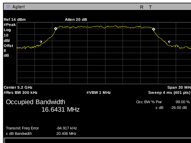
Plot 15. 26 dB Occupied Bandwidth, 802.11a, 5200 MHz
