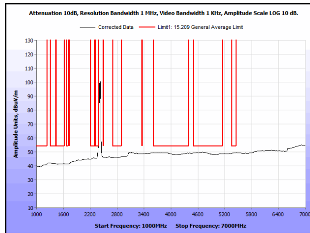
Plot 212. Radiated Spurs, Co-Location, 802.11n 20 MHz, 2412 MHz & 2412 MHz, 1 GHz – 7 GHz, Avg., Omni
