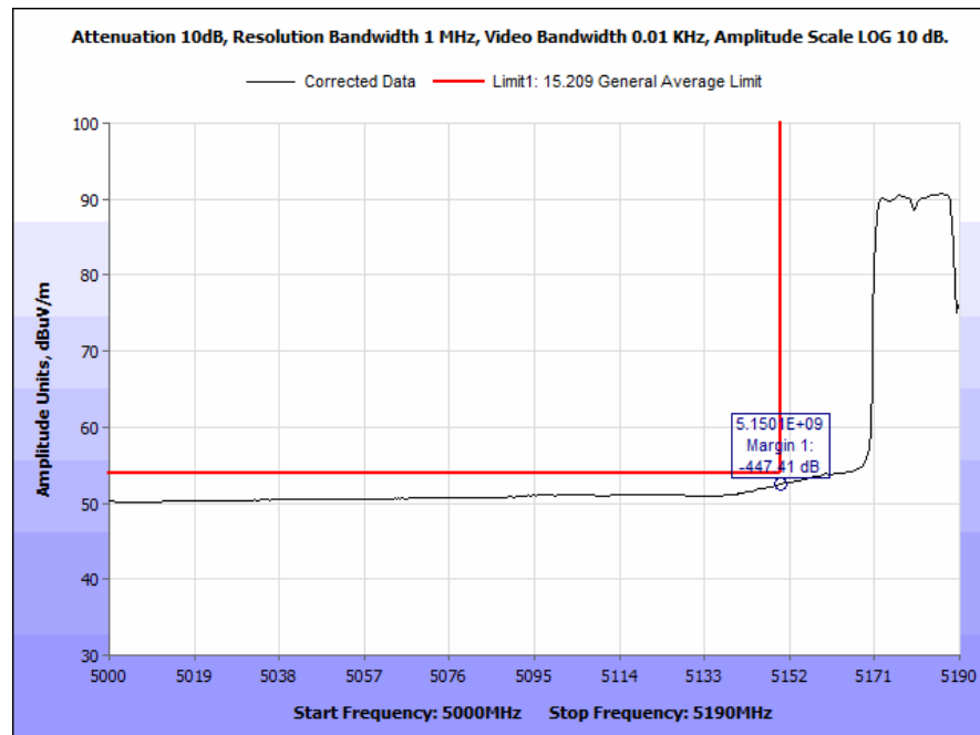
Plot 194. Radiated Band Edge, 802.11a, 40 MHz, Low Channel, 7 dBi Antenna, Average
