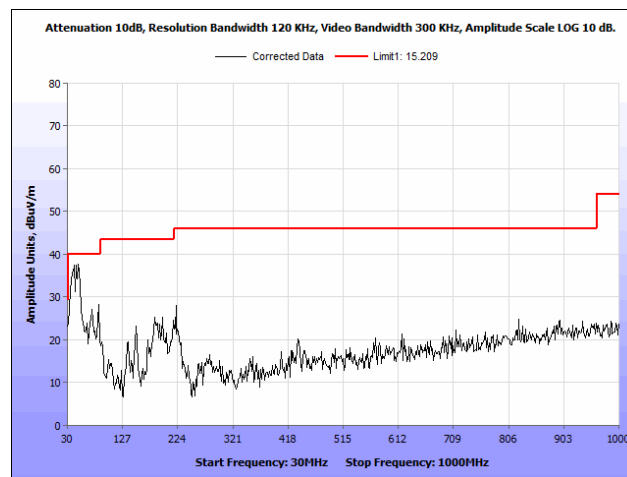
Plot 123. Radiated Spurious Emissions, 802.11a, 40 MHz, High Channel, 30 MHz – 1 GHz, Patch Antenna
