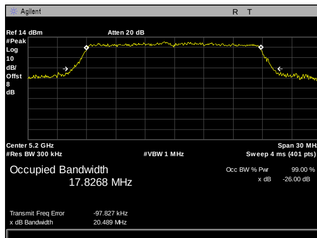
Plot 25. 26 dB Occupied Bandwidth, 802.11n, Port 2, 5200 MHz
