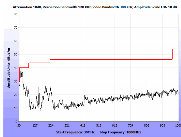
Plot 104. Radiated Spurious Emissions, 802.11ac, 80 MHz, 30 MHz – 1 GHz, Omni Antenna
