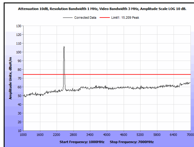
Plot 233. Radiated Spurs, Co-Location, 802.11n 20 MHz, 2462 MHz & 2462 MHz, 1 GHz – 7 GHz, Peak, Omni
