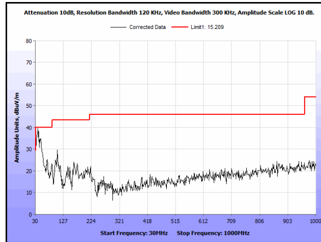
Plot 307. Radiated Spurs, Co-Location, 802.11n 20 MHz, 5300 MHz & 5785 MHz, 30 MHz – 1 GHz, Peak, Omni
