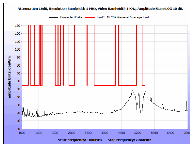
Plot 144. Radiated Spurious Emissions, 802.11n, 40 MHz, High Channel, 1 GHz – 7 GHz, Average, Patch Antenna
