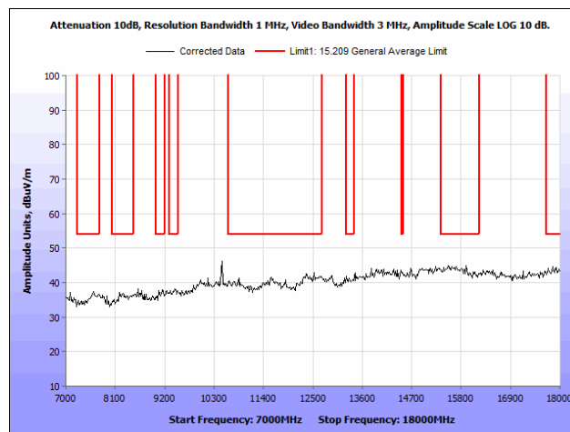
Plot 85. Radiated Spurious Emissions, 802.11a, 20 MHz, High Channel, 7 GHz – 18 GHz, Omni Antenna
