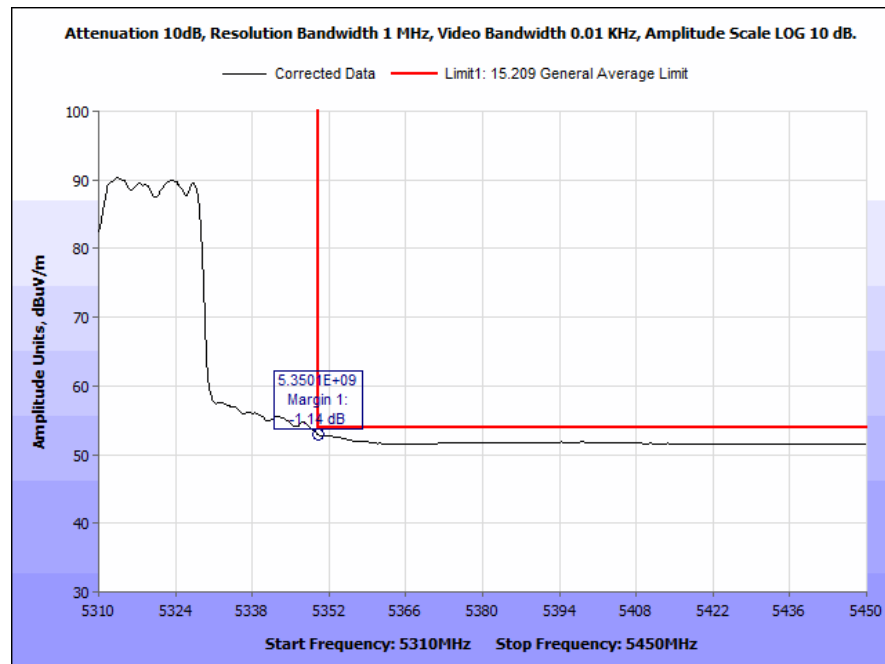
Plot 186. Radiated Band Edge, 802.11n, 40 MHz, High Channel, 4 dBi Antenna, Average
