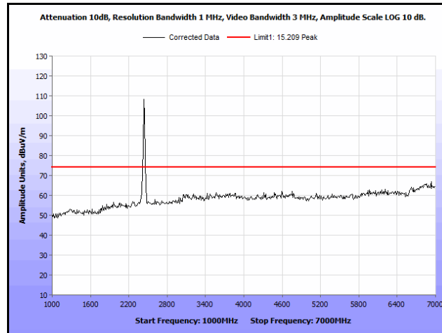
Plot 229. Radiated Spurs, Co-Location, 802.11n 20 MHz, 2437 MHz & 2462 MHz, 1 GHz – 7 GHz, Peak, Omni
