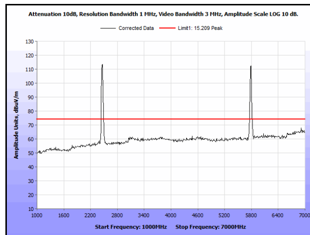
Plot 369. Radiated Spurs, Co-Location, 802.11n 20 MHz, 2462 MHz & 5785 MHz, 1 GHz – 7 GHz, Peak, Patch
