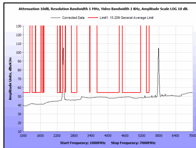
Plot 336. Radiated Spurs, Co-Location, 802.11n 20 MHz, 2412 MHz & 5785 MHz, 1 GHz – 7 GHz, Avg., Patch
