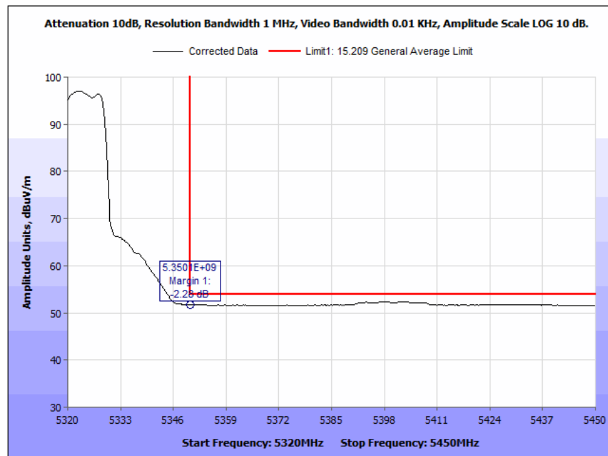
Plot 184. Radiated Band Edge, 802.11n, 20 MHz, High Channel, 4 dBi Antenna, Average
