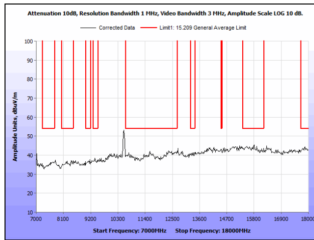
Plot 146. Radiated Spurious Emissions, 802.11n, 40 MHz, High Channel, 7 GHz – 18 GHz, Peak, Patch Antenna
