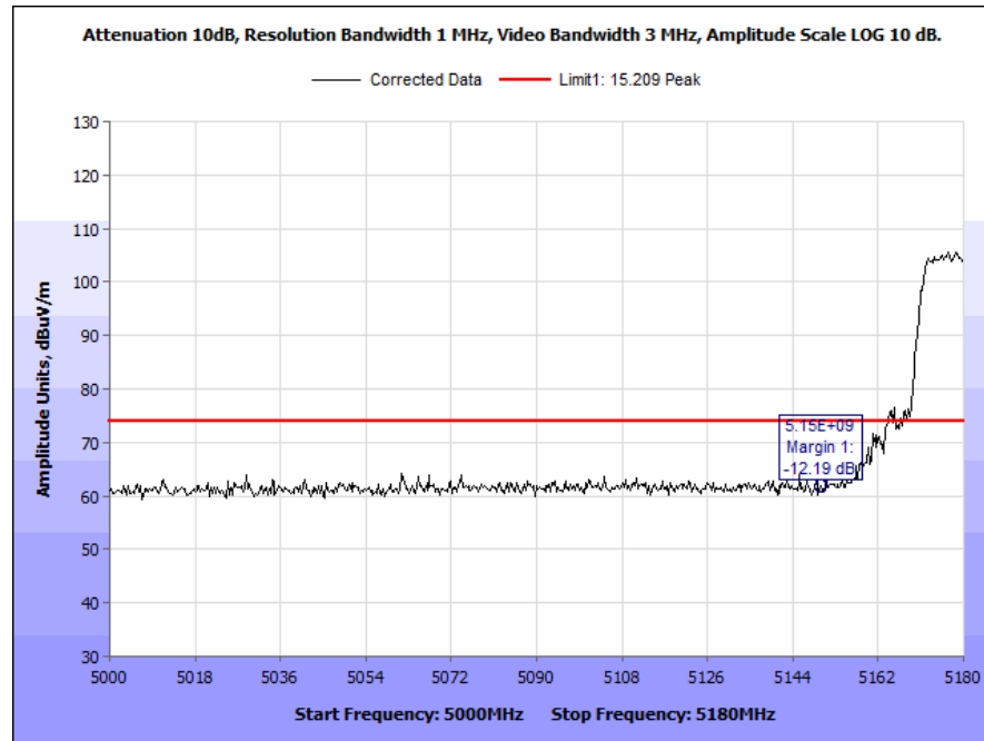
Plot 171. Radiated Band Edge, 802.11a, 20 MHz, Low Channel, 4 dBi Antenna, Peak
