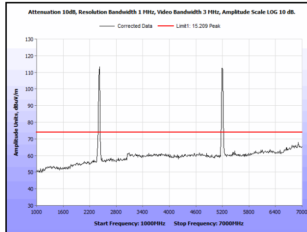
Plot 341. Radiated Spurs, Co-Location, 802.11n 20 MHz, 2437 MHz & 5200 MHz, 1 GHz – 7 GHz, Peak, Patch
