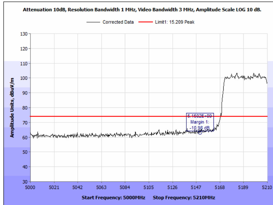
Plot 207. Radiated Band Edge, 802.11ac, 80 MHz, Low Channel, 7 dBi Antenna, Peak
