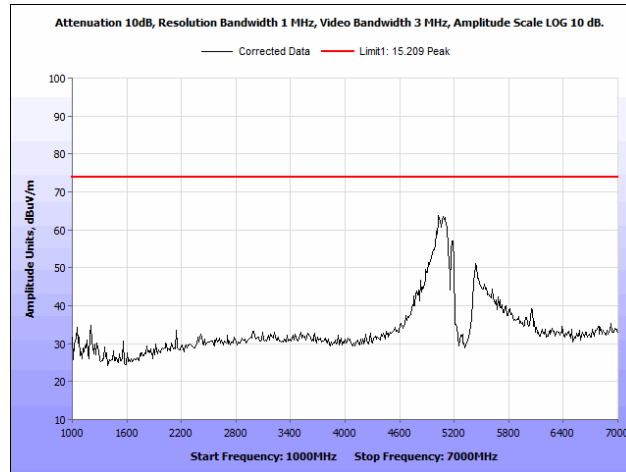
Plot 113. Radiated Spurious Emissions, 802.11a, 40 MHz, Low Channel, 1 GHz – 7 GHz, Peak, Patch Antenna
