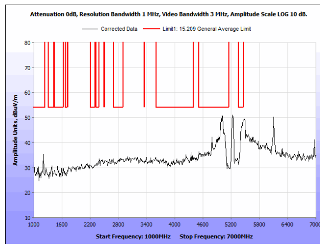
Plot 102. Radiated Spurious Emissions, 802.11n, 40 MHz, High Channel, 1 GHz – 7 GHz, Average, Omni Antenna
