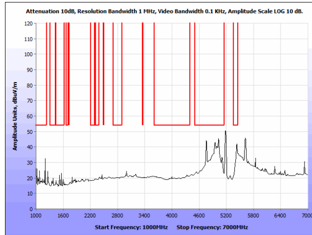
Plot 39. Radiated Spurious Emissions, 802.11a, Mid Channel, 1 GHz – 7 GHz, Average, Ceiling Antenna
