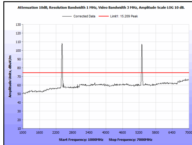
Plot 241. Radiated Spurs, Co-Location, 802.11n 20 MHz, 2412 MHz & 5300 MHz, 1 GHz – 7 GHz, Peak, Omni
