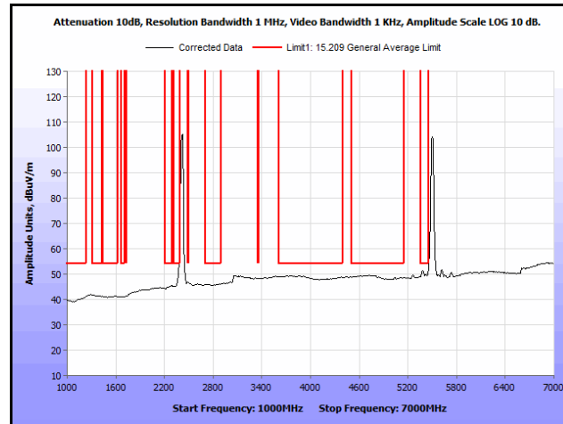
Plot 332. Radiated Spurs, Co-Location, 802.11n 20 MHz, 2412 MHz & 5580 MHz, 1 GHz – 7 GHz, Avg., Patch
