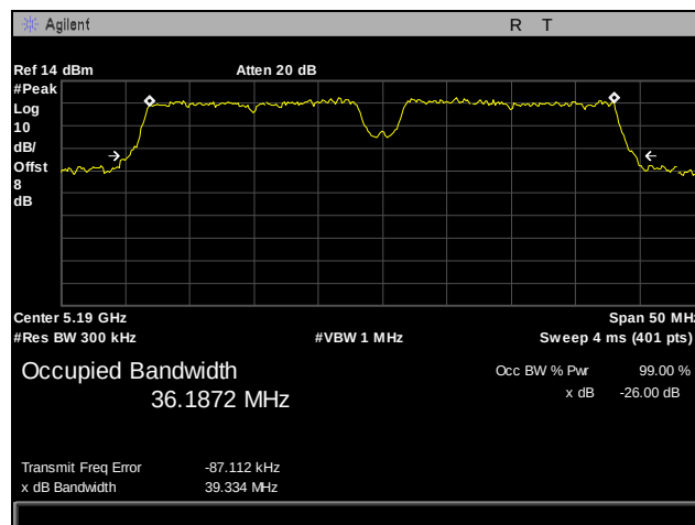
Plot 14. 26 dB Occupied Bandwidth, 802.11a, 5190 MHz
