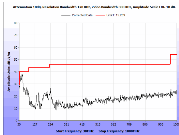
Plot 143. Radiated Spurious Emissions, 802.11n, 40 MHz, High Channel, 30 MHz – 1 GHz, Patch Antenna
