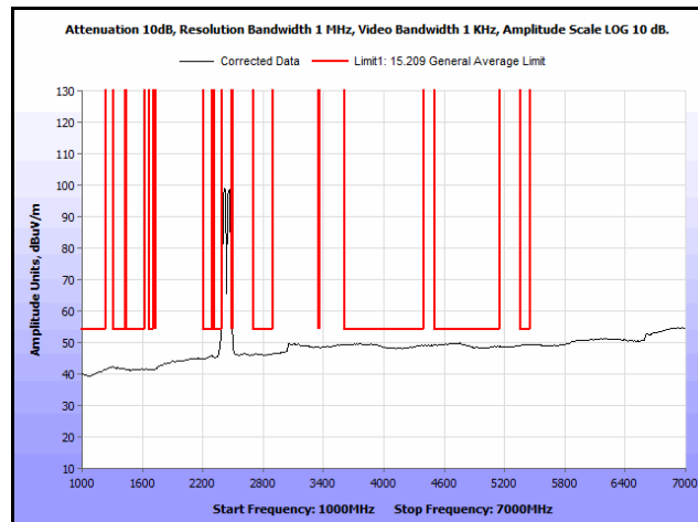
Plot 216. Radiated Spurs, Co-Location, 802.11n 20 MHz, 2412 MHz & 2437 MHz, 1 GHz – 7 GHz, Avg., Omni
