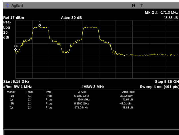
Plot 376. Frequency Stability, 5150 – 5350 MHz, 10°C, 120 V
