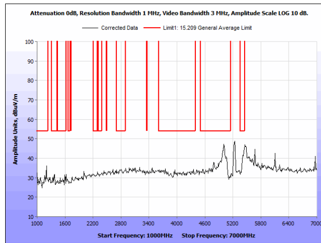
Plot 78. Radiated Spurious Emissions, 802.11a, 40 MHz, Low Channel, 1 GHz – 7 GHz, Average, Omni Antenna
