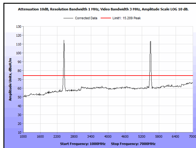
Plot 349. Radiated Spurs, Co-Location, 802.11n 20 MHz, 2437 MHz & 5580 MHz, 1 GHz – 7 GHz, Peak, Patch
