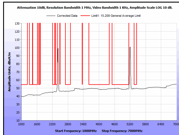
Plot 236. Radiated Spurs, Co-Location, 802.11n 20 MHz, 2412 MHz & 5200 MHz, 1 GHz – 7 GHz, Avg., Omni
