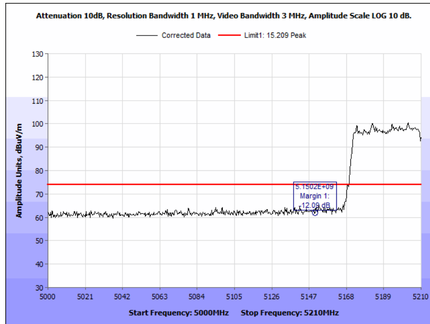
Plot 187. Radiated Band Edge, 802.11ac, 80 MHz, Low Channel, 4 dBi Antenna, Peak
