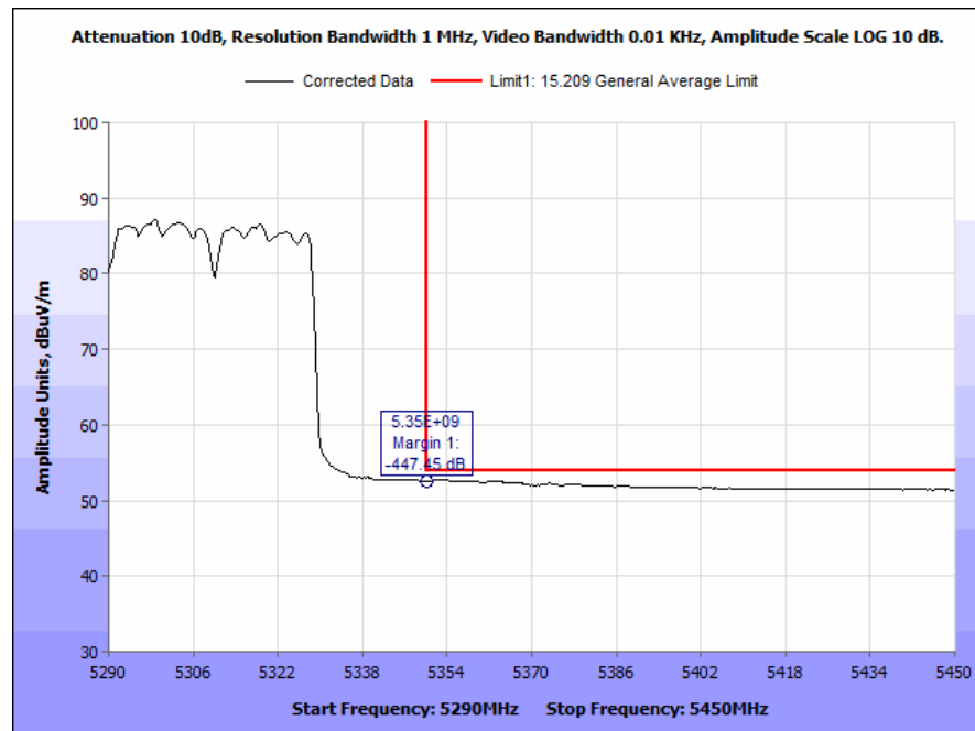
Plot 210. Radiated Band Edge, 802.11ac, 80 MHz, High Channel, 7 dBi Antenna, Average
