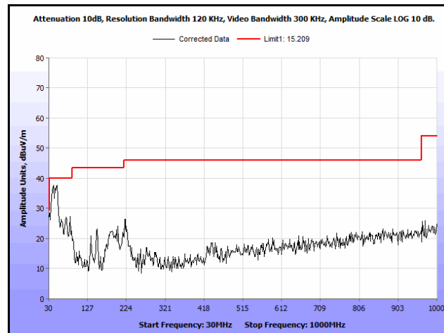
Plot 303. Radiated Spurs, Co-Location, 802.11n 20 MHz, 5300 MHz & 5580 MHz, 30 MHz – 1 GHz, Peak, Omni
