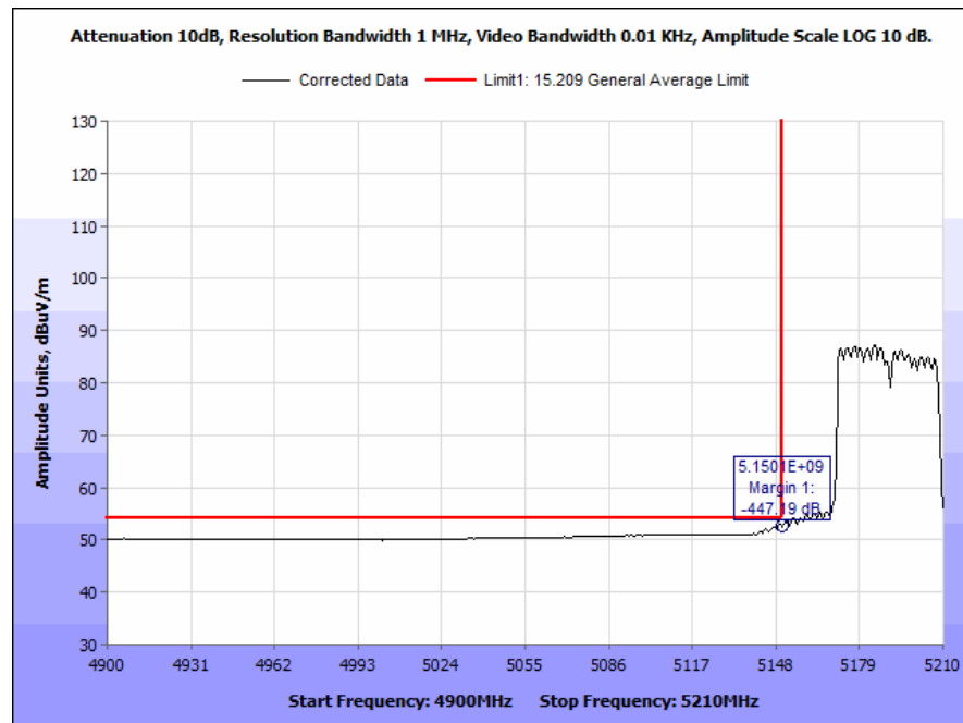
Plot 154. Radiated Band Edge, 802.11a, 40 MHz, Low Channel, 6 dBi Omni Outdoor Antenna, Average
