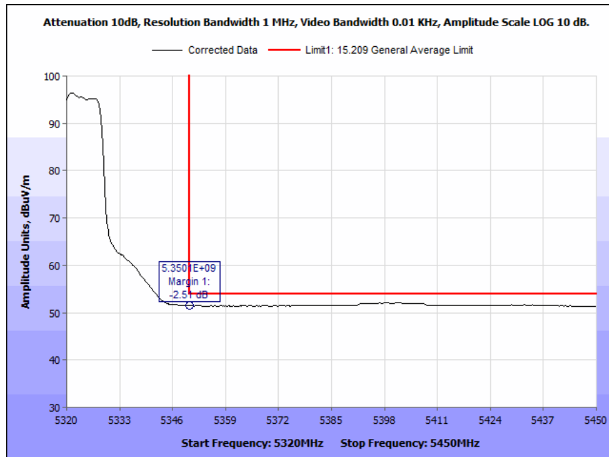
Plot 196. Radiated Band Edge, 802.11a, 20 MHz, High Channel, 7 dBi Antenna, Average
