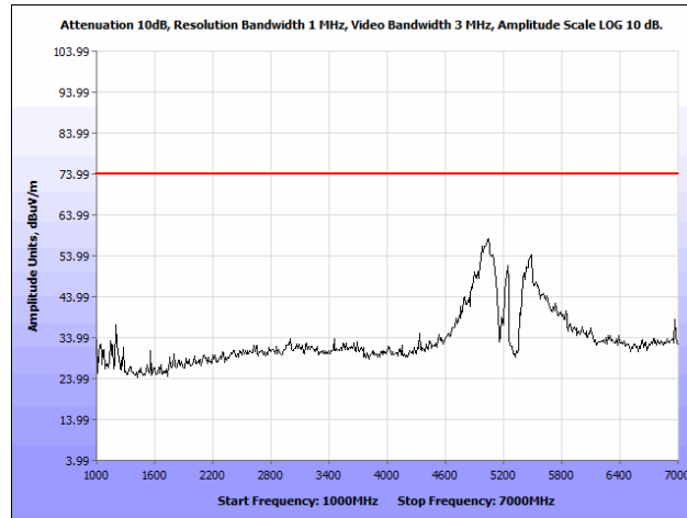
Plot 48. Radiated Spurious Emissions, 802.11a, 40 MHz, High Channel, 1 GHz – 7 GHz, Peak, Ceiling Antenna
