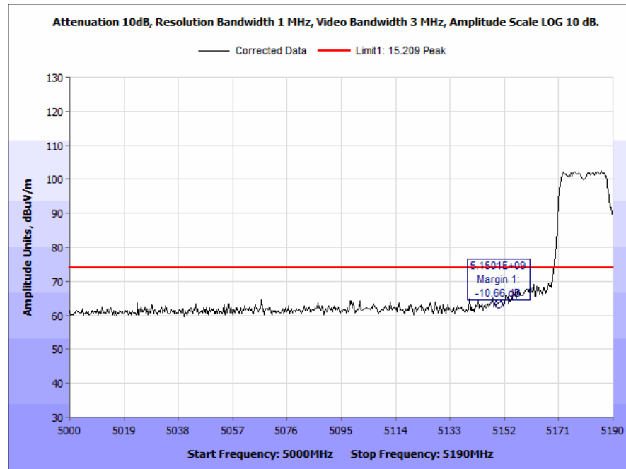
Plot 193. Radiated Band Edge, 802.11a, 40 MHz, Low Channel, 7 dBi Antenna, Peak
