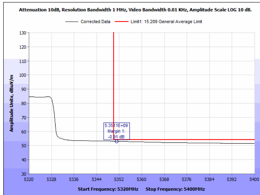
Plot 170. Radiated Band Edge, 802.11ac, 80 MHz, High Channel, 6 dBi Omni Outdoor Antenna, Average
