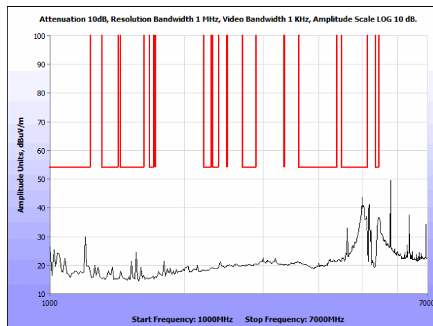
Plot 72. Radiated Spurious Emissions, 802.11ac, 1 GHz – 7 GHz, Peak, Ceiling Antenna
