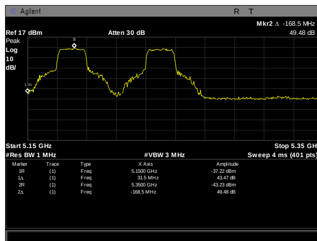
Plot 372. Frequency Stability, 5150 – 5350 MHz, -30°C, 120 V
