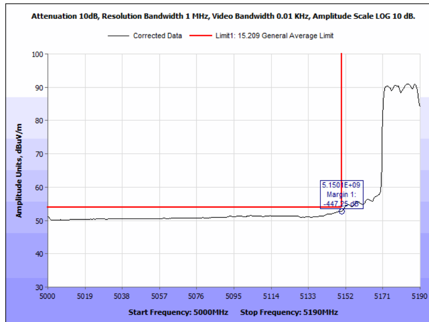
Plot 202. Radiated Band Edge, 802.11n, 40 MHz, Low Channel, 7 dBi Antenna, Average
