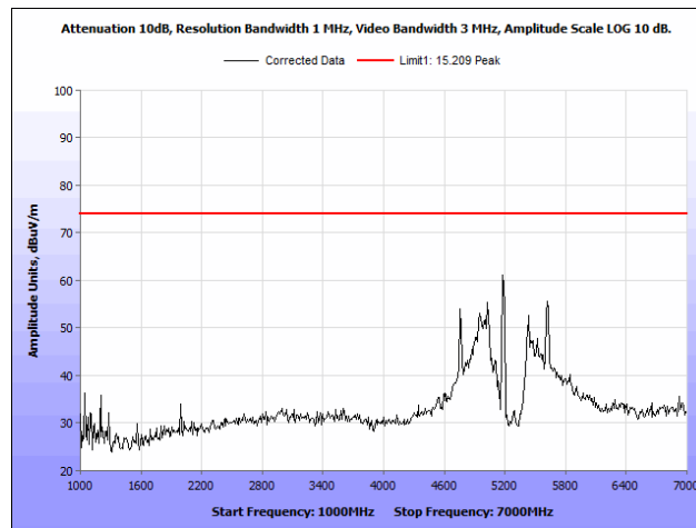
Plot 40. Radiated Spurious Emissions, 802.11a, Mid Channel, 1 GHz – 7 GHz, Peak, Ceiling Antenna
