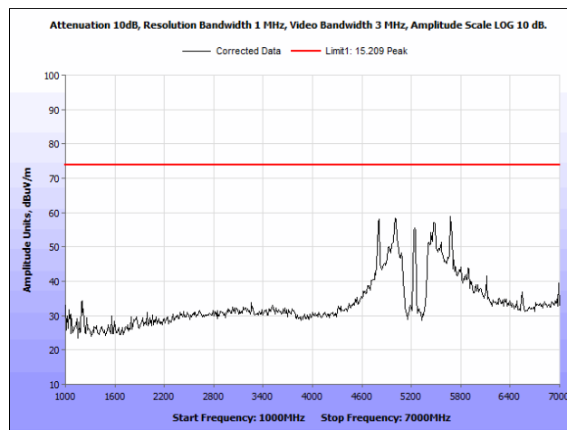
Plot 64. Radiated Spurious Emissions, 802.11n, High Channel, 1 GHz – 7 GHz, Peak, Ceiling Antenna
