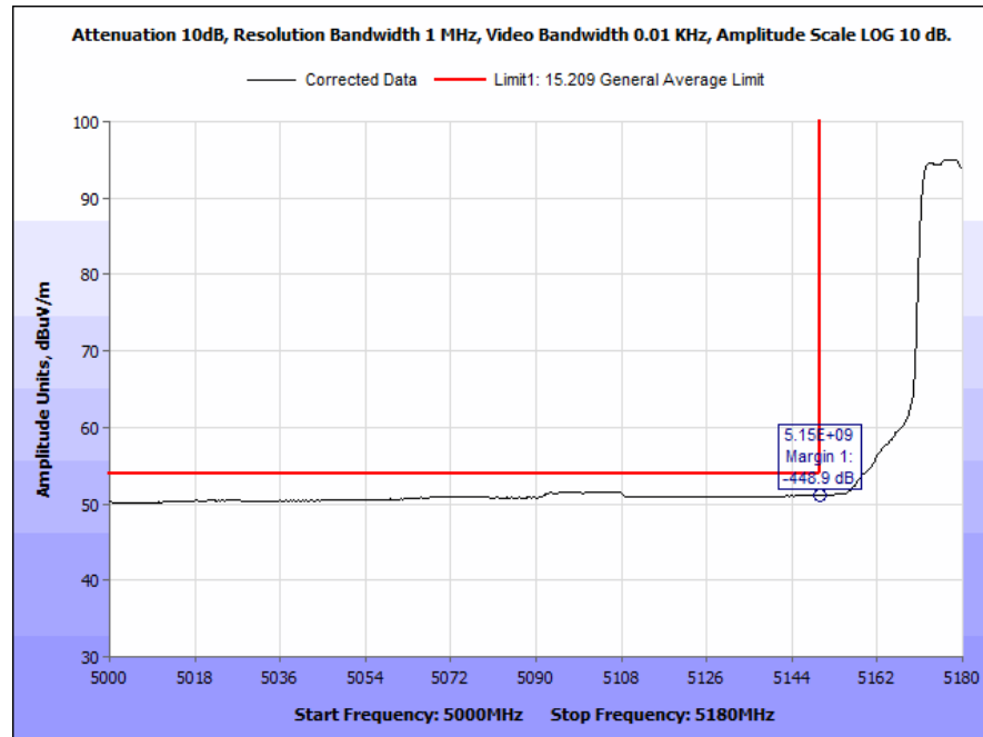
Plot 192. Radiated Band Edge, 802.11a, 20 MHz, Low Channel, 7 dBi Antenna, Average
