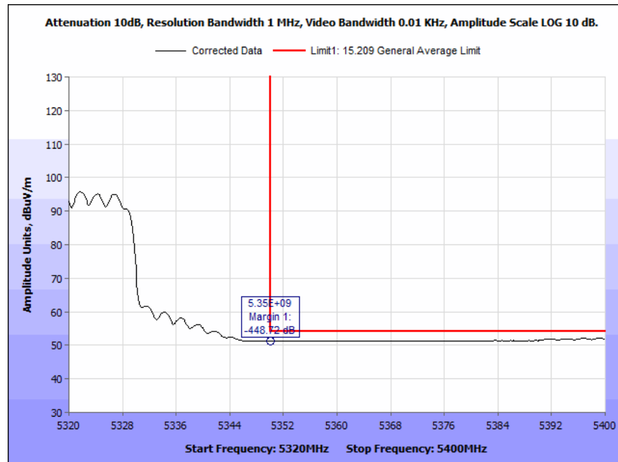
Plot 164. Radiated Band Edge, 802.11n, 20 MHz, High Channel, 6 dBi Omni Outdoor Antenna, Average
