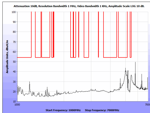
Plot 149. Radiated Spurious Emissions, 802.11ac, 1 GHz – 7 GHz, Peak, Patch Antenna
