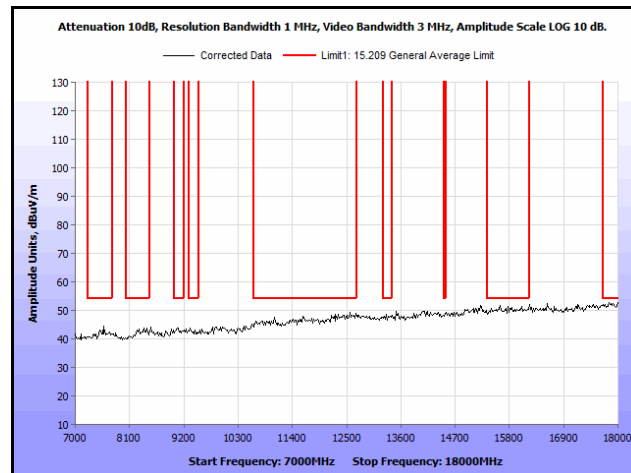
Plot 370. Radiated Spurs, Co-Location, 802.11n 20 MHz, 2462 MHz & 5785 MHz, 7 GHz – 18 GHz, Peak, Patch
