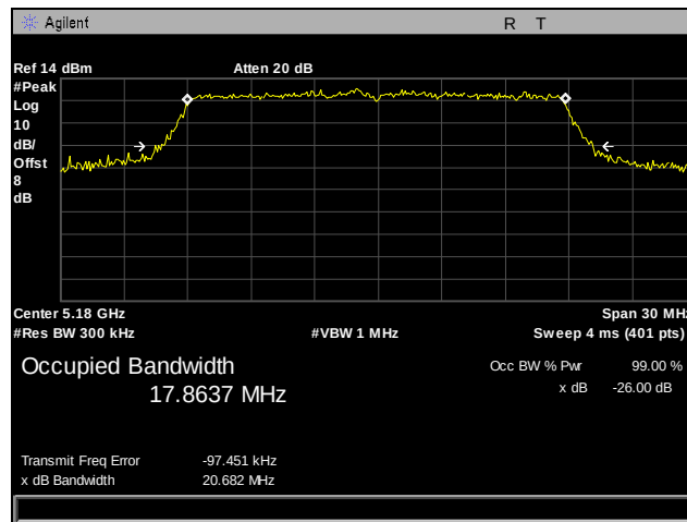
Plot 23. 26 dB Occupied Bandwidth, 802.11n, Port 2, 5180 MHz
