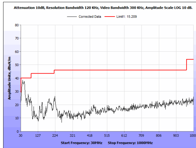
Plot 107. Radiated Spurious Emissions, 802.11a, 20 MHz, Low Channel, 30 MHz – 1 GHz, Patch Antenna
