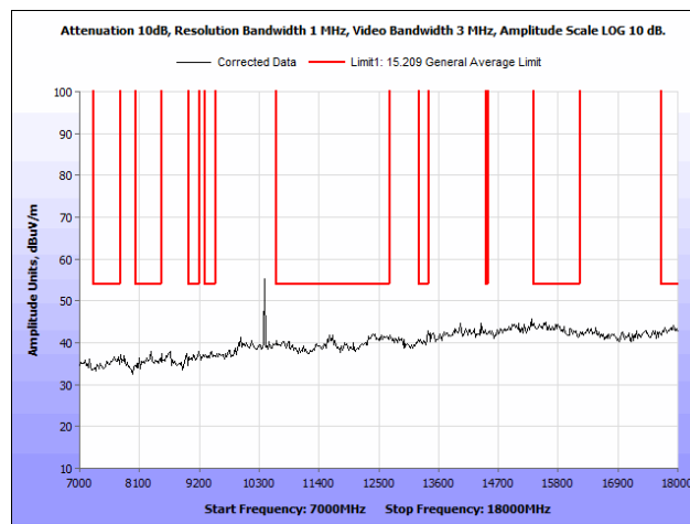
Plot 97. Radiated Spurious Emissions, 802.11n, 20 MHz, Mid Channel, 7 GHz – 18 GHz, Omni Antenna
