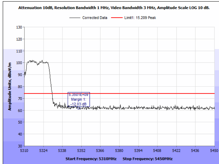
Plot 157. Radiated Band Edge, 802.11a, 40 MHz, Low Channel, 6 dBi Omni Outdoor Antenna, Peak
