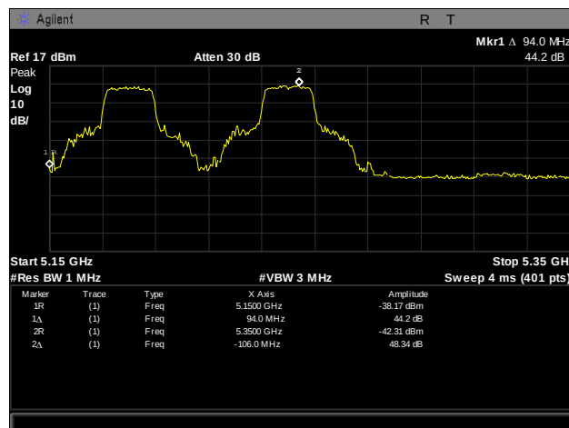
Plot 373. Frequency Stability, 5150 – 5350 MHz, -20°C, 120 V
