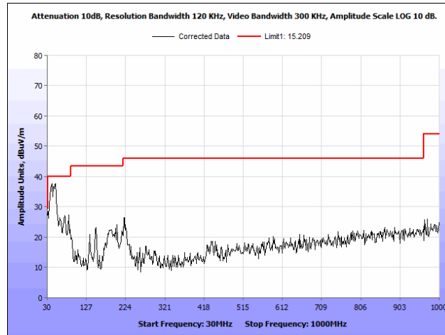
Plot 101. Radiated Spurious Emissions, 802.11n, 40 MHz, High Channel, 30 MHz – 1 GHz, Omni Antenna
