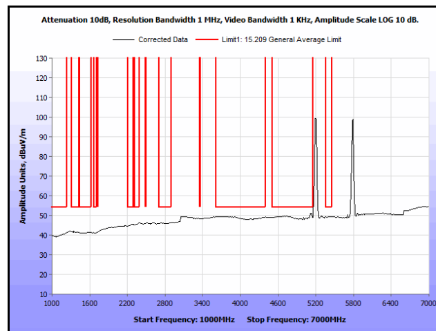
Plot 296. Radiated Spurs, Co-Location, 802.11n 20 MHz, 5200 MHz & 5785 MHz, 1 GHz – 7 GHz, Avg., Omni
