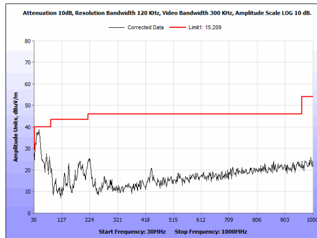
Plot 34. Radiated Spurious Emissions, 802.11a, 40 MHz, Low Channel, 30 MHz – 1 GHz, Ceiling Antenna
