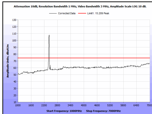
Plot 213. Radiated Spurs, Co-Location, 802.11n 20 MHz, 2412 MHz & 2412 MHz, 1 GHz – 7 GHz, Peak, Omni
