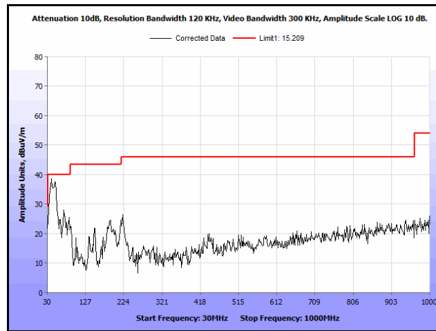
Plot 211. Radiated Spurs, Co-Location, 802.11n 20 MHz, 2412 MHz & 2412 MHz, 30 MHz – 1 GHz, Peak, Omni
