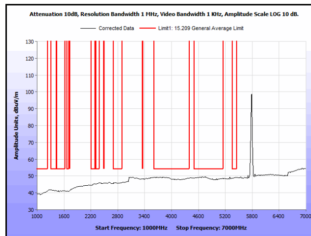
Plot 320. Radiated Spurs, Co-Location, 802.11n 20 MHz, 5785 MHz & 5785 MHz, 1 GHz – 7 GHz, Avg., Omni
