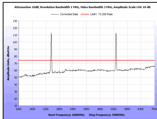
Plot 345. Radiated Spurs, Co-Location, 802.11n 20 MHz, 2437 MHz & 5300 MHz, 1 GHz – 7 GHz, Peak, Patch
