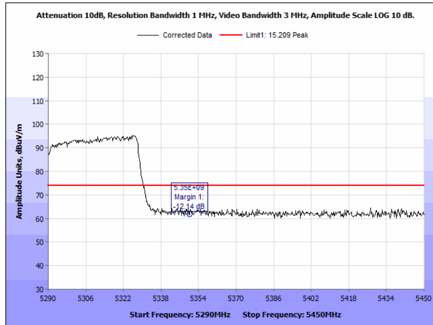
Plot 169. Radiated Band Edge, 802.11ac, 80 MHz, High Channel, 6 dBi Omni Outdoor Antenna, Peak
