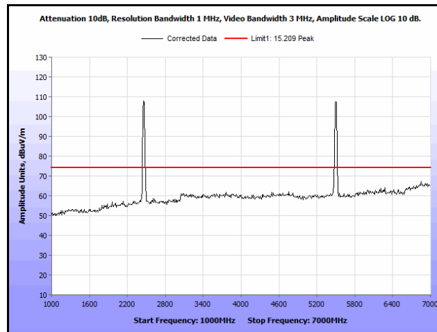
Plot 239. Radiated Spurs, Co-Location, 802.11n 20 MHz, 2462 MHz & 5580 MHz, 1 GHz – 7 GHz, Peak
