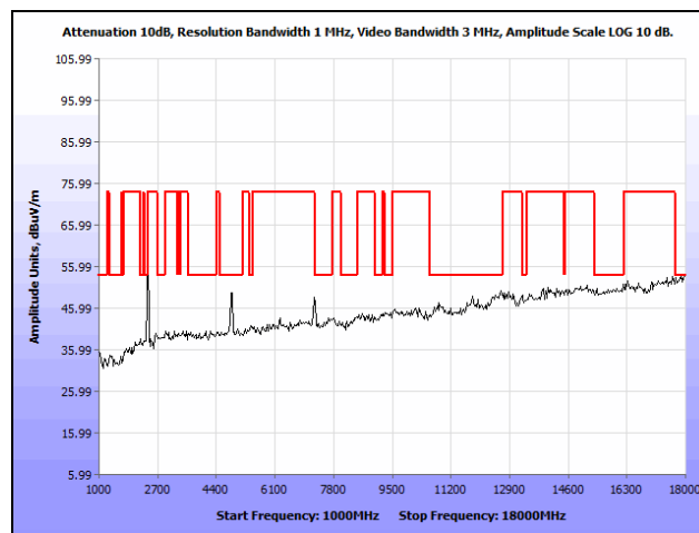
Plot 80. Radiated Spurious Emissions, Low Channel, 802.11n 20 MHz, 1 GHz – 18 GHz
