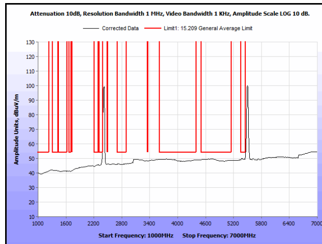
Plot 206. Radiated Spurs, Co-Location, 802.11n 20 MHz, 2412 MHz & 5580 MHz, 1 GHz – 7 GHz, Avg.
