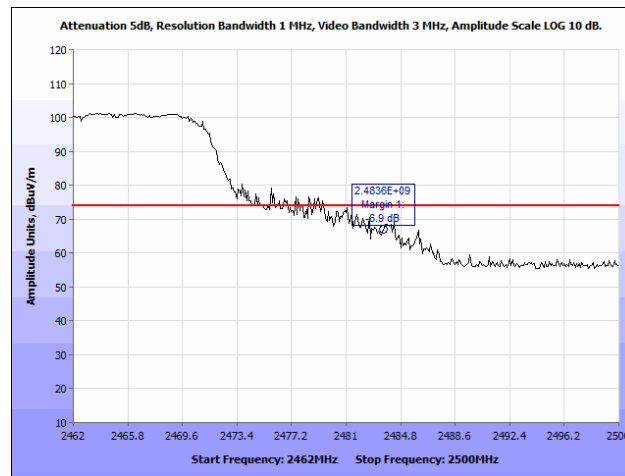
Plot 102. Radiated Restricted Band Edge, 802.11n 20 MHz, 2462 MHz @ 2483.5 MHz, Peak
