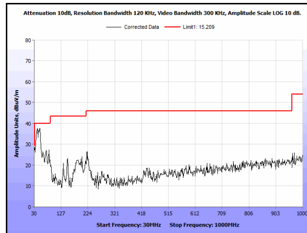
Plot 209. Radiated Spurs, Co-Location, 802.11n 20 MHz, 2412 MHz & 5785 MHz, 30 MHz – 1 GHz, Peak
