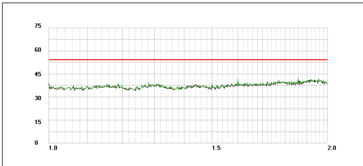
Plot 6. Radiated Emissions, 1 GHz – 2 GHz, PoE
