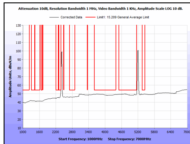
Plot 198. Radiated Spurs, Co-Location, 802.11n 20 MHz, 2412 MHz & 5200 MHz, 1 GHz – 7 GHz, Avg.
