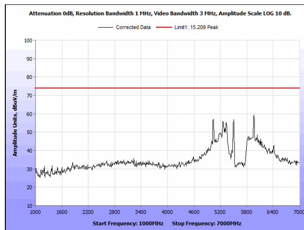
Plot 145. Radiated Spurious Emissions, 802.11n 20 MHz, High Channel, 1 GHz – 7 GHz, Peak
