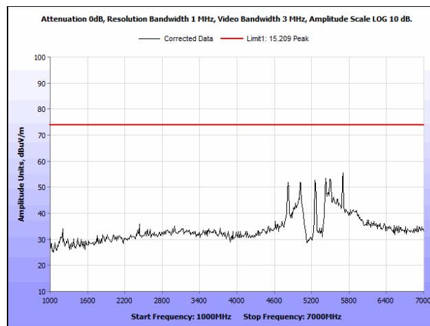
Plot 81. Radiated Spurious Emissions, 802.11a 20 MHz, High Channel, 1 GHz – 7 GHz, Peak
