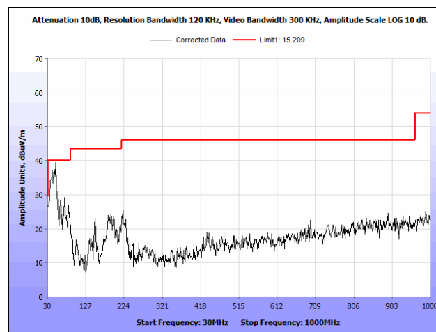
Plot 135. Radiated Spurious Emissions, 802.11n 40 MHz, Low Channel, 30 MHz – 1 GHz
