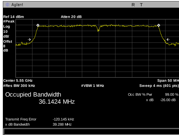
Plot 54. 26 dB Occupied Bandwidth, 802.11n, 5550 MHz, Port 2
