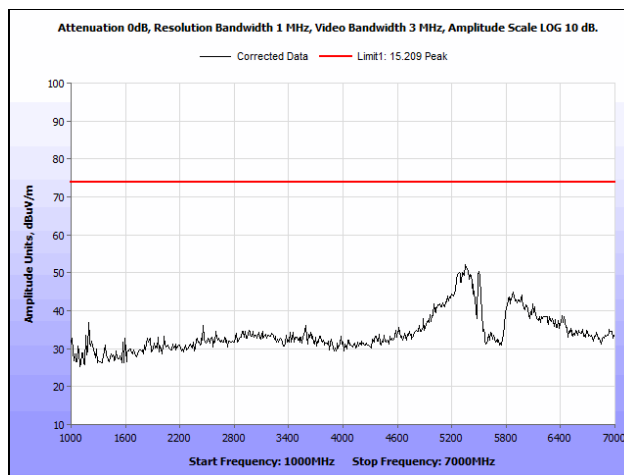
Plot 117. Radiated Spurious Emissions, 802.11a 40 MHz, Low Channel, 1 GHz – 7 GHz, Peak
