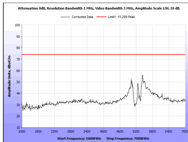
Plot 109. Radiated Spurious Emissions, 802.11ac 80 MHz, 1 GHz – 7 GHz, Peak
