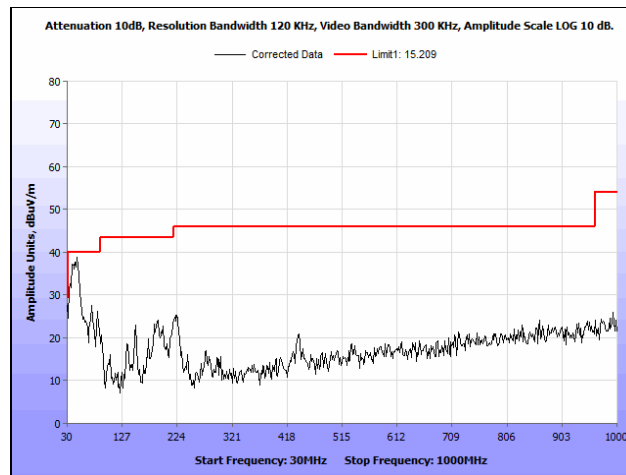
Plot 115. Radiated Spurious Emissions, 802.11a 40 MHz, Low Channel, 30 MHz – 1 GHz
