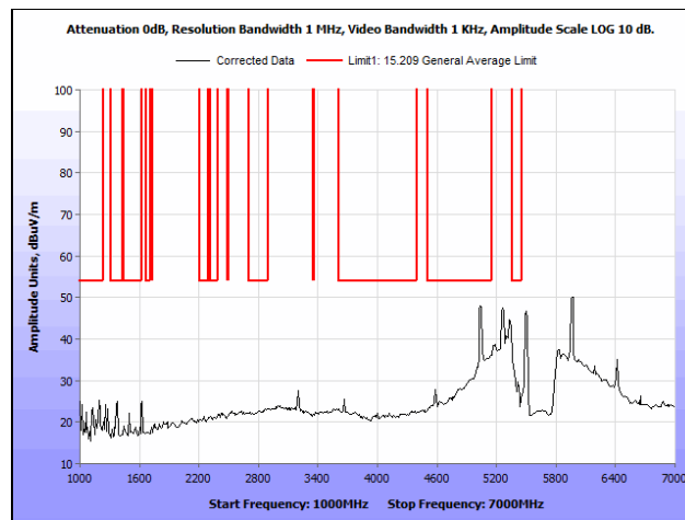
Plot 132. Radiated Spurious Emissions, 802.11n 20 MHz, Low Channel, 1 GHz – 7 GHz, Average
