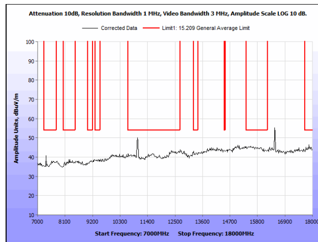
Plot 134. Radiated Spurious Emissions, 802.11n 20 MHz, Low Channel, 7 GHz – 18 GHz
