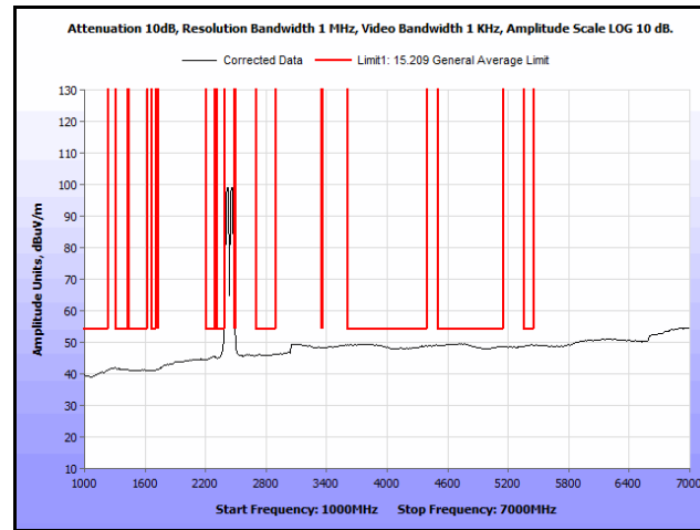
Plot 167. Radiated Spurs, Co-Location, 802.11n 20 MHz, 2412 MHz & 2462 MHz, 1 GHz – 7 GHz, Avg
