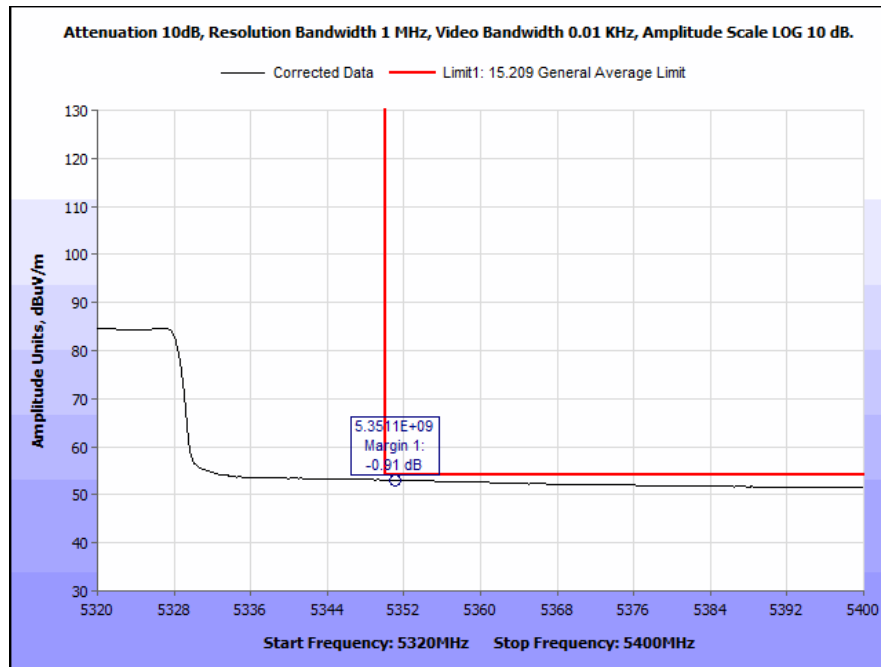
Plot 157. Radiated Band Edge, 802.11ac 80 MHz (5350 MHz), Average
