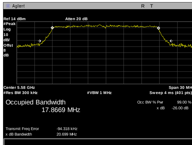
Plot 39. 26 dB Occupied Bandwidth, 802.11n, 5580 MHz, Port 1
