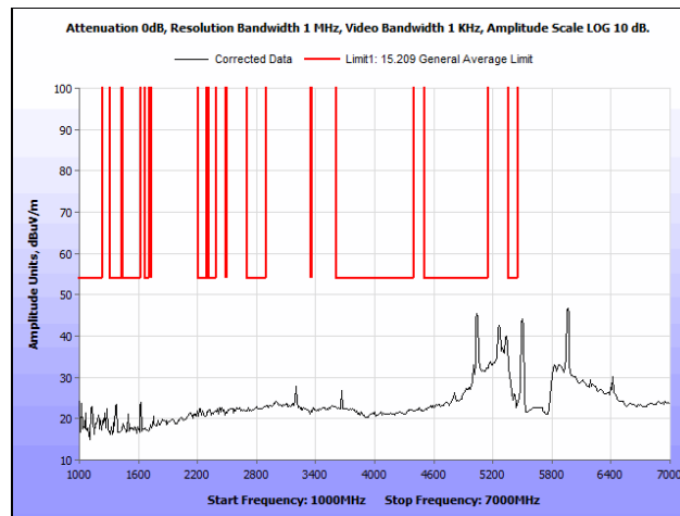
Plot 124. Radiated Spurious Emissions, 802.11a 20 MHz, High Channel, 1 GHz – 7 GHz, Average
