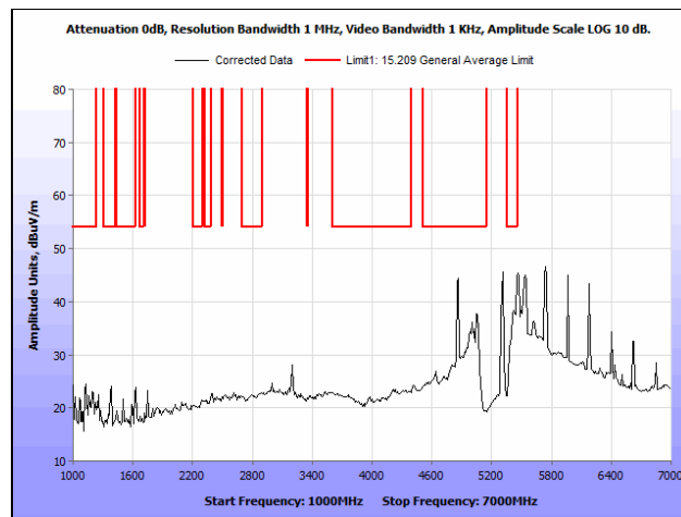
Plot 88. Radiated Spurious Emissions, 802.11n 20 MHz, Low Channel, 1 GHz – 7 GHz, Average
