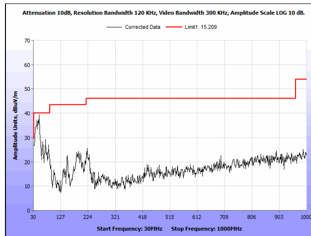
Plot 91. Radiated Spurious Emissions, 802.11n 40 MHz, Low Channel, 30 MHz – 1 GHz
