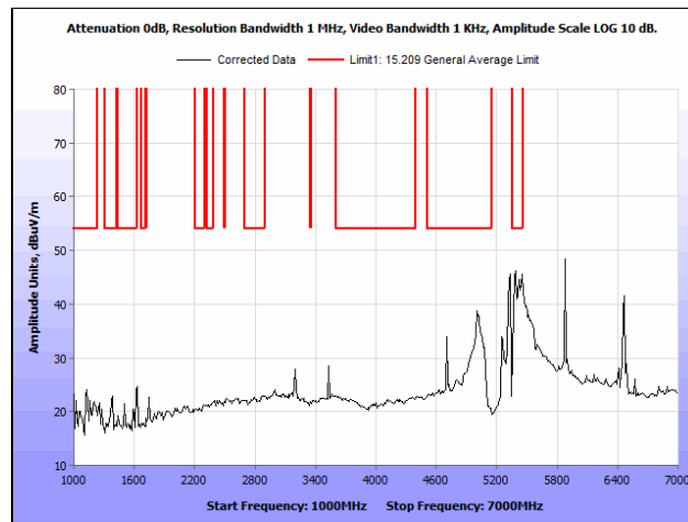
Plot 80. Radiated Spurious Emissions, 802.11a 20 MHz, High Channel, 1 GHz – 7 GHz, Average
