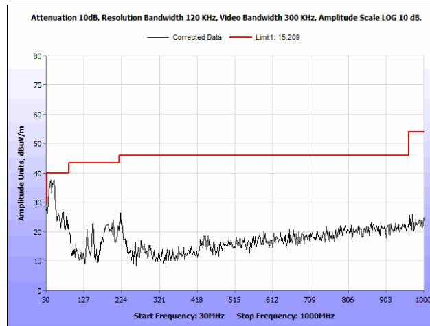
Plot 147. Radiated Spurious Emissions, 802.11n 40 MHz, High Channel, 30 MHz – 1 GHz
