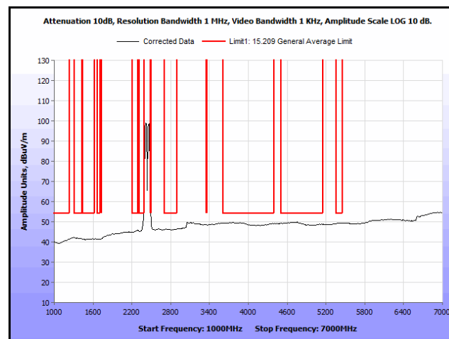
Plot 163. Radiated Spurs, Co-Location, 802.11n 20 MHz, 2412 MHz & 2437 MHz, 1 GHz – 7 GHz, Avg
