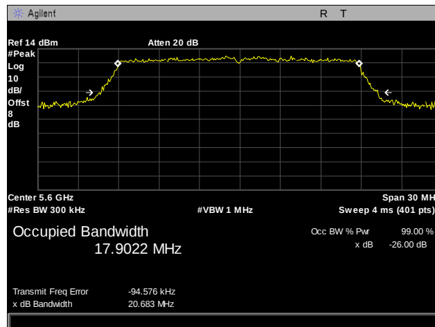
Plot 56. 26 dB Occupied Bandwidth, 802.11n, 5600 MHz, Port 2
