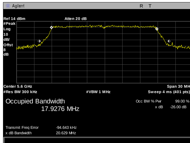
Plot 40. 26 dB Occupied Bandwidth, 802.11n, 5600 MHz, Port 1
