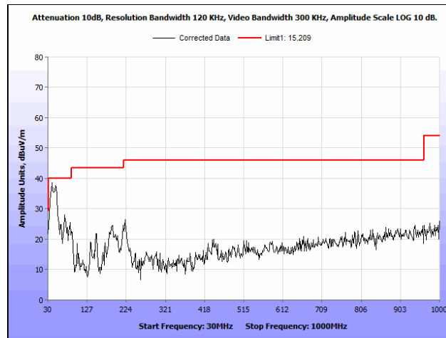
Plot 67. Radiated Spurious Emissions, 802.11a 20 MHz, Low Channel, 30 MHz – 1 GHz
