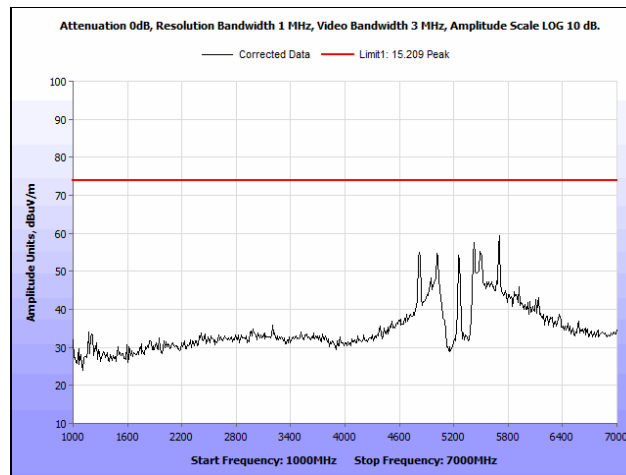
Plot 97. Radiated Spurious Emissions, 802.11n 20 MHz, Mid Channel, 1 GHz – 7 GHz, Peak
