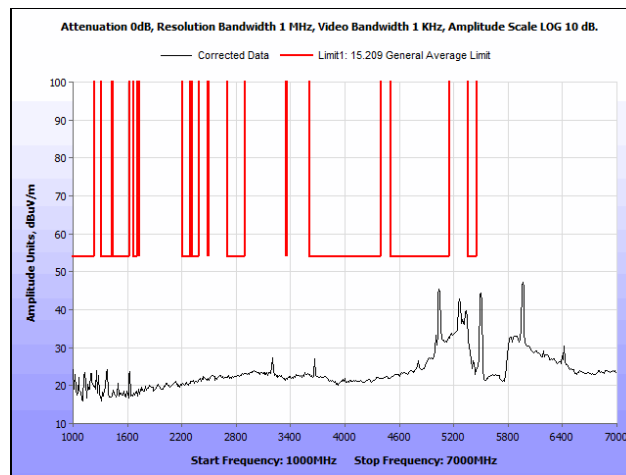
Plot 112. Radiated Spurious Emissions, 802.11a 20 MHz, Low Channel, 1 GHz – 7 GHz, Average
