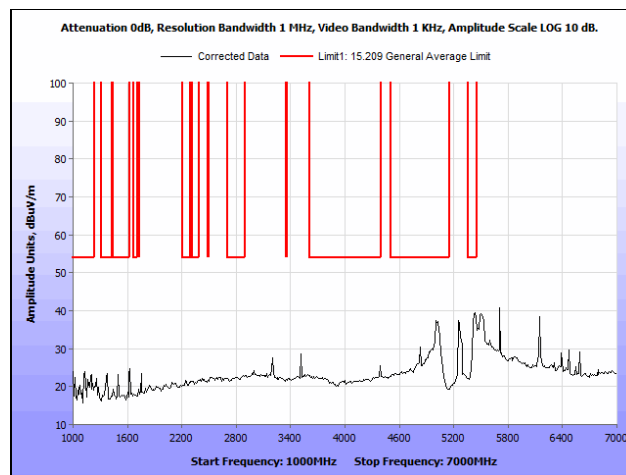
Plot 92. Radiated Spurious Emissions, 802.11n 40 MHz, Low Channel, 1 GHz – 7 GHz, Average
