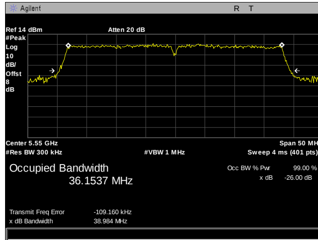
Plot 38. 26 dB Occupied Bandwidth, 802.11n, 5550 MHz, Port 1
