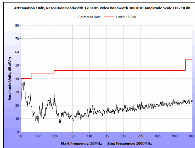
Plot 127. Radiated Spurious Emissions, 802.11a 40 MHz, High Channel, 30 MHz – 1 GHz
