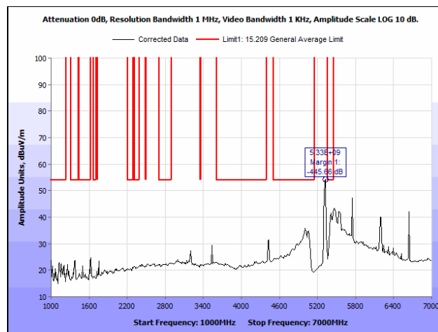
Plot 84. Radiated Spurious Emissions, 802.11a 40 MHz, High Channel, 1 GHz – 7 GHz, Average
