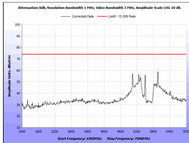
Plot 141. Radiated Spurious Emissions, 802.11n 20 MHz, Mid Channel, 1 GHz – 7 GHz, Peak
