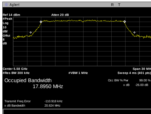
Plot 55. 26 dB Occupied Bandwidth, 802.11n, 5580 MHz, Port 2
