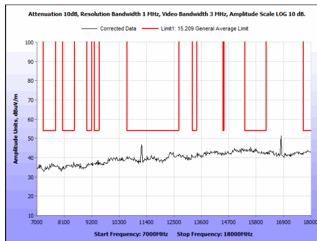
Plot 122. Radiated Spurious Emissions, 802.11a 20 MHz, Mid Channel, 7 GHz – 18 GHz
