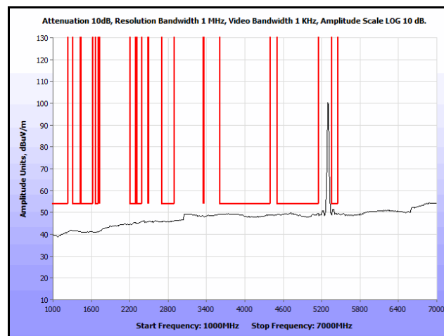
Plot 247. Radiated Spurs, Co-Location, 802.11n 20 MHz, 5300 MHz & 5300 MHz, 1 GHz – 7 GHz, Avg
