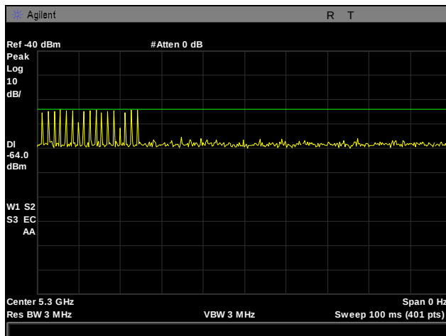
Plot 299. Radar Type 0 Calibration, 5300 MHz
