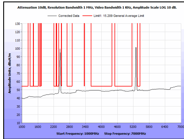
Plot 203. Radiated Spurs, Co-Location, 802.11n 20 MHz, 2437 MHz & 5300 MHz, 1 GHz – 7 GHz, Avg
