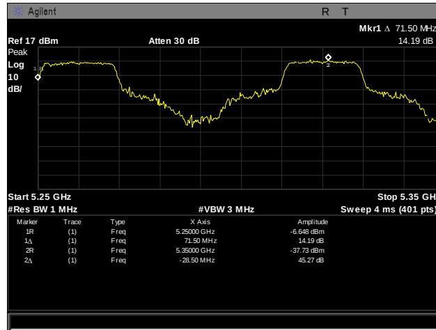
Plot 273. Frequency Stability, 5250 – 5350 MHz, -10°C, 120 V
