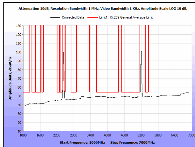
Plot 199. Radiated Spurs, Co-Location, 802.11n 20 MHz, 2437 MHz & 5200 MHz, 1 GHz – 7 GHz, Avg
