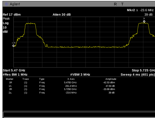
Plot 291. Frequency Stability, 5470 – 5725 MHz, 55°C, 120 V
