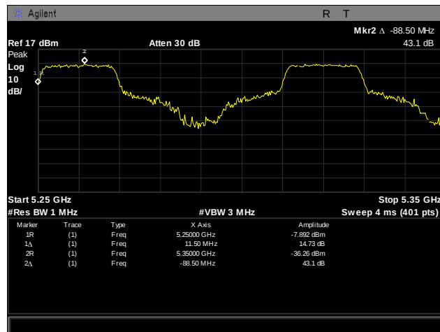
Plot 278. Frequency Stability, 5250 – 5350 MHz, 40°C, 120 V
