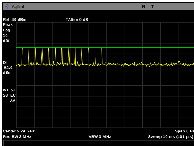
Plot 296. Radar Type 4 Calibration, 5290 MHz
