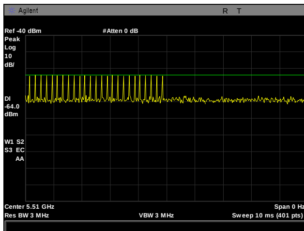
Plot 308. Radar Type 2 Calibration, 5510 MHz
