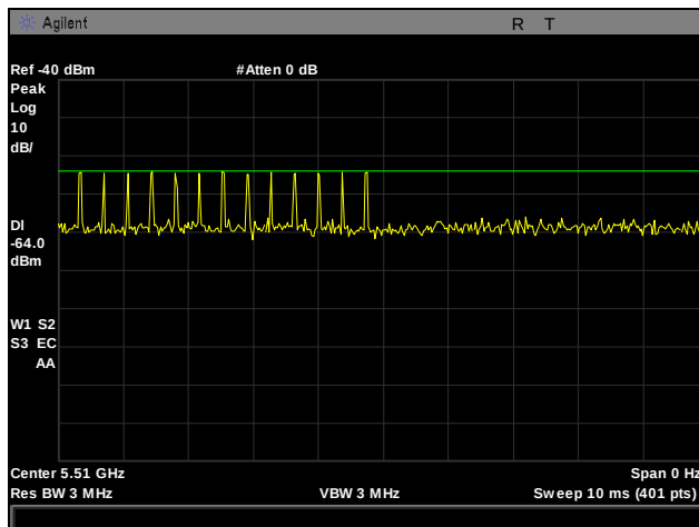
Plot 310. Radar Type 4 Calibration, 5510 MHz
