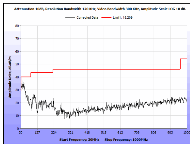
Plot 262. Radiated Spurs, Co-Location, 802.11n 20 MHz, 5580 MHz & 5785 MHz, 30 MHz – 1 GHz, Peak
