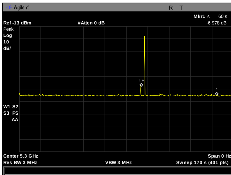
Plot 318. Radar Burst at the End of CACT, 5300 MHz
