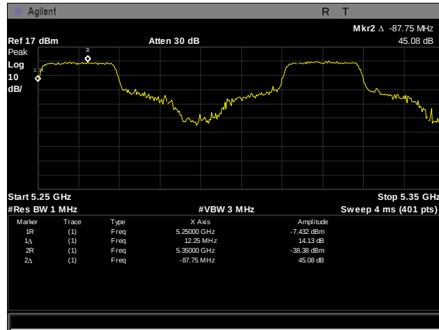
Plot 276. Frequency Stability, 5250 – 5350 MHz, 20°C, 120 V
