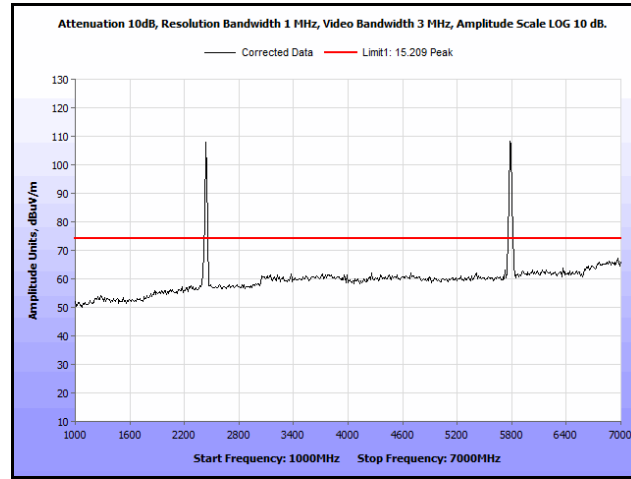
Plot 212. Radiated Spurs, Co-Location, 802.11n 20 MHz, 2437 MHz & 5785 MHz, 1 GHz – 7 GHz, Peak
