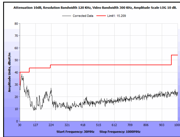
Plot 182. Radiated Spurs, Co-Location, 802.11n 20 MHz, 2412 MHz & 5200 MHz, 30 MHz – 1 GHz, Peak
