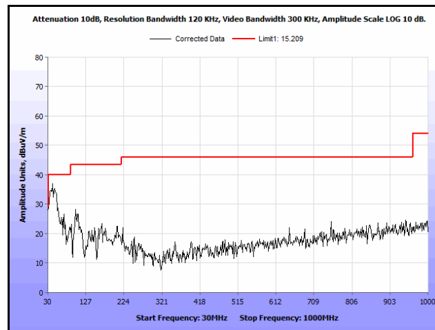
Plot 214. Radiated Spurs, Co-Location, 802.11n 20 MHz, 2462 MHz & 5200 MHz, 30 MHz – 1 GHz, Peak
