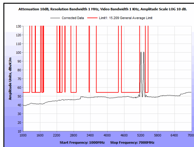
Plot 235. Radiated Spurs, Co-Location, 802.11n 20 MHz, 5200 MHz & 5300 MHz, 1 GHz – 7 GHz, Avg
