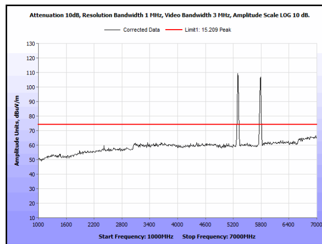
Plot 256. Radiated Spurs, Co-Location, 802.11n 20 MHz, 5300 MHz & 5785 MHz, 1 GHz – 7 GHz, Peak
