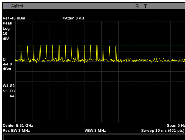
Plot 309. Radar Type 3 Calibration, 5510 MHz
