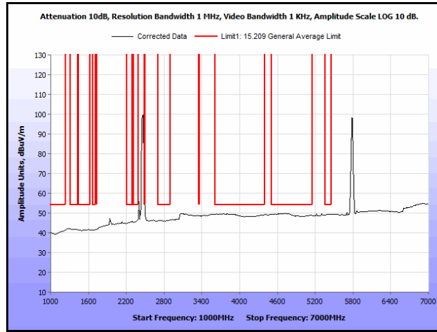
Plot 227. Radiated Spurs, Co-Location, 802.11n 20 MHz, 2462 MHz & 5785 MHz, 1 GHz – 7 GHz, Avg
