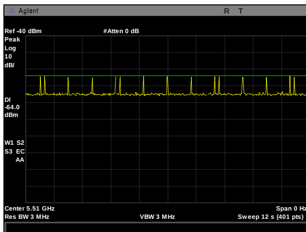
Plot 311. Radar Type 5 Calibration, 5510 MHz
