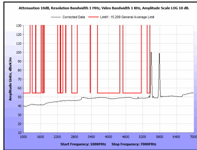
Plot 263. Radiated Spurs, Co-Location, 802.11n 20 MHz, 5580 MHz & 5785 MHz, 1 GHz – 7 GHz, Avg
