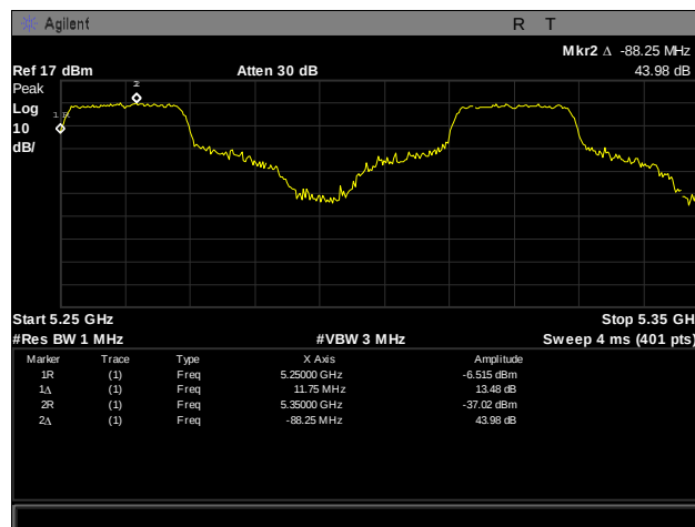
Plot 275. Frequency Stability, 5250 – 5350 MHz, 10°C, 120 V
