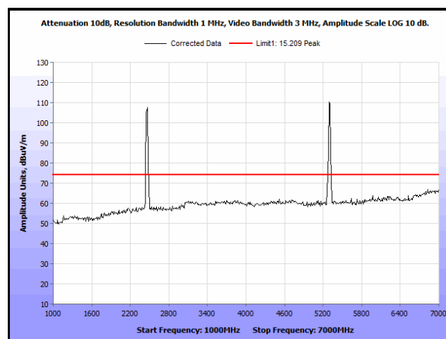
Plot 220. Radiated Spurs, Co-Location, 802.11n 20 MHz, 2462 MHz & 5300 MHz, 1 GHz – 7 GHz, Peak
