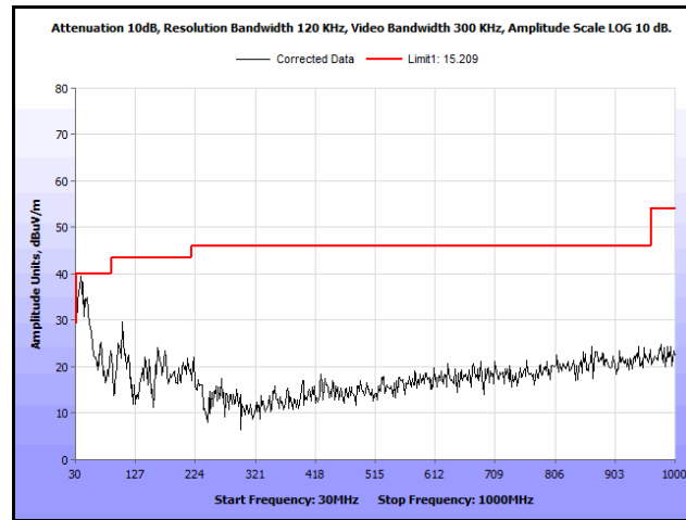
Plot 254. Radiated Spurs, Co-Location, 802.11n 20 MHz, 5300 MHz & 5785 MHz, 30 MHz – 1 GHz, Peak
