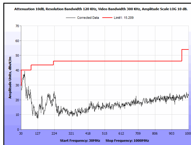
Plot 190. Radiated Spurs, Co-Location, 802.11n 20 MHz, 2412 MHz & 5580 MHz, 30 MHz – 1 GHz, Peak
