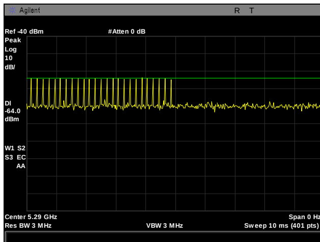
Plot 295. Radar Type 3 Calibration, 5290 MHz
