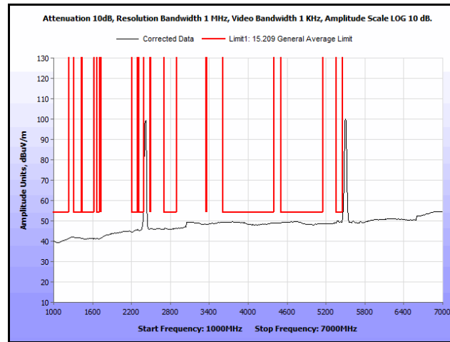
Plot 191. Radiated Spurs, Co-Location, 802.11n 20 MHz, 2412 MHz & 5580 MHz, 1 GHz – 7 GHz, Avg
