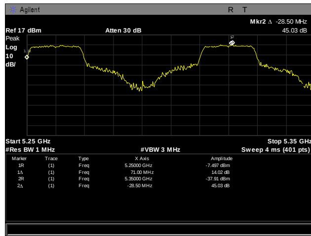
Plot 277. Frequency Stability, 5250 – 5350 MHz, 30°C, 120 V
