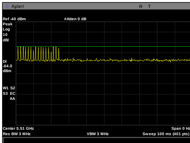
Plot 306. Radar Type 0 Calibration, 5510 MHz
