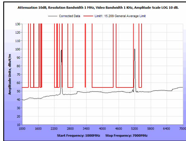
Plot 215. Radiated Spurs, Co-Location, 802.11n 20 MHz, 2462 MHz & 5200 MHz, 1 GHz – 7 GHz, Avg
