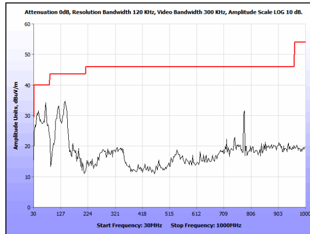
Plot 427. Radiated Spurious Emissions, 802.11n 40 MHz, Low Channel, 30 MHz – 1 GHz, Omni, 5510 MHz
