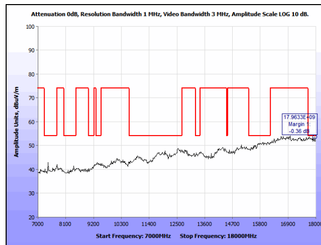
Plot 346. Radiated Spurious Emissions, 802.11n 40 MHz, Mid Channel, 7 GHz – 18 GHz, Patch, 5550 MHz
