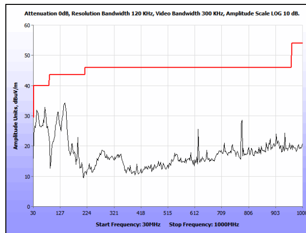
Plot 211. Radiated Spurious Emissions, 802.11a, Mid Channel, 30 MHz – 1 GHz, Patch, 5300 MHz
