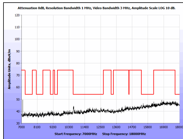
Plot 310. Radiated Spurious Emissions, 802.11n 40 MHz, High Channel, 7 GHz – 18 GHz, Omni, 5310 MHz
