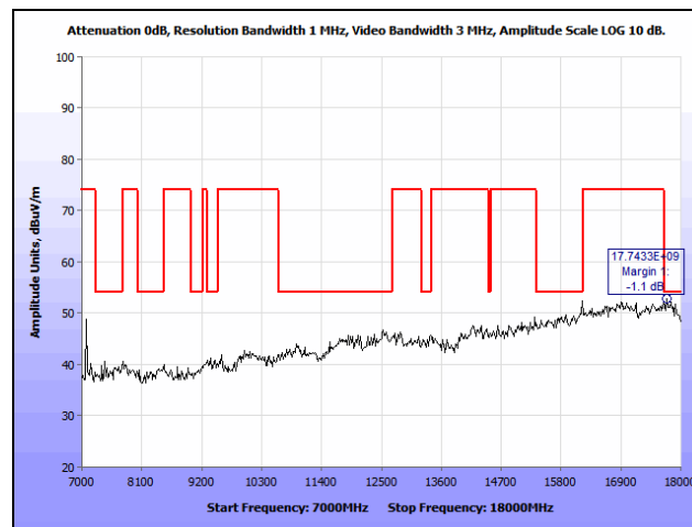
Plot 226. Radiated Spurious Emissions, 802.11n 20 MHz, Mid Channel, 7 GHz – 18 GHz, Patch, 5300 MHz
