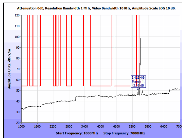
Plot 316. Radiated Spurious Emissions, 802.11a, Low Channel, 1 GHz – 7 GHz, Avg., Patch, 5500 MHz
