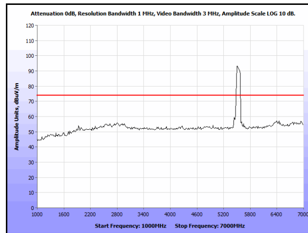
Plot 352. Radiated Spurious Emissions, 802.11n 80 MHz, 1-7 GHz, Patch, Peak, 5530 MHz
