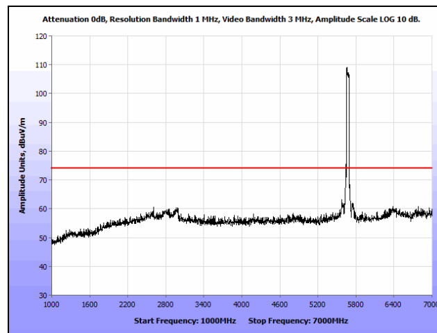
Plot 437. Radiated Spurious Emissions, 802.11n 40 MHz, High Channel, 1 GHz – 7 GHz, Peak, Omni, 5670 MHz
