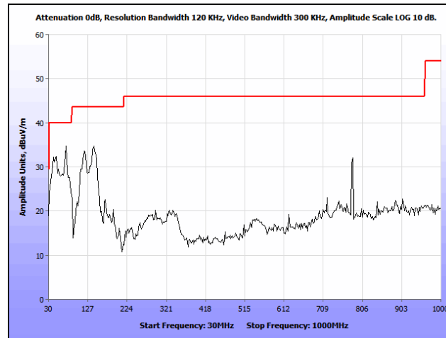
Plot 415. Radiated Spurious Emissions, 802.11n 20 MHz, Low Channel, 30 MHz – 1 GHz, Omni, 5500 MHz
