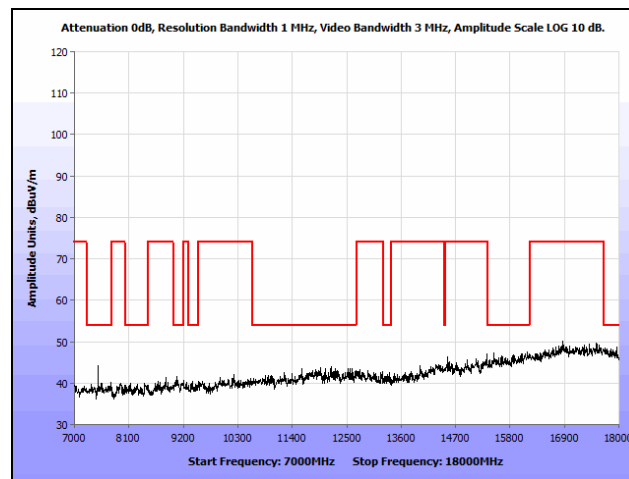
Plot 446. Radiated Spurious Emissions, 802.11n 80 MHz, 7 GHz – 18 GHz, Omni, 5610 MHz
