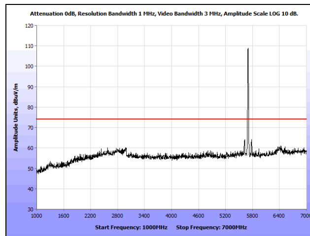
Plot 425. Radiated Spurious Emissions, 802.11n 20 MHz, High Channel, 1 GHz – 7 GHz, Peak, Omni, 5700 MHz
