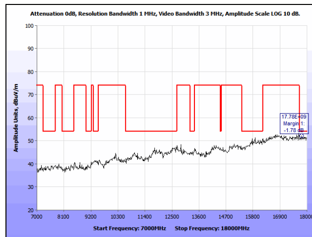
Plot 322. Radiated Spurious Emissions, 802.11a, Mid Channel, 7 GHz – 18 GHz, Patch, 5580 MHz
