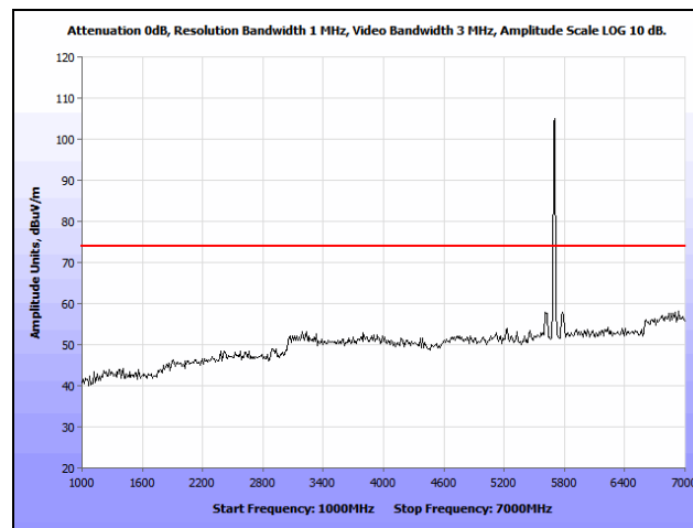
Plot 337. Radiated Spurious Emissions, 802.11n 20 MHz, High Channel, 1 GHz – 7 GHz, Peak, Patch, 5700 MHz
