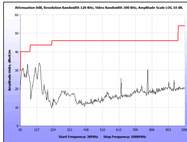
Plot 351. Radiated Spurious Emissions, 802.11n 80 MHz, 30 MHz – 1 GHz, Patch, 5530 MHz
