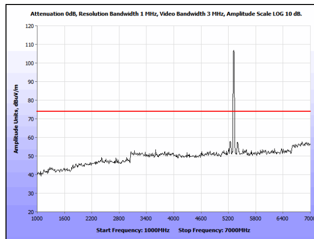
Plot 229. Radiated Spurious Emissions, 802.11n 20 MHz, High Channel, 1 GHz – 7 GHz, Peak, Patch, 5320 MHz
