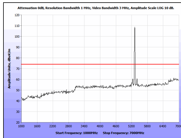
Plot 217. Radiated Spurious Emissions, 802.11a, High Channel, 1 GHz – 7 GHz, Peak, Patch, 5320 MHz
