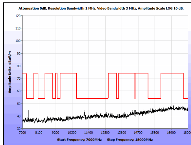
Plot 434. Radiated Spurious Emissions, 802.11n 40 MHz, Mid Channel, 7 GHz – 18 GHz, Omni, 5550 MHz
