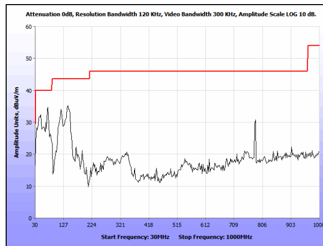
Plot 443. Radiated Spurious Emissions, 802.11n 80 MHz, 30 MHz – 1 GHz, Omni, 5610 MHz
