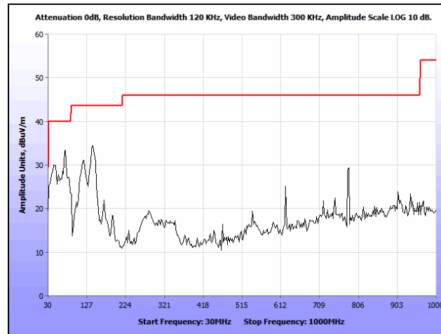
Plot 219. Radiated Spurious Emissions, 802.11n 20 MHz, Low Channel, 30 MHz – 1 GHz, Patch, 5260 MHz
