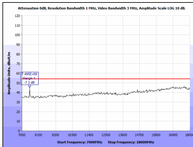
Plot 358. Radiated Spurious Emissions, 802.11n 80 MHz, 7-18 GHz, Patch, 5610 MHz
