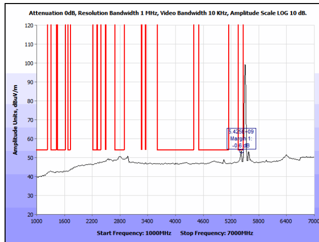
Plot 360. Radiated Spurious Emissions, 802.11a, Low Channel, 1 GHz – 7 GHz, Average, Ceiling, 5500 MHz
