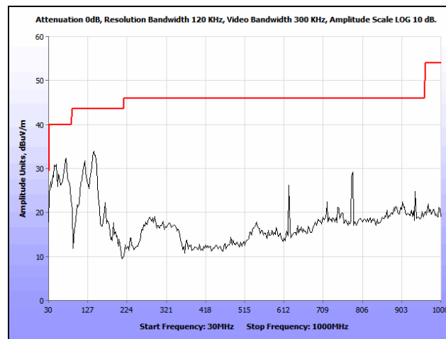
Plot 331. Radiated Spurious Emissions, 802.11n 20 MHz, Mid Channel, 30 MHz – 1 GHz, Patch, 5580 MHz
