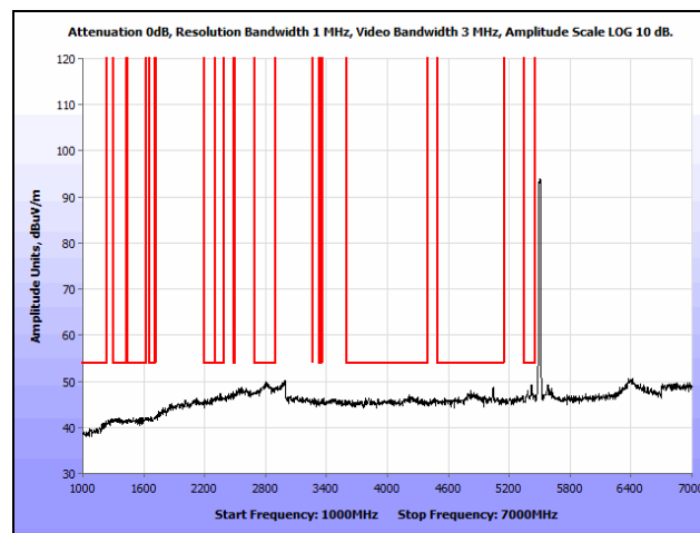
Plot 404. Radiated Spurious Emissions, 802.11a, Low Channel, 1 GHz – 7 GHz, Avg., Omni, 5500 MHz
