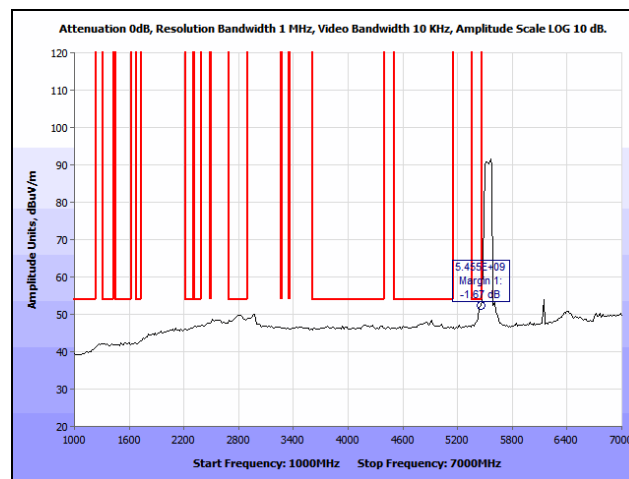
Plot 396. Radiated Spurious Emissions, 802.11n 80 MHz, 1 GHz – 7 GHz, Average, Ceiling, 5530 MHz
