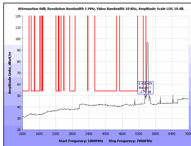
Plot 340. Radiated Spurious Emissions, 802.11n 40 MHz, Low Channel, 1 GHz – 7 GHz, Avg., Patch, 5510 MHz
