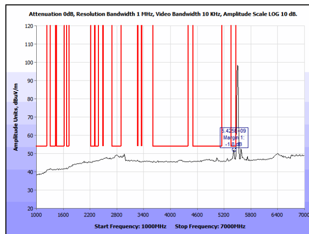
Plot 372. Radiated Spurious Emissions, 802.11n 20 MHz, Low Channel, 1 GHz – 7 GHz, Average, Ceiling, 5500 MHz
