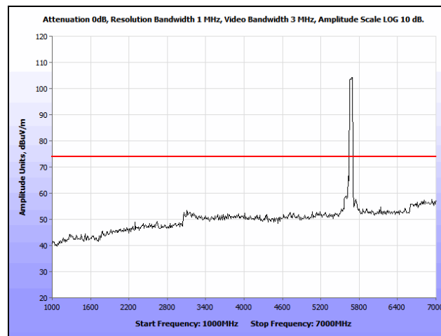
Plot 349. Radiated Spurious Emissions, 802.11n 40 MHz, High Channel, 1 GHz – 7 GHz, Peak, Patch, 5670 MHz
