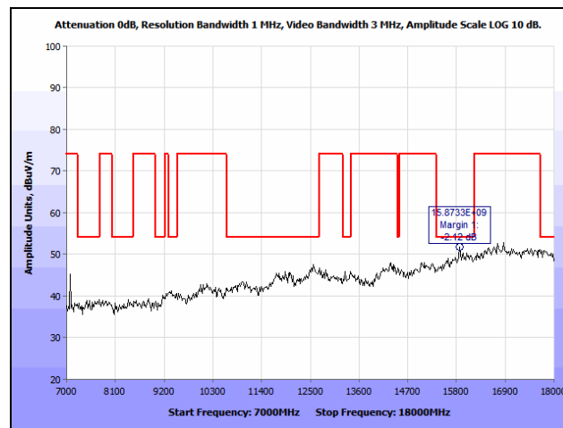
Plot 238. Radiated Spurious Emissions, 802.11n 40 MHz, High Channel, 7 GHz – 18 GHz, Patch, 5310 MHz
