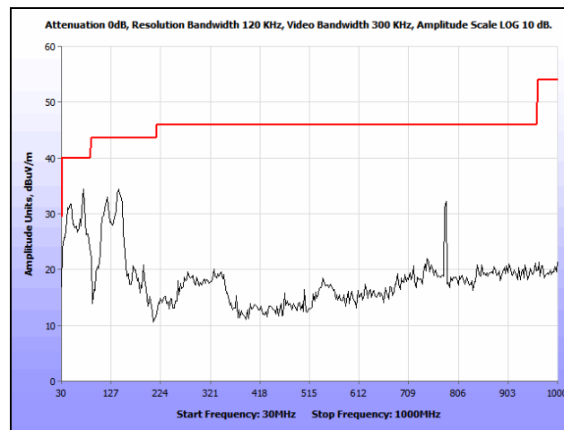
Plot 295. Radiated Spurious Emissions, 802.11n 20 MHz, Mid Channel, 30 MHz – 1 GHz, Omni, 5300 MHz
