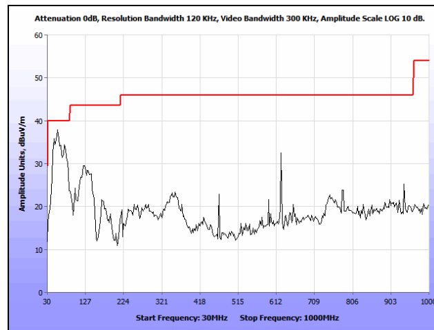
Plot 255. Radiated Spurious Emissions, 802.11n 20 MHz, Low Channel, 30 MHz – 1 GHz, Ceiling, 5260 MHz
