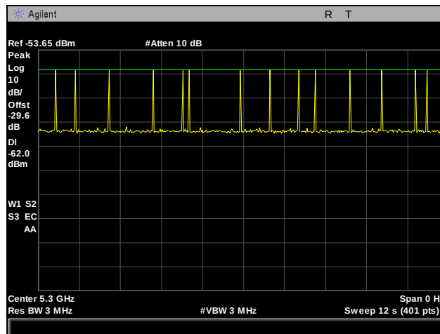
Plot 760. Radar Type 5 Calibration, 5300 MHz
