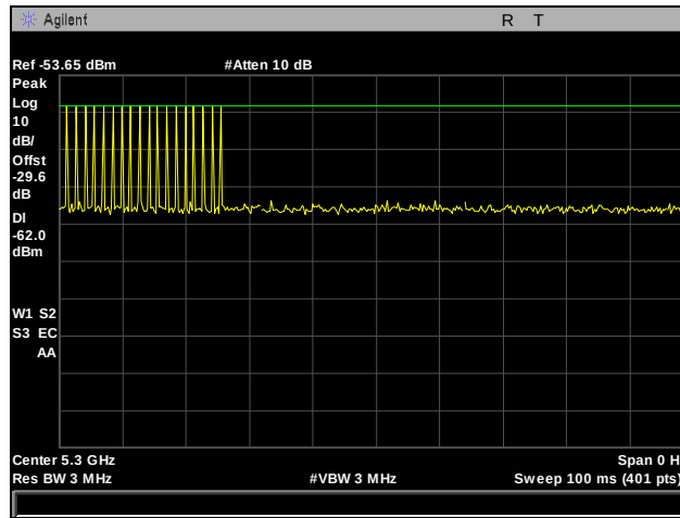
Plot 756. Radar Type 1 Calibration, 5300 MHz
