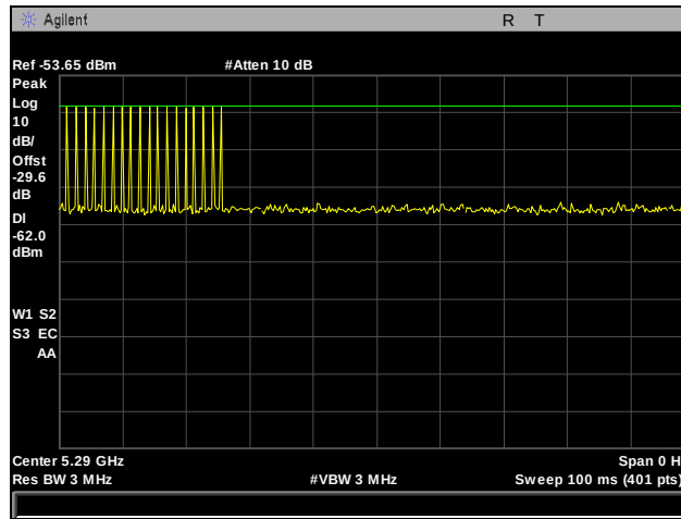
Plot 750. Radar Type 1 Calibration, 5290 MHz
