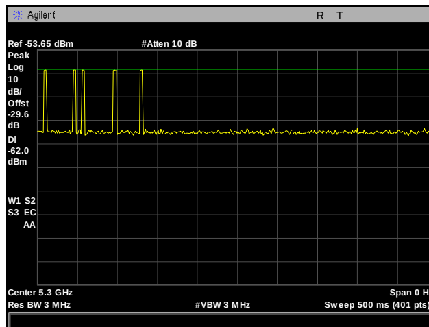
Plot 761. Radar Type 6 Calibration, 5300 MHz
