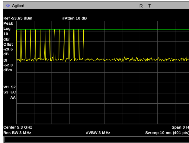
Plot 759. Radar Type 4 Calibration, 5300 MHz
