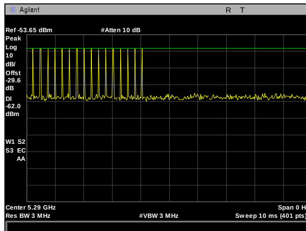
Plot 752. Radar Type 3 Calibration, 5290 MHz
