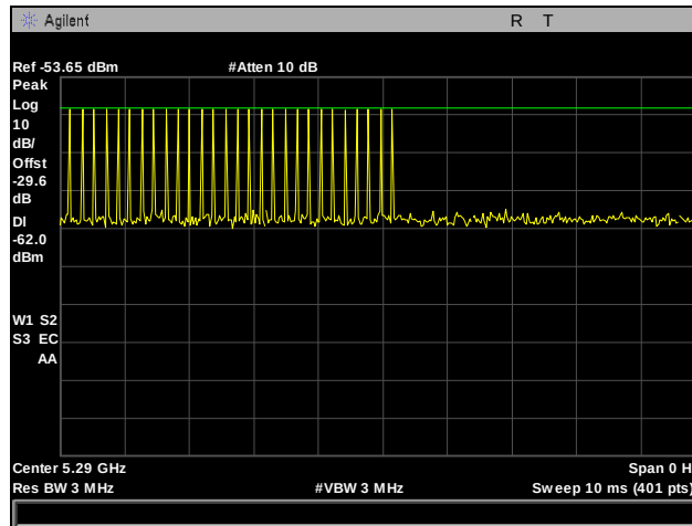
Plot 751. Radar Type 2 Calibration, 5290 MHz
