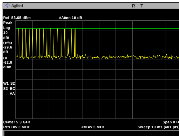
Plot 758. Radar Type 3 Calibration, 5300 MHz
