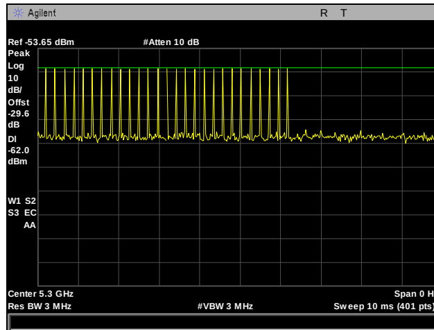
Plot 757. Radar Type 2 Calibration, 5300 MHz
