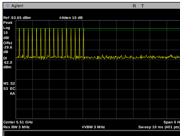
Plot 764. Radar Type 3 Calibration, 5510 MHz
