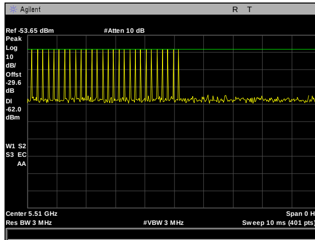
Plot 763. Radar Type 2 Calibration, 5510 MHz
