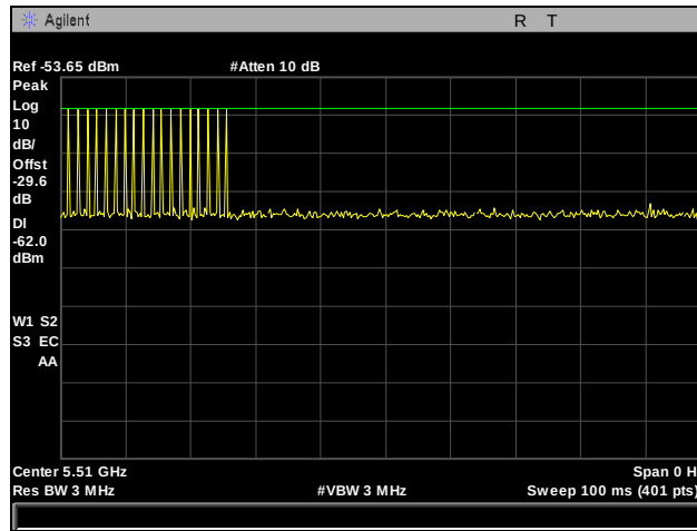
Plot 762. Radar Type 1 Calibration, 5510 MHz
