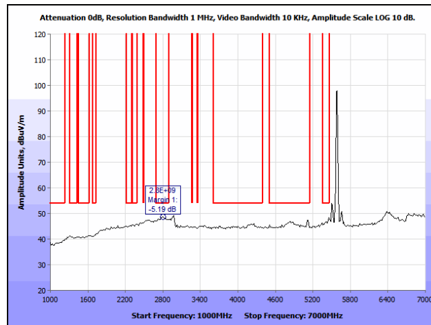
Plot 248. Radiated Spurious Emissions, 802.11a, Mid Channel, 1 GHz – 7 GHz, Avg., Internal, 5580 MHz
