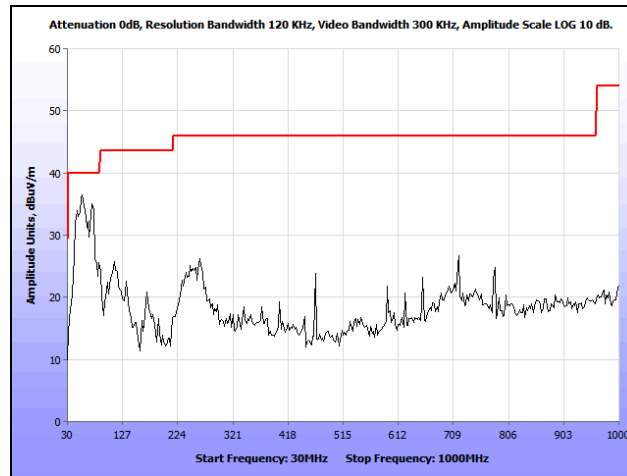
Plot 247. Radiated Spurious Emissions, 802.11a, Mid Channel, 30 MHz – 1 GHz, Internal, 5580 MHz
