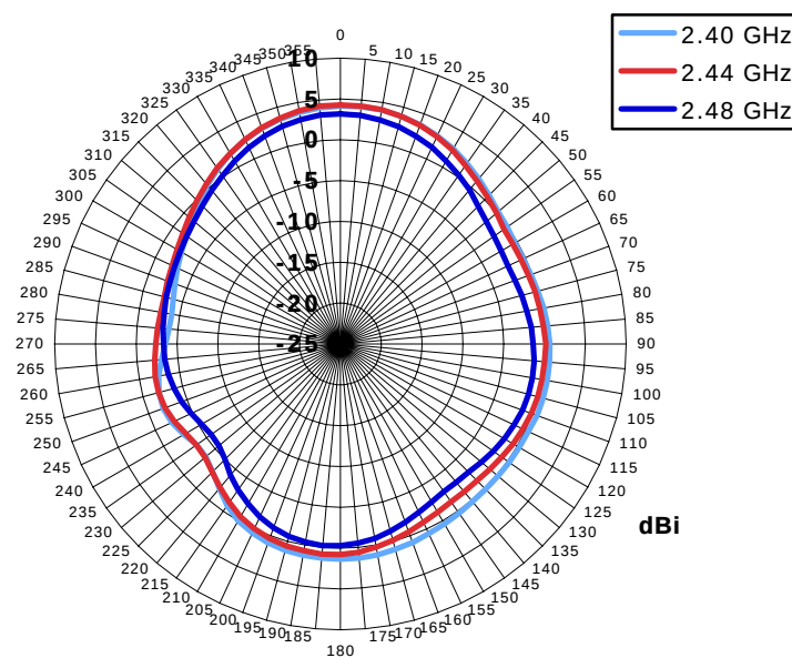
Azimuth Pattern, 2.4 GHz Band
