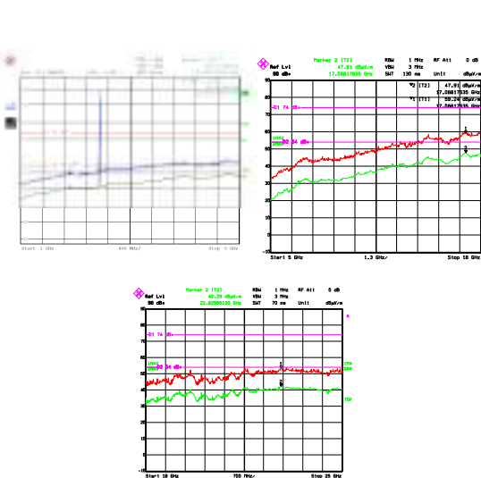
Mid channel
