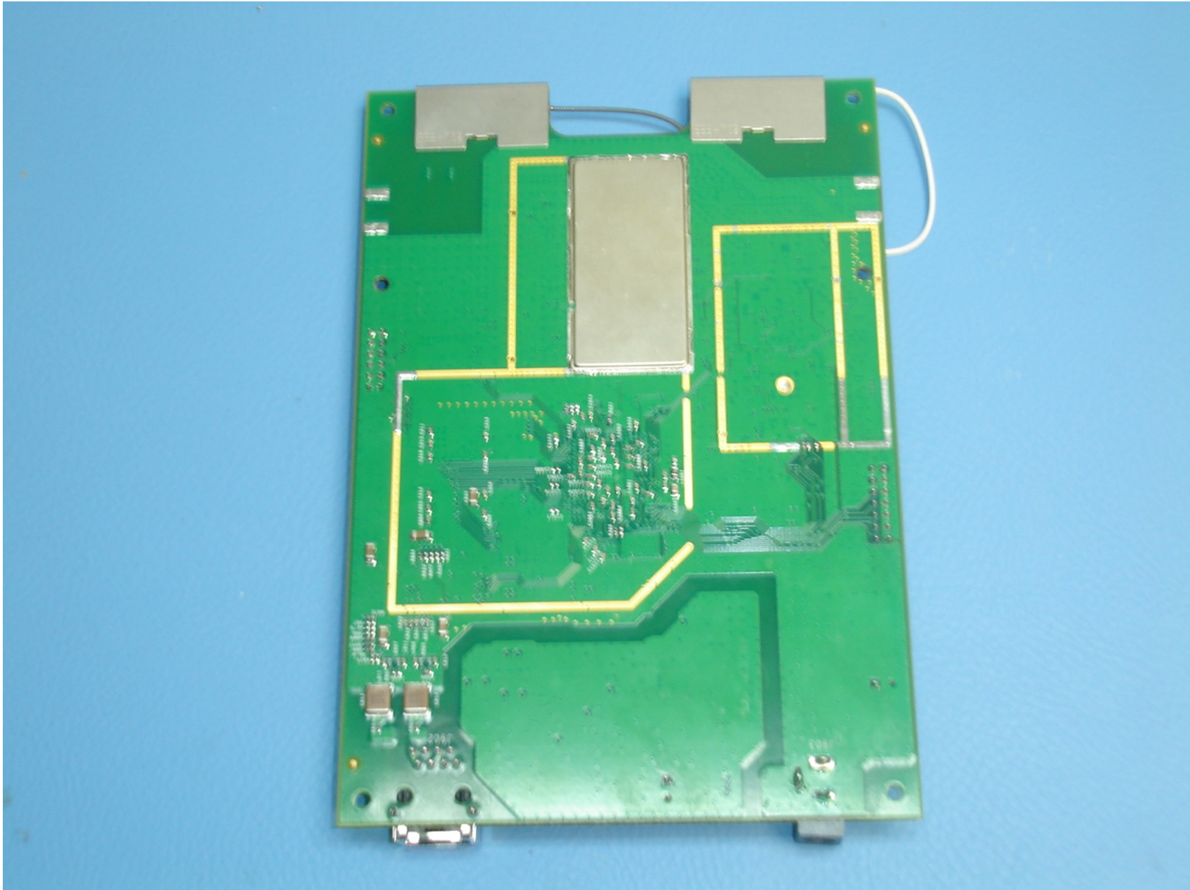
Models AP2610 or AP2630 with Internal Antennas
