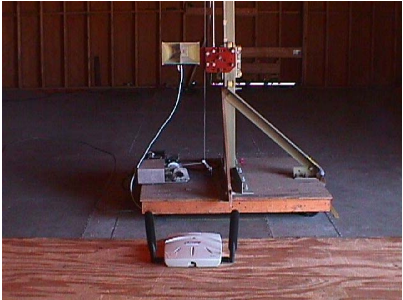
External Antenna Unit Radiated Emissions at 3 Meters (Orthogonal Position # 1)
