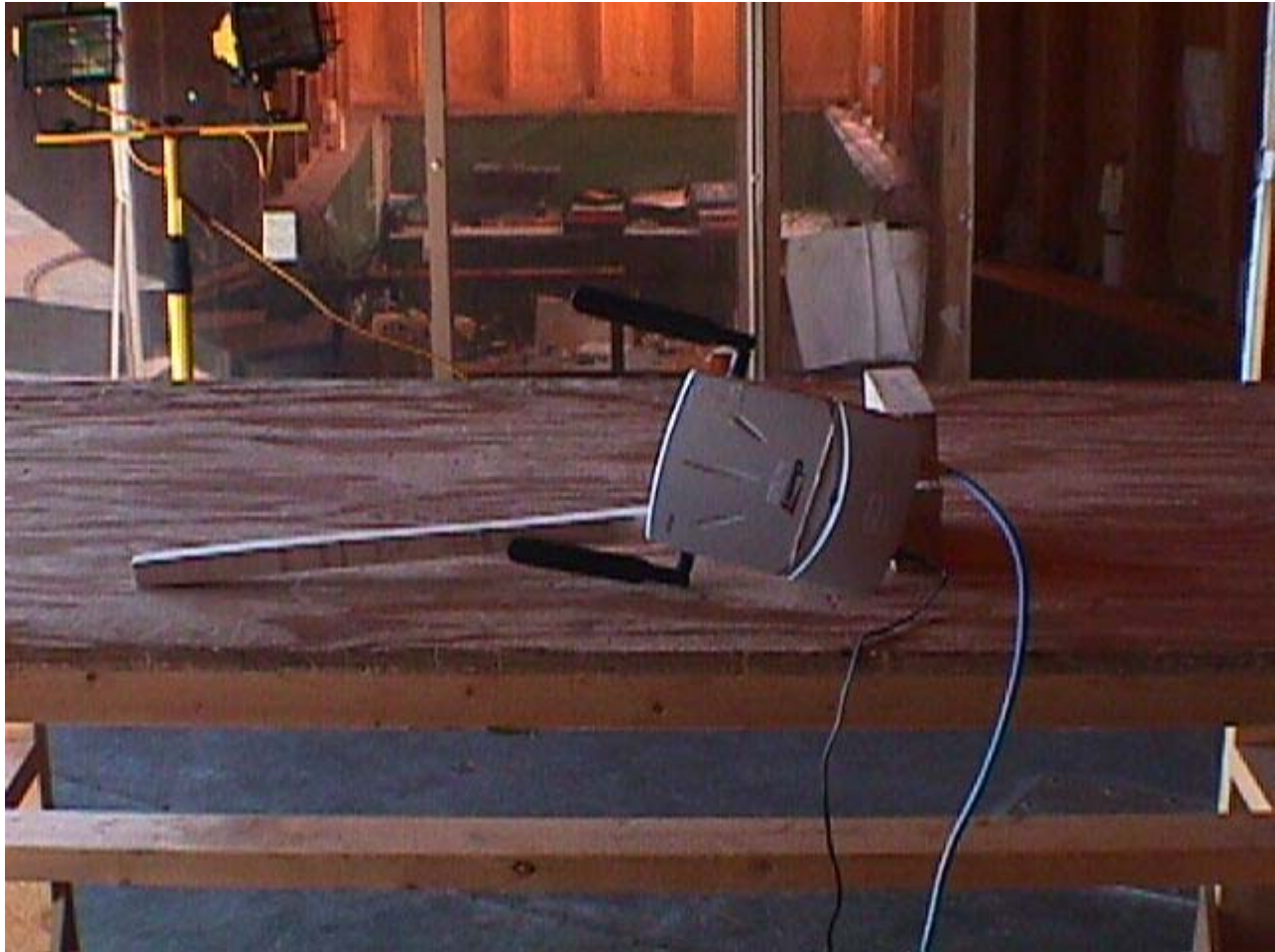
External Antenna Unit Radiated Emissions at 3 Meters (Orthogonal Position # 3)
