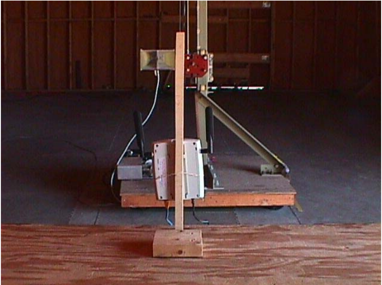
External Antenna Unit Radiated Emissions at 3 Meters (Orthogonal Position # 2)
