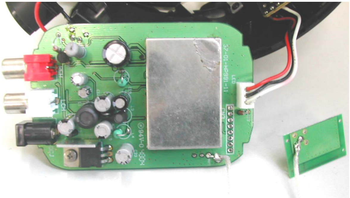
Top View of the Transmitter's Inner Circuit
