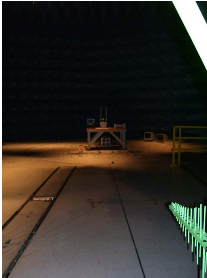
Photograph 3. Radiated Emission Test Setup 30 MHz - 1 GHz
