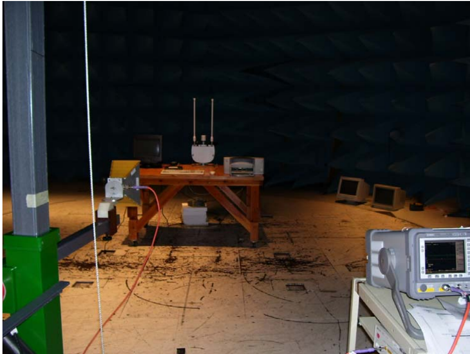
Photograph 4. Radiated Emission Limits Test Setup 1 - 2GHz
