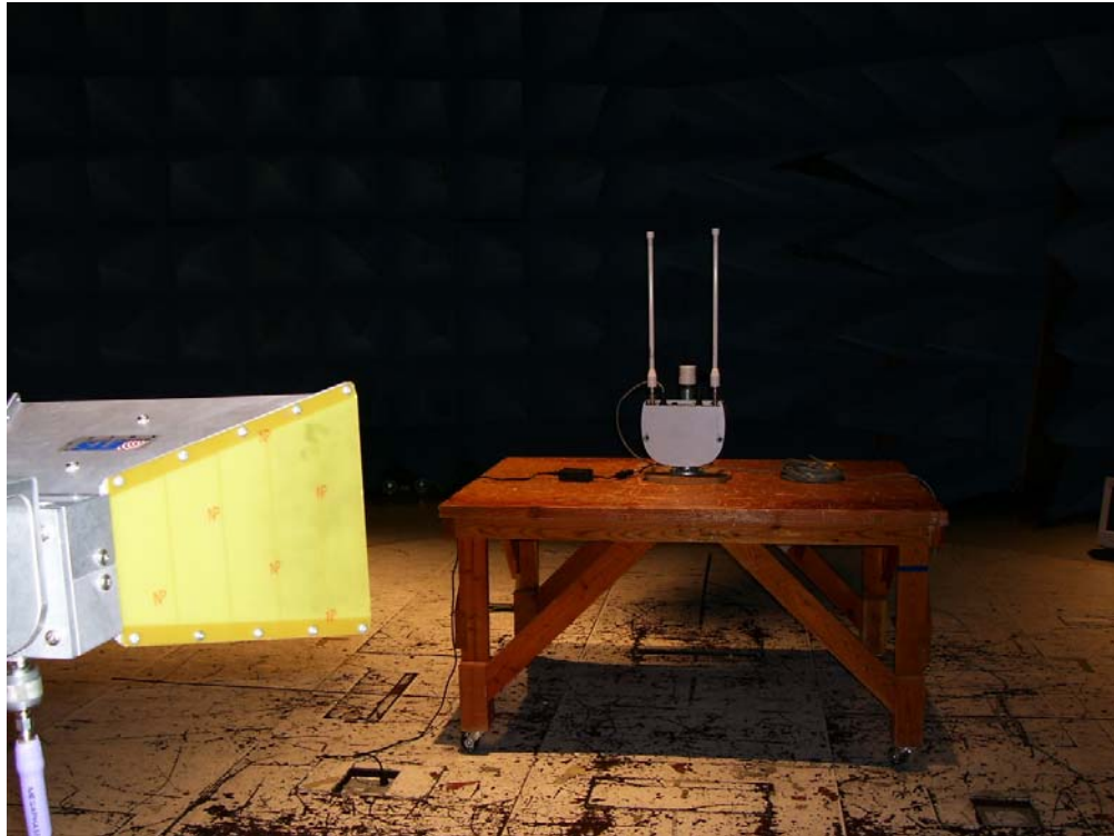
Photograph 6. Test Equipment and setup for various Radiated Measurements
