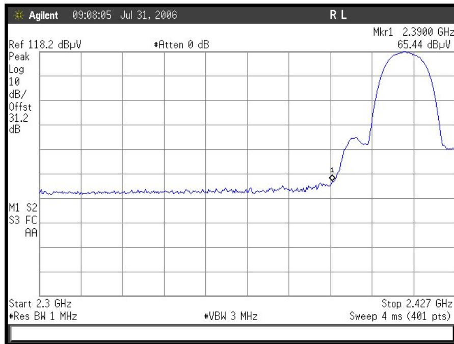
802.11/b radiated restricted band 2310- 2390 MHz Peak
