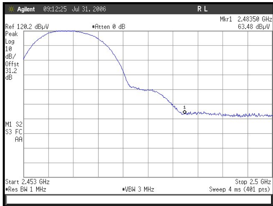
802.11/b radiated restricted band 2483.5 – 2500MHz Peak
