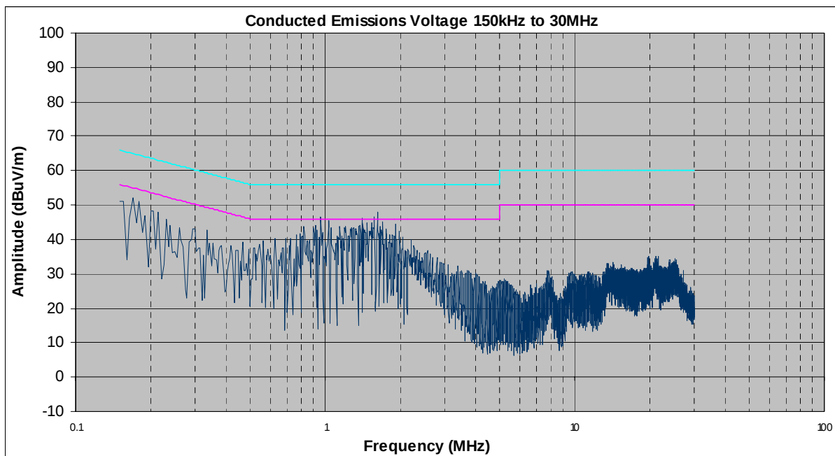
Conducted Emission, Neutral Plots
