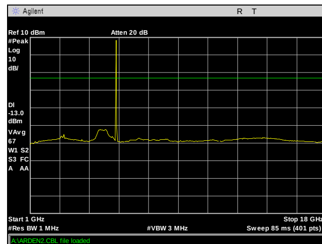
Plot 18. Conducted Spurious Emissions, 1 GHz – 18 GHz – 13 dBm, 10 MHz, Ch. 5920M, 16 dBi
