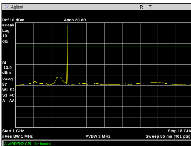
Plot 28. Conducted Spurious Emissions, 1 GHz – 18 GHz – 13 dBm, 10 MHz, Ch. 5920M, 19 dBi
