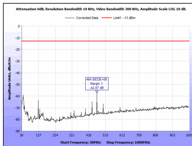
Plot 45. Radio Spurious Emissions, 30 MHz – 1 GHz – 13 dBm, 10 MHz, Ch. 5860M
