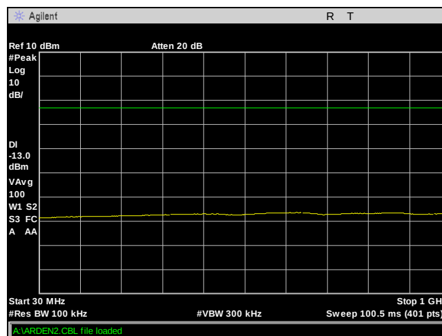
Plot 23. Conducted Spurious Emissions, 30 MHz – 1 GHz – 13 dBm, 10 MHz, Ch. 5920M, 16 dBi
