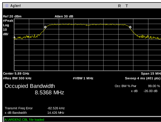
Plot 2. Occupied Bandwidth, 10 MHz, Ch. 5890M, 16 dBi, TP15.5
