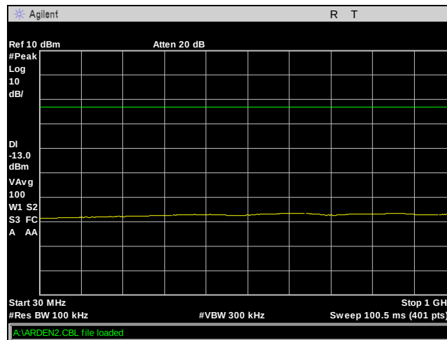
Plot 21. Conducted Spurious Emissions, 30 MHz – 1 GHz – 13 dBm, 10 MHz, Ch. 5860M, 16 dBi
