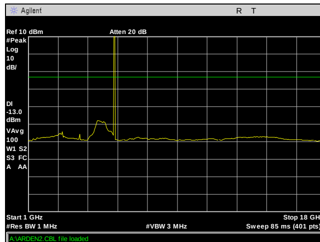
Plot 17. Conducted Spurious Emissions, 1 GHz – 18 GHz – 13 dBm, 10 MHz, Ch. 5890M, 16 dBi
