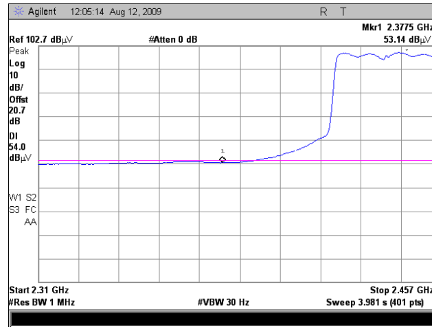
Plot 89. Lower Band Edge, Average, 2.4 GHz, Combined Ports, 802.11n 40MHz, 13 dBi Sector
