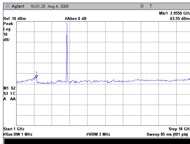
Plot 111. Radiated Spurious Emissions, High Channel, 5 GHz, 802.11a 20MHz, 19 dBi Panel
