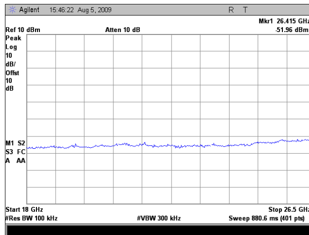
Plot 183. Conducted Emissions, High Channel, 5 GHz, Port 1, 802.11n 20MHz, 18 GHz – 26.5 GHz
