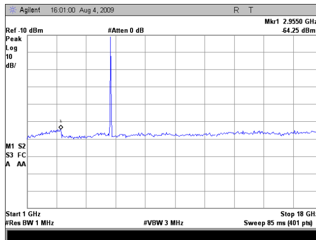
Plot 110. Radiated Spurious Emissions, Mid Channel, 5 GHz, 802.11a 20MHz, 19 dBi Panel
