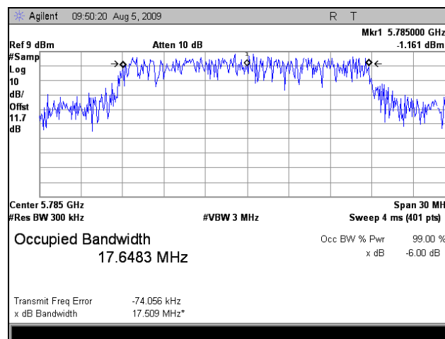
Plot 32. Occupied Band Width, Mid Channel, 5 GHz, Port 2, 802.11n 20MHz
