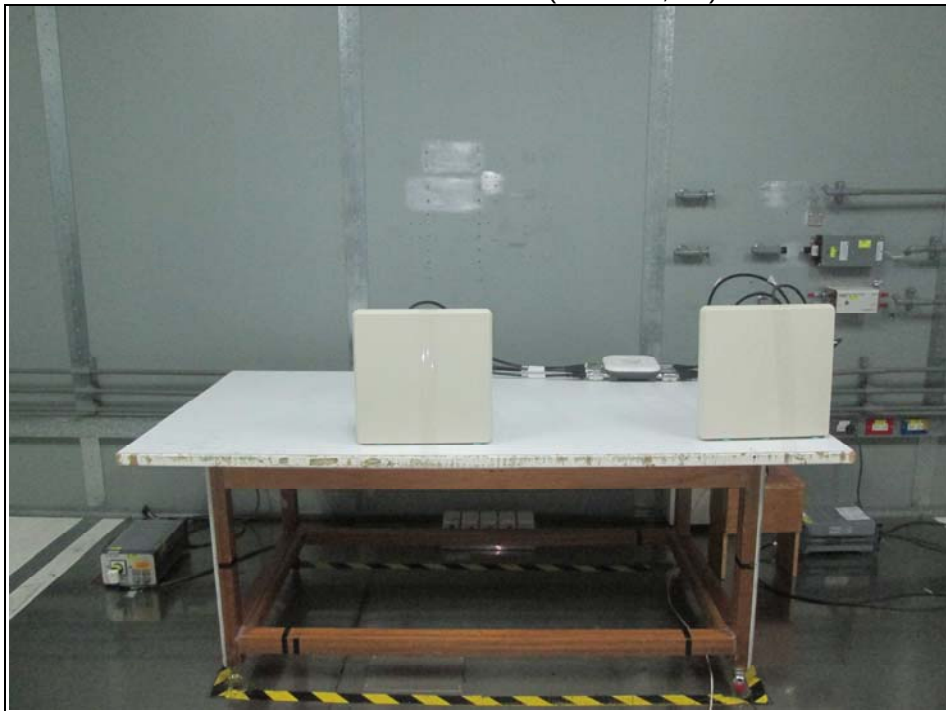
Conducted Emission Test (Mode A2, B2)
