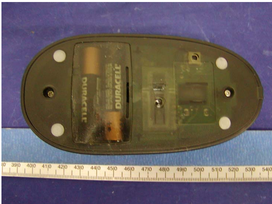
Chassis - Bottom View
