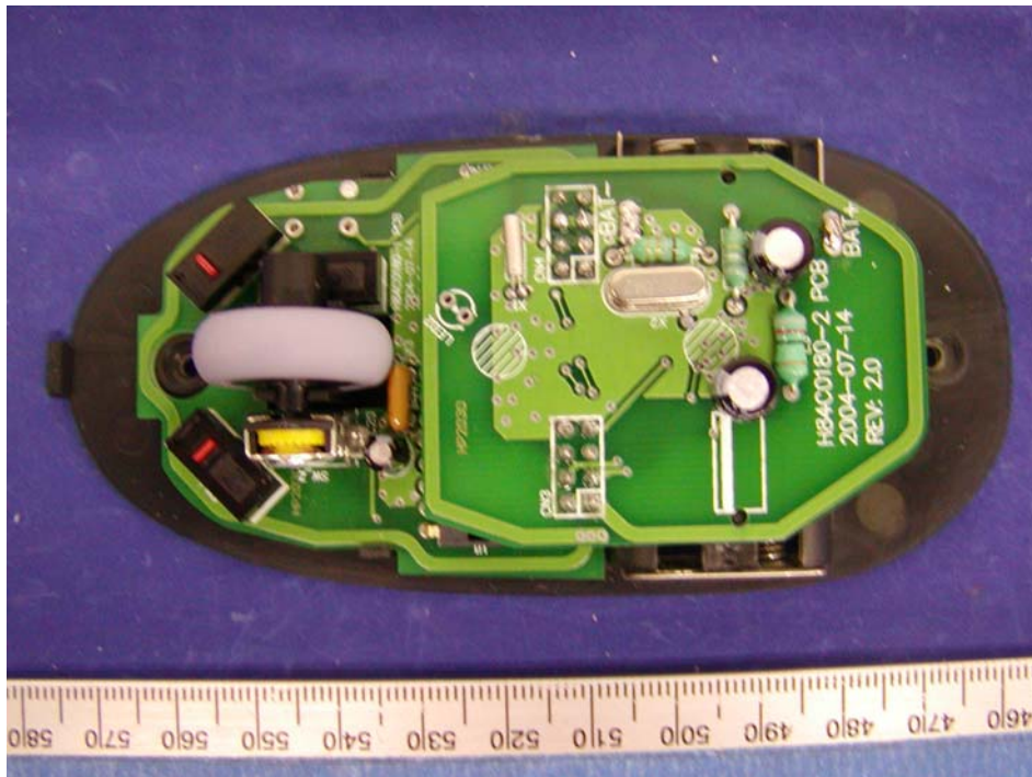
Chassis – Cover Off View
