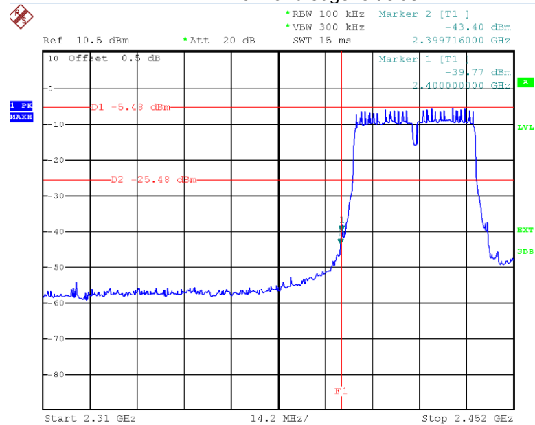
TX 11n HT40: Band edge-left side
