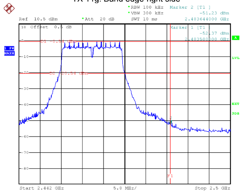
TX 11g: Band edge-right side
