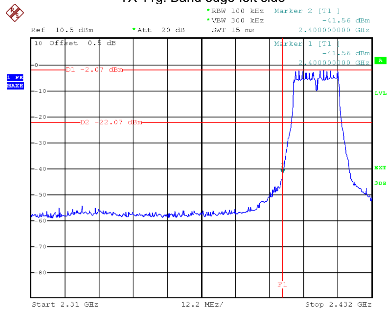
TX 11g: Band edge-left side
