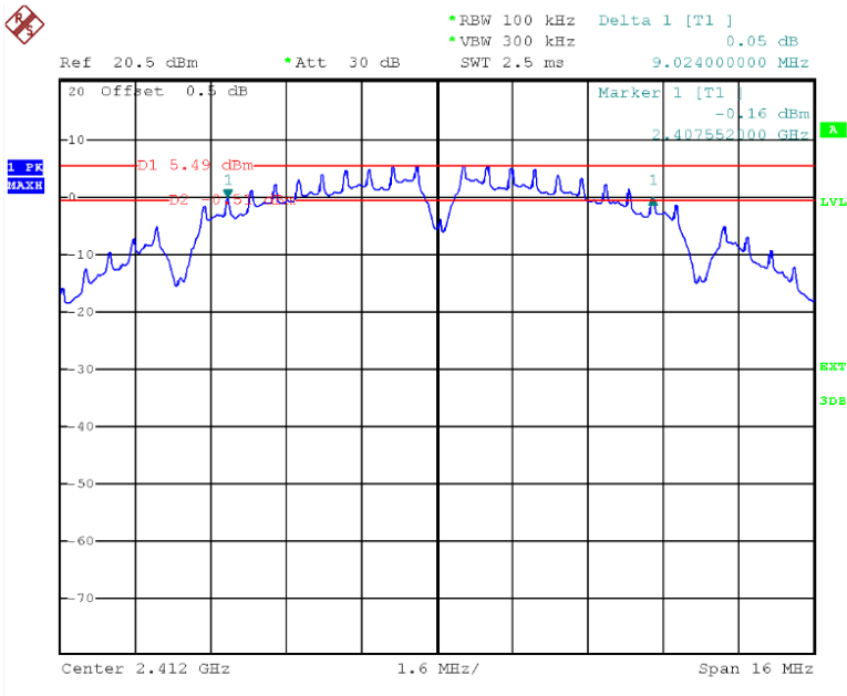
6dB Bandwidth Mode: TX 11b channel 1
