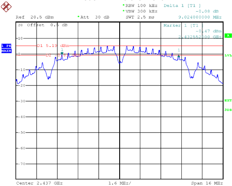
Mode: TX 11b channel 6
