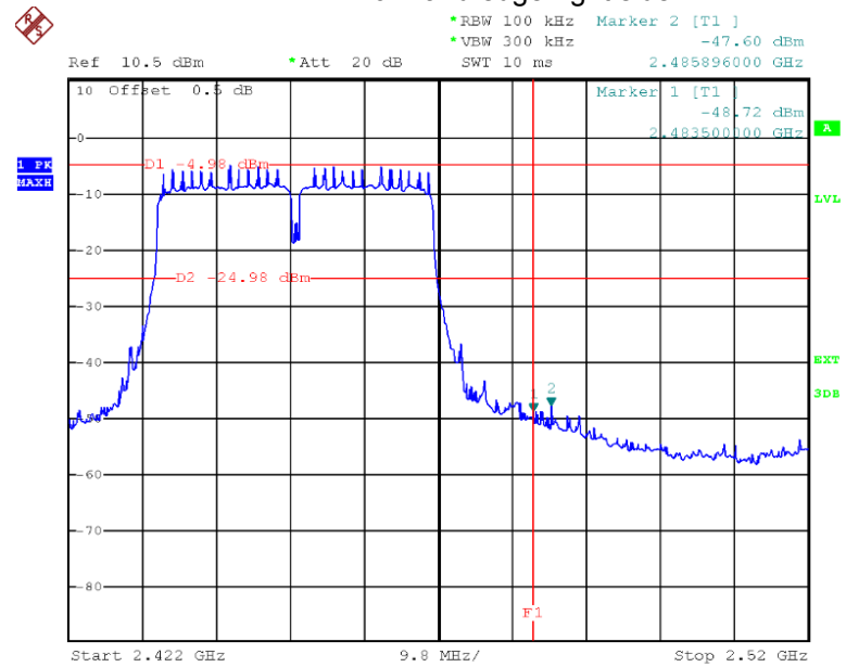
TX 11n HT40: Band edge-right side
