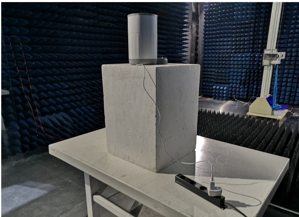
For Above 1GHz Test Site 1#
