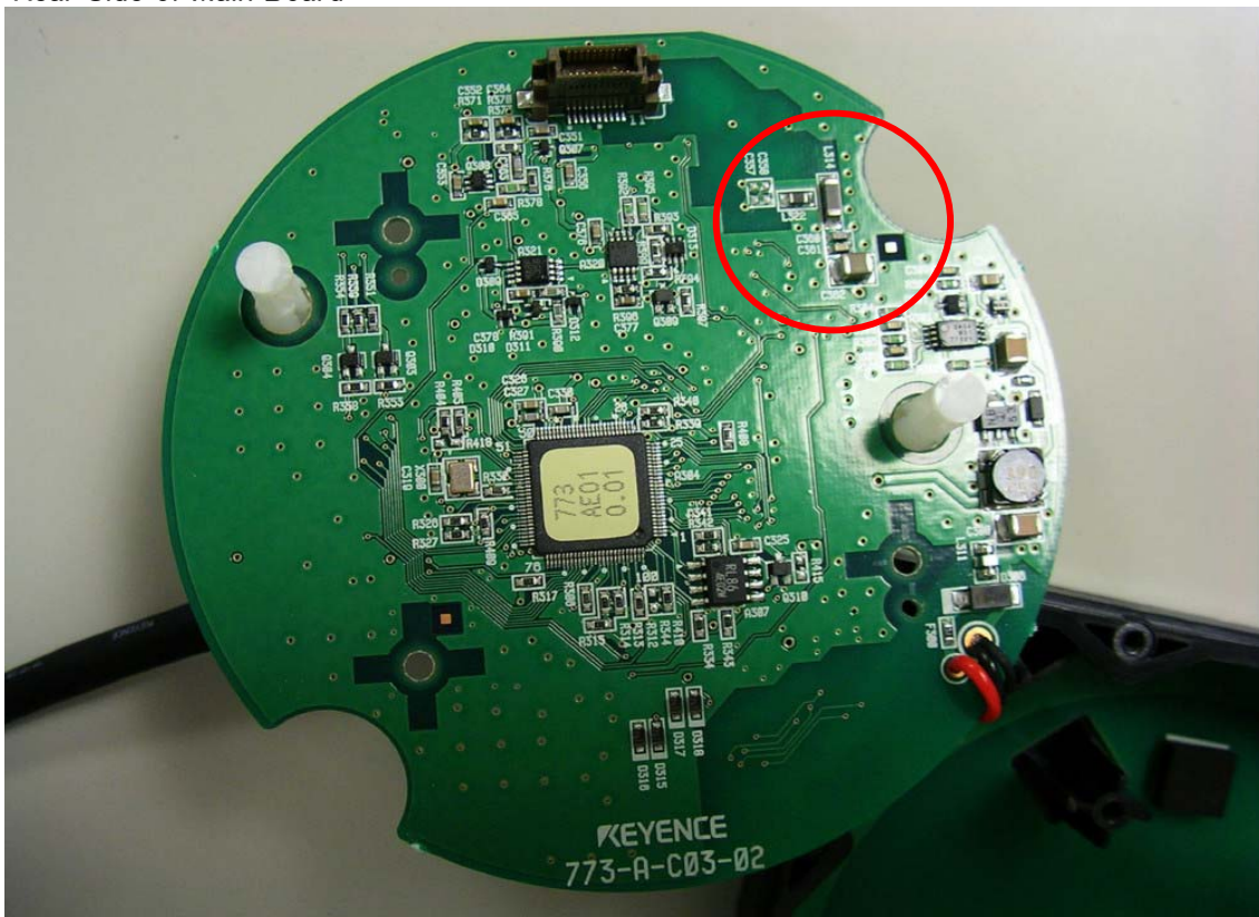
Rear Side of Main Board
