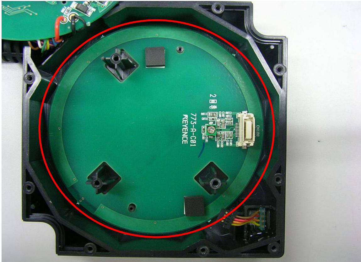
Internal View of RFID (Antenna Board)
