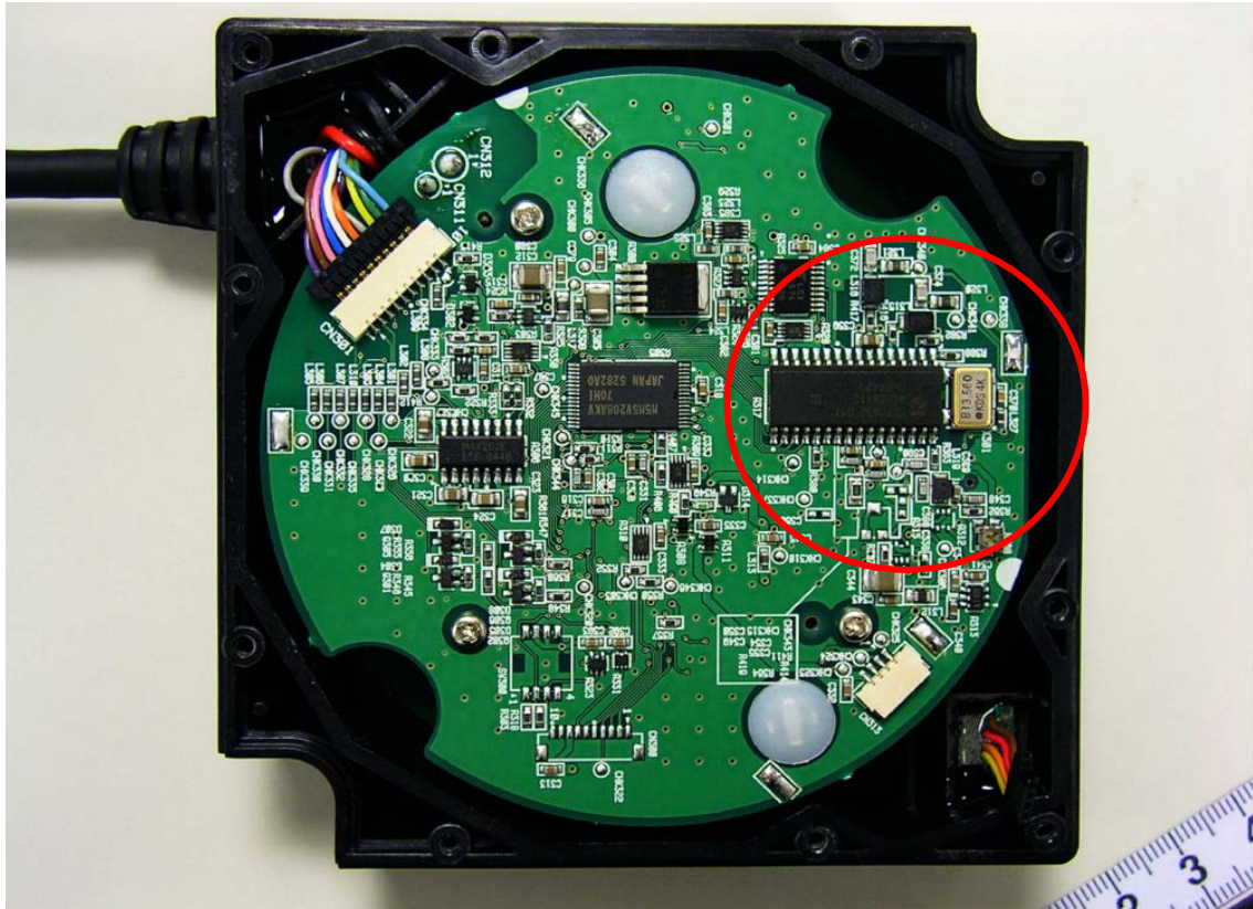
Internal View of RFID without Shield (Main Board)
