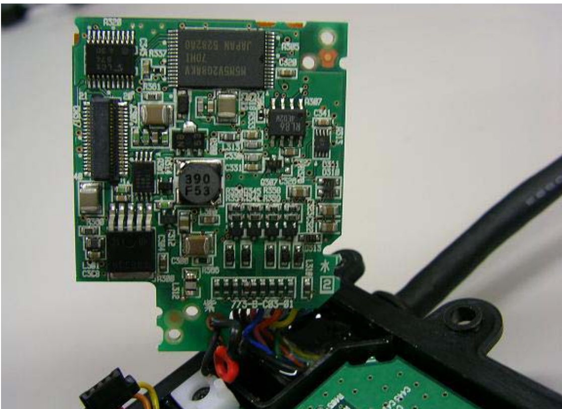
Rear Side of Digital Board
