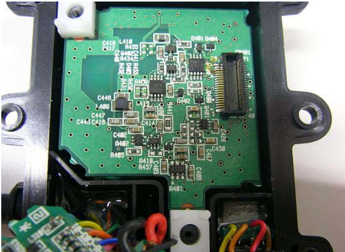
Rear Side of Analog Board
