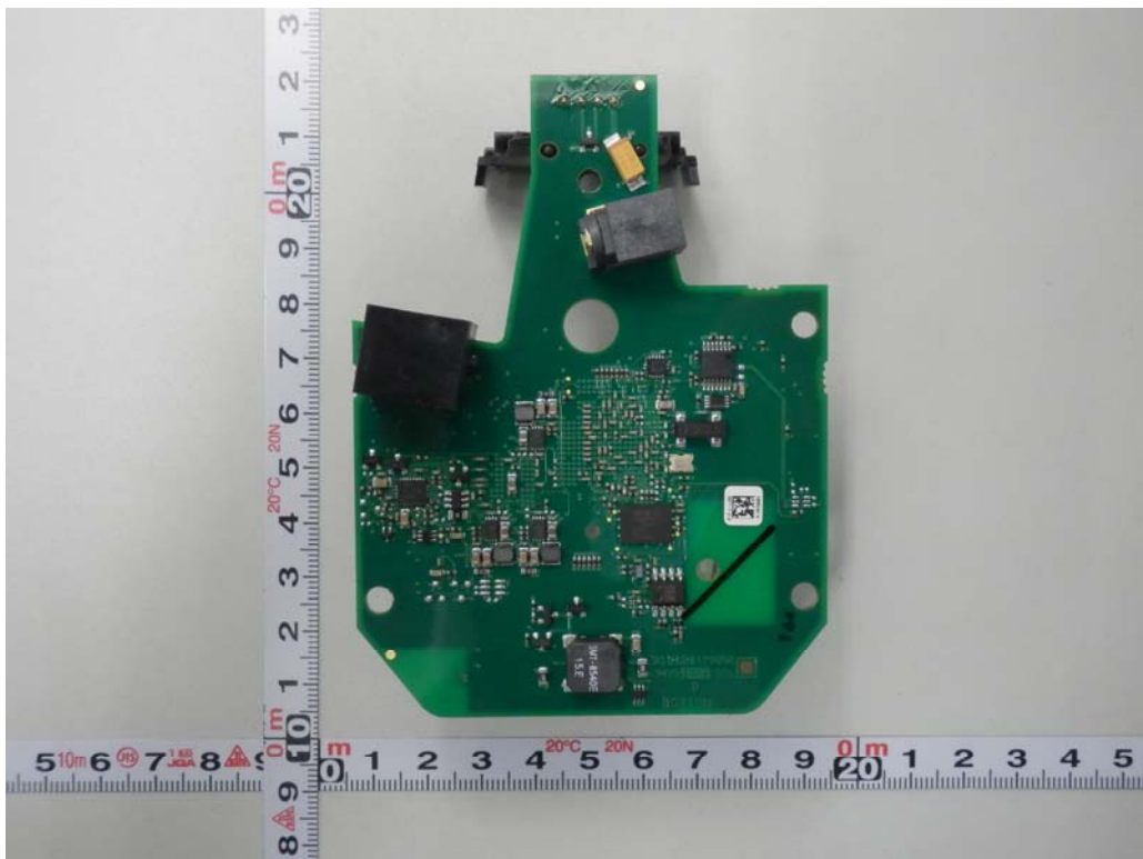
Board (Bottom)
