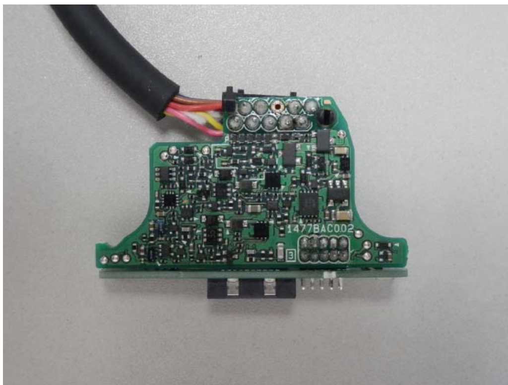
Sensor
